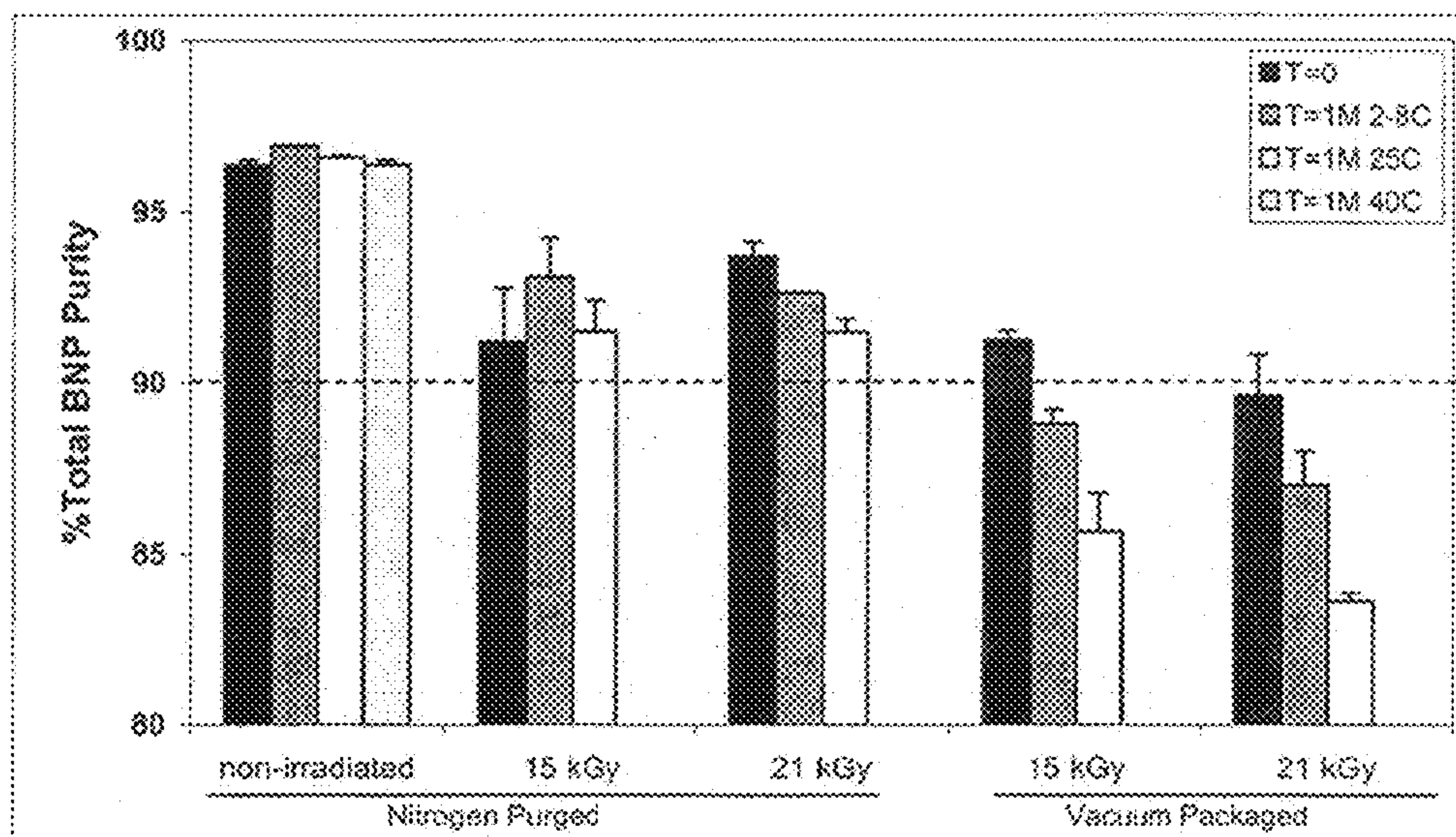
Figure 11. IM Stability Data following E-Beam Treatment
