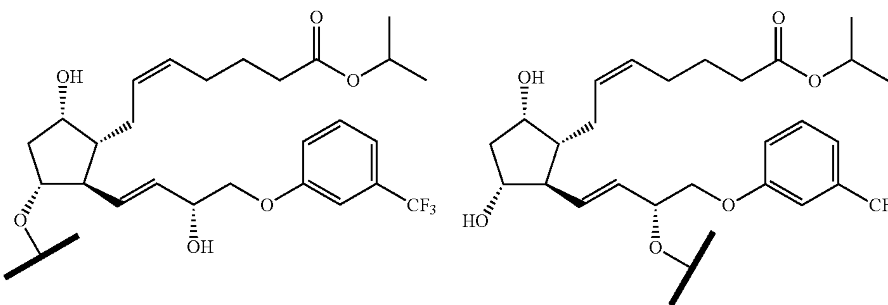
Travoprost
