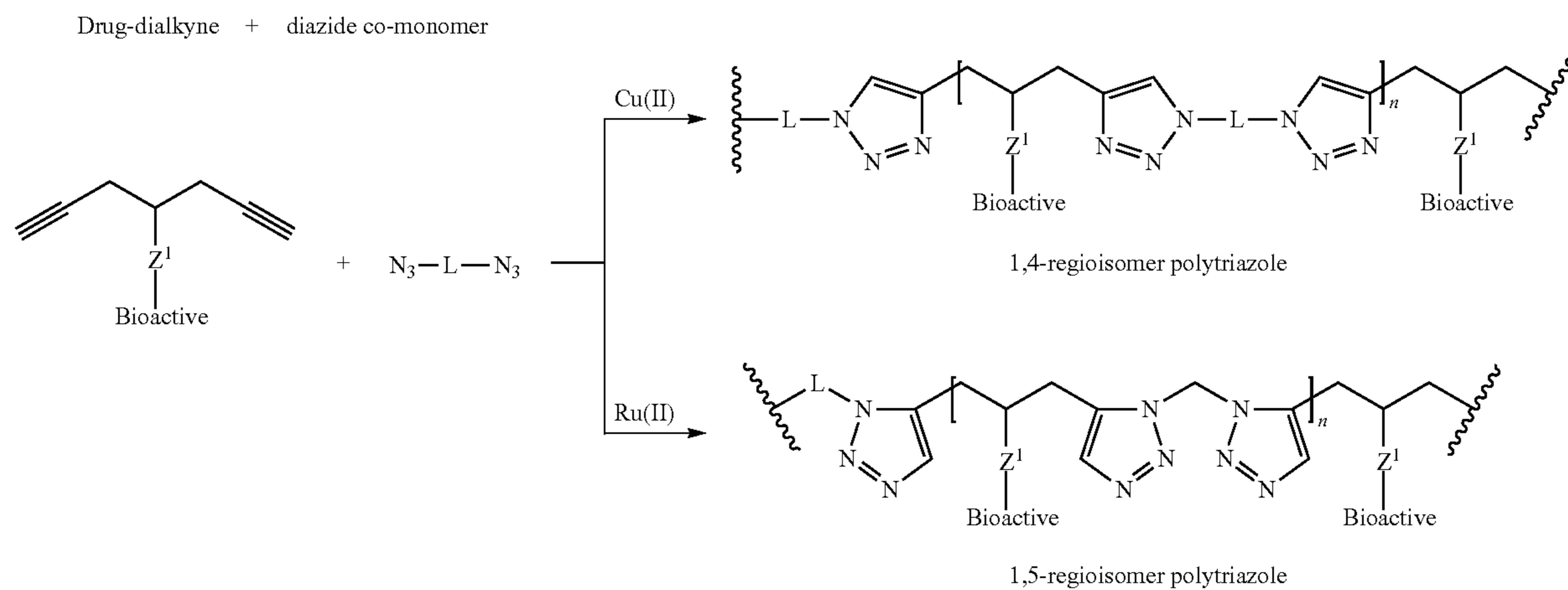
Scheme 4
