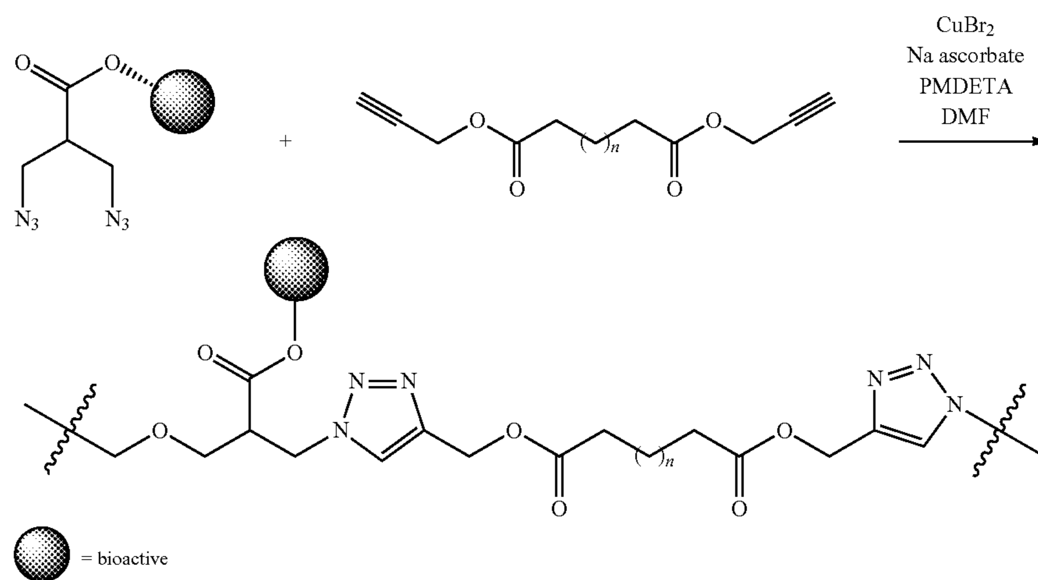
Scheme 3
