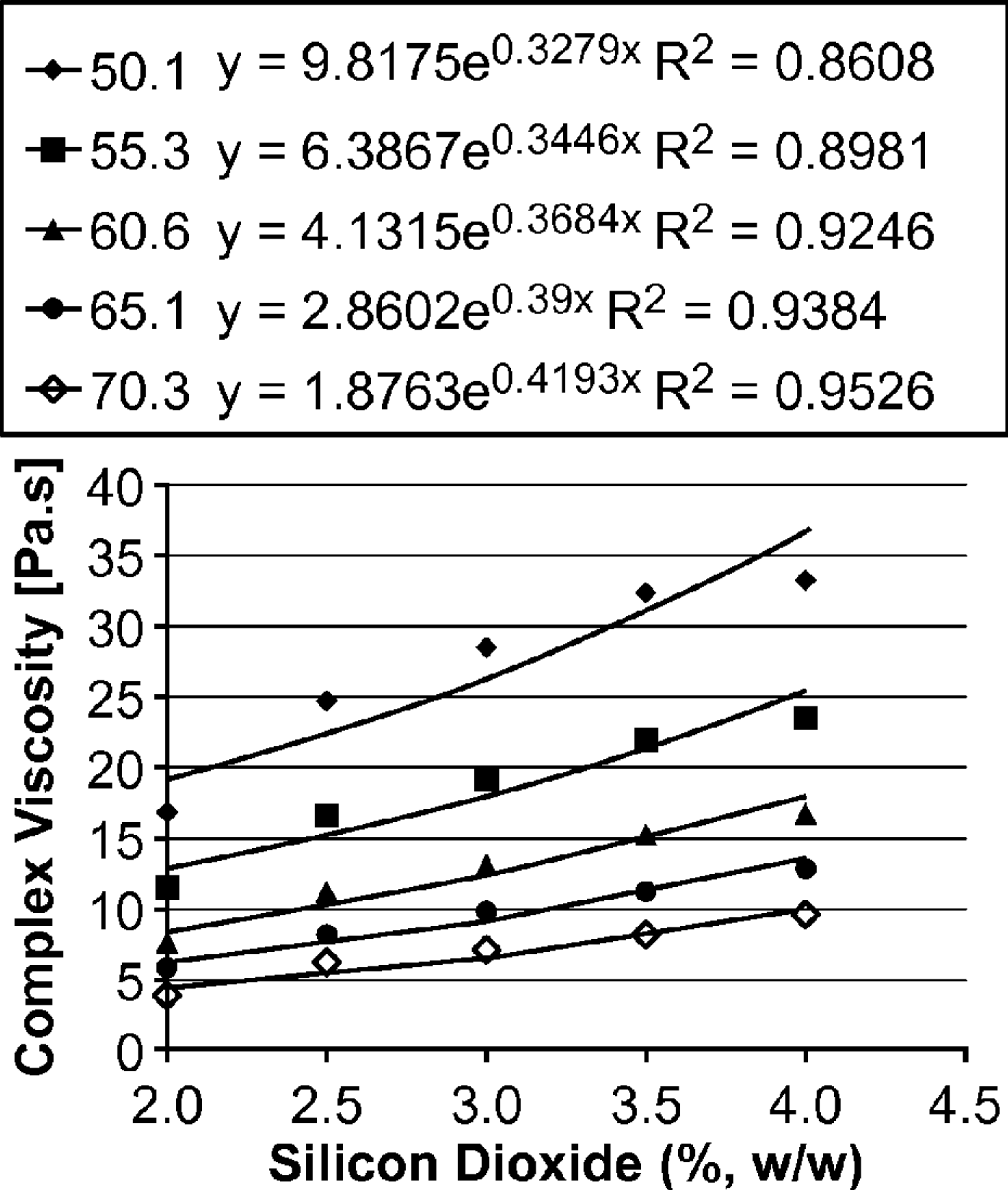
Panel A Complex Viscosity vs. SiO 2 Composition at 50-70°C
