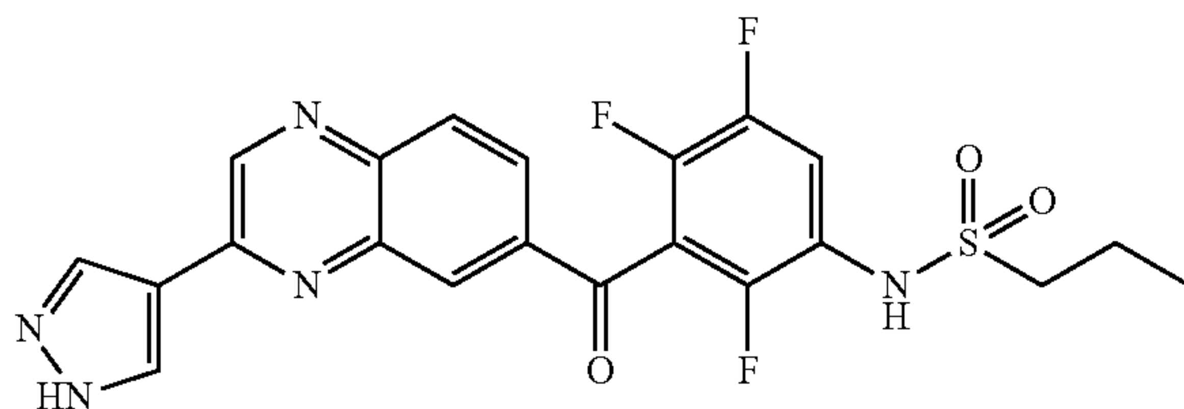
N-(3-(3-(1H-pyrazol-4-yl)quinoxaline-6-carbonyl)-2,4,5-trifluorophenyl)propane-1-sulfonamide
