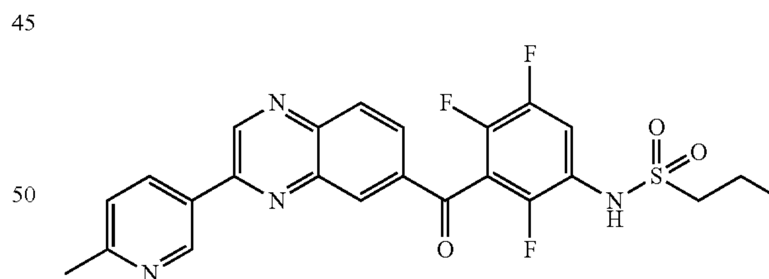
N-(2,4, 5-trifluoro-3-(3-(6-methylpyridin-3-yl)quinoxaline-6-carbonyl)phenyl)propane-1-sulfonamide
