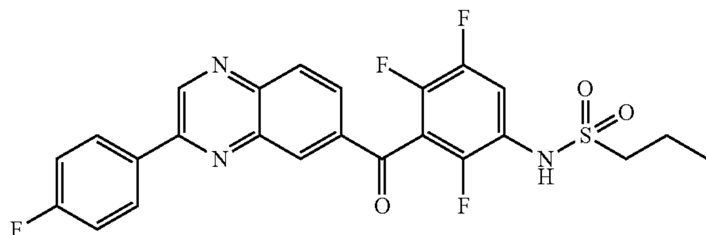
N-(2,4, 5-trifluoro-3-(3-(4-fluorophenyl)quinoxaline-6-carbonyl)phenyl)propane-1-sulfonamide
