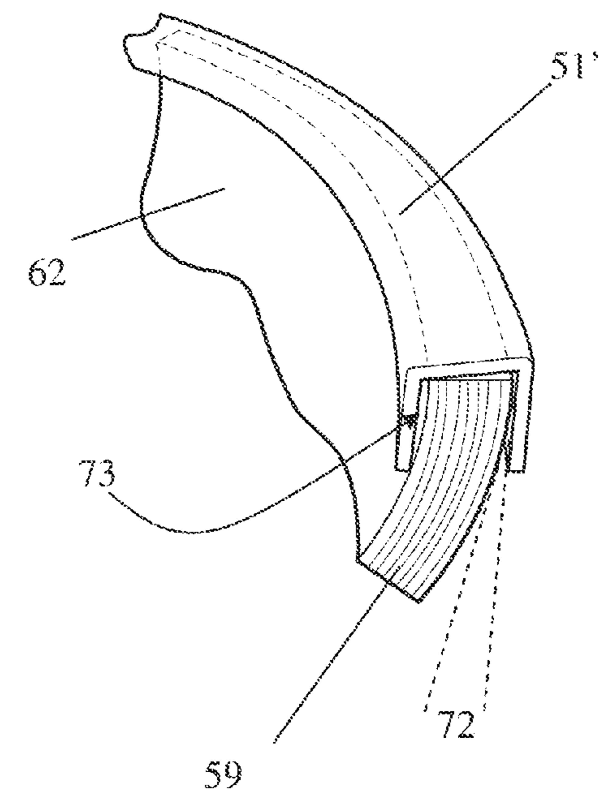
FIG. 2c (PRIOR ART)
