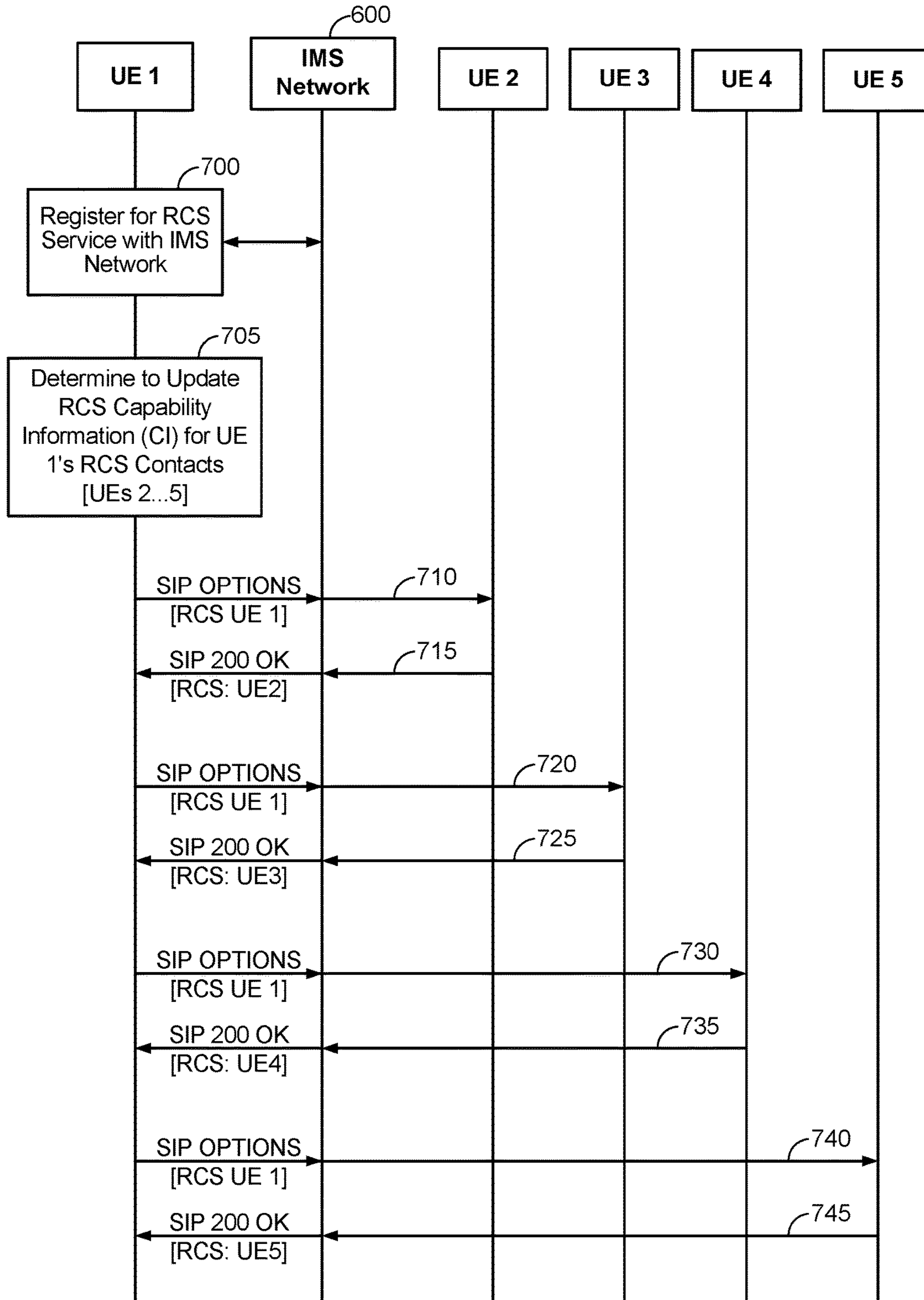
FIG. 7 – CONVENTIONAL ART
