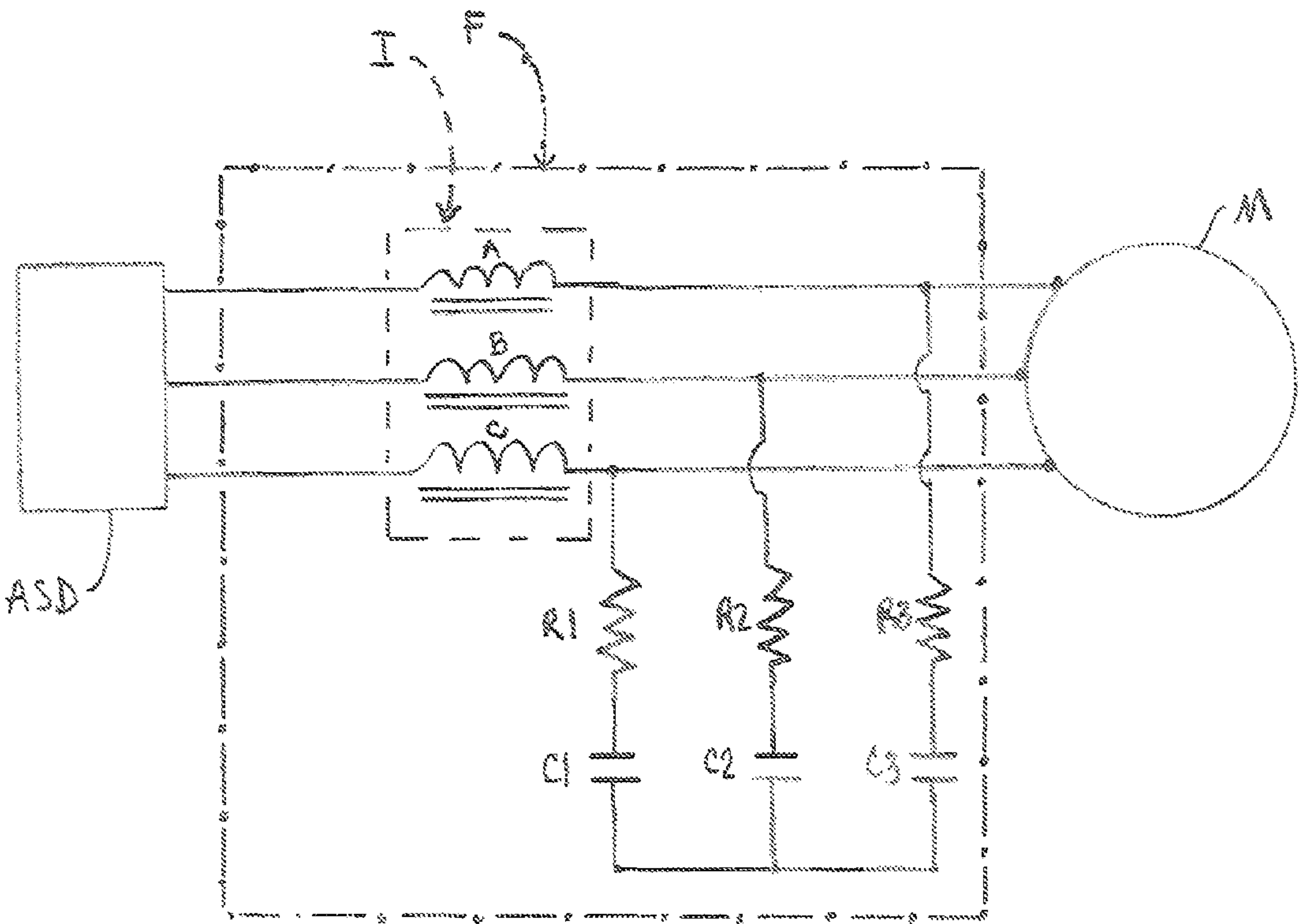
(PRIOR ART)
