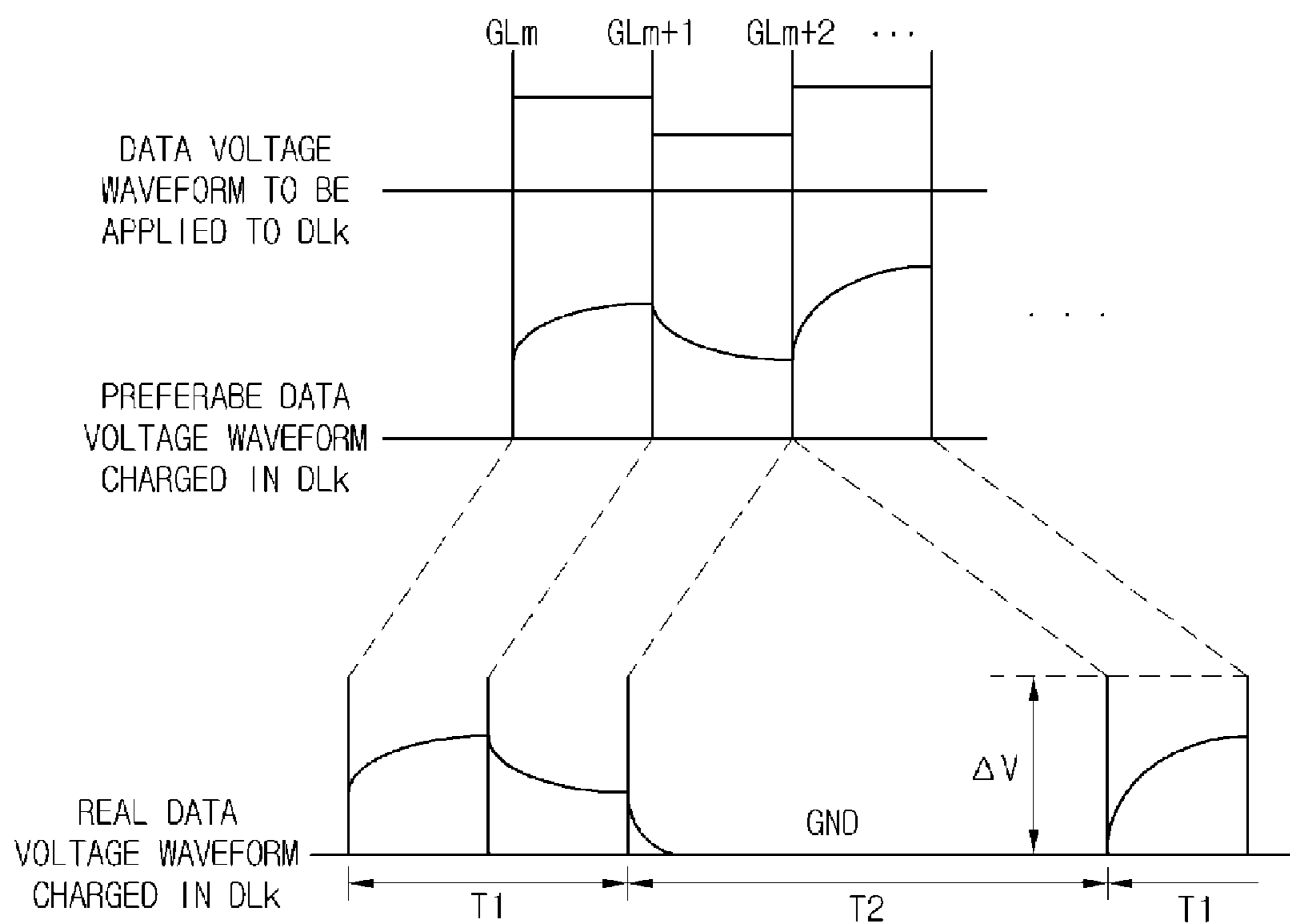
FIG. 3 (RELATED ART)
