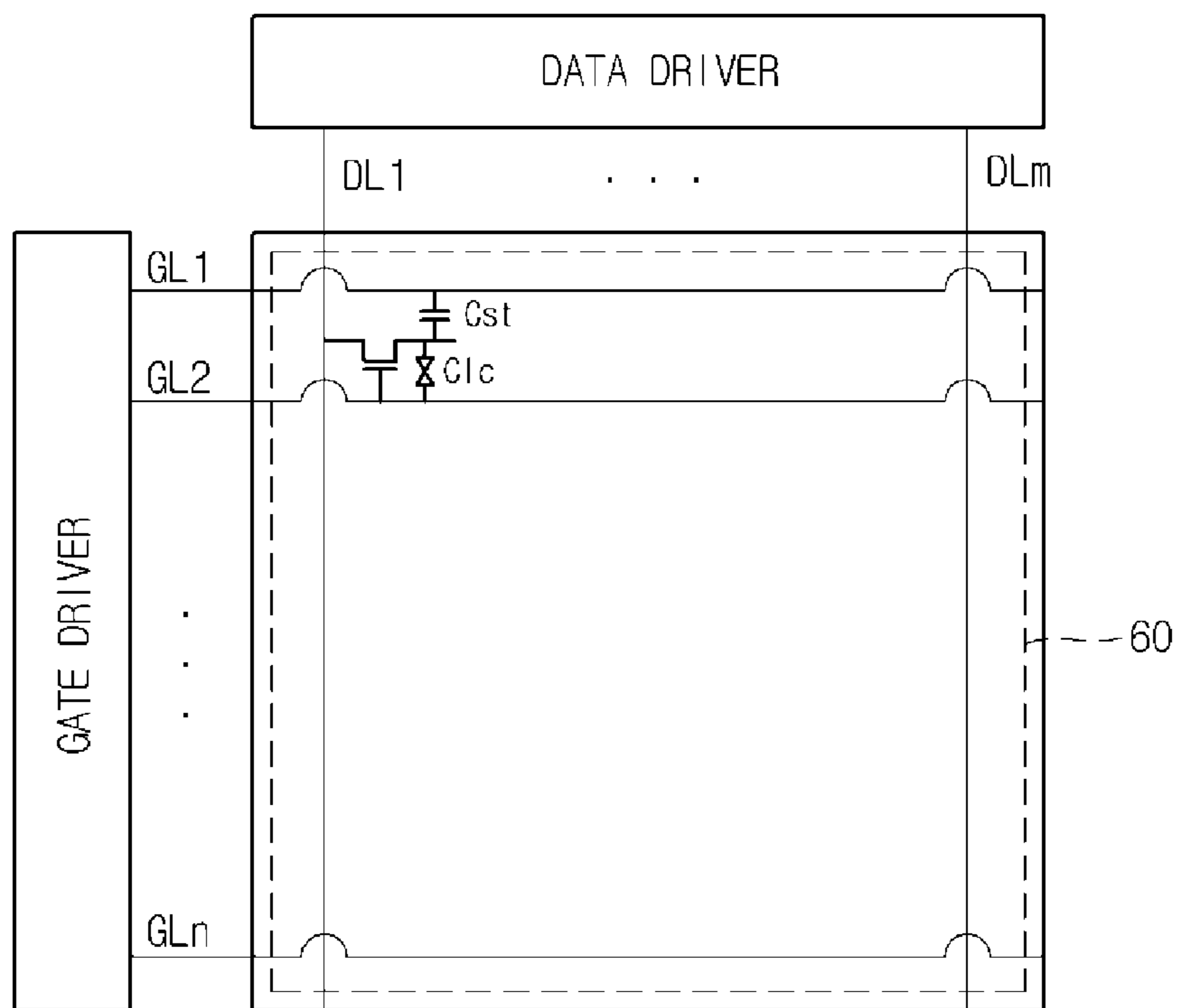
FIG. 2 (RELATED ART)
