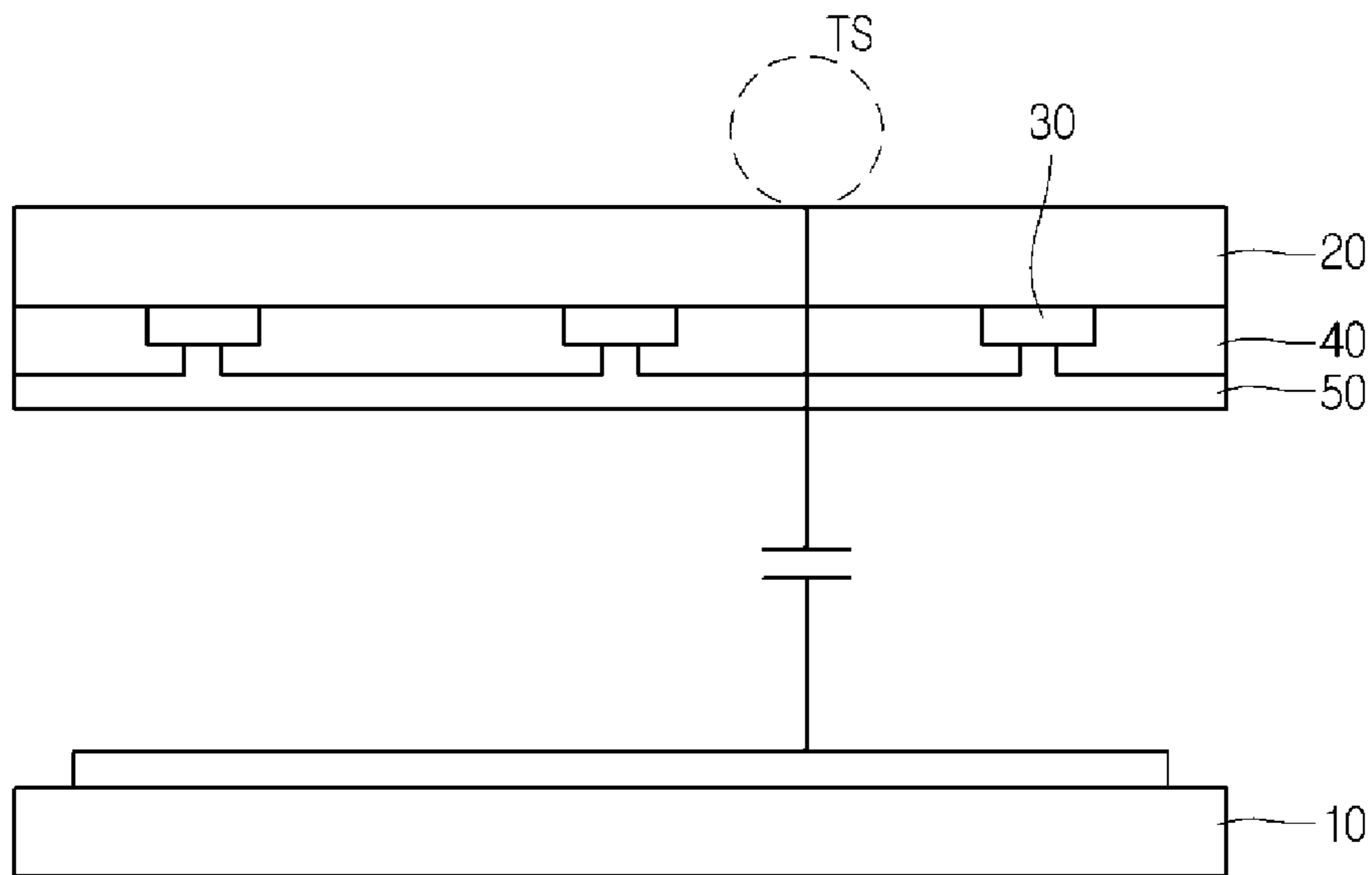
FIG. 1 (RELATED ART)
