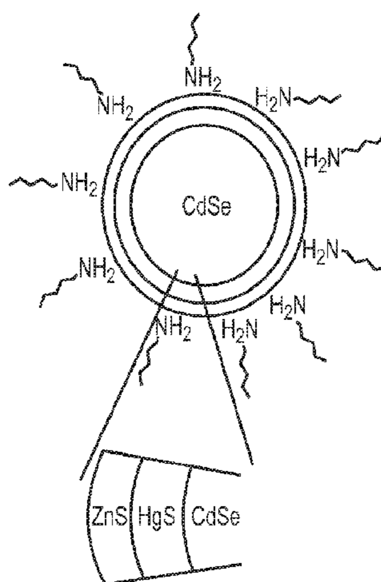
CORE-MULTI SHELL ORGANIC CAPPED PARTICLE
