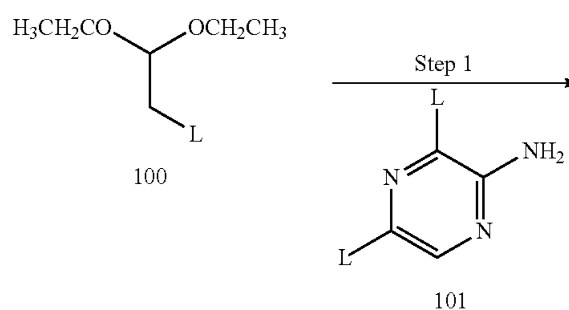
Reaction Scheme 1
