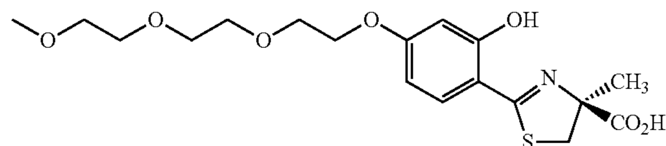
(S)-4'-(HO)-DADFT-PE
