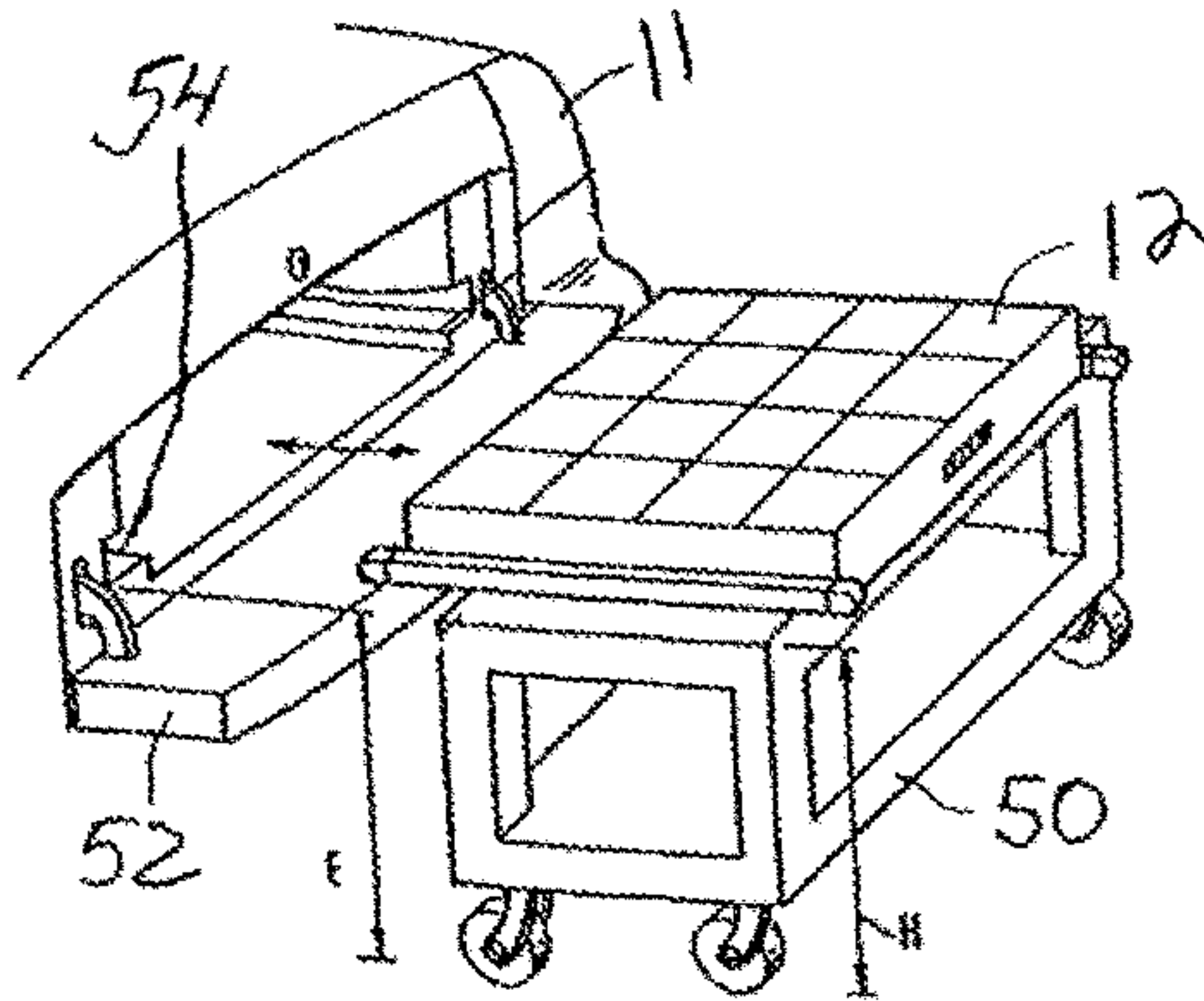
FIG. 5 PRIOR ART
