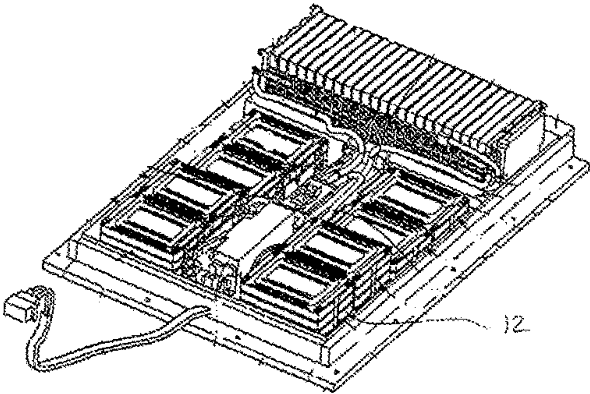
FIG. 2 PRIOR ART
