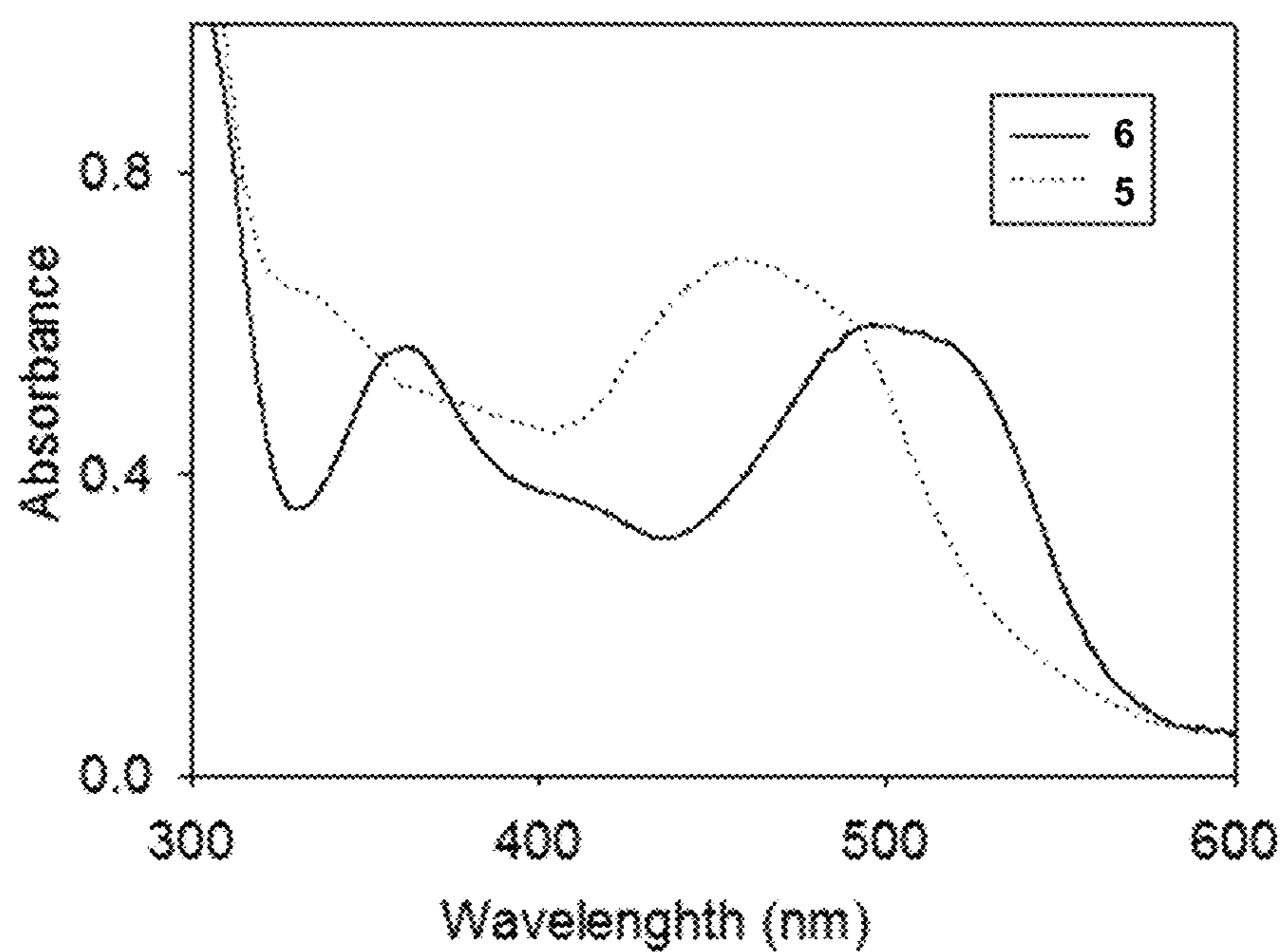
Figure 20. UV-vis Spectra of Ru-complexes 6 (Solid line) and 5 (dotted line) in CH 2 Cl 2 .
