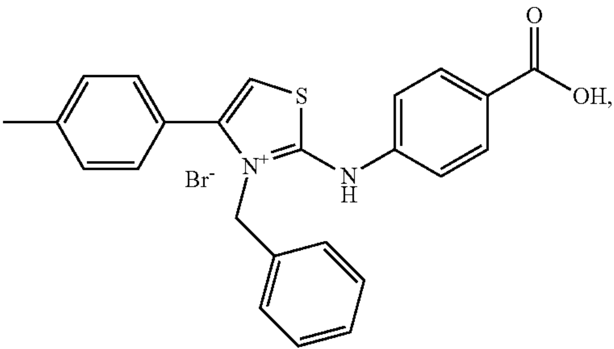
Compound 127
