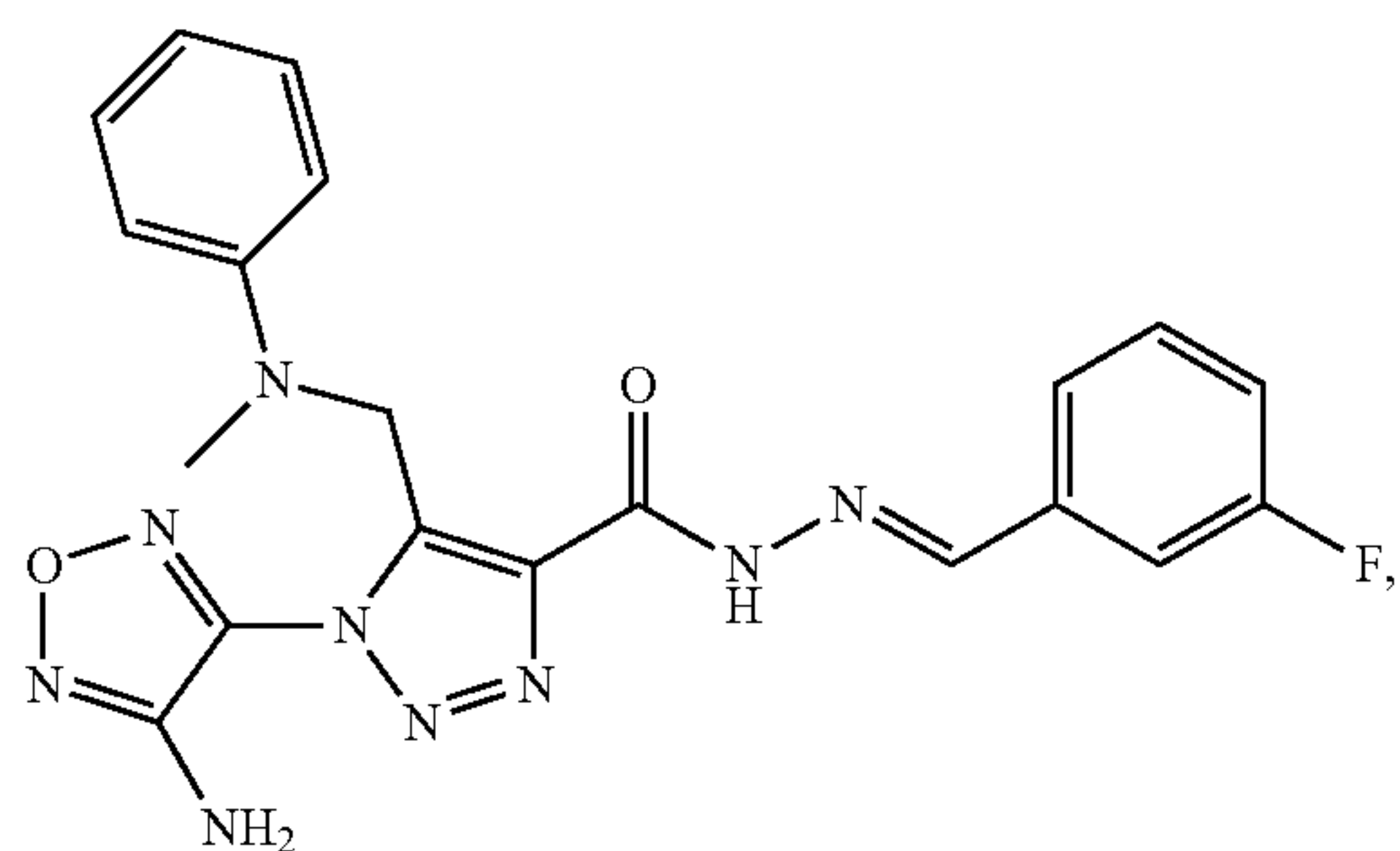
Compound 98
