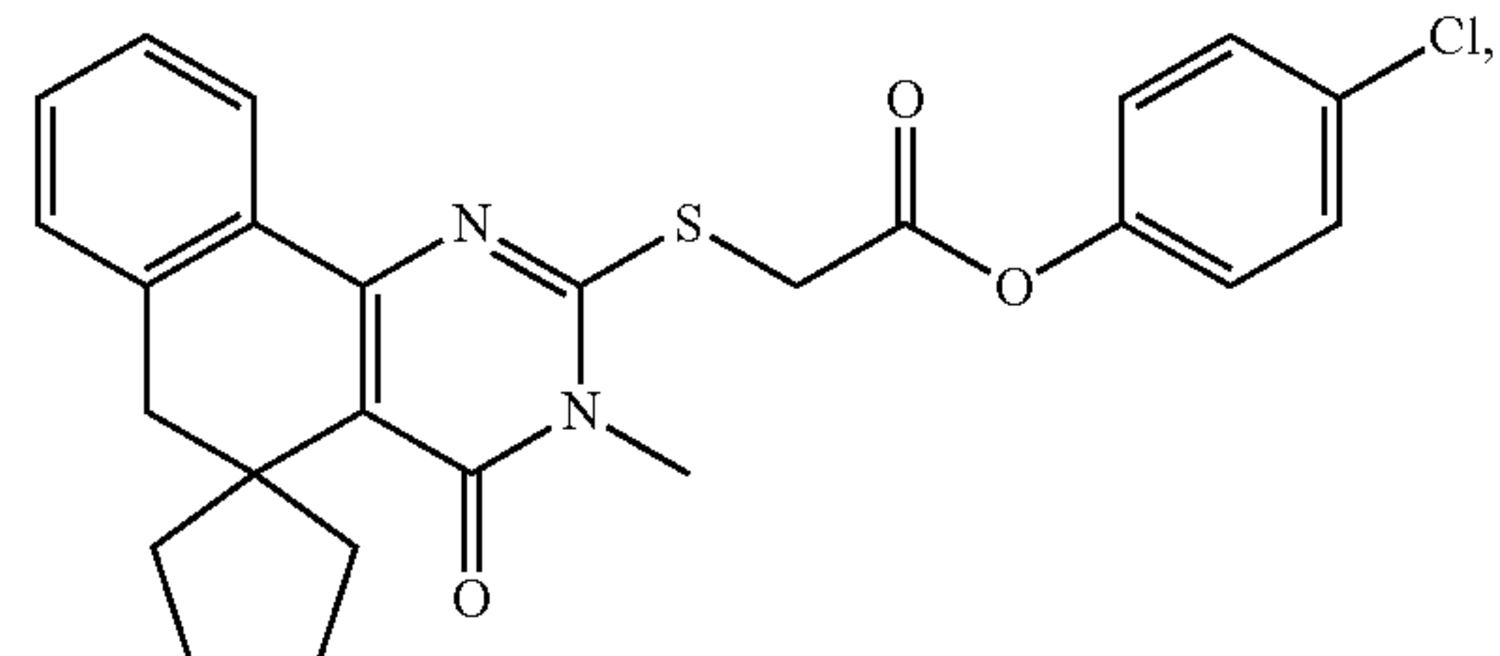
Compound 246
