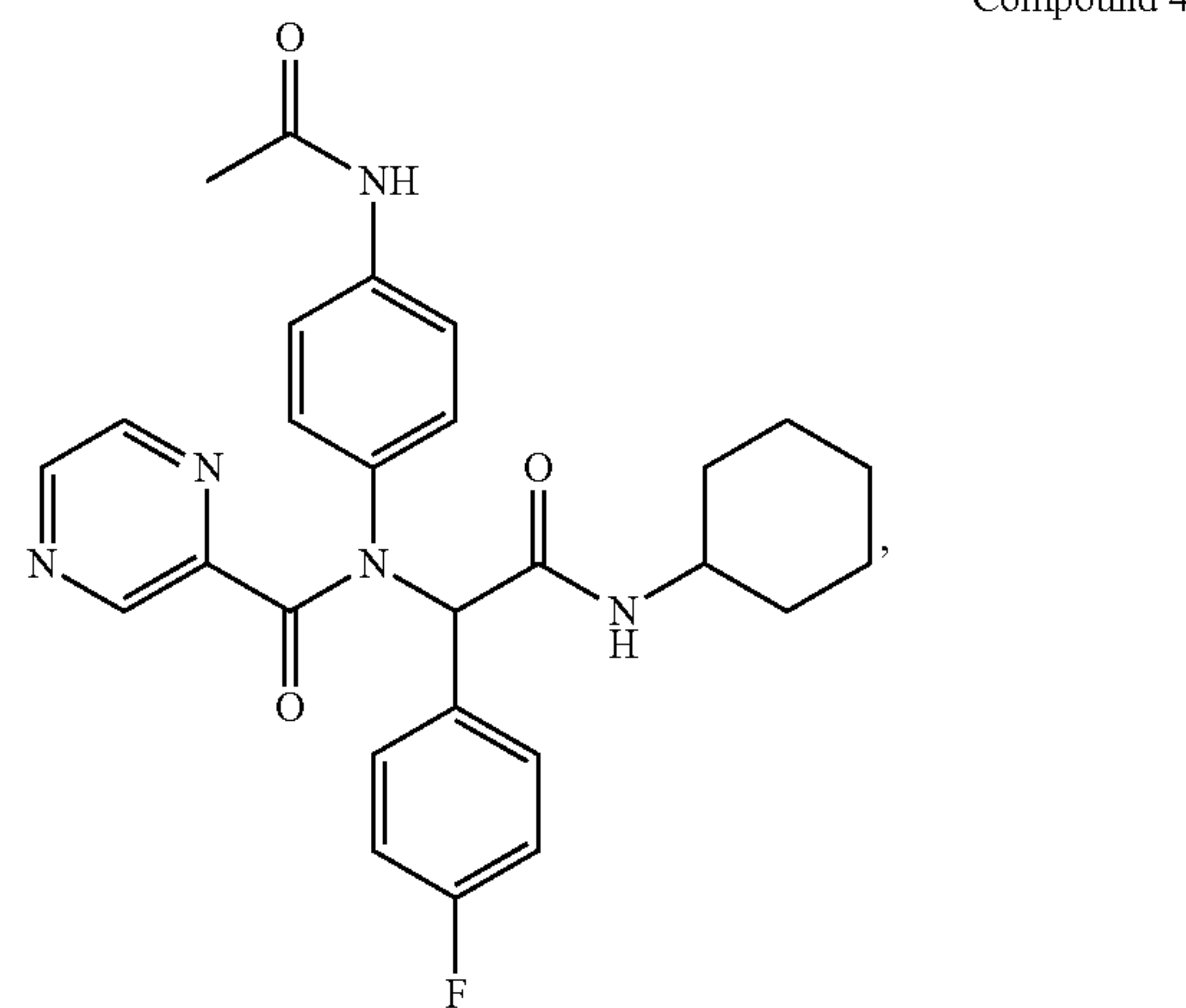
Compound 44
