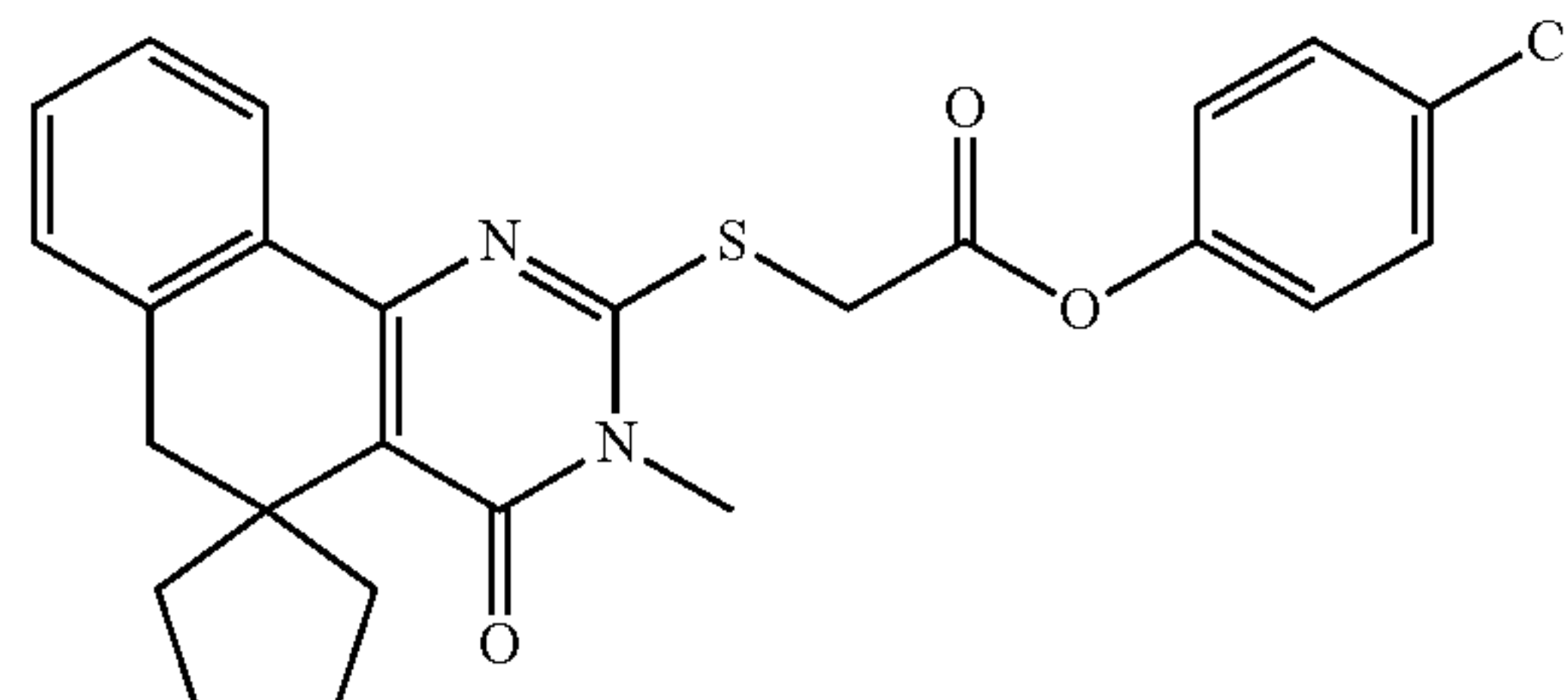
Compound 246
