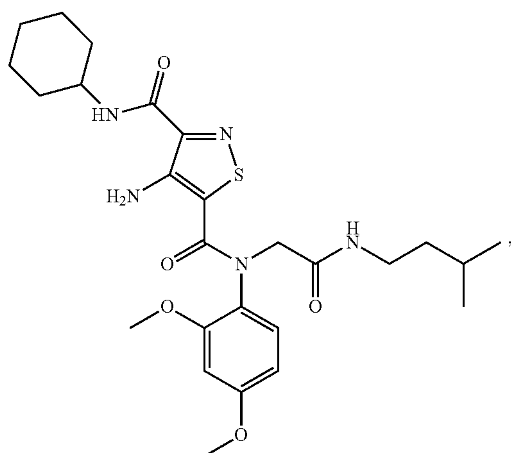
Compound 99
