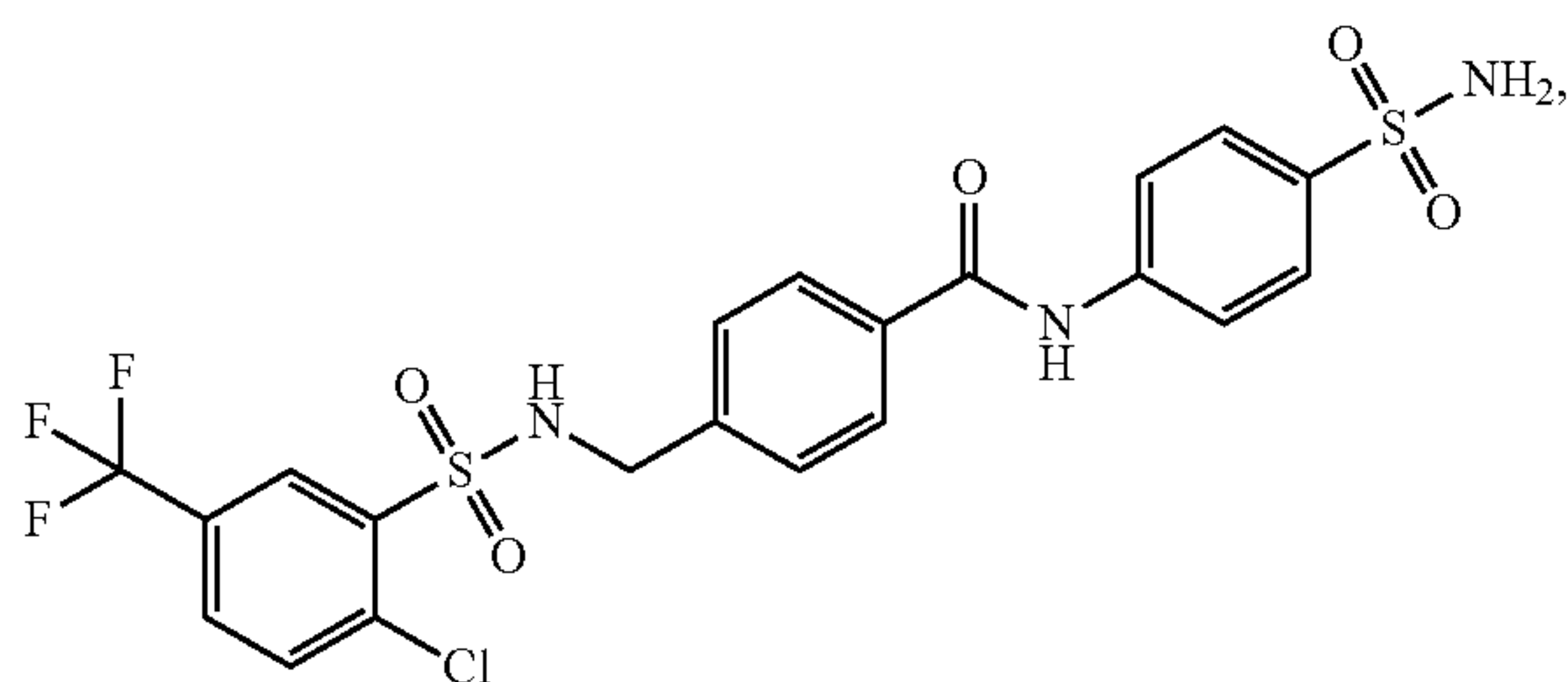
Compound 208
