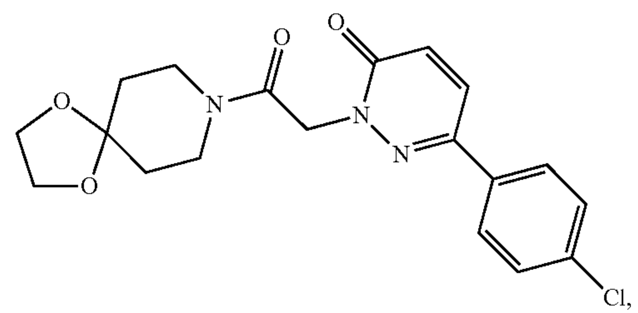
Compound 222
