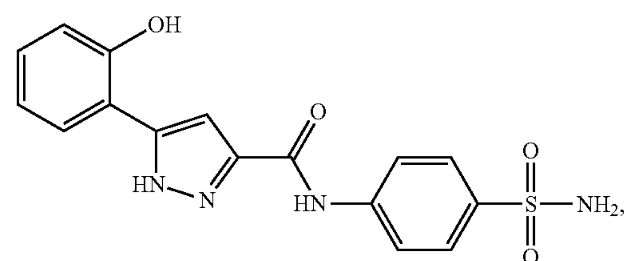
Compound 105
