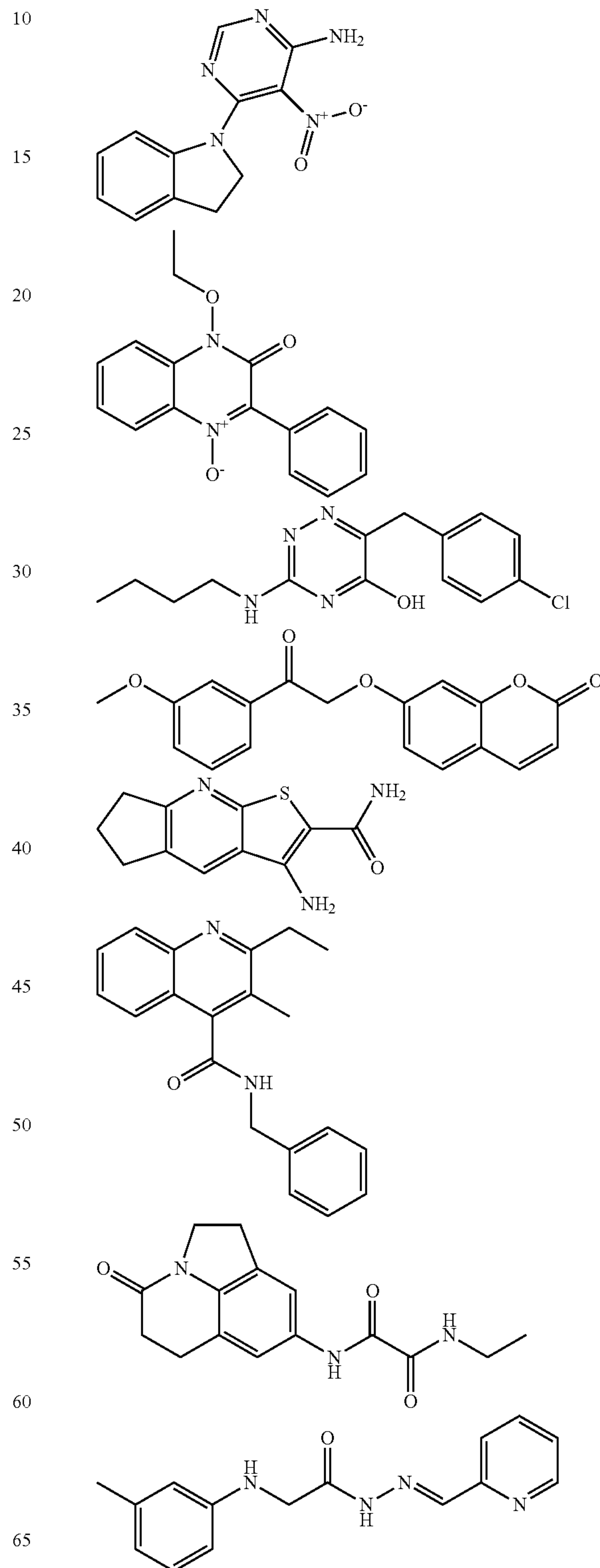
Formula 12
