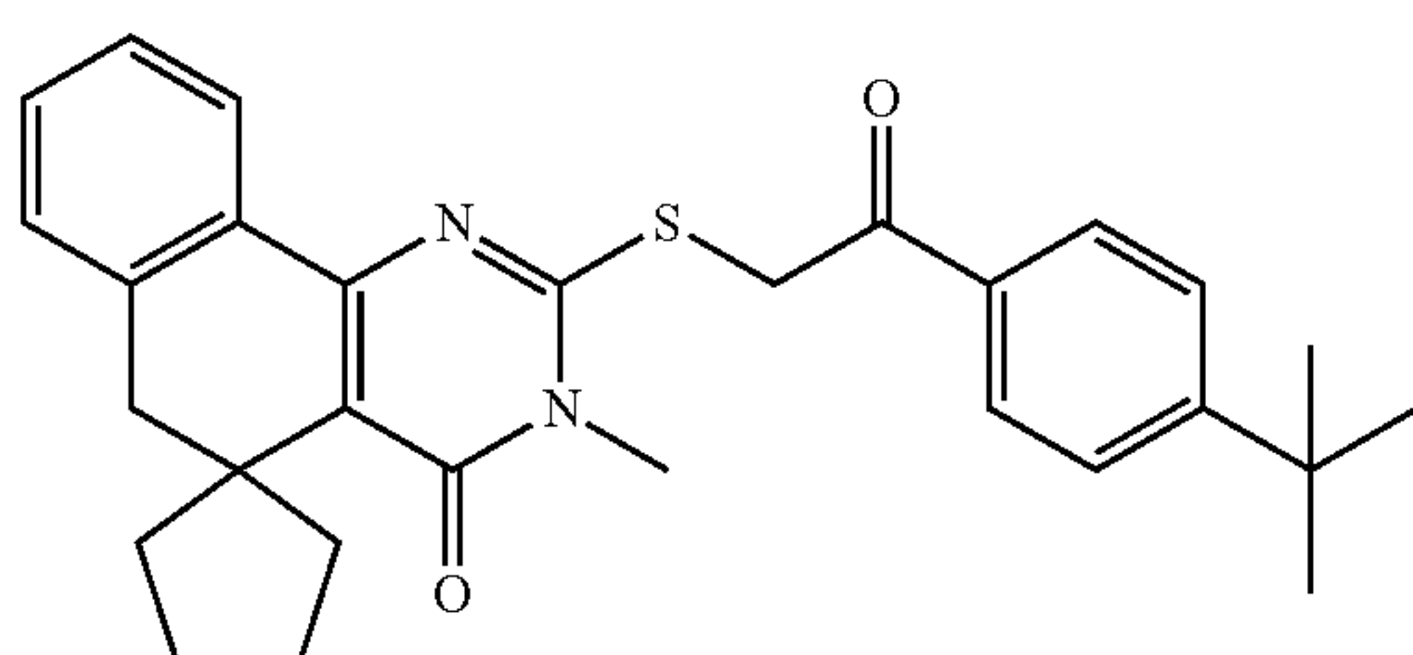
Compound 232
