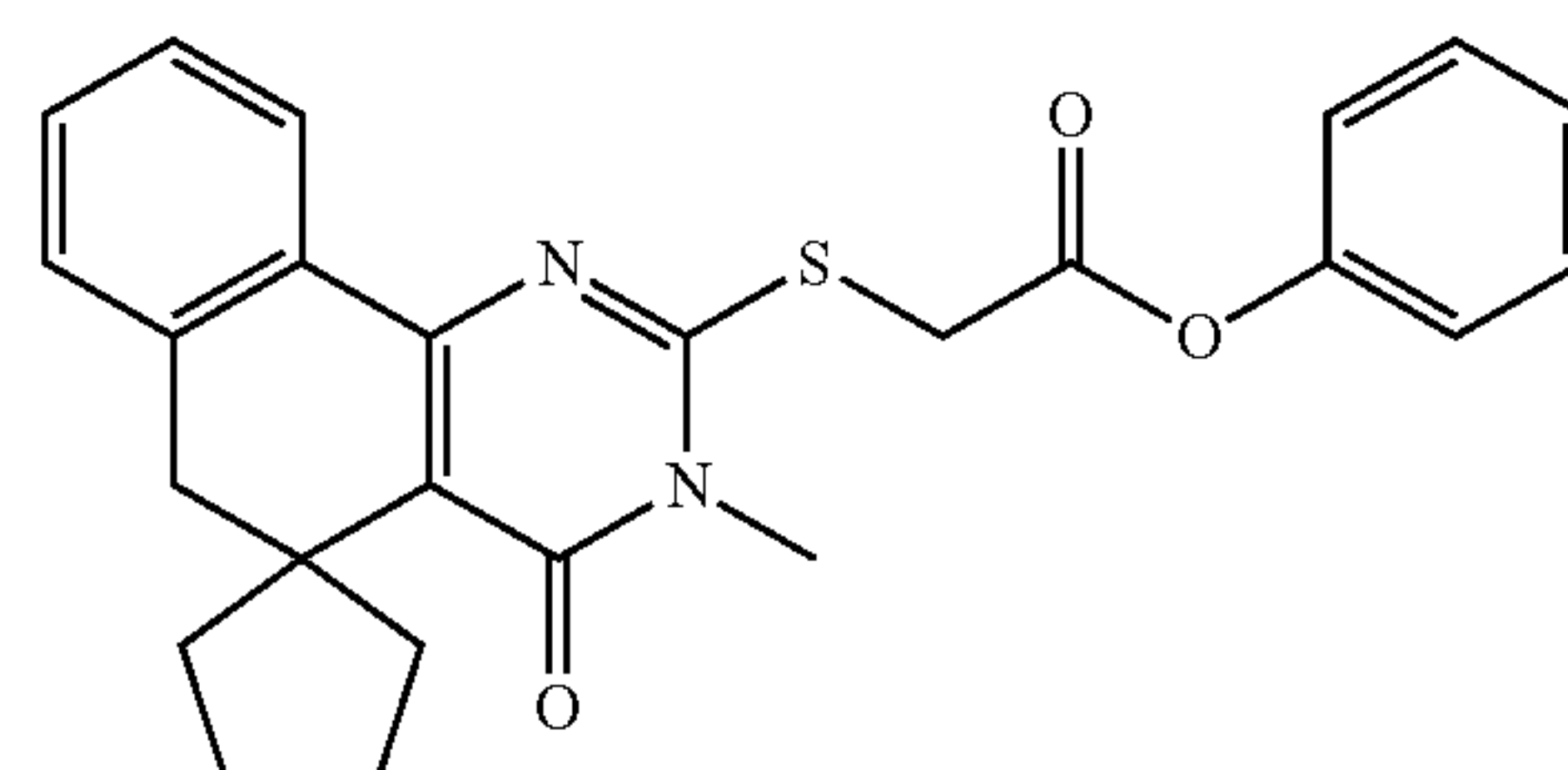
Compound 247
