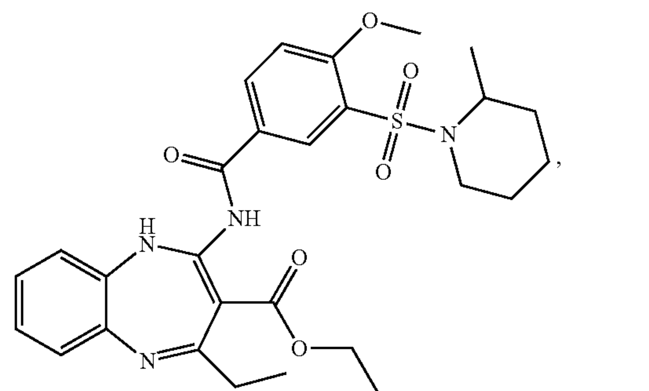
Compound 45
