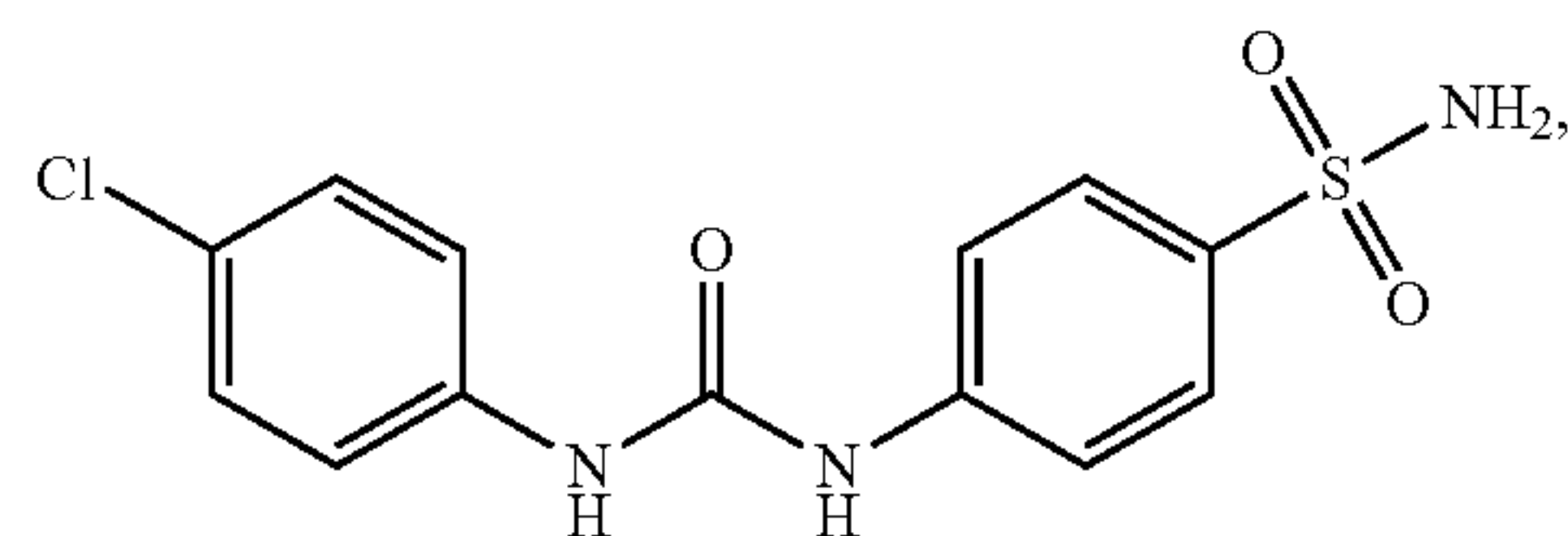
Compound 203
