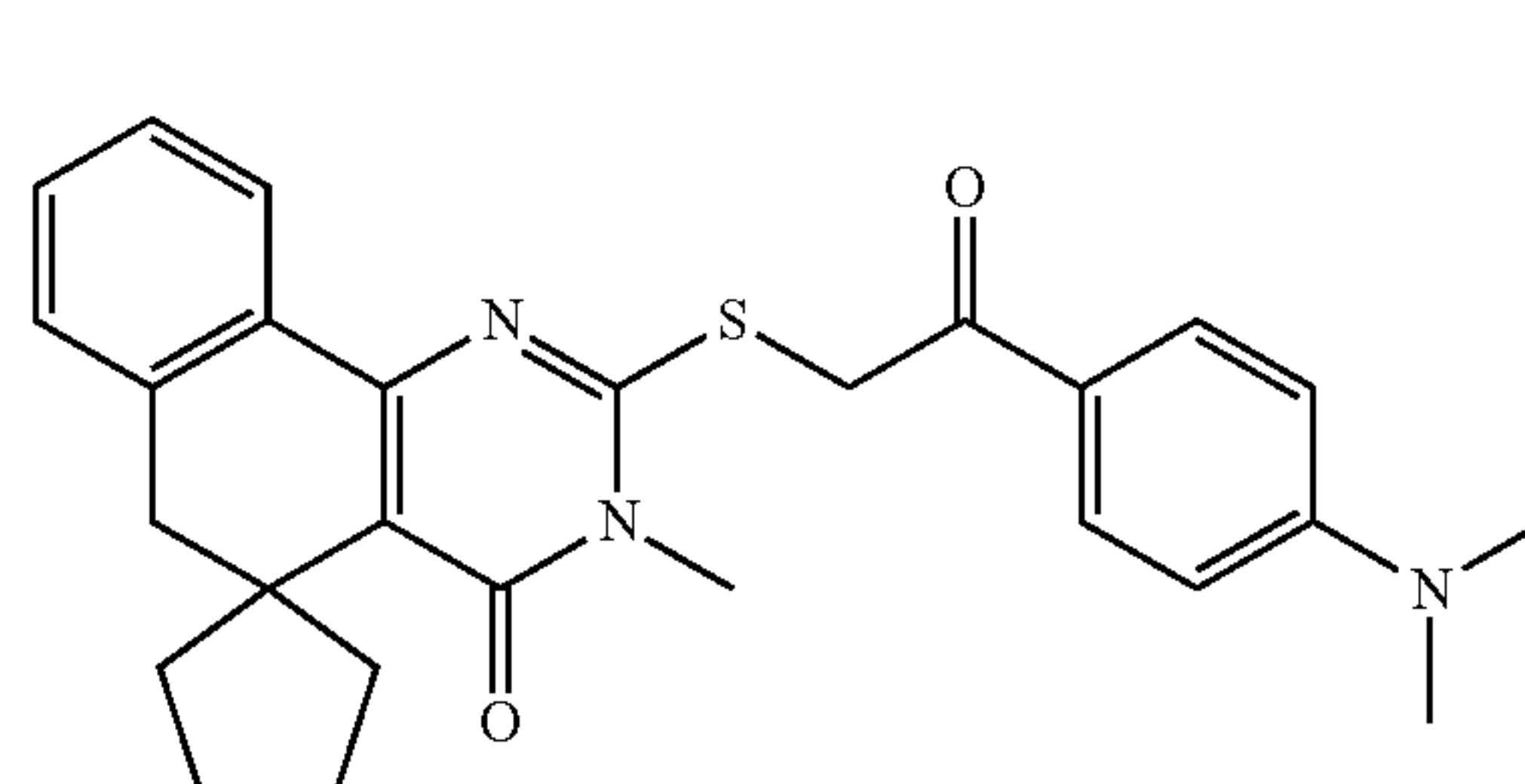
Compound 234
