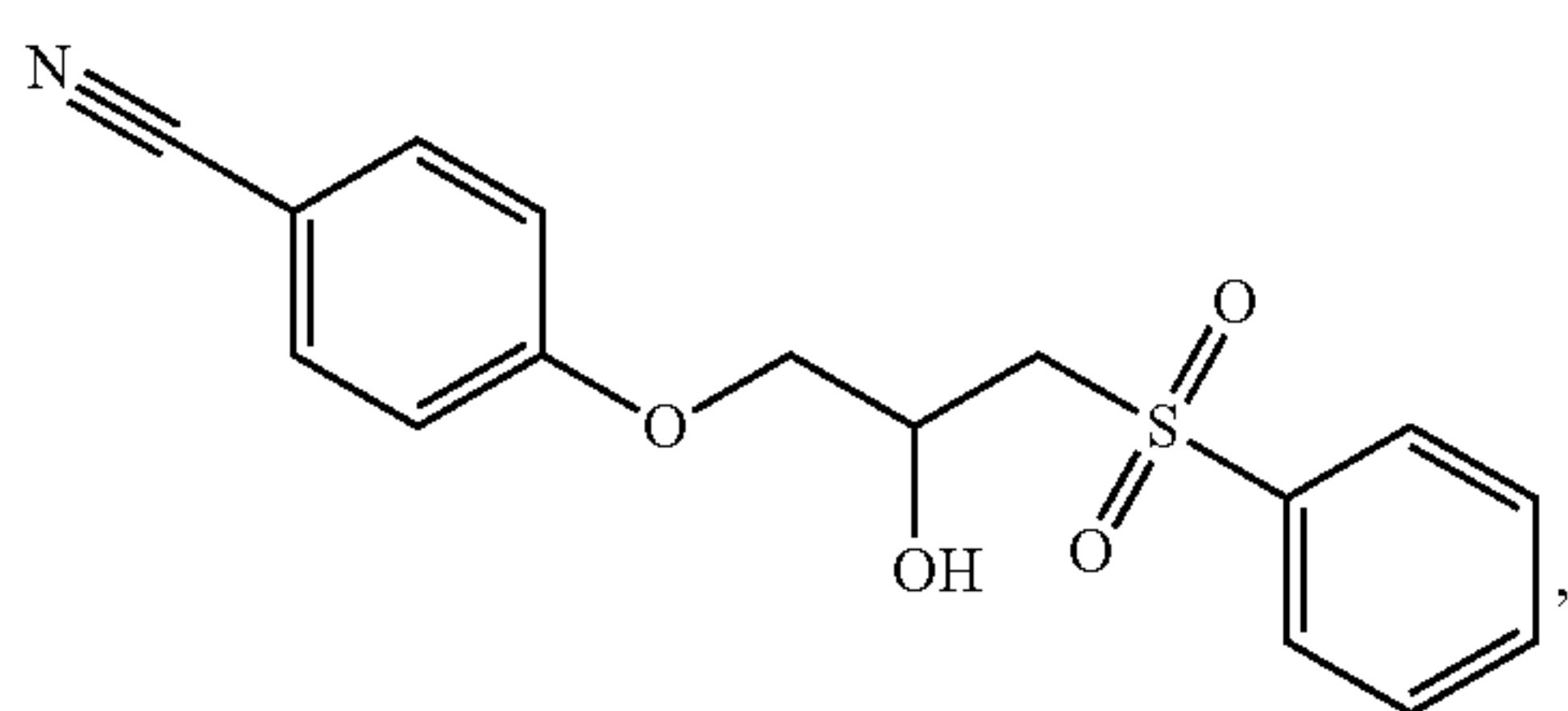
Compound 195
