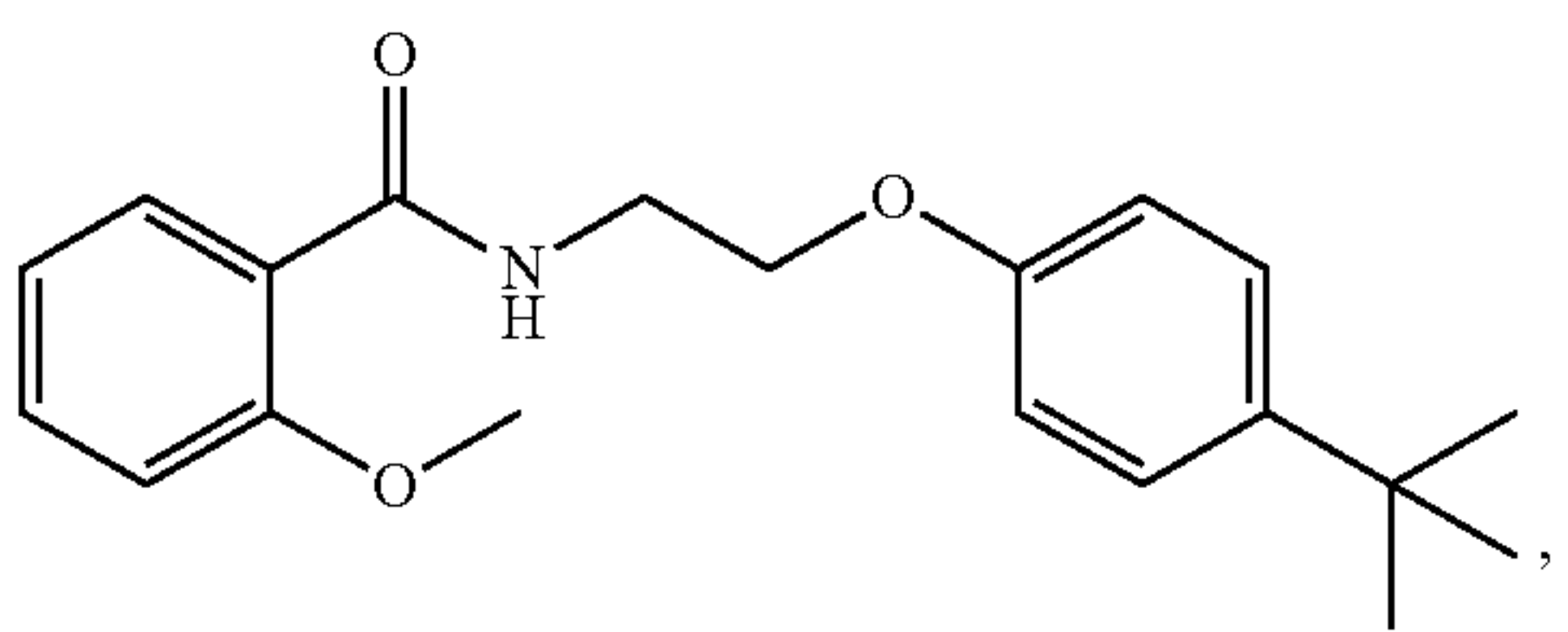
Compound 169
