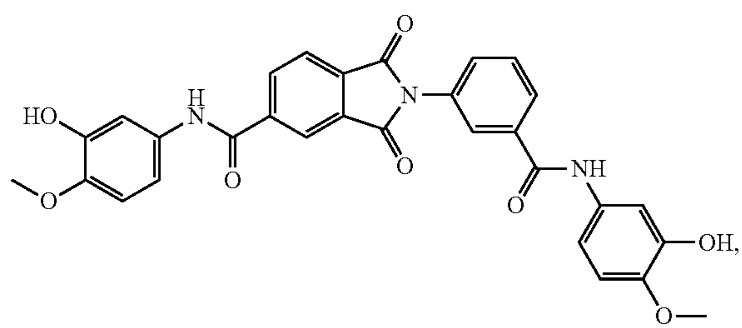
Compound 13
