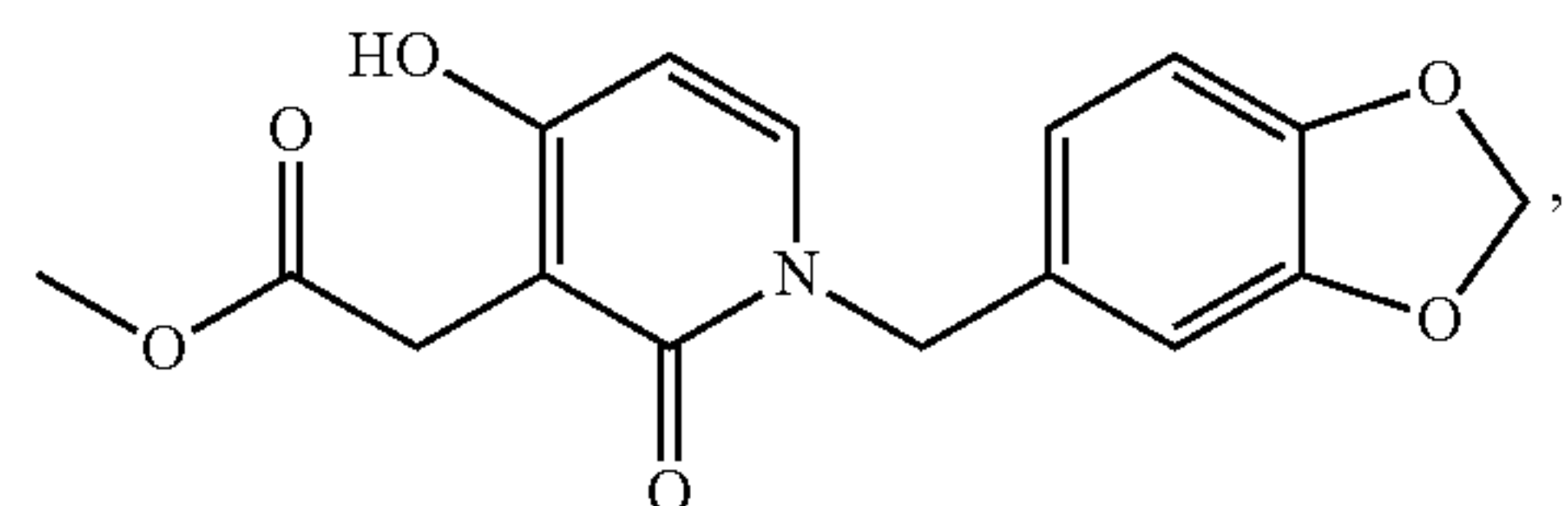
Compound 81
