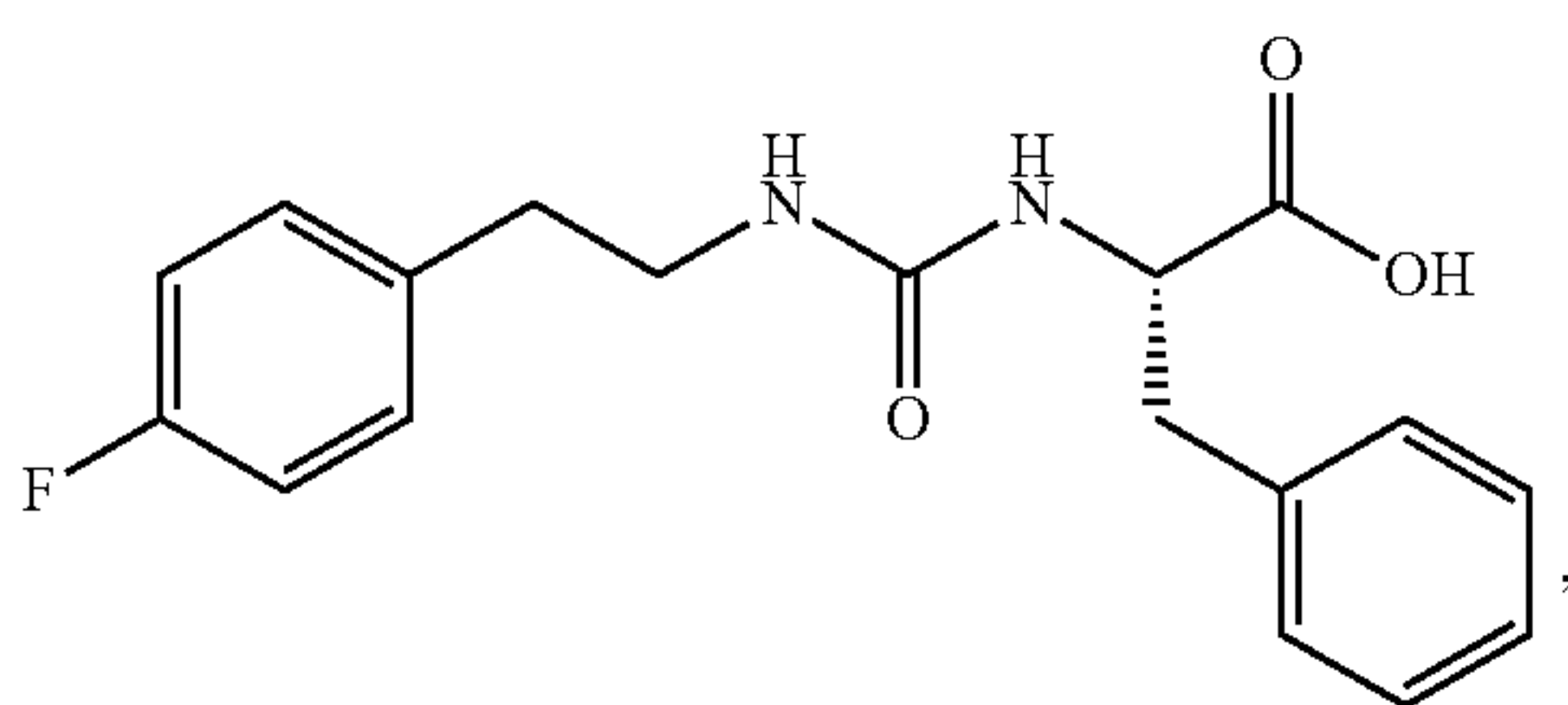
Compound 165
