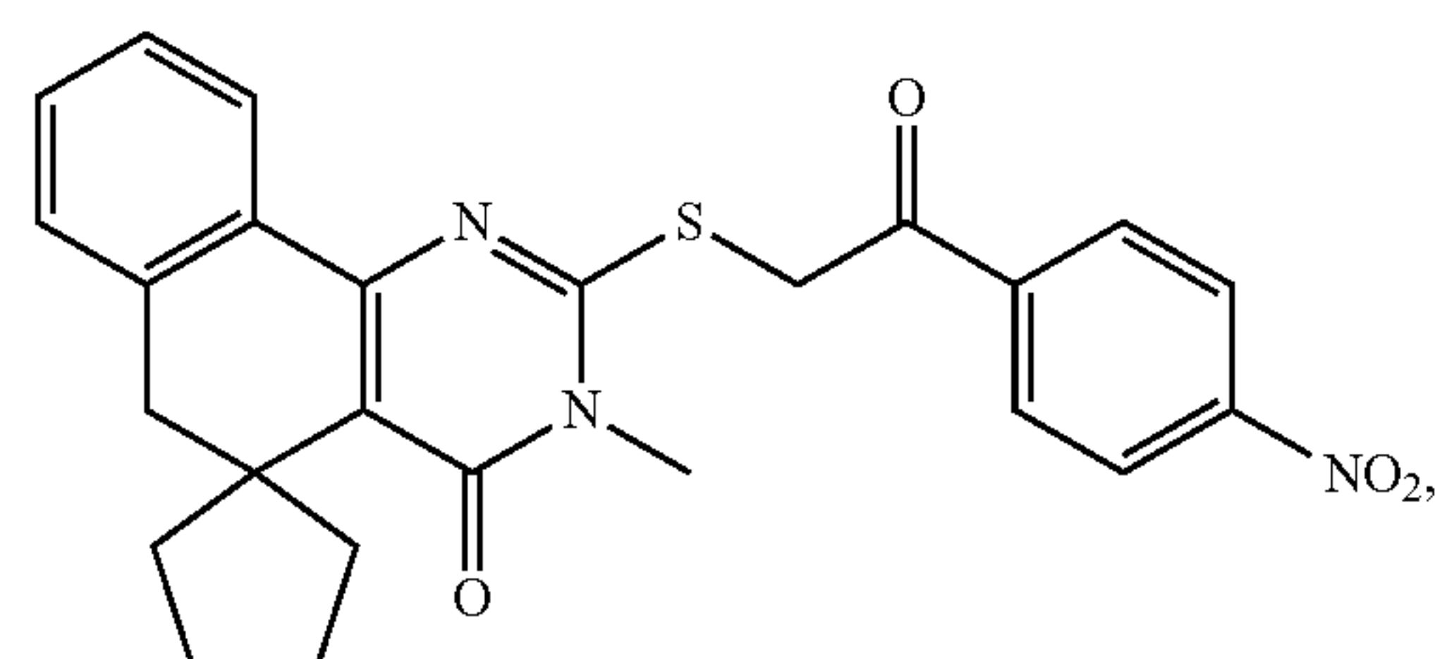
Compound 235
