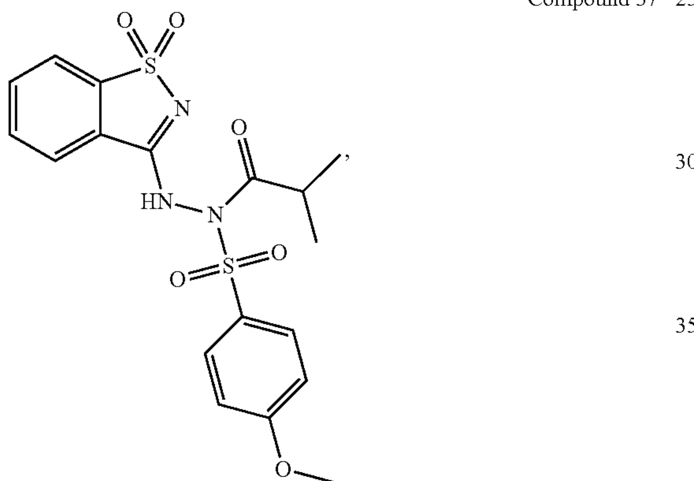
Compound 38
