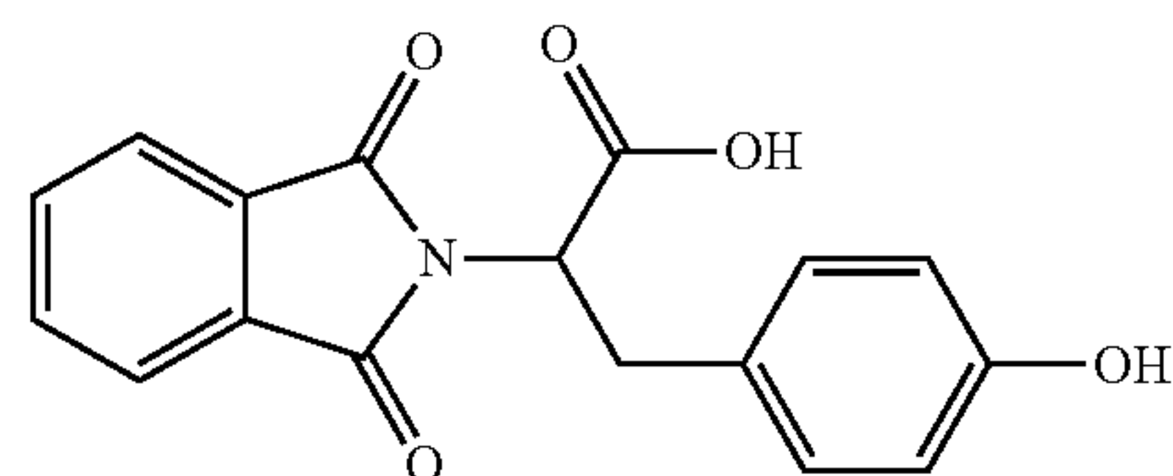
Formula 4
