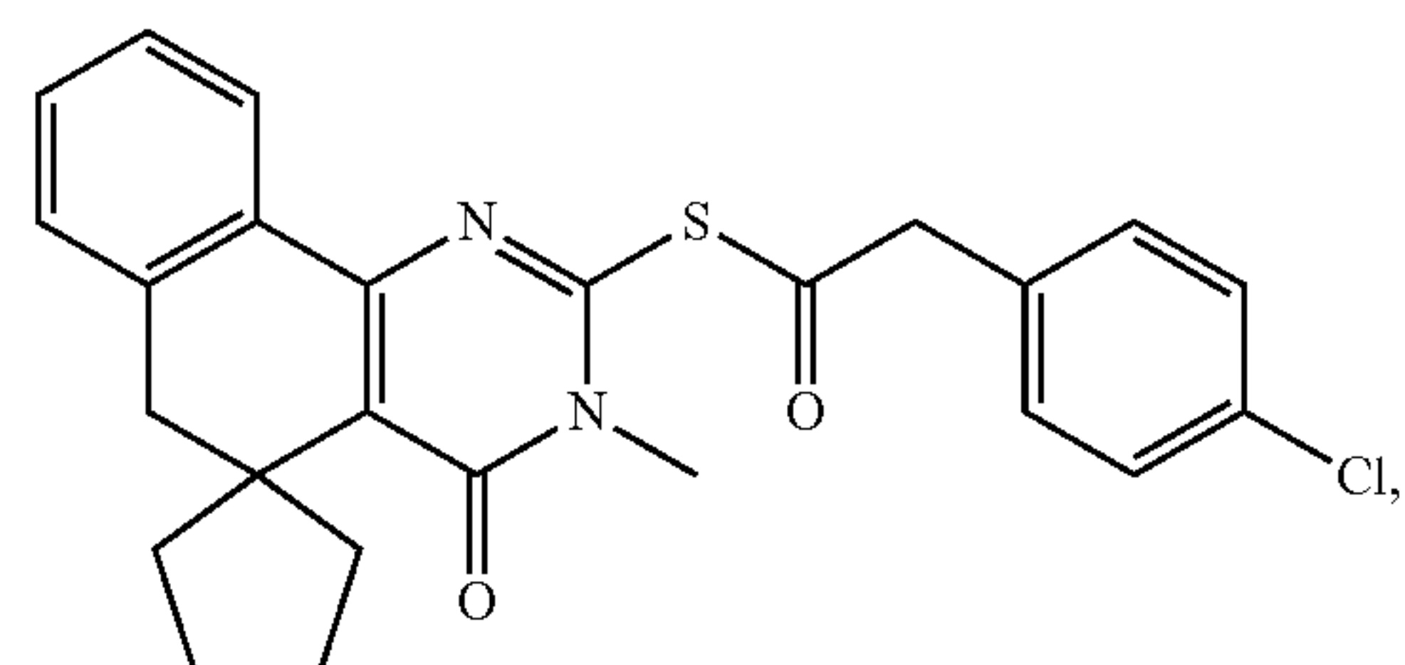
Compound 261
