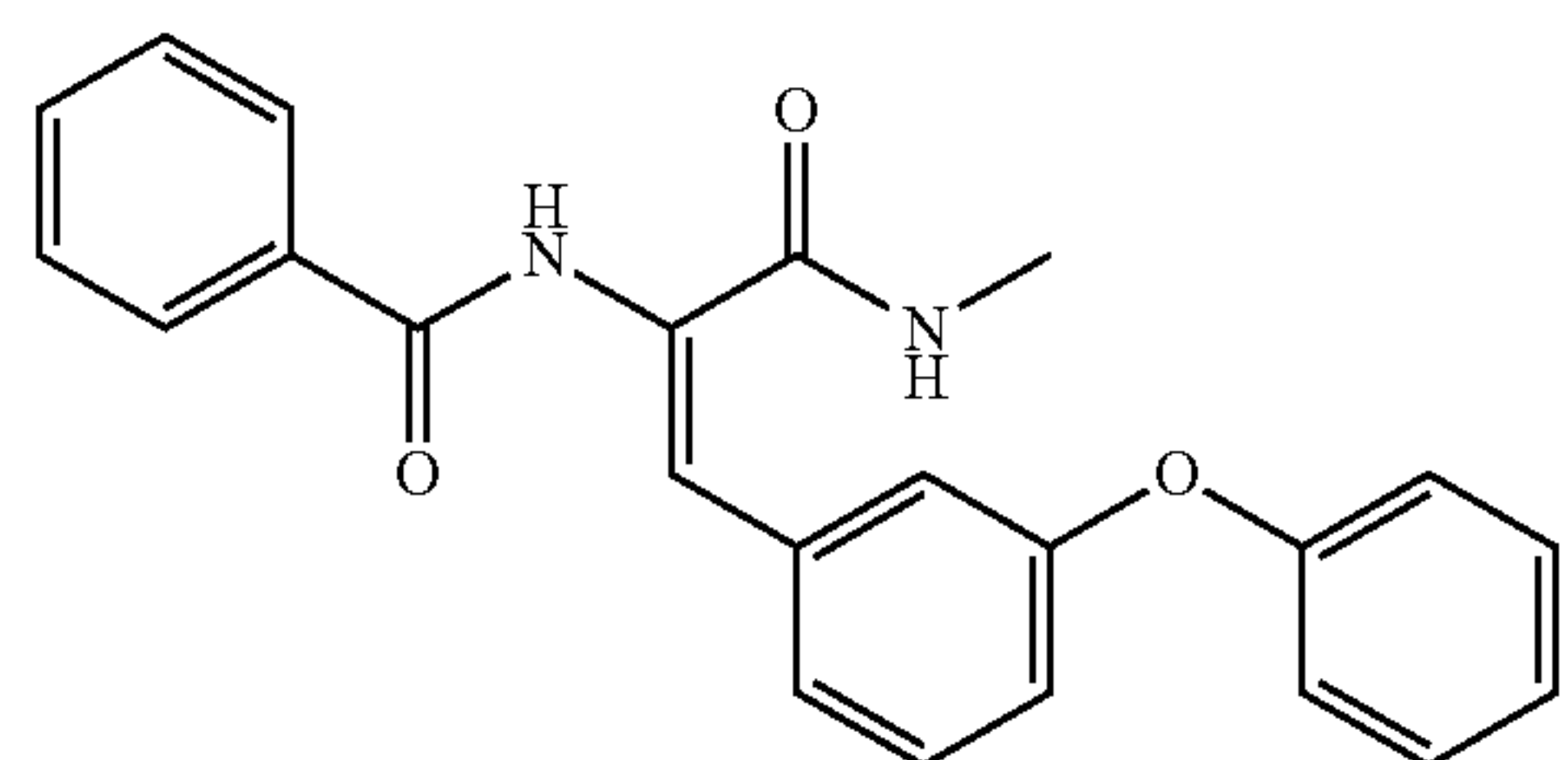
Compound 212
