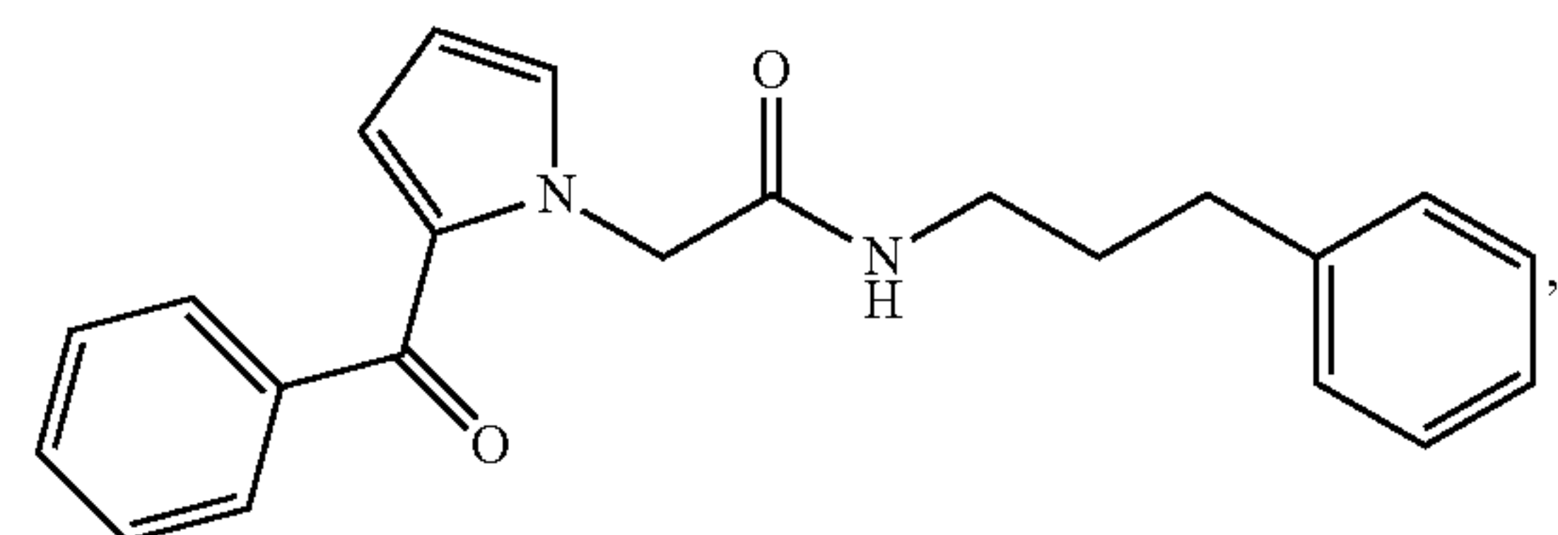
Compound 43
