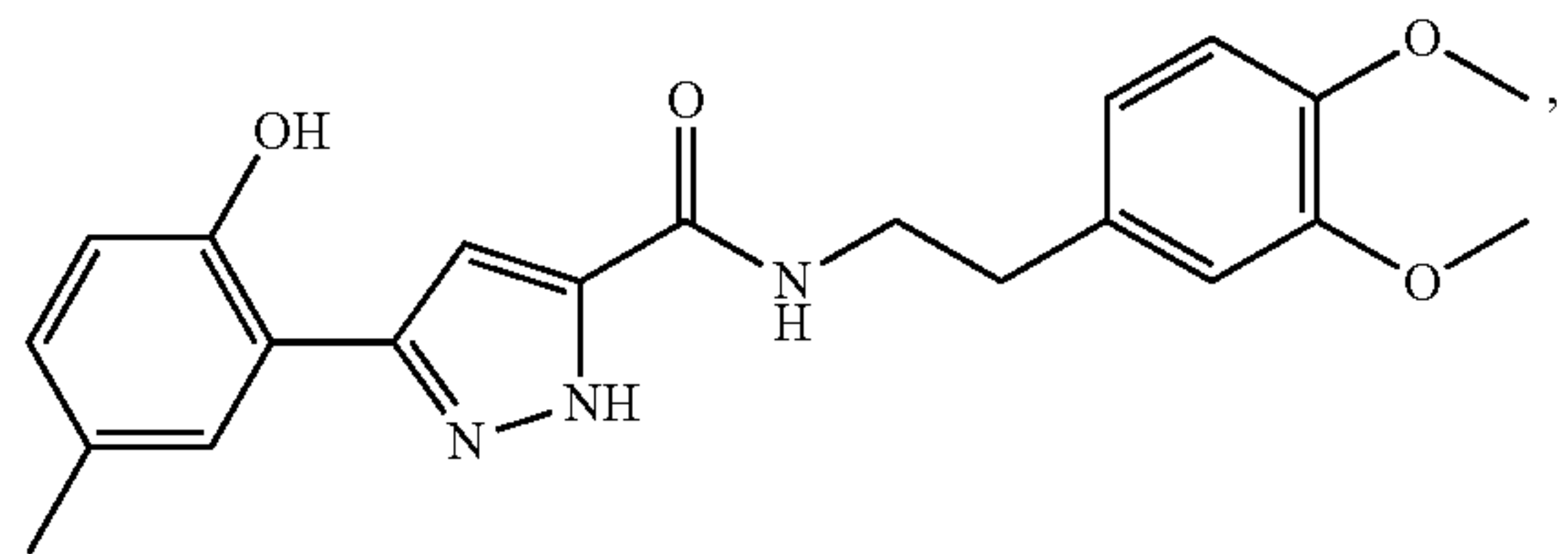
Compound 217
