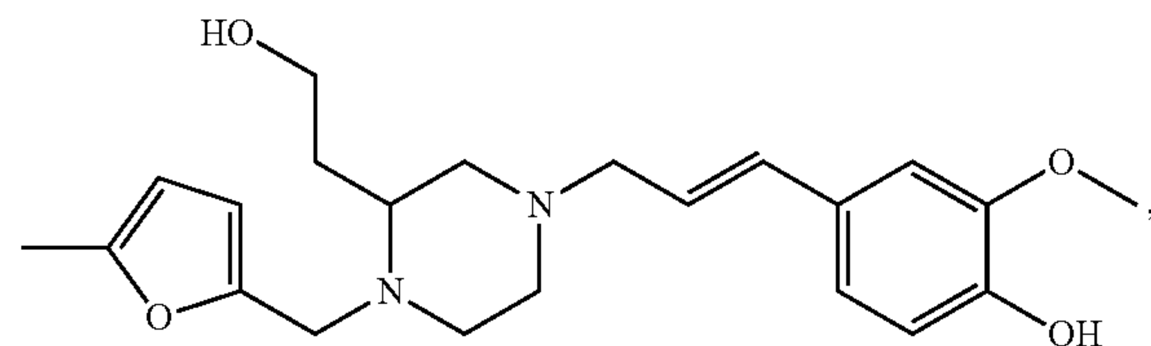
Compound 42
