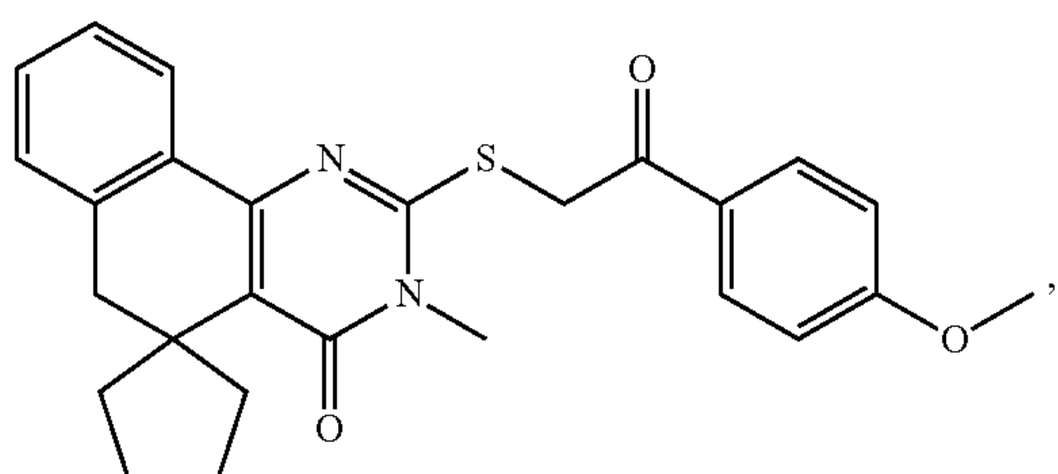
Compound 229
