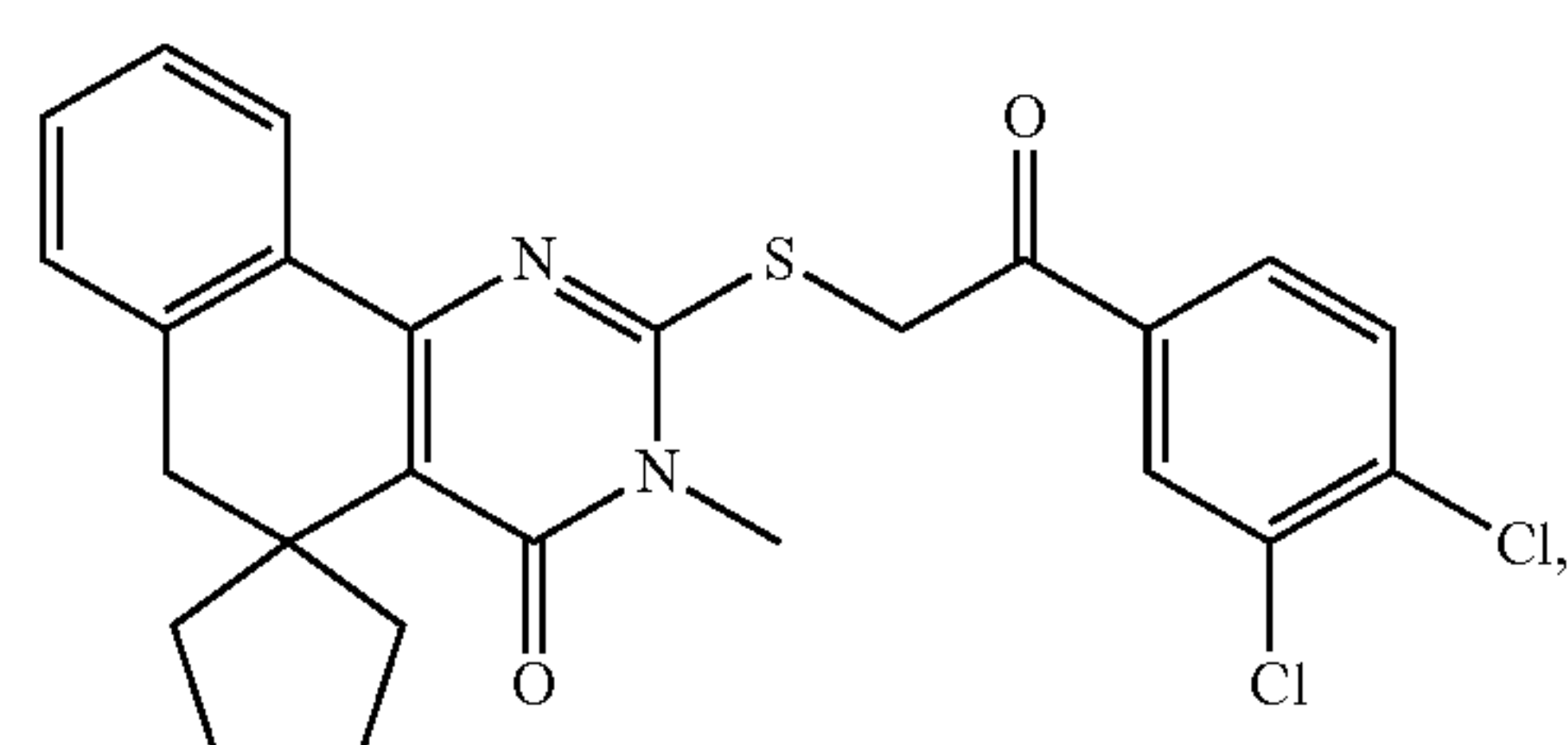
Compound 239
