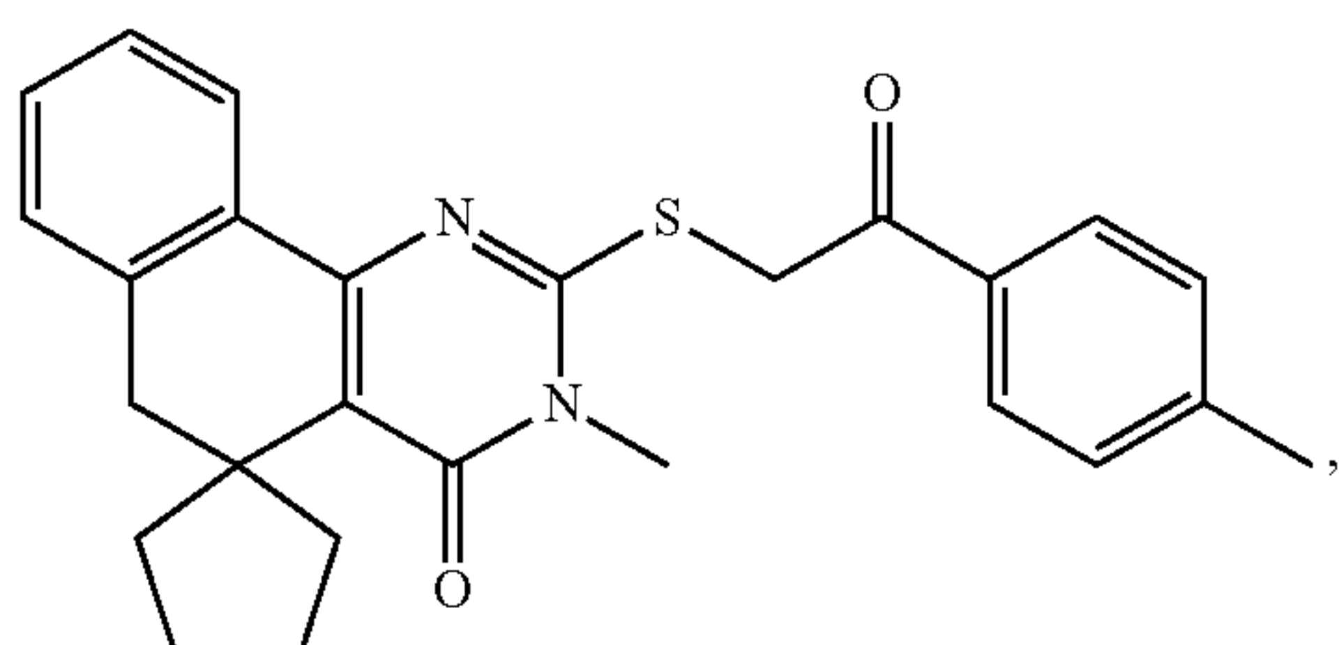
Compound 230
