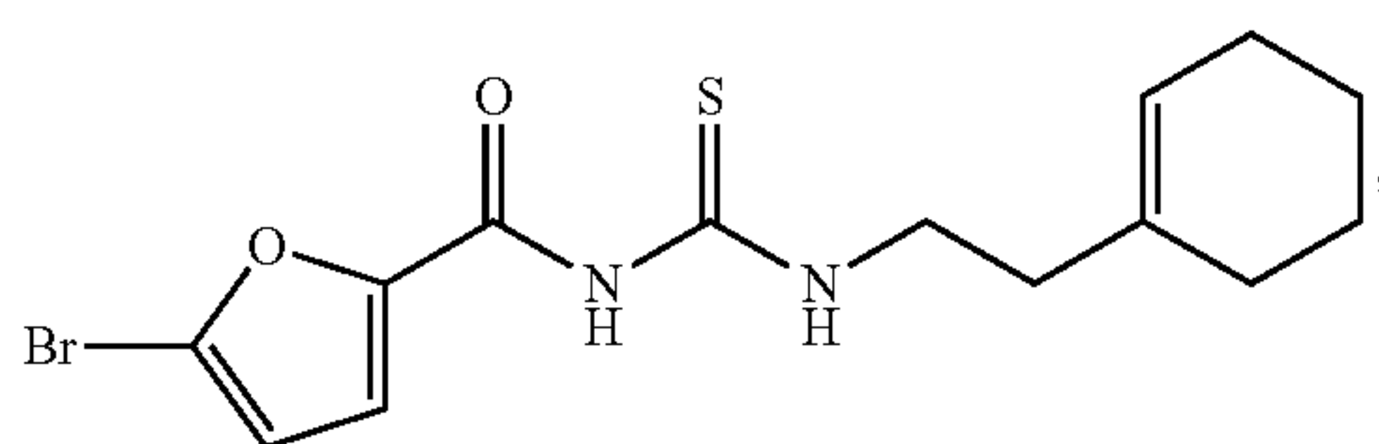
Compound 206
