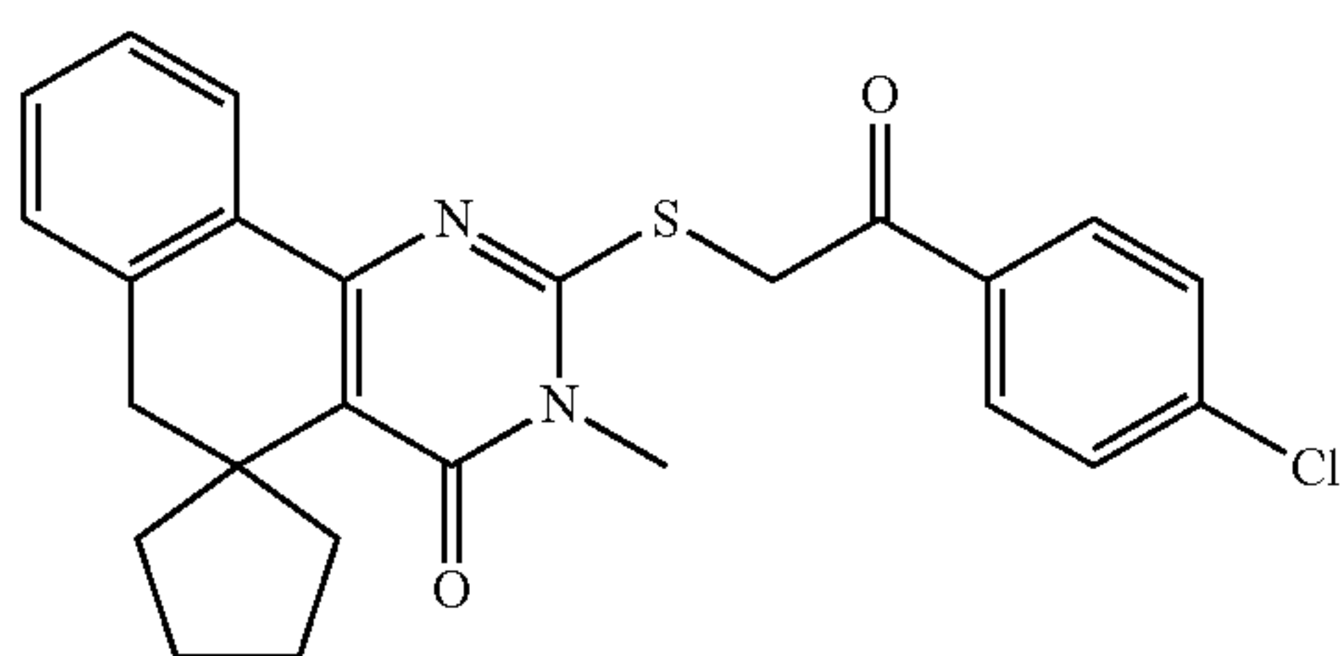
Compound 228
