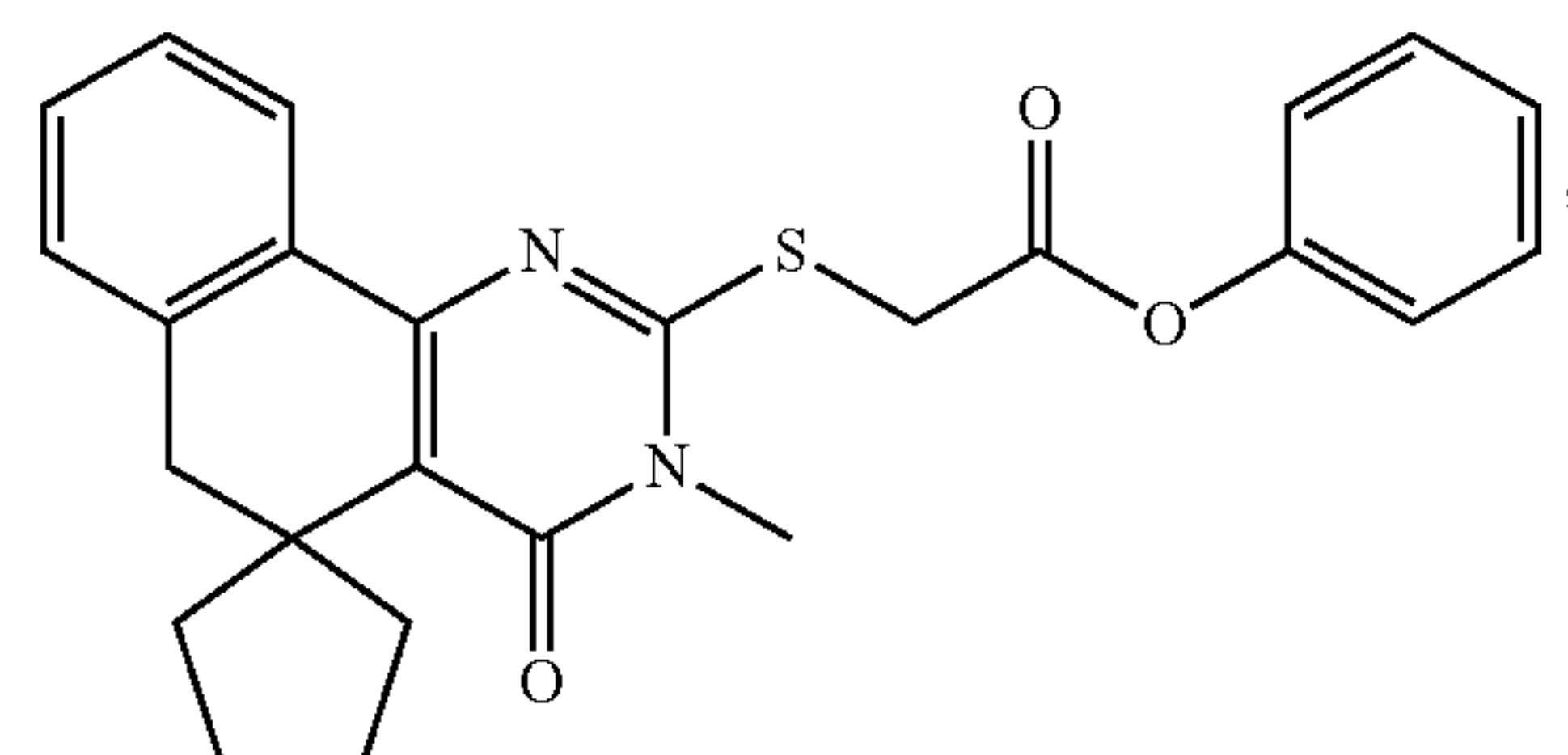
Compound 247
