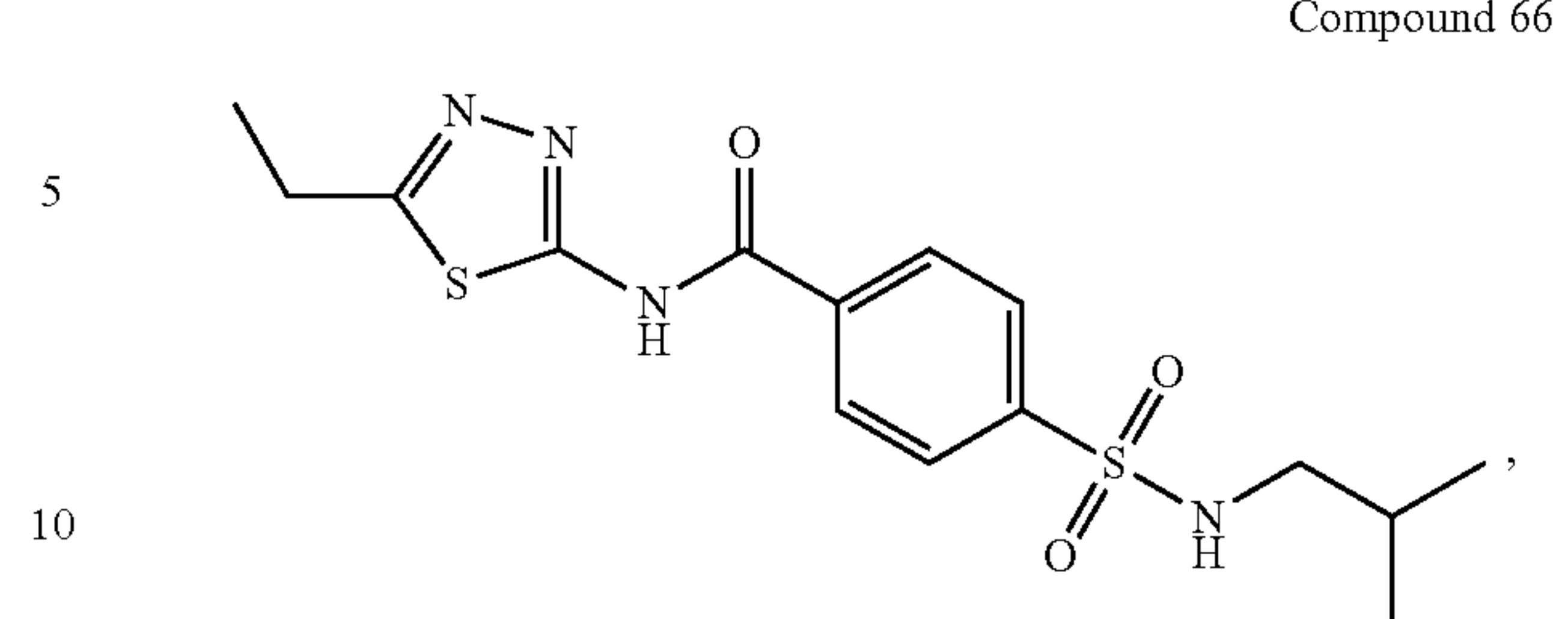
Compound 66
