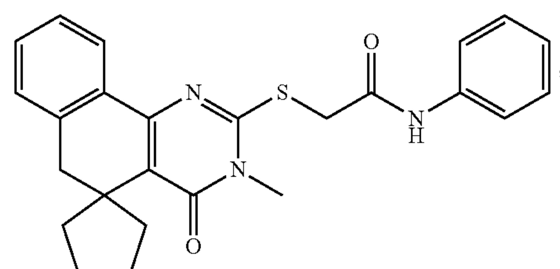
Compound 250
