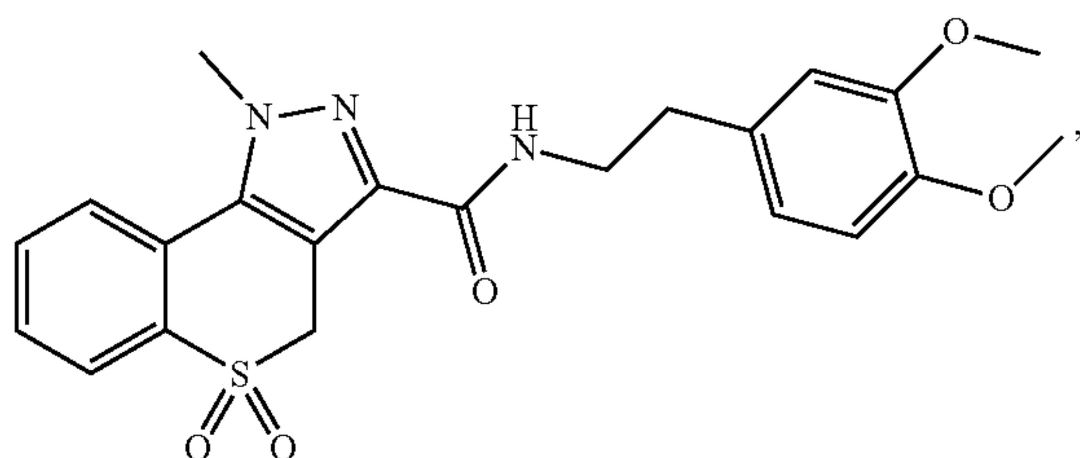
Compound 74
