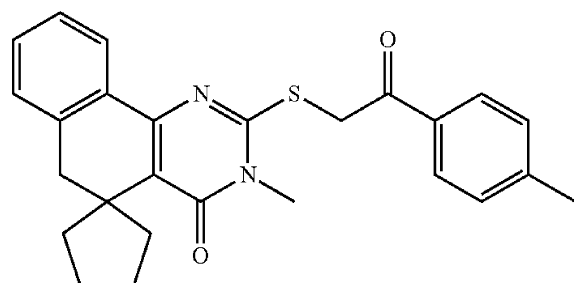
Compound 230
