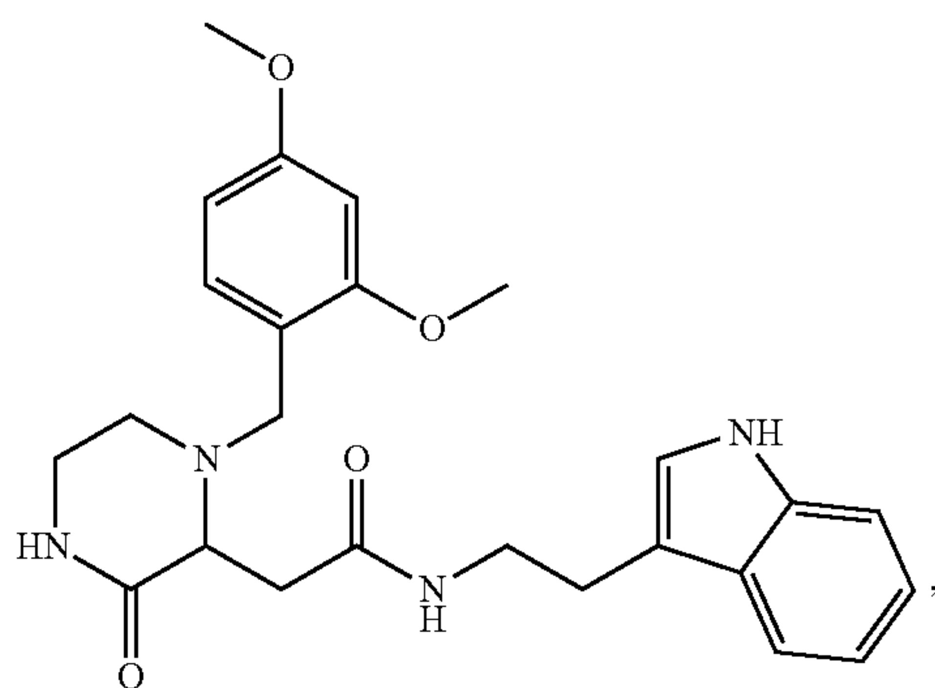
Compound 209
