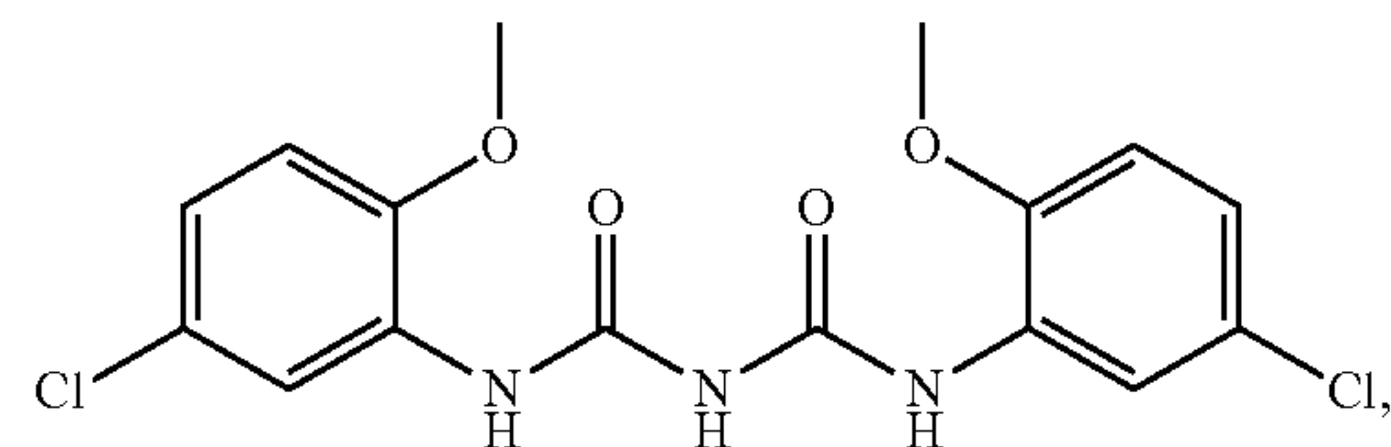
Compound 41
