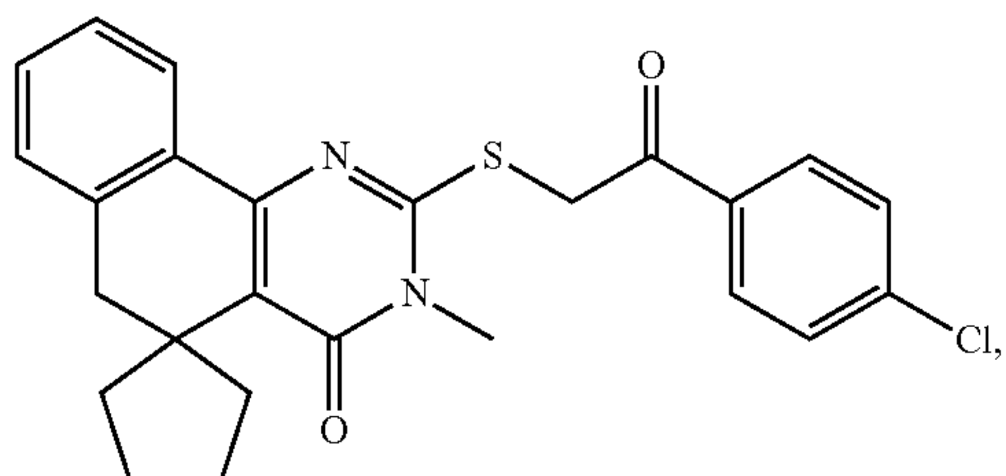
Compound 228
