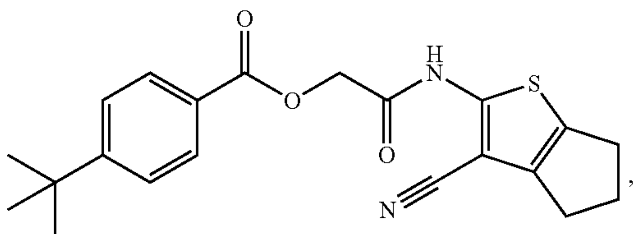
Compound 85
