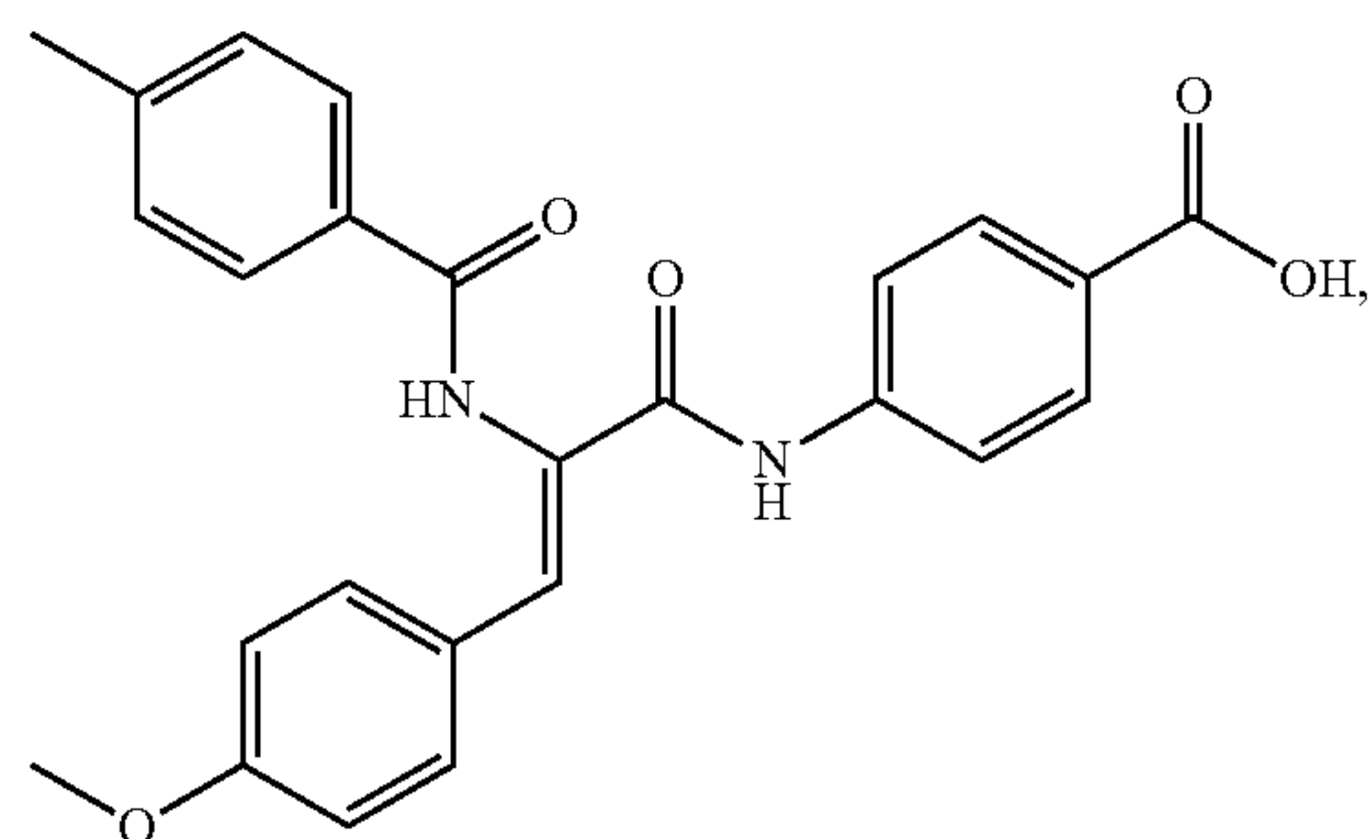
Compound 160
