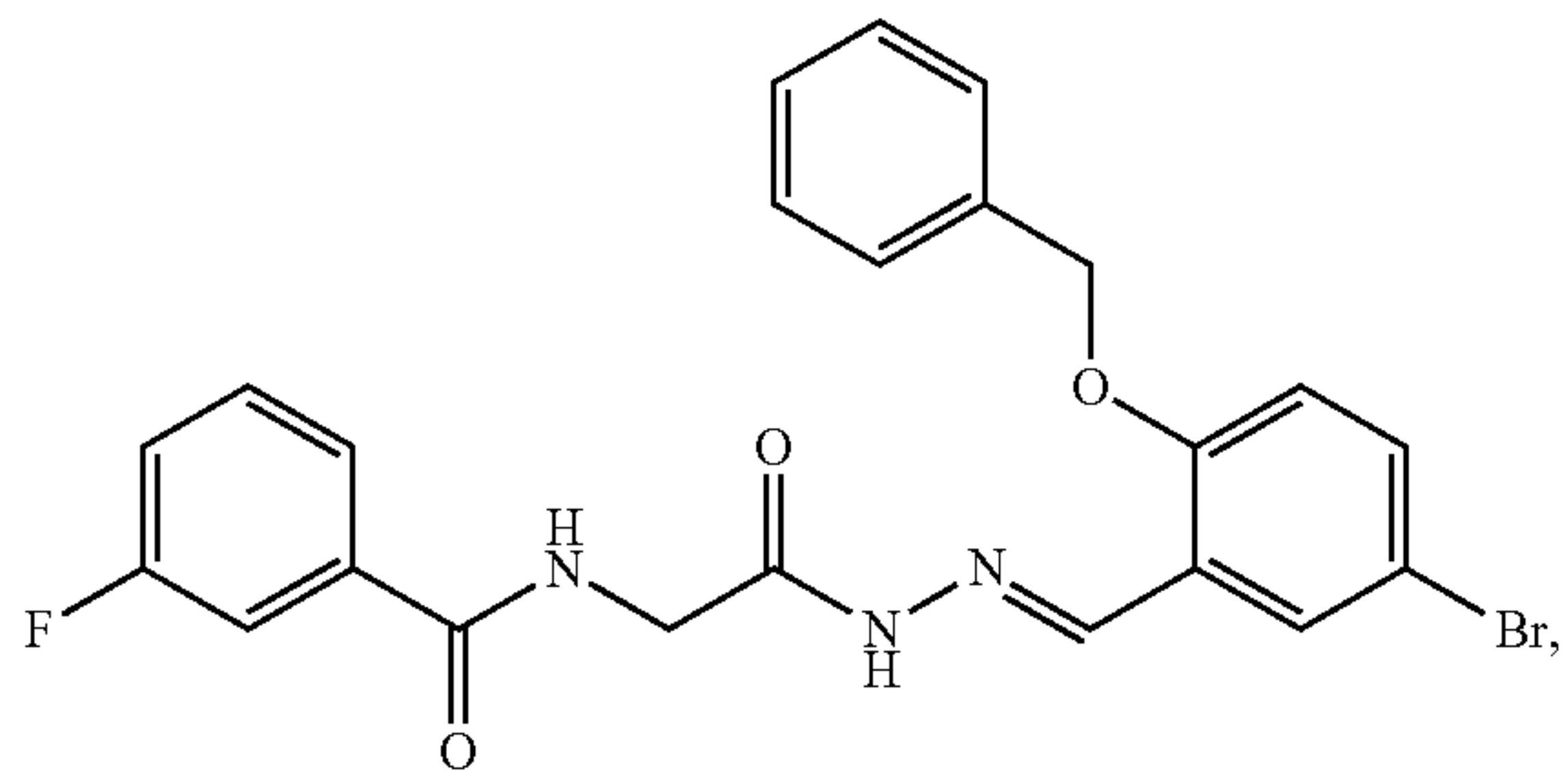
Compound 216
