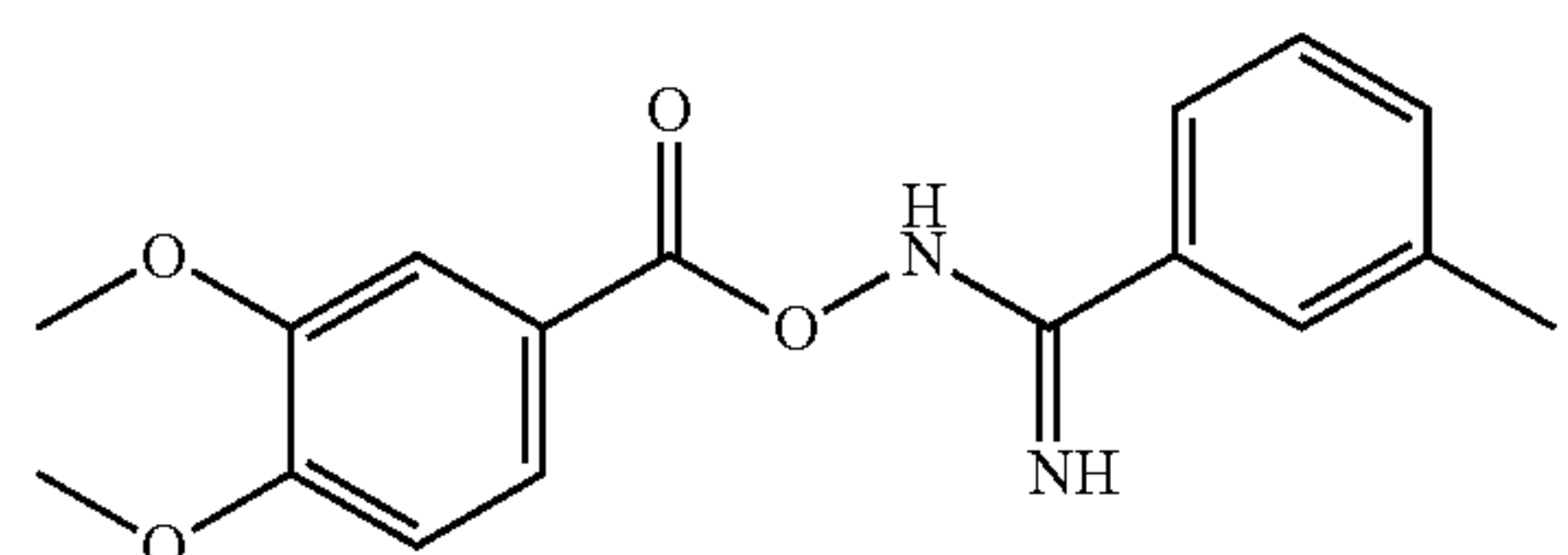
Compound 78
