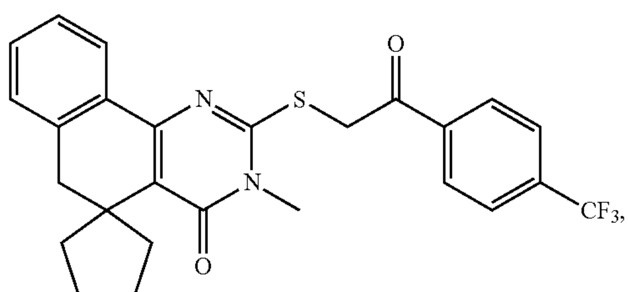
Compound 232
