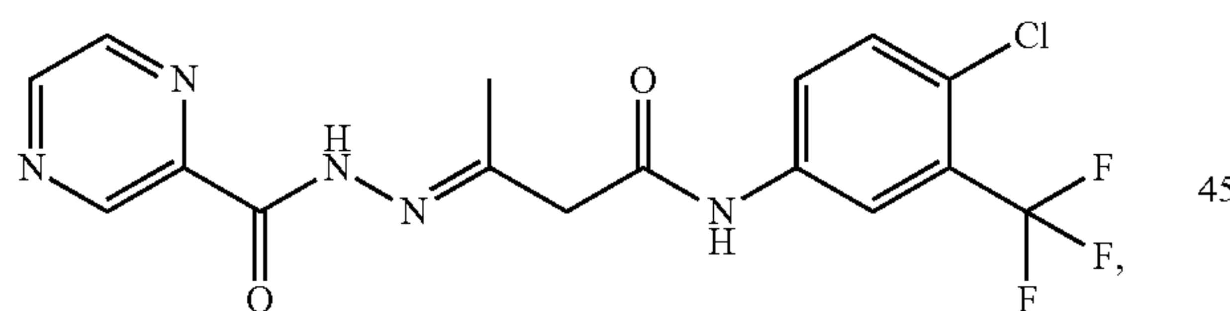
Compound 39
