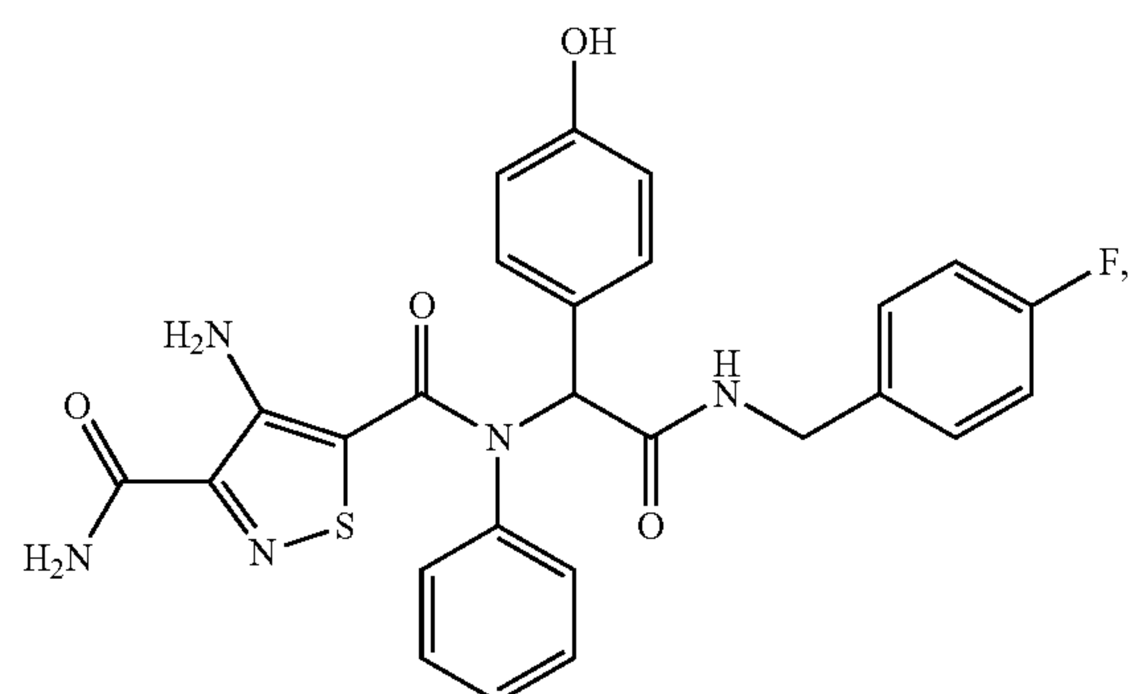
Compound 16
