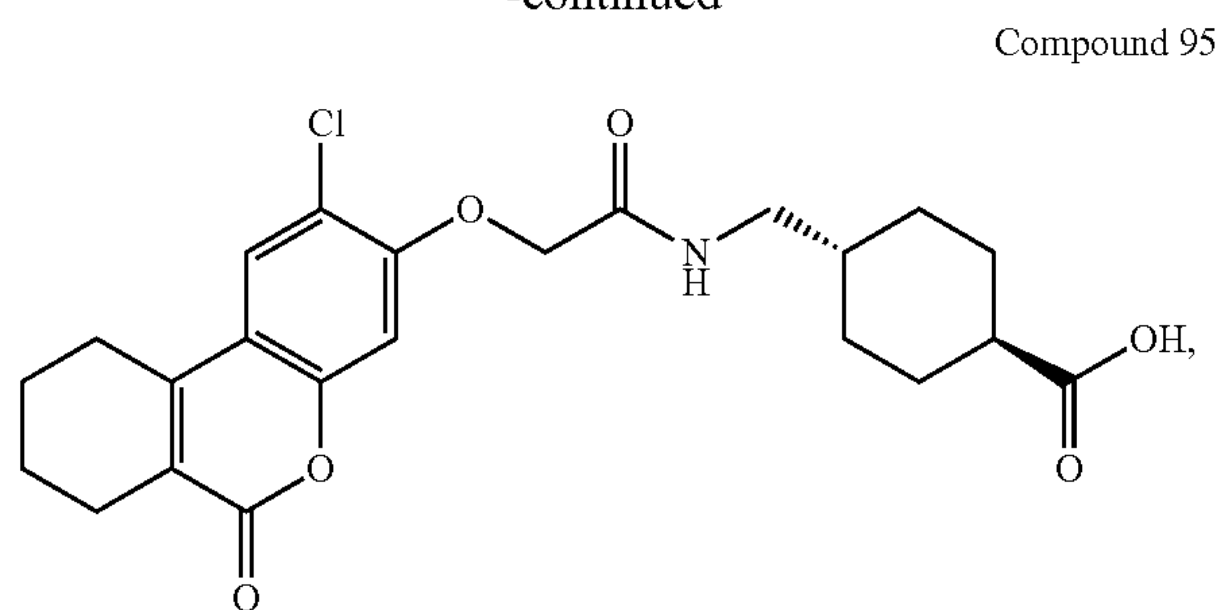
Compound 96
