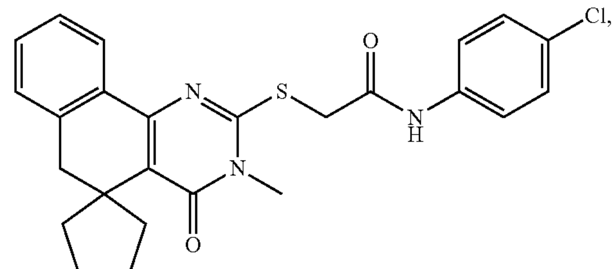
Compound 248
