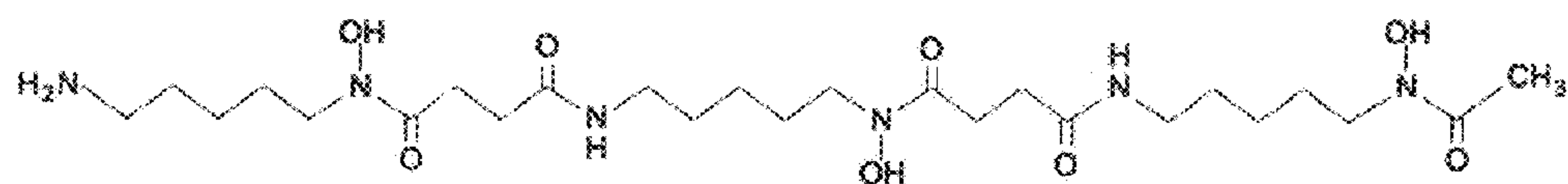
Deferoxamine
