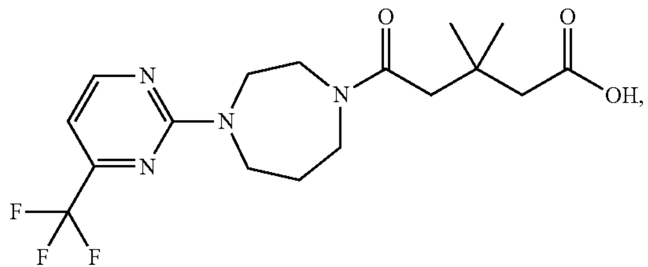
Compound 57
