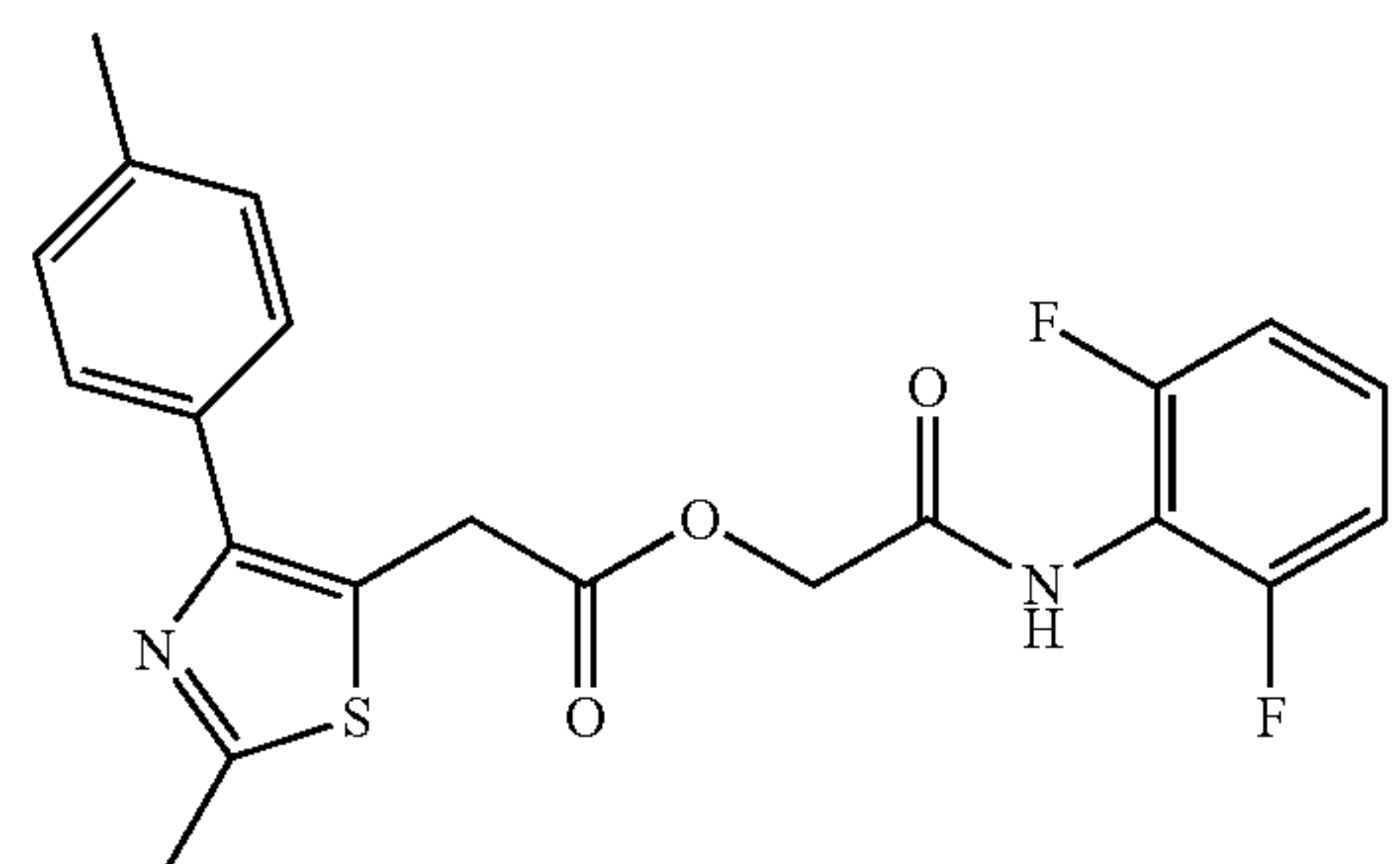
Compound 211
