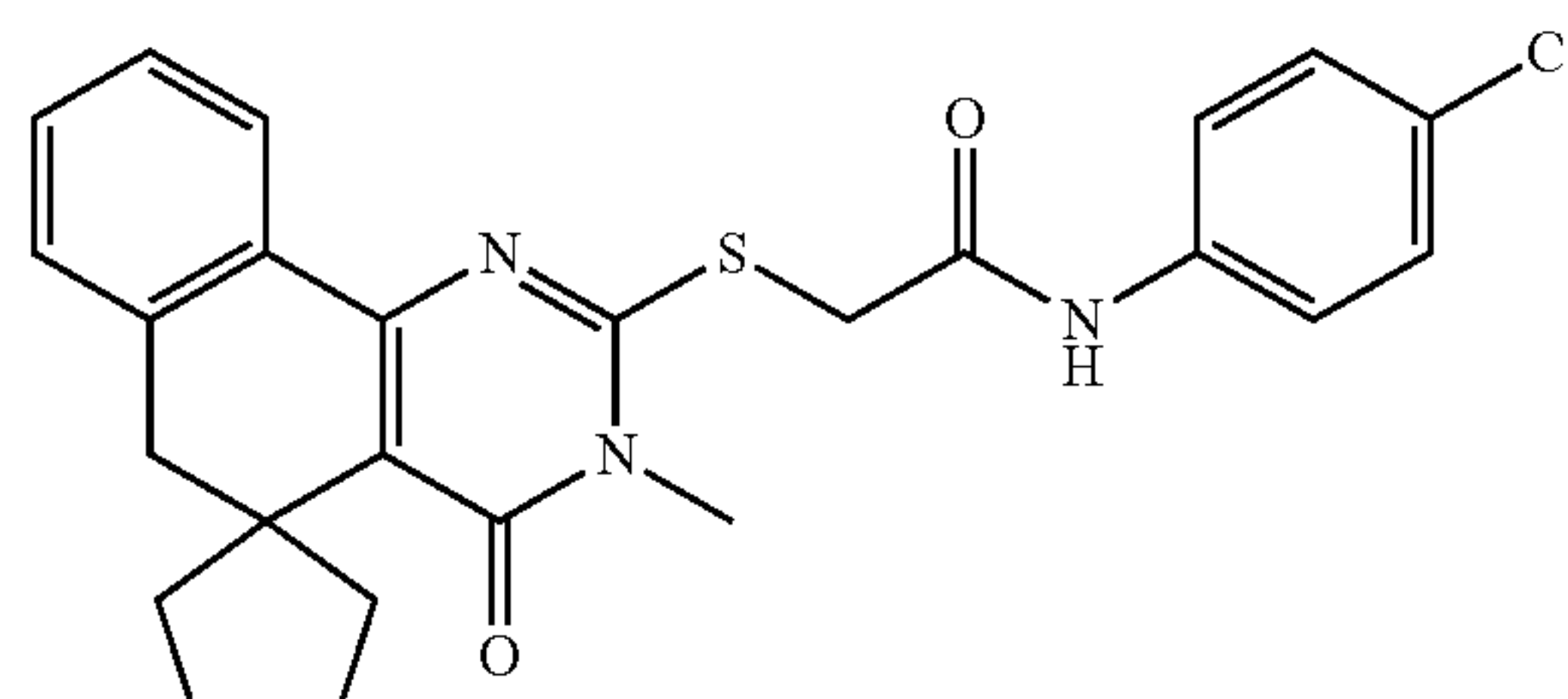
Compound 248
