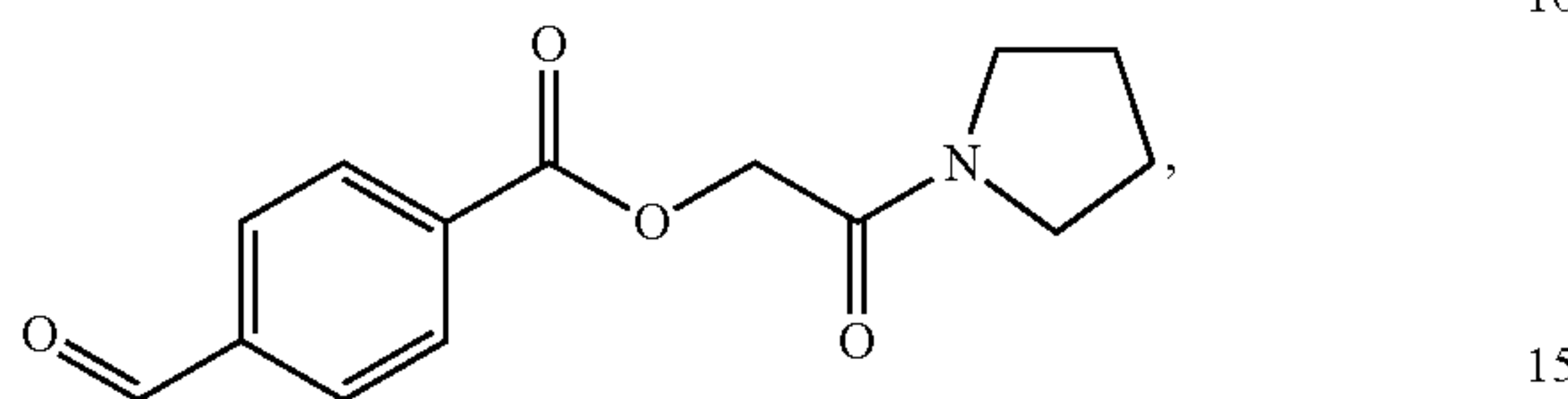
Compound 36
