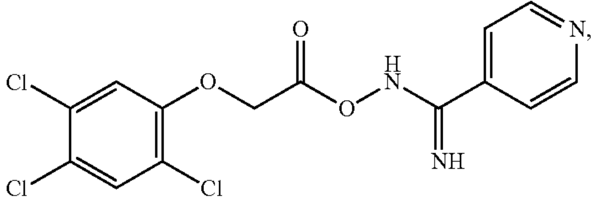
Compound 125
