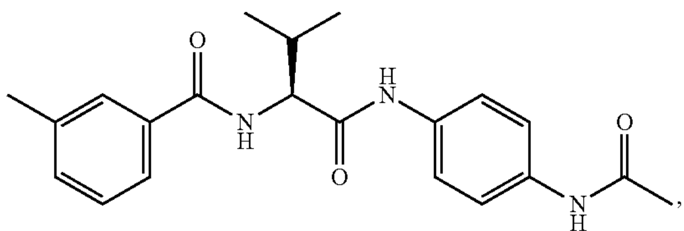
Compound 48
