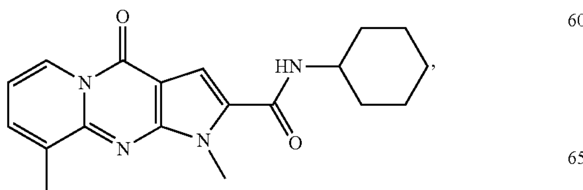
Compound 40
