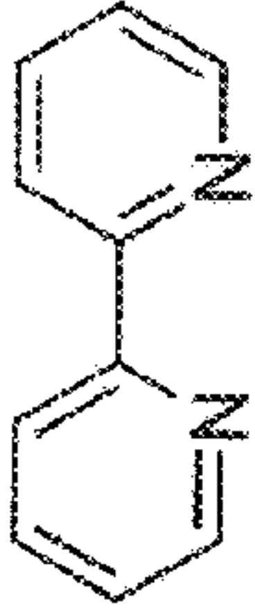
PRTH-002-E 2,2'-dipyridyl
