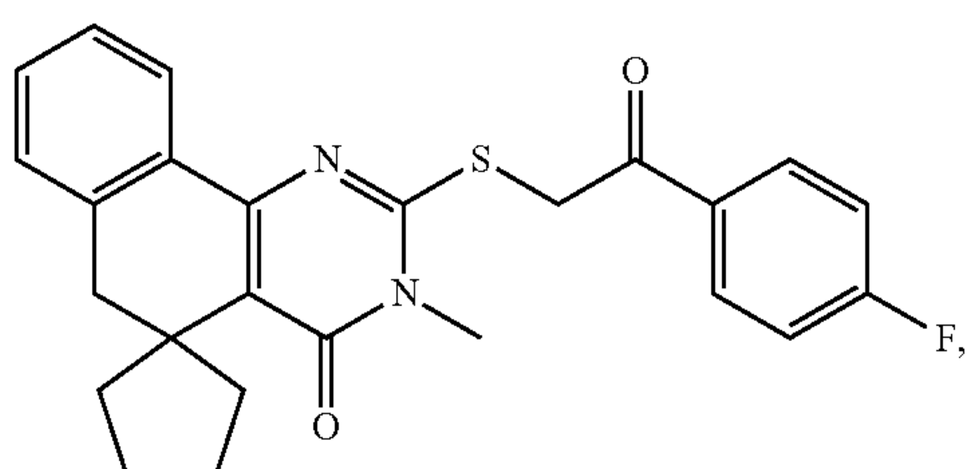
Compound 233
