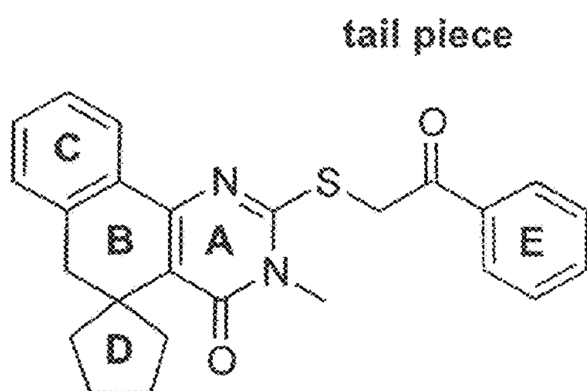
PRTH-002-F id#1001
