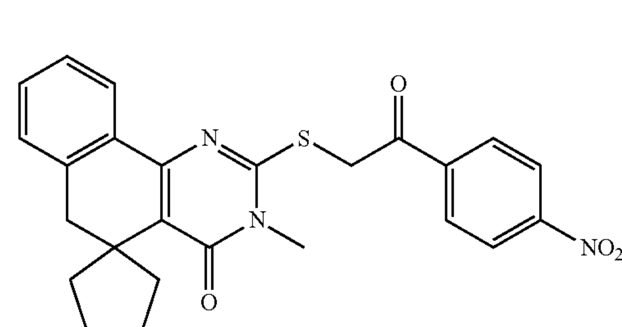
Compound 235
