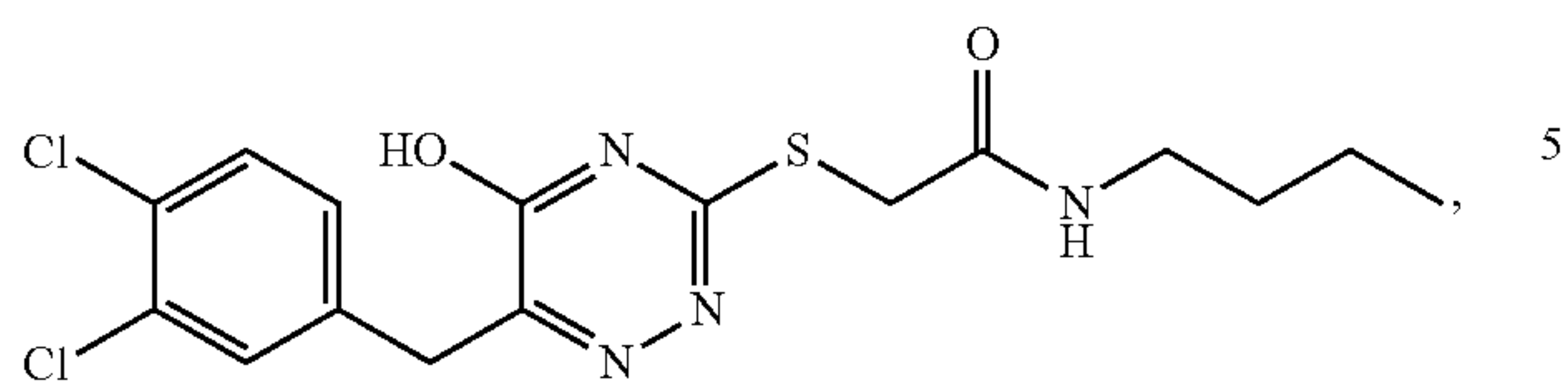
Compound 35
