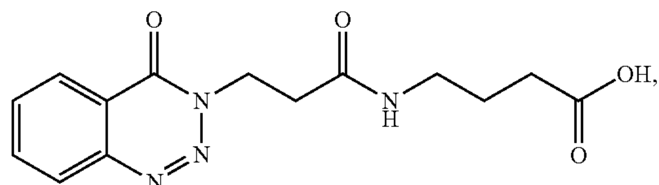
Compound 175
