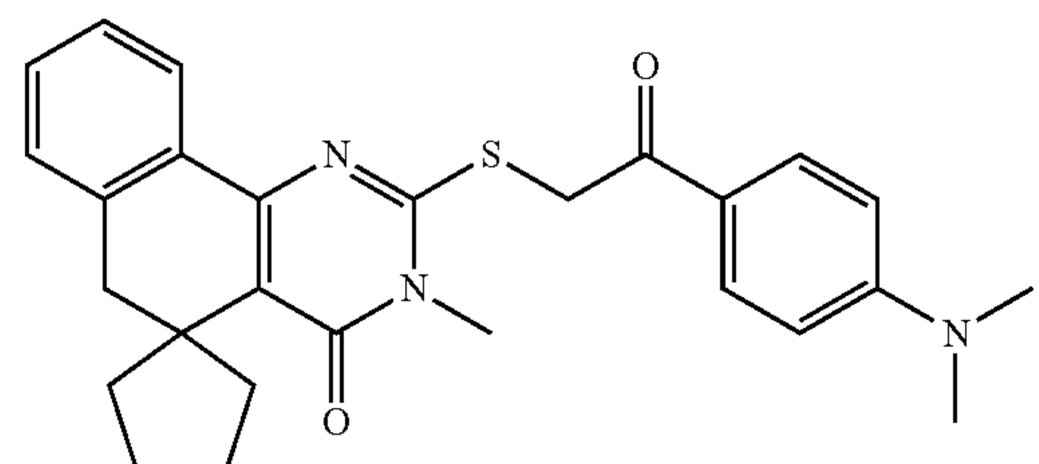
Compound 234
