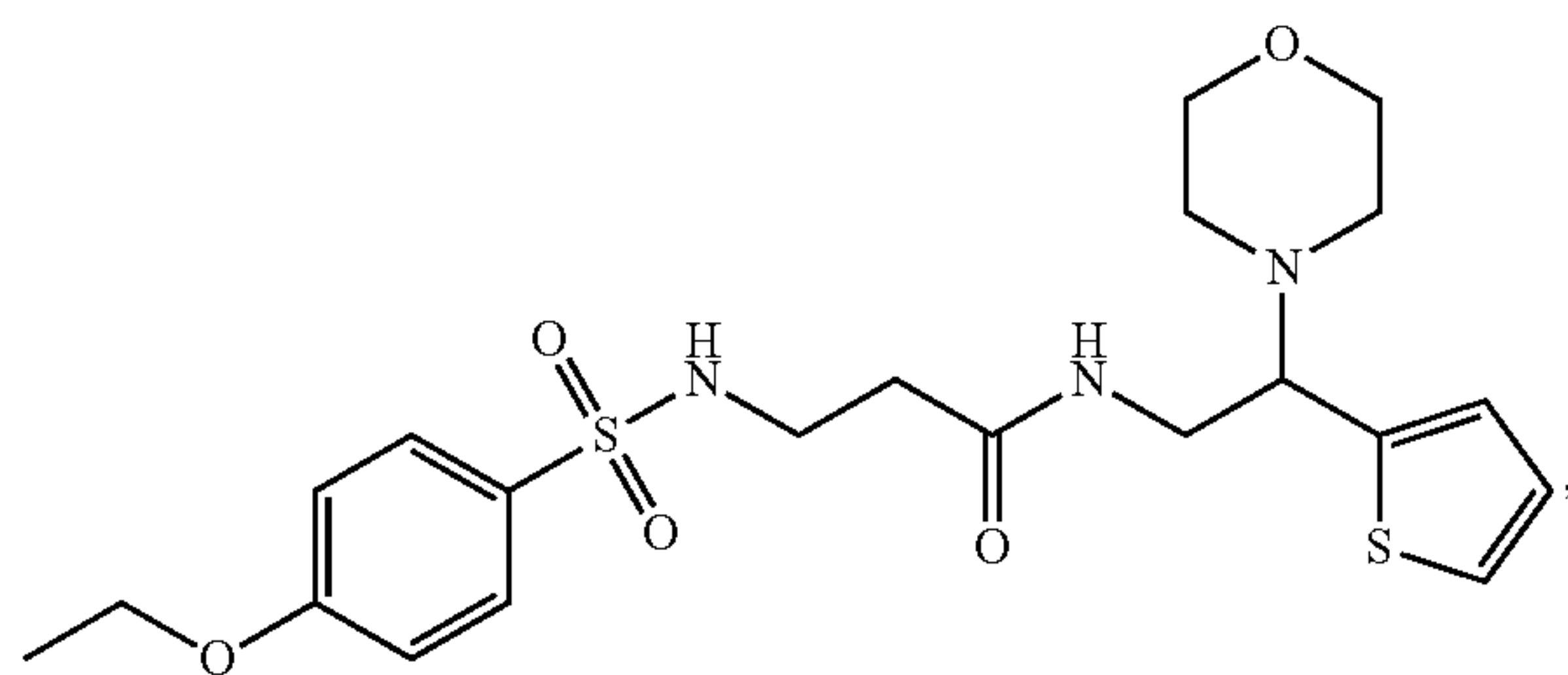
Compound 14
