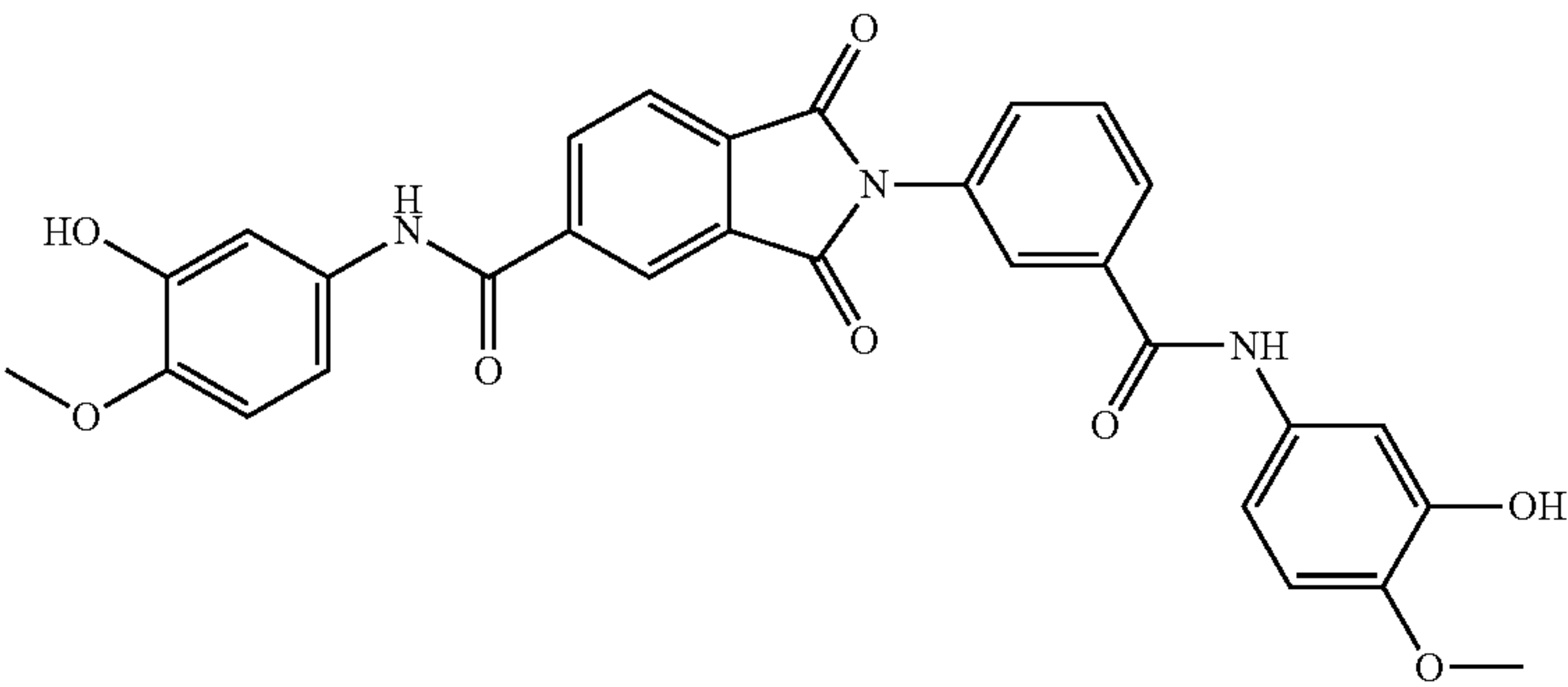
Compound 13
