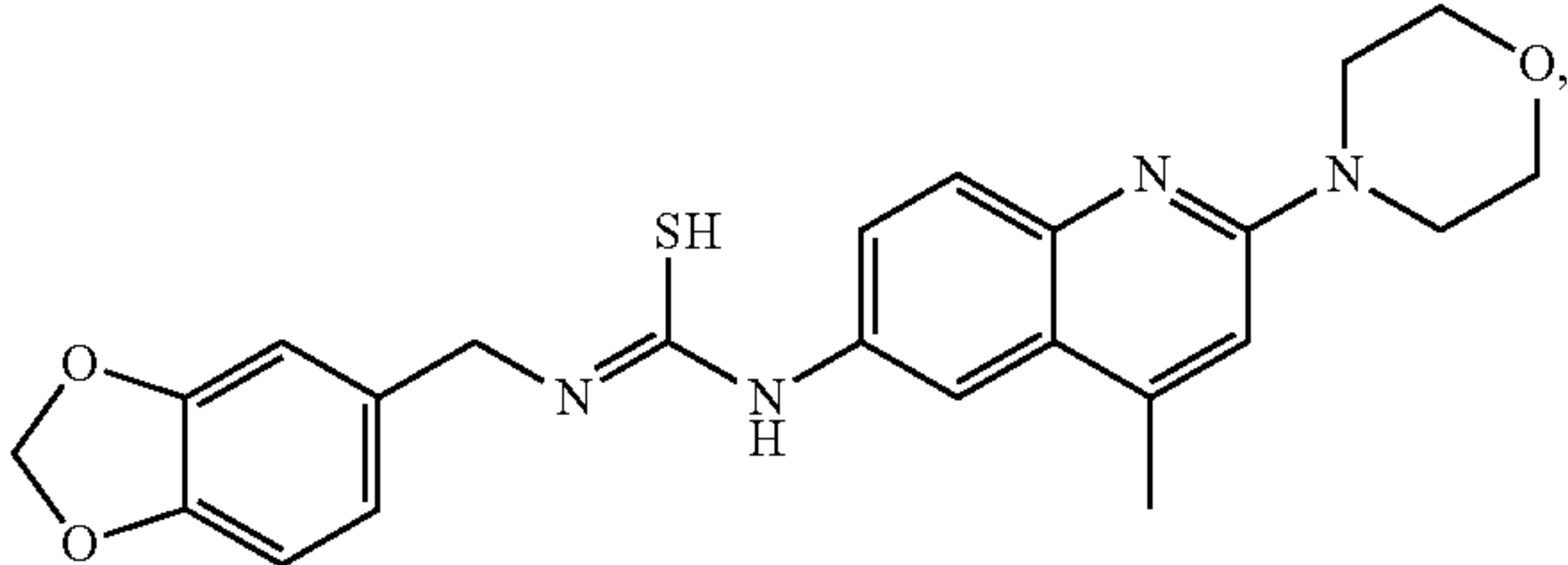
Compound 122
