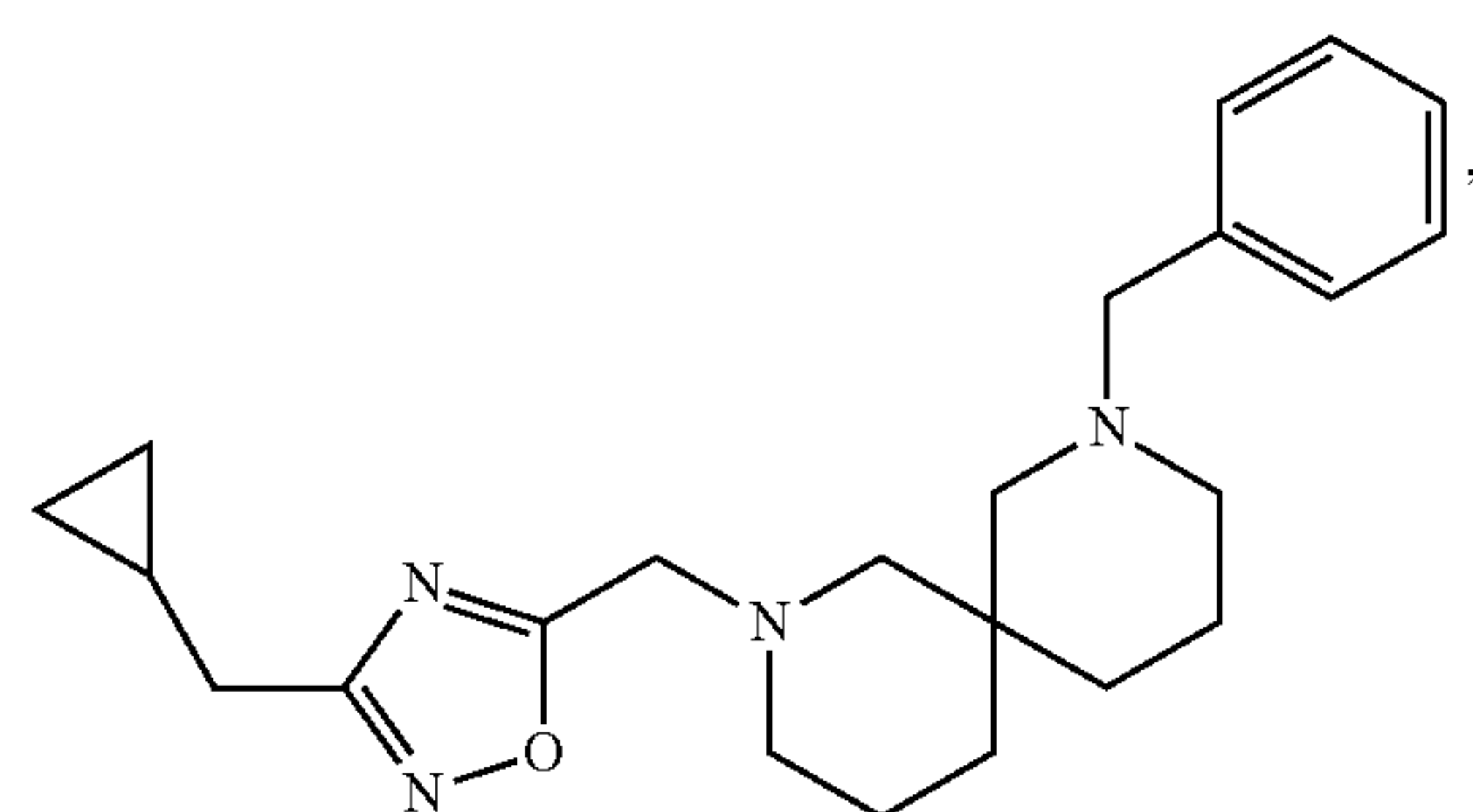
Compound 200
