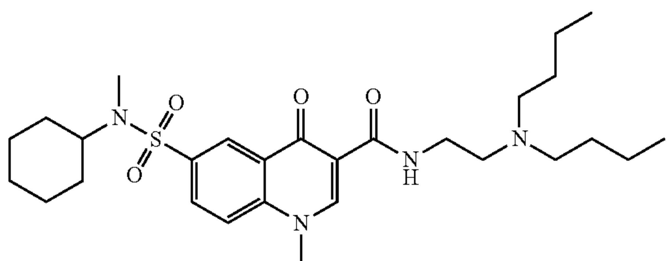
Compound 158
