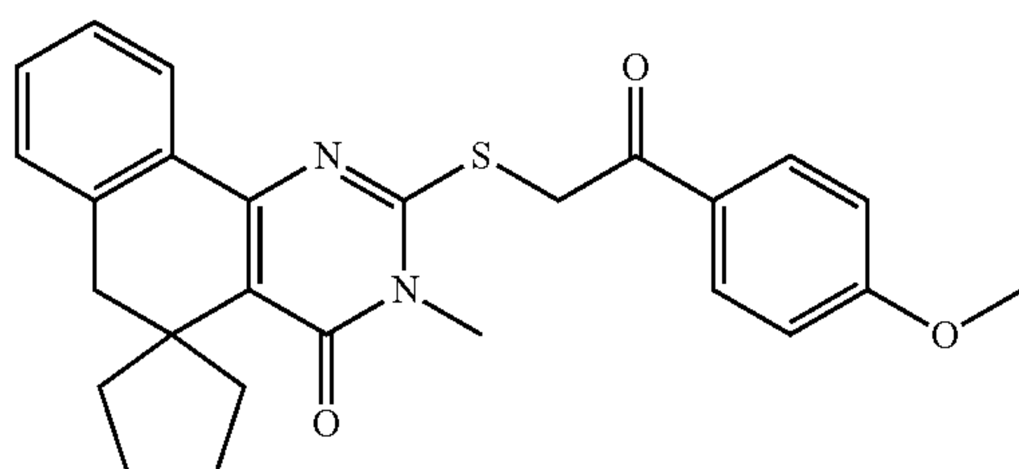
Compound 229
