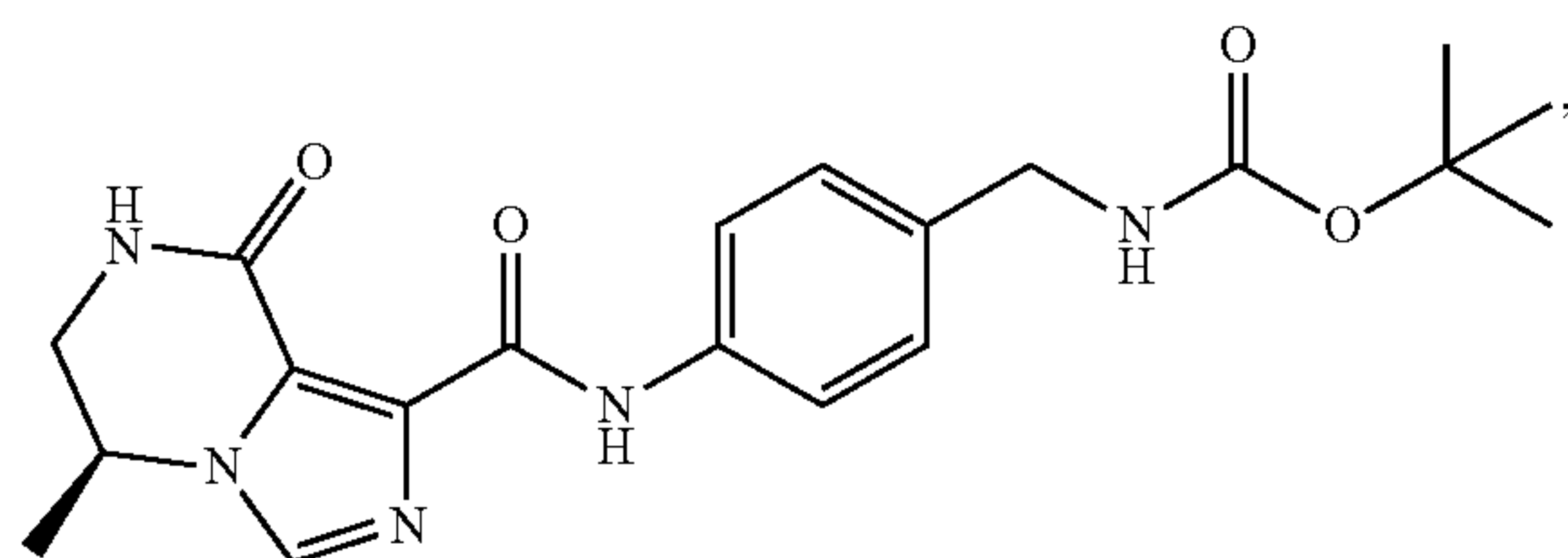
Compound 89
