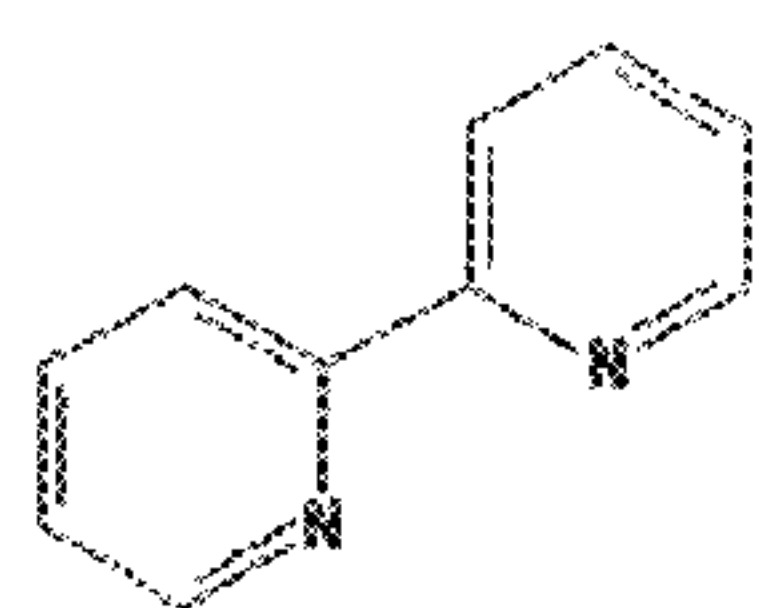
2,2-Dipyridyl
