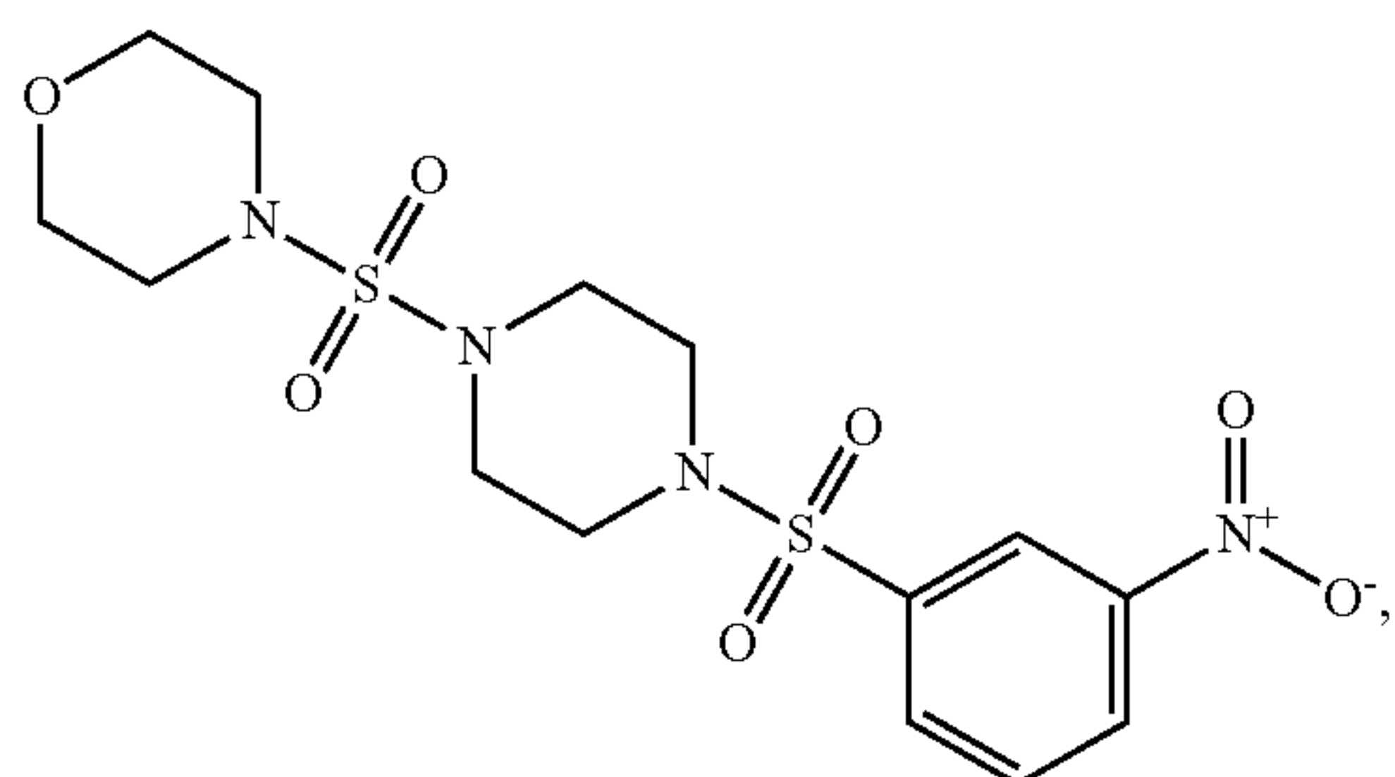
Compound 158
