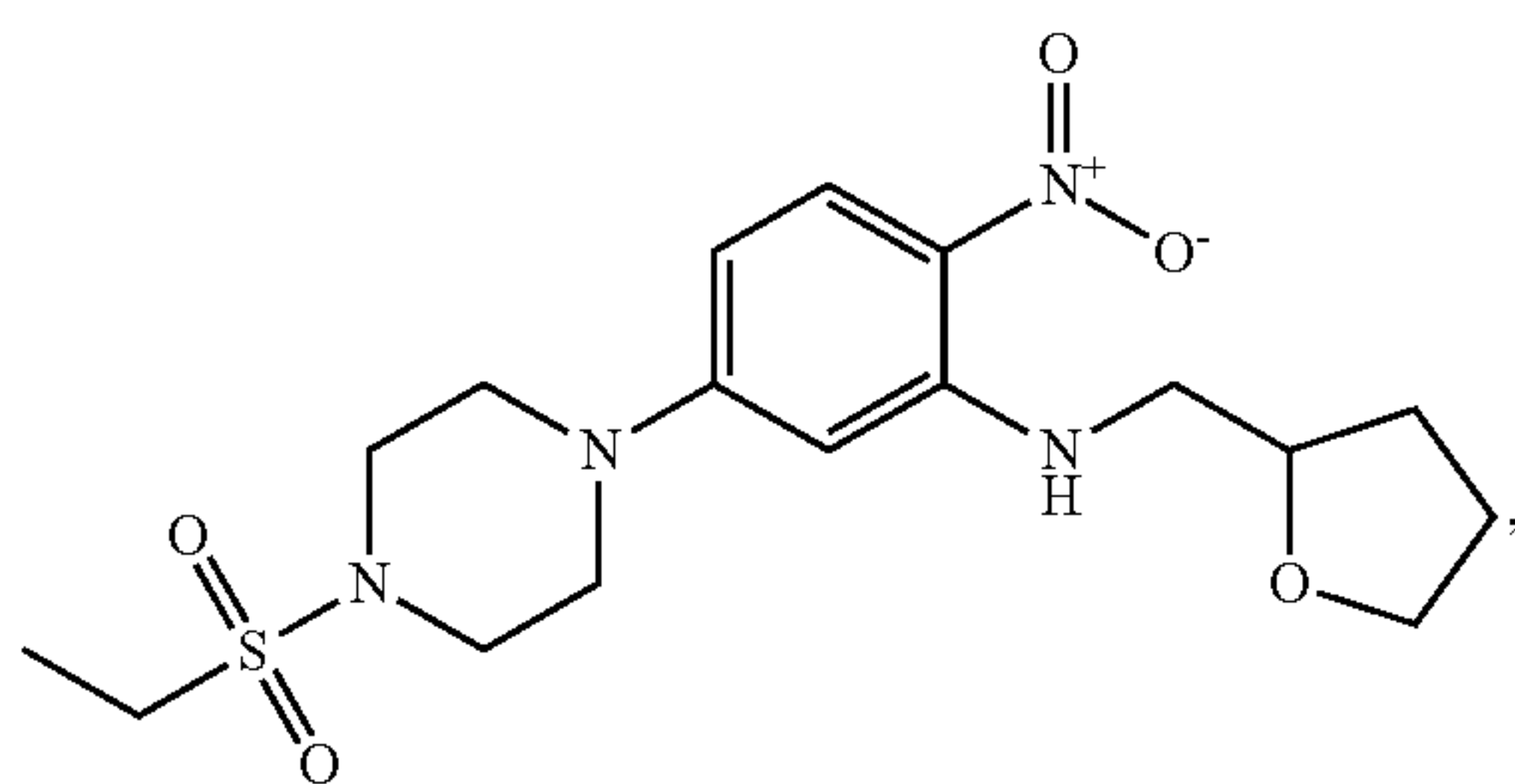
Compound 205
