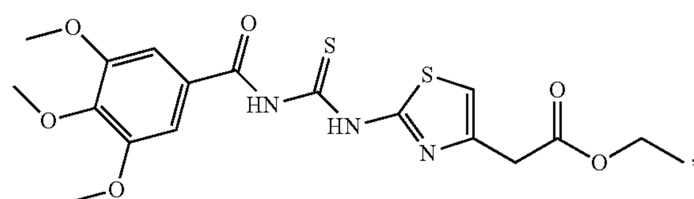
Compound 20
