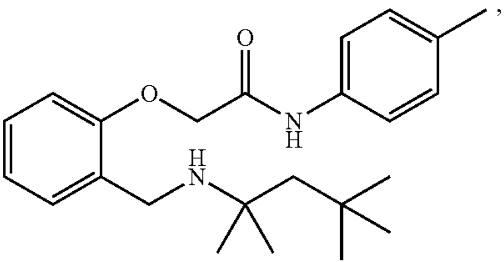
Compound 132
