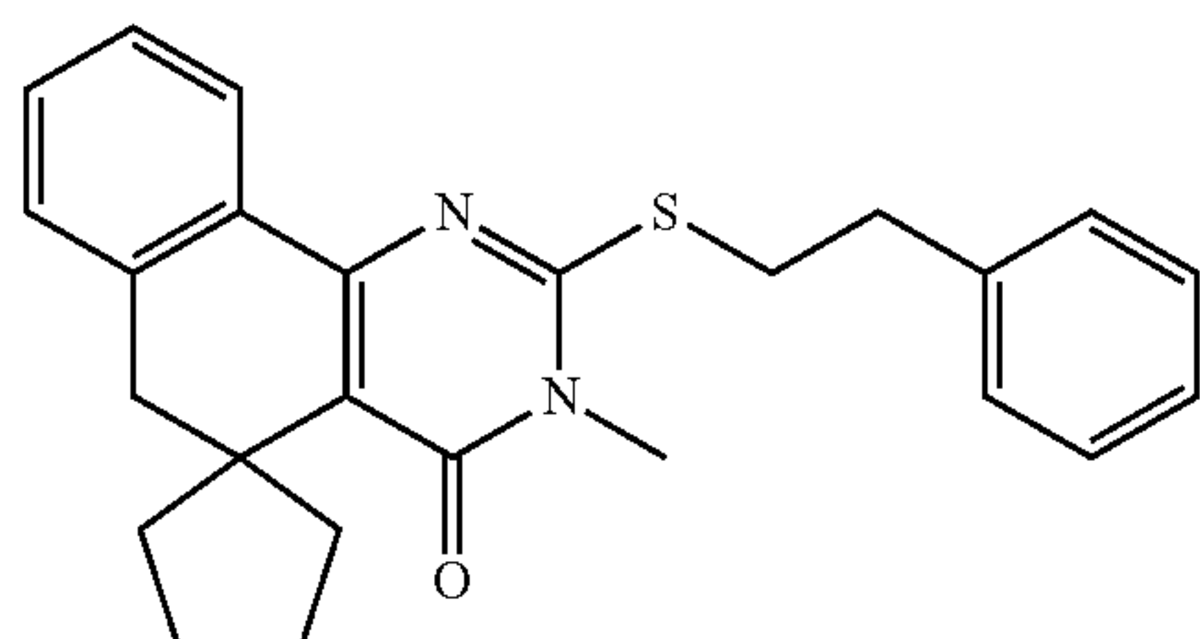
Compound 240
