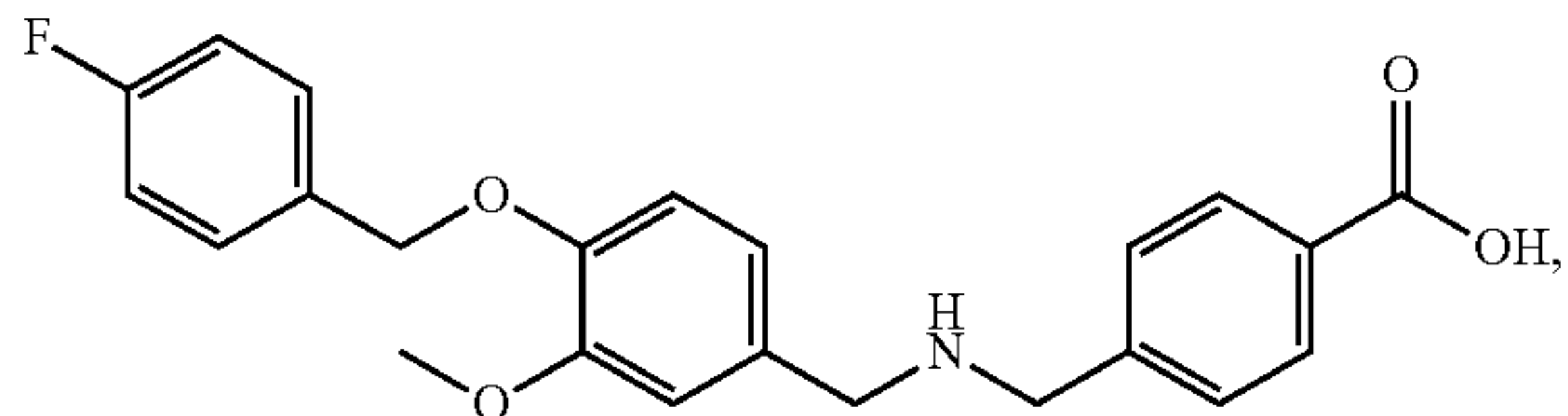
Compound 58
