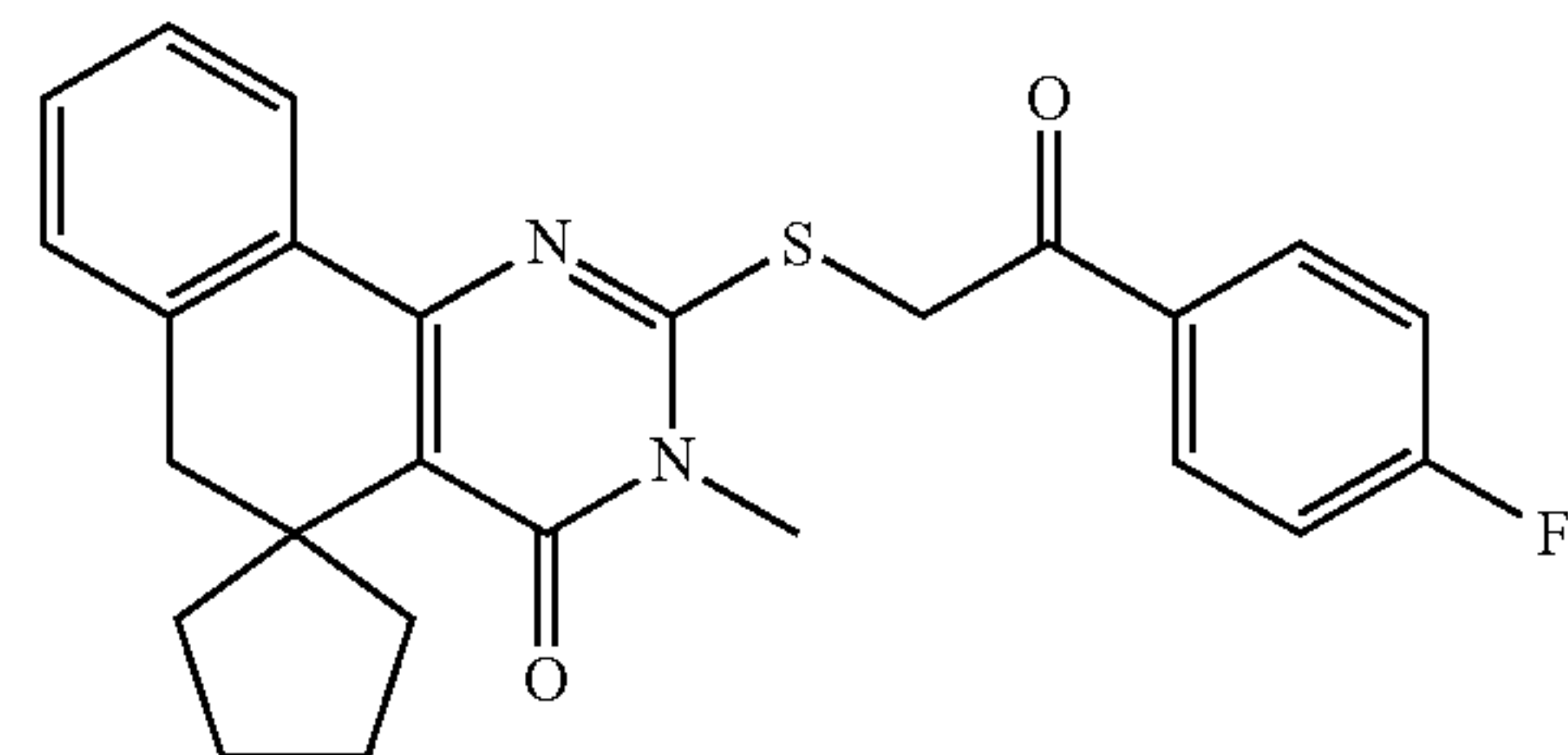
Compound 233
