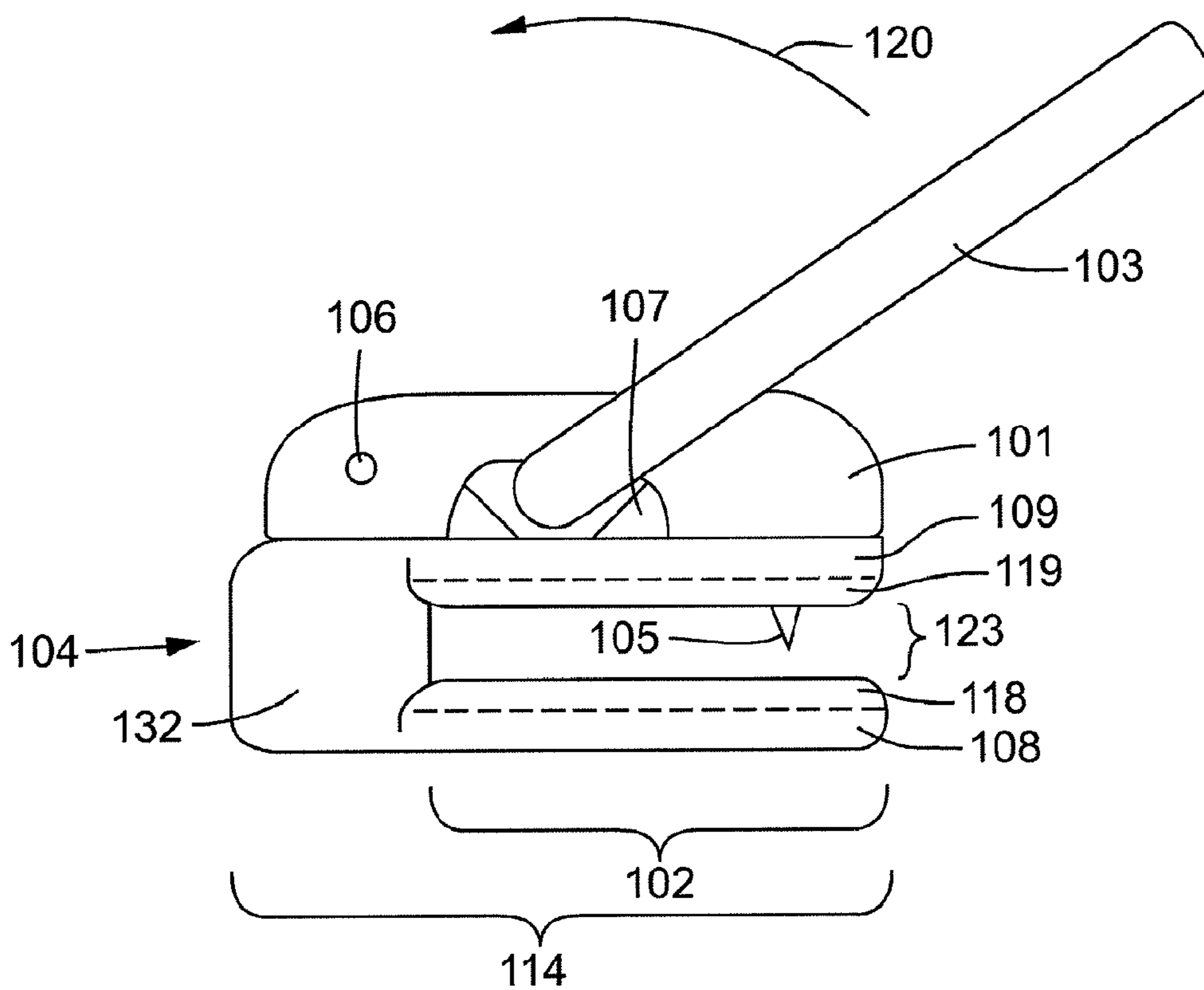
FIG. 1 (PRIOR ART)
