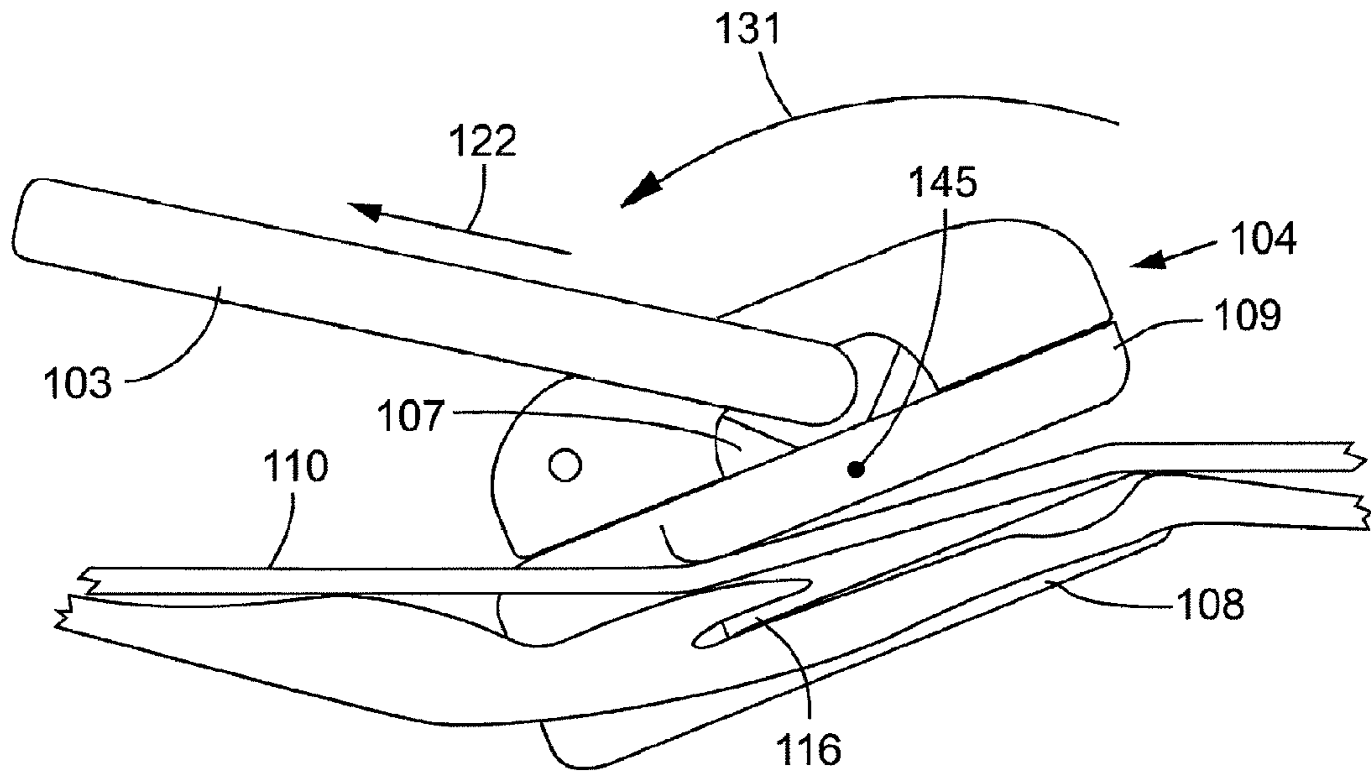
FIG. 4c (Prior Art)
