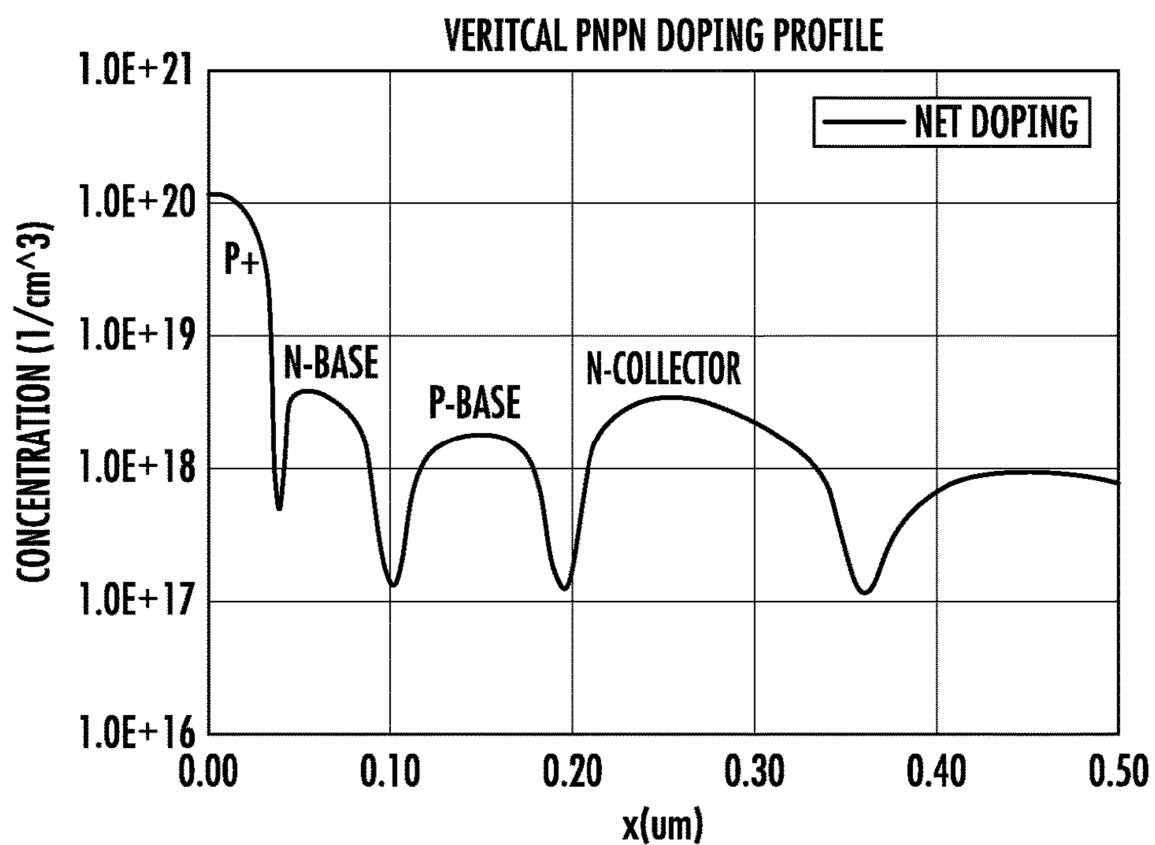
SRAM CELL DOPING PROFILE FIG. 33
