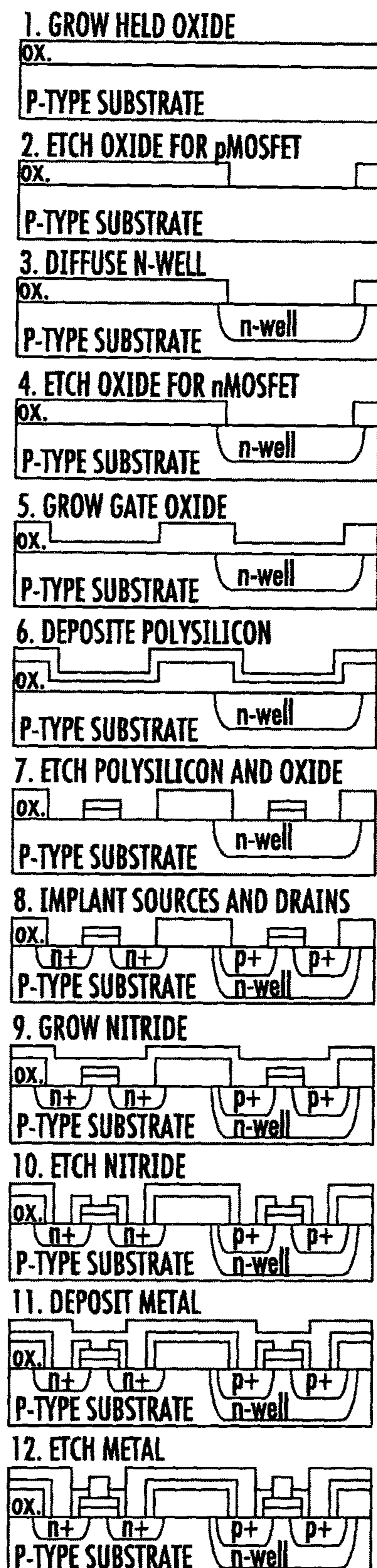
FIG. 10 (PRIOR ART)
