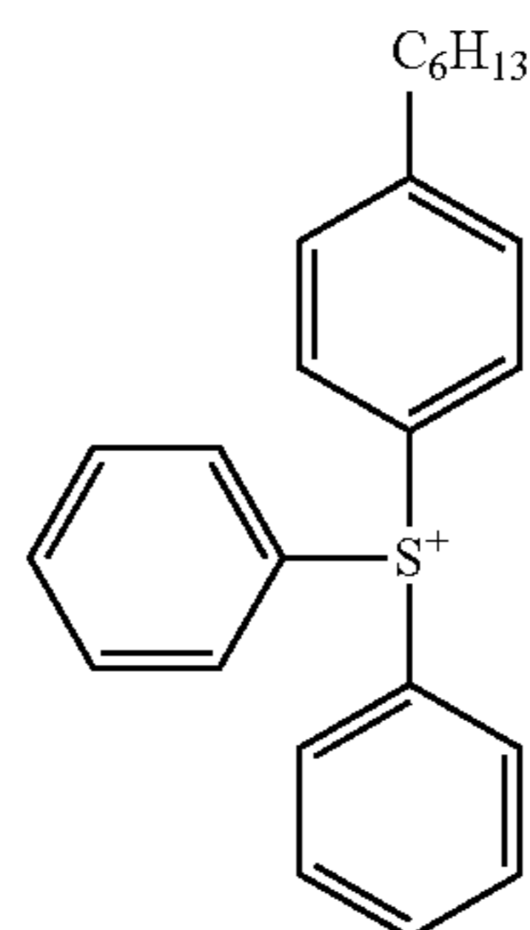
(b2-c-3)
