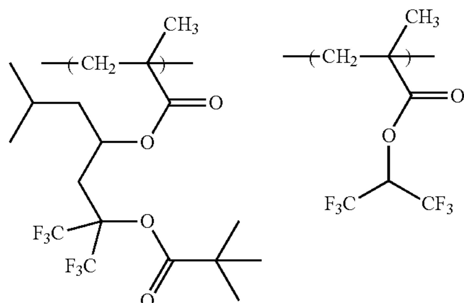
Synthesis Example 11
