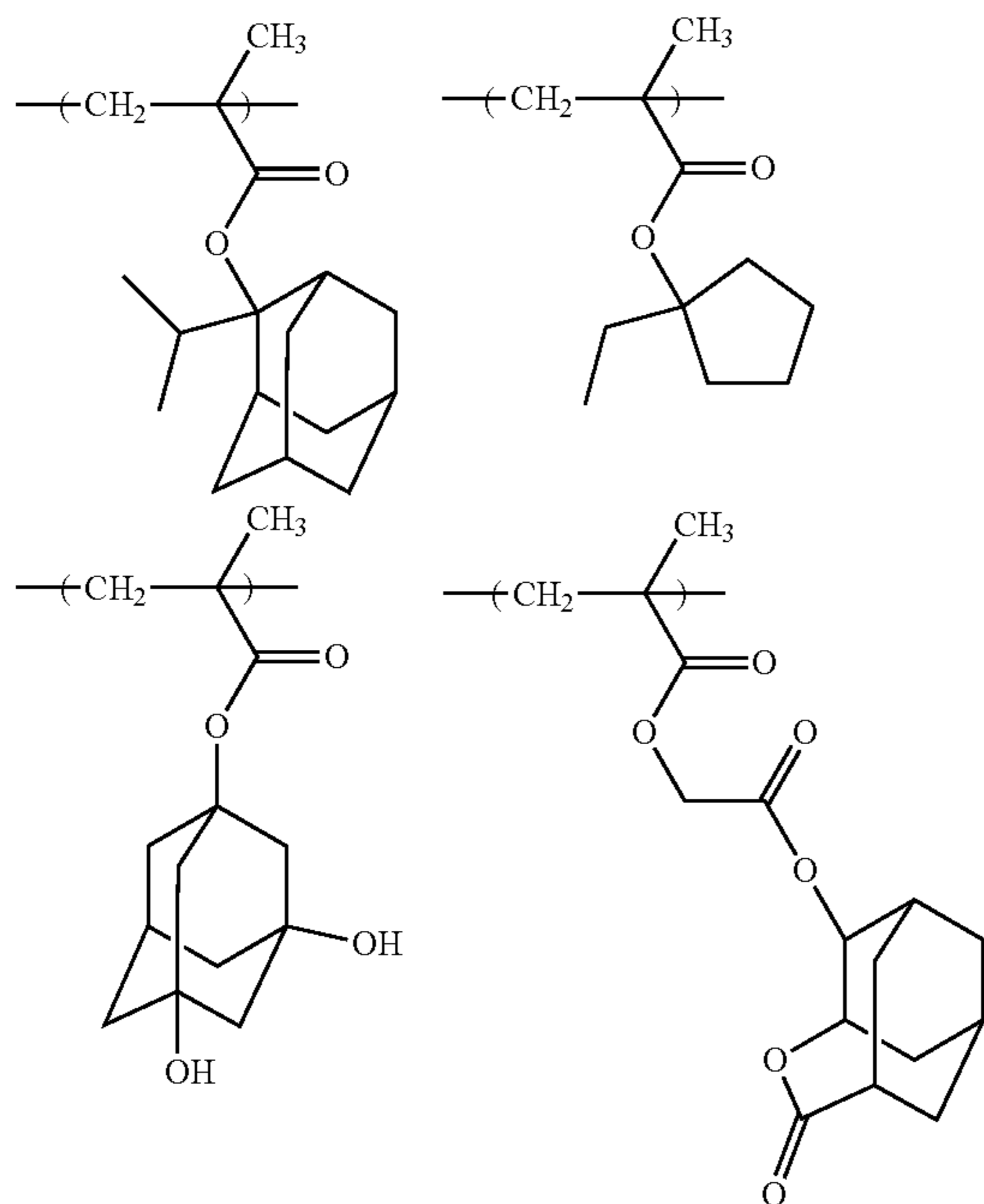
Synthesis Example 7
