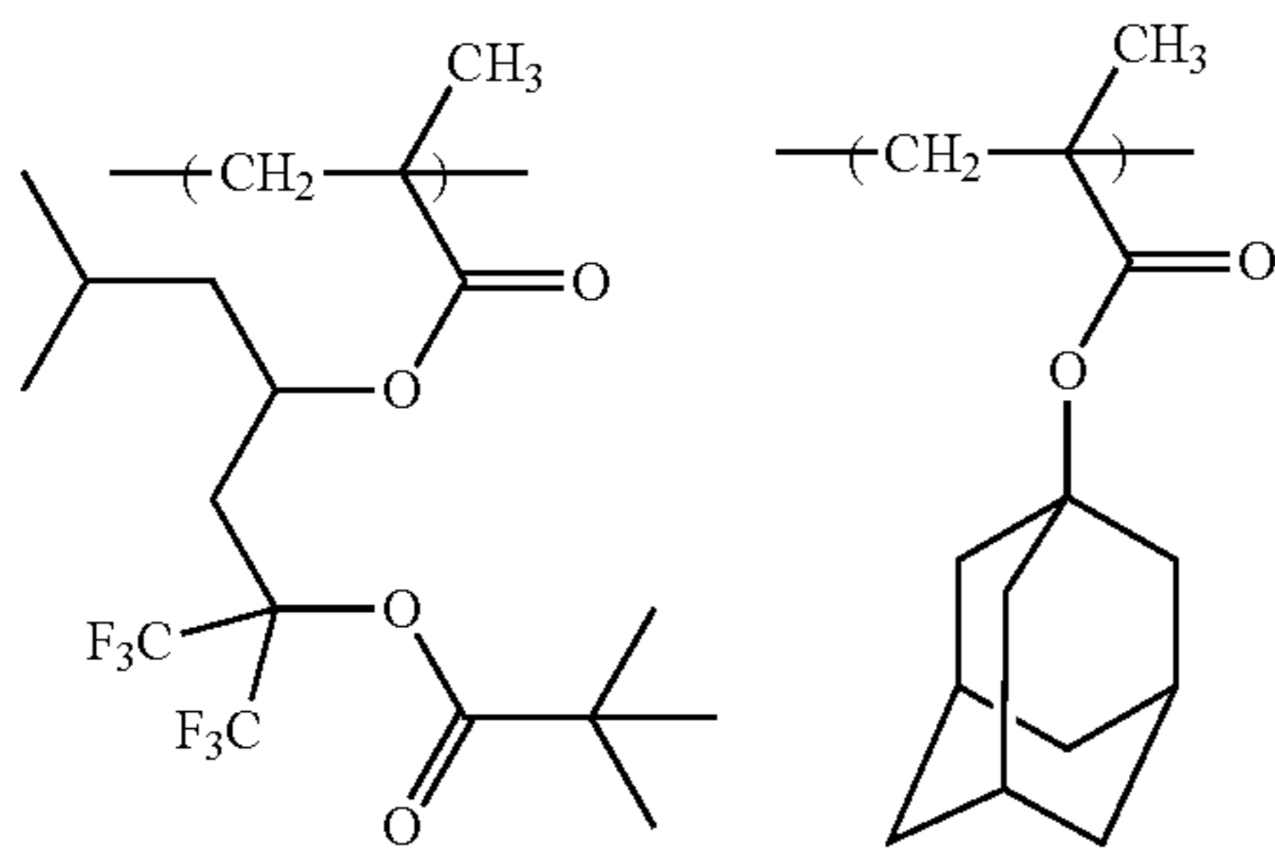
Synthesis Example 10
