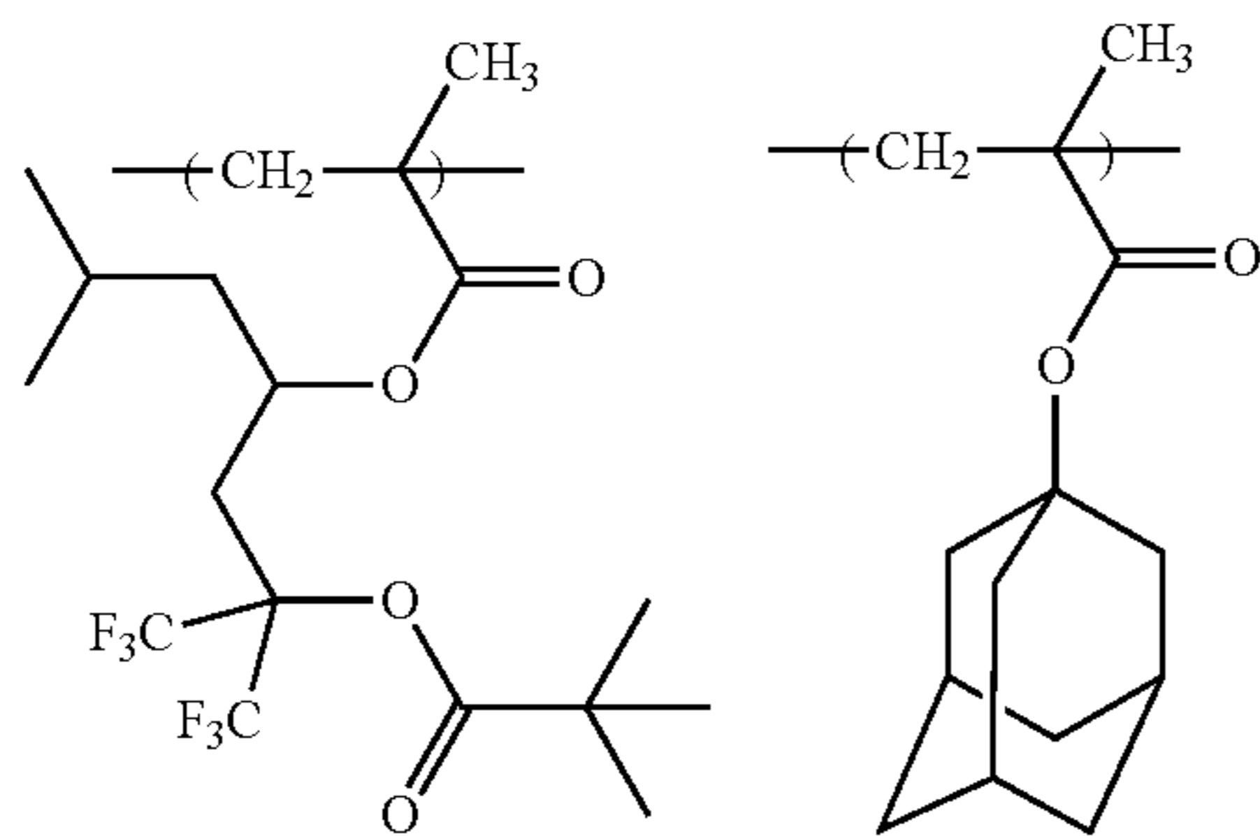
Synthesis Example 10
