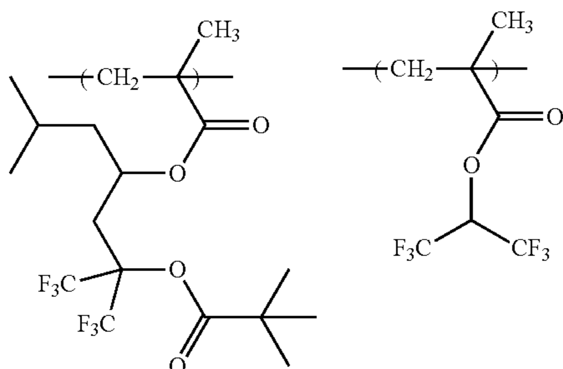
Synthesis Example 11
