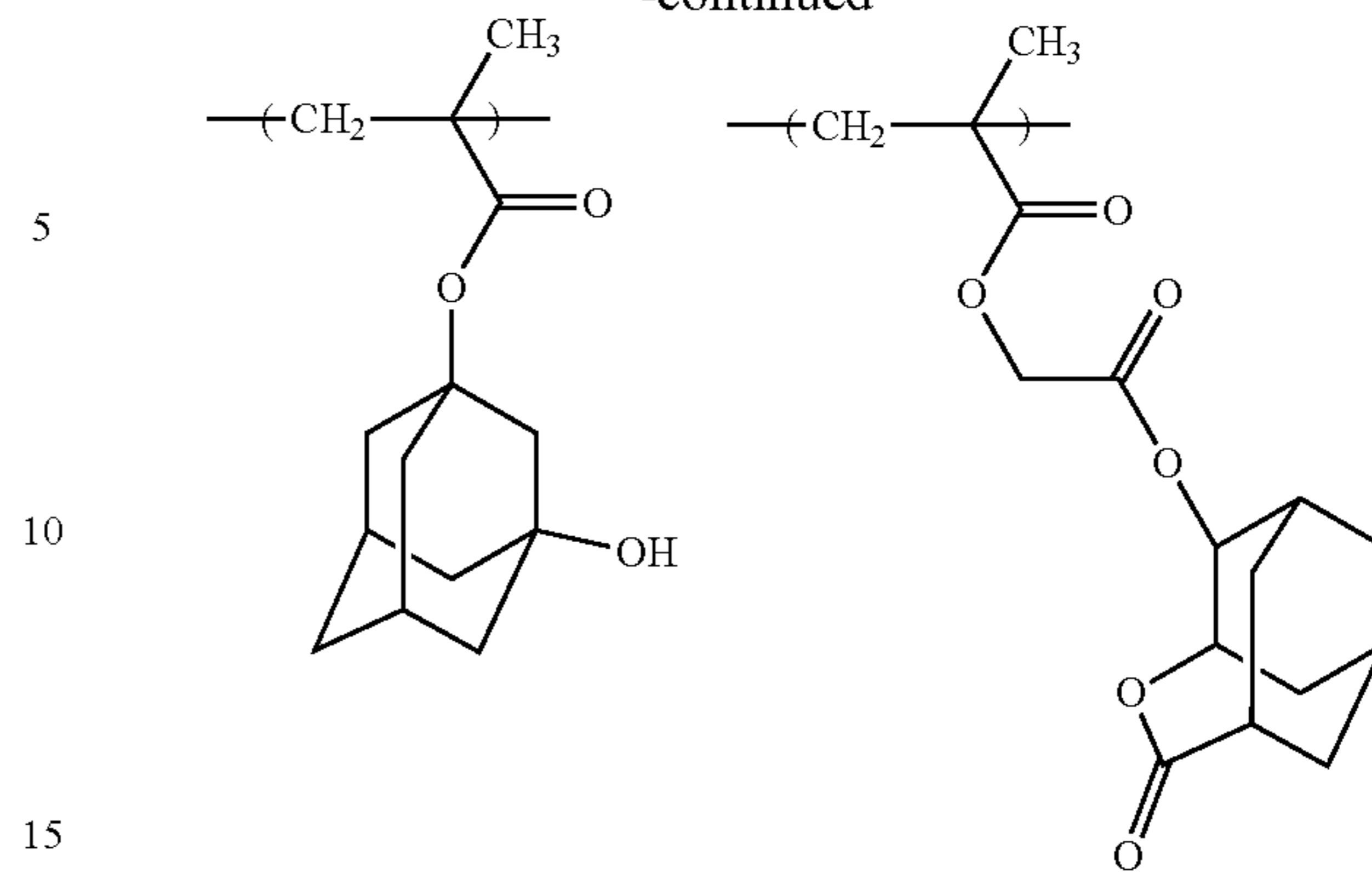
Synthesis Example 8
