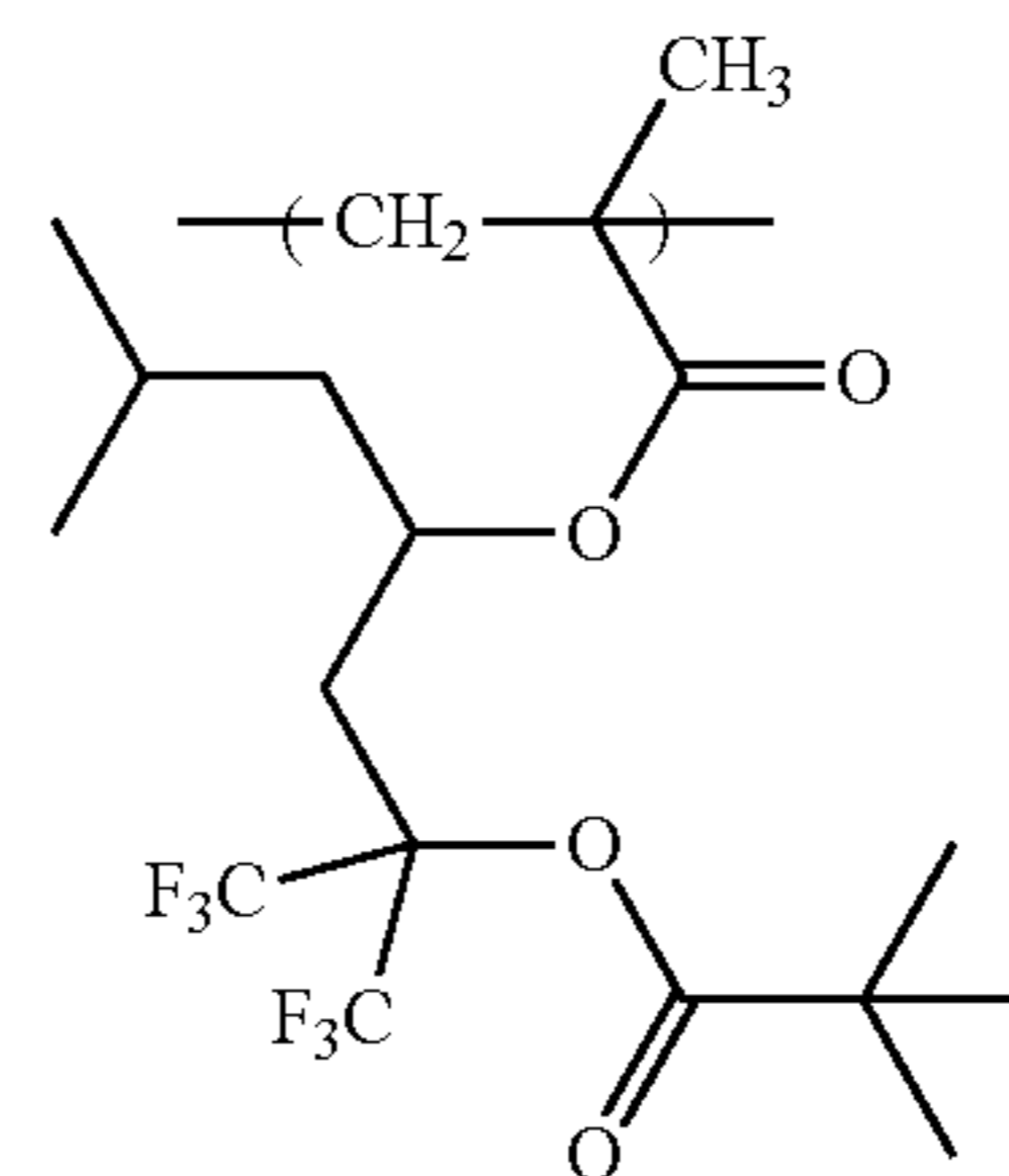
Synthesis Example 9
