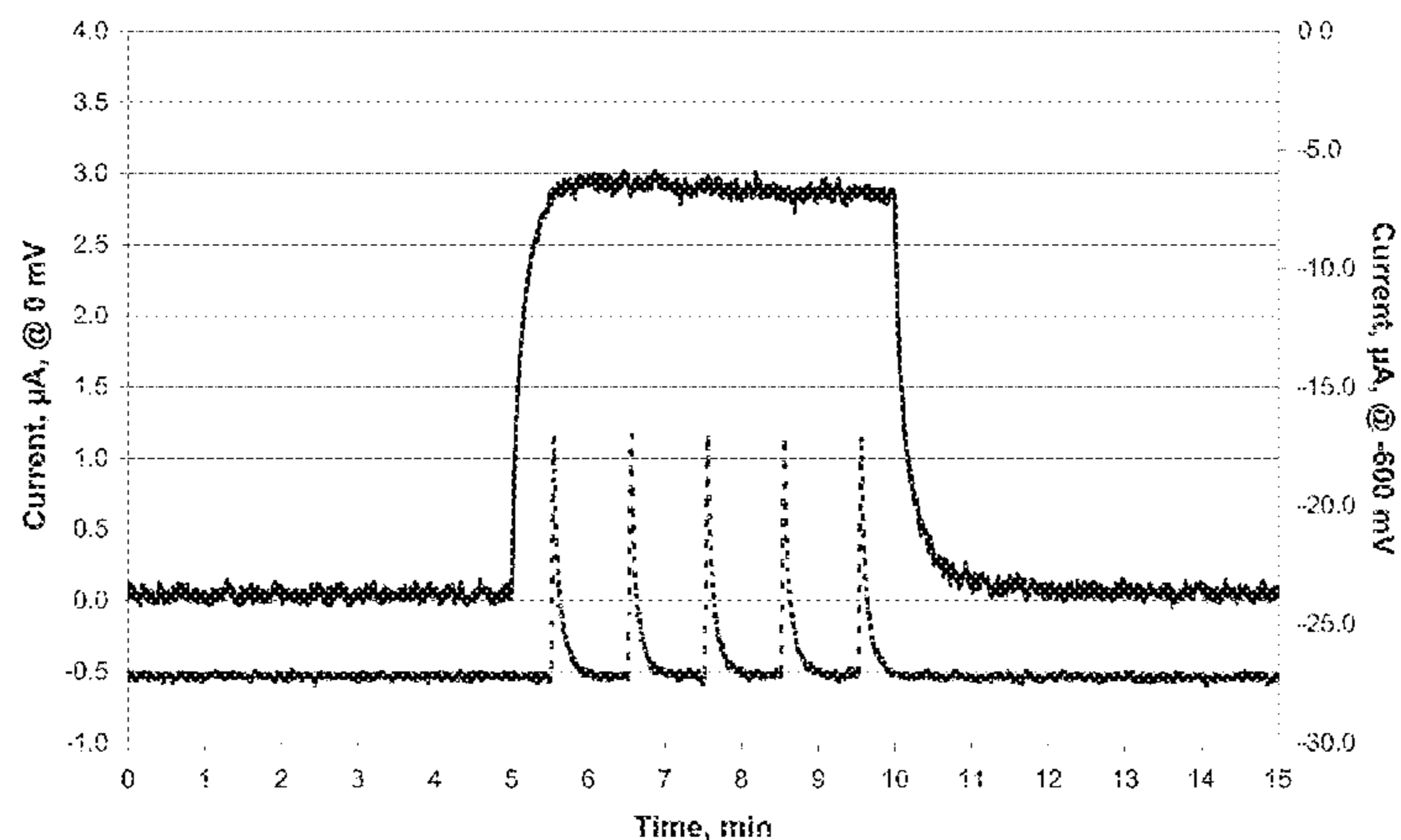
H 2 S Sensor w/Interrogation, Operated at Two Potentials
