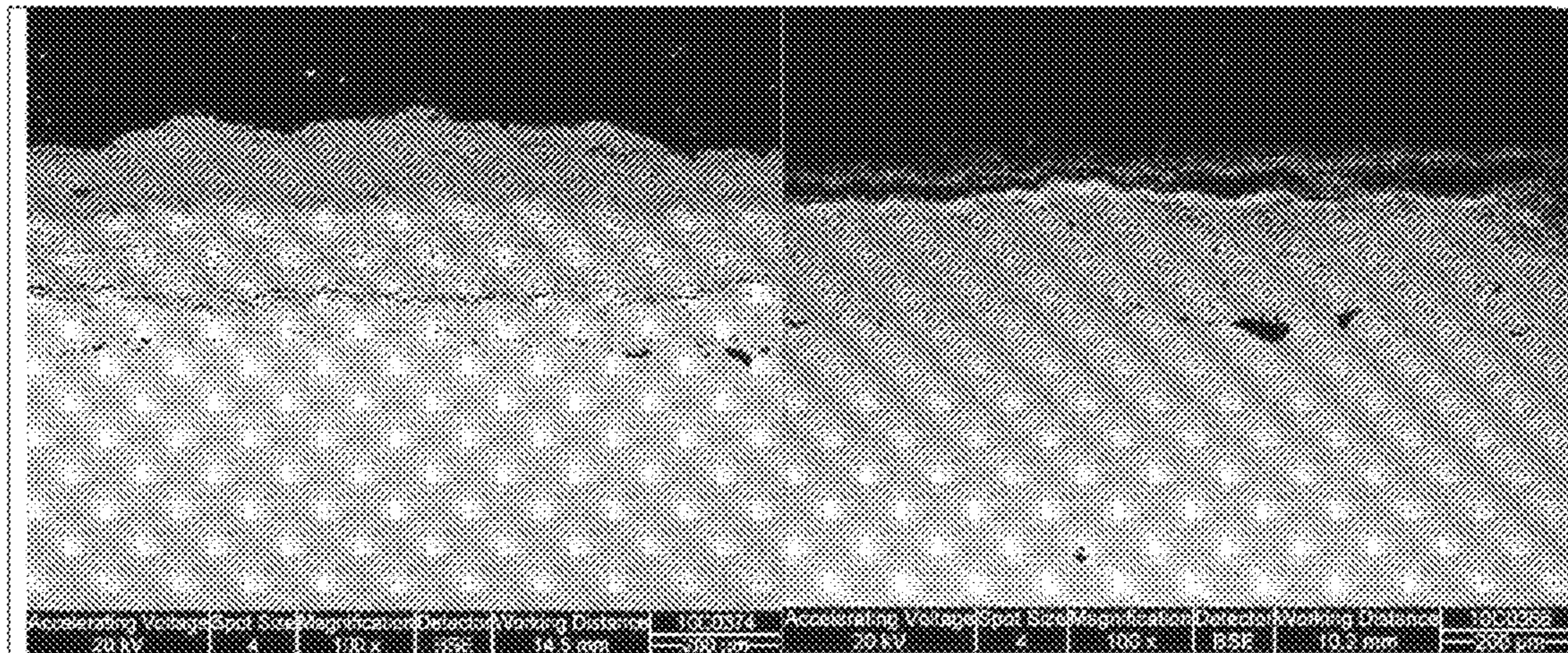
Reference NiCr coating after KCl exposure
