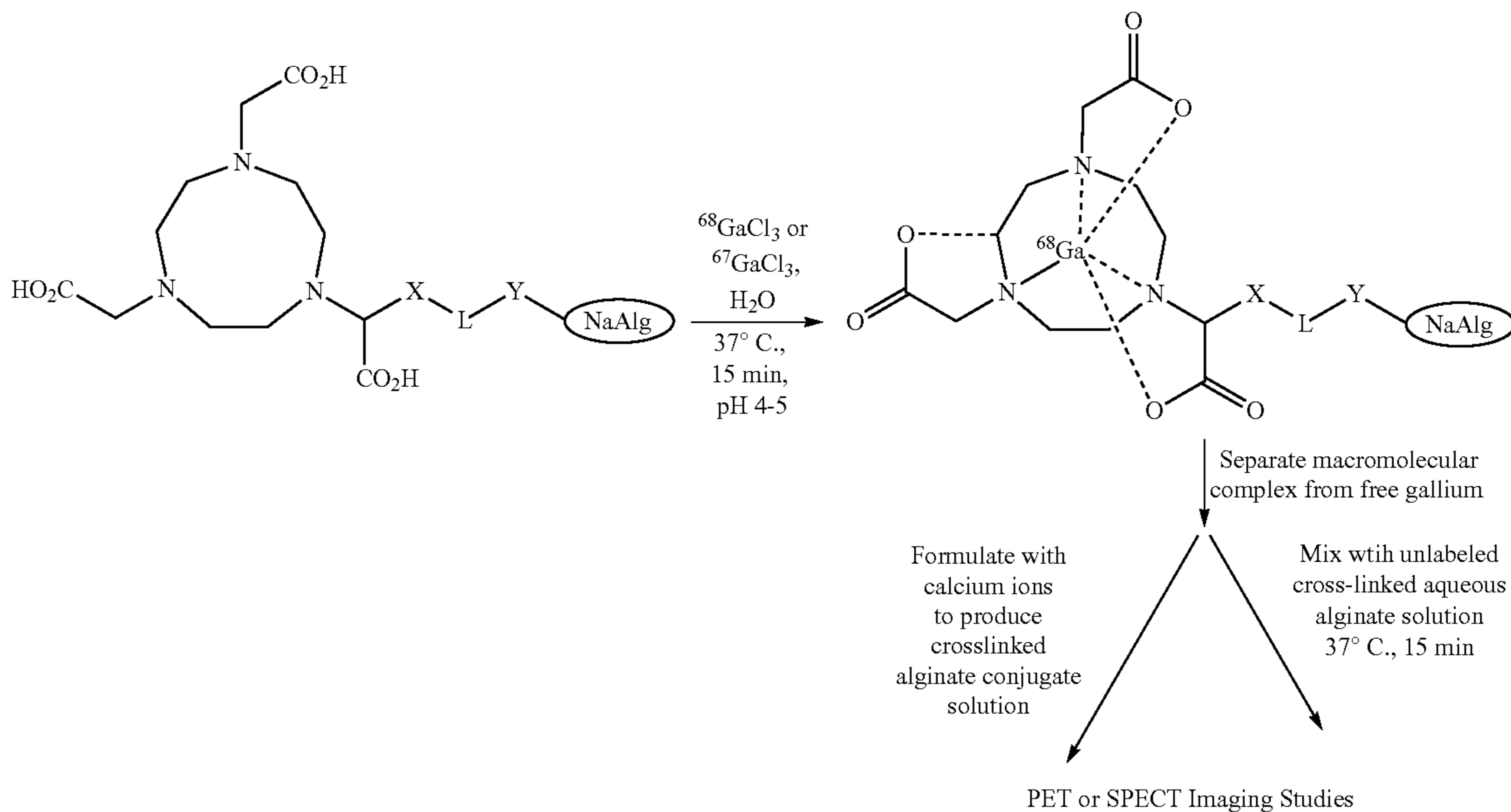
Scheme 6: Gallium Labeling of NOTA-Alginate Conjugate
