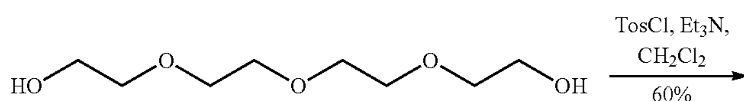
Scheme 4: Synthesis of N-methylhydroxylamine-Containing NOTA Linker
