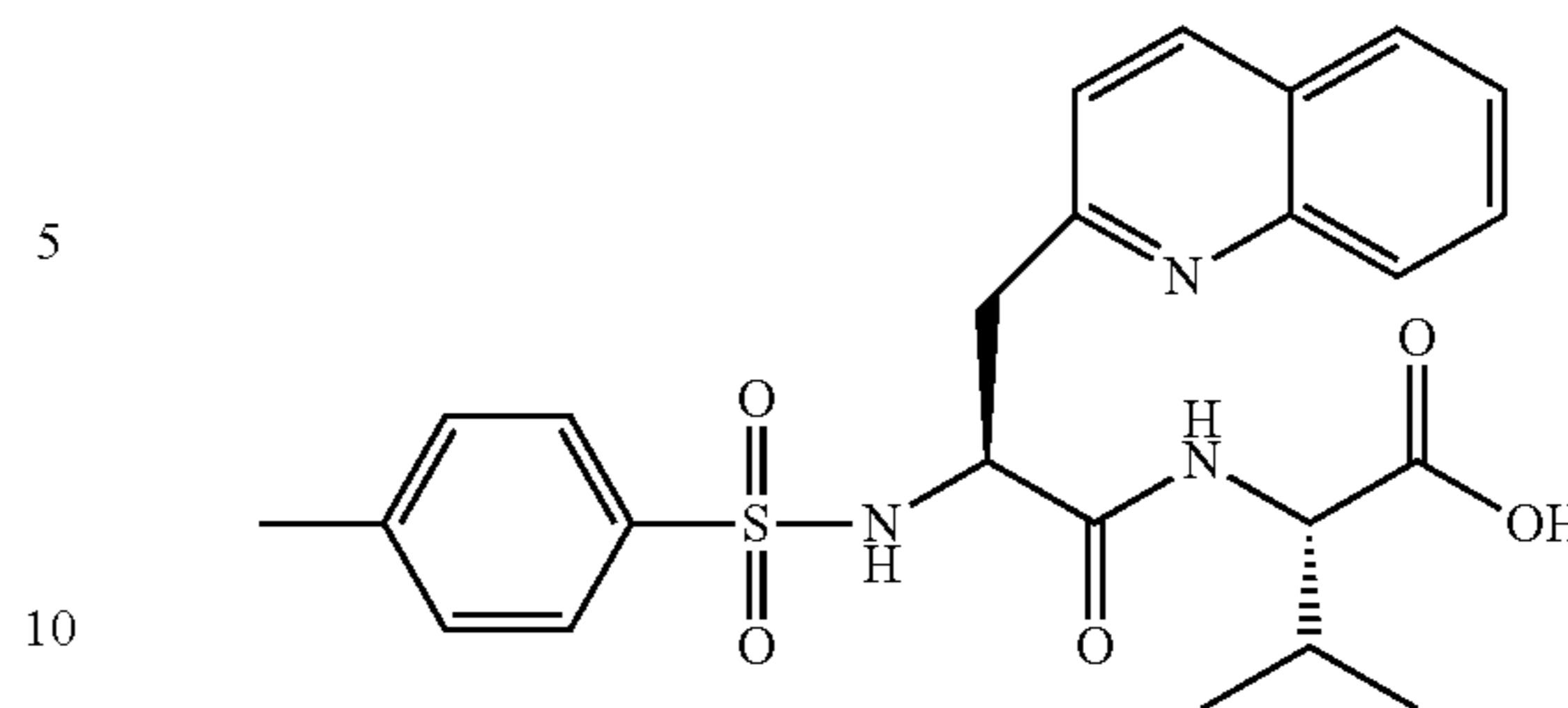
c) Ts-Ala(2'-quinolylyl)-Val-OH
