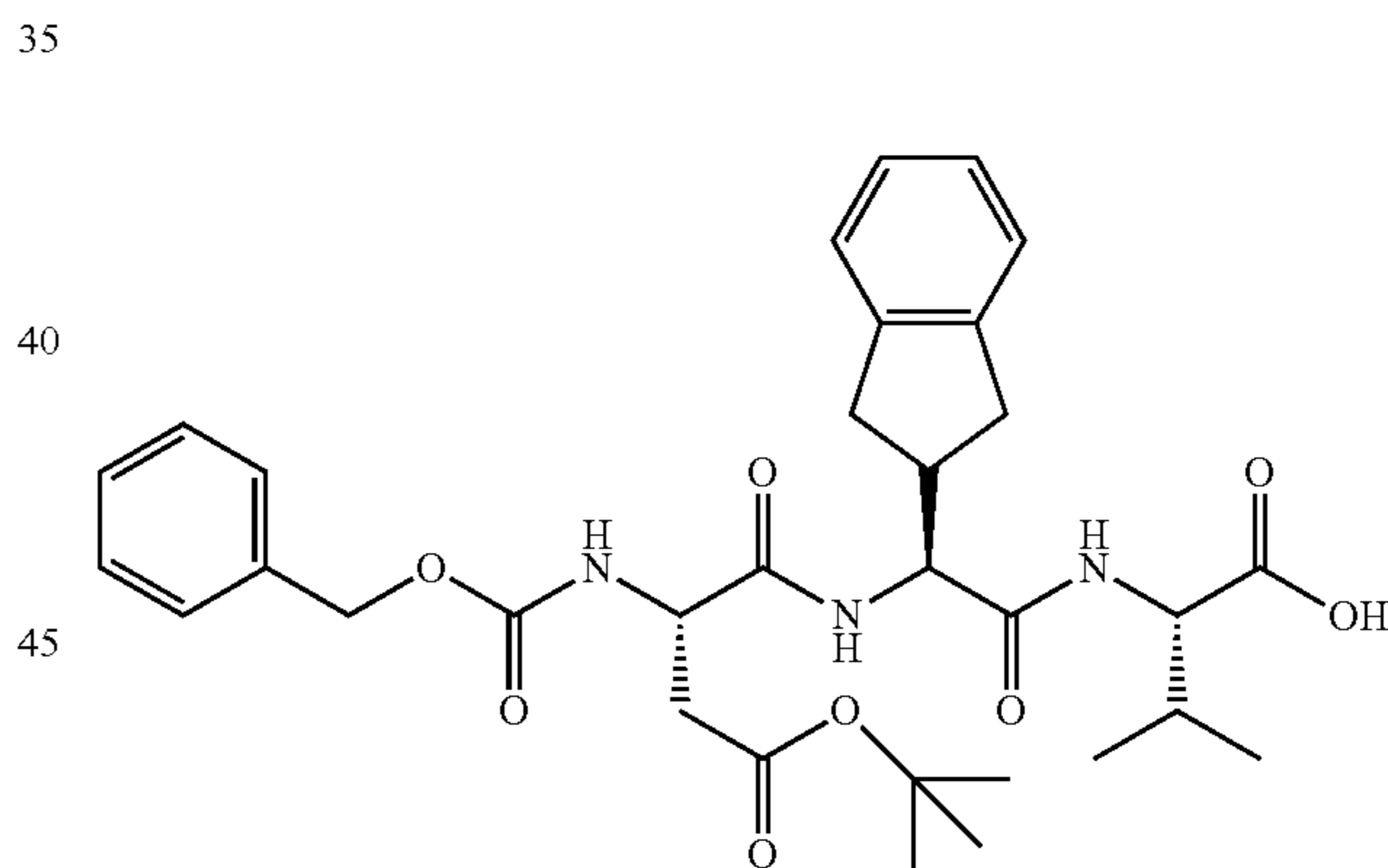
a) Fmoc-Indanylglycine-Val-OAllyl
