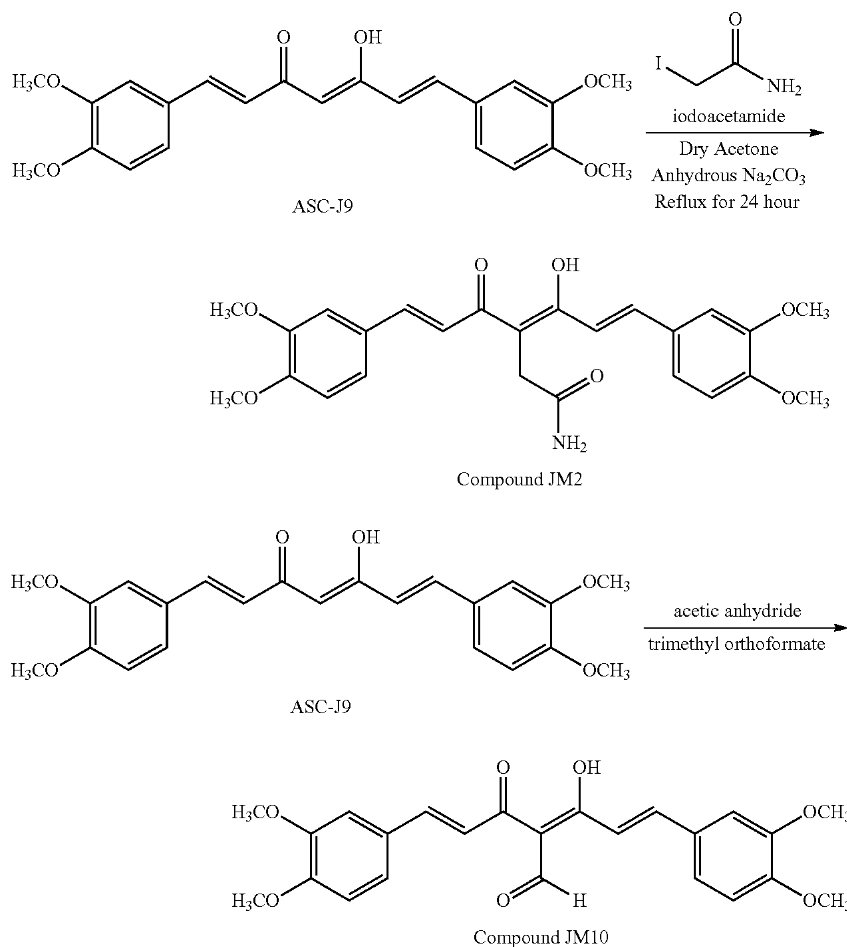
Scheme 7
