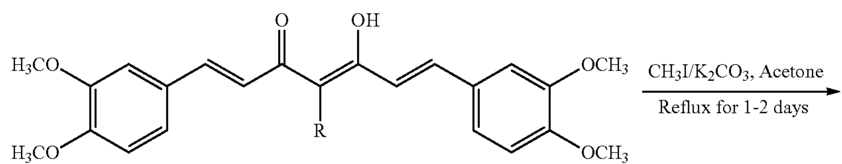
Scheme 14
