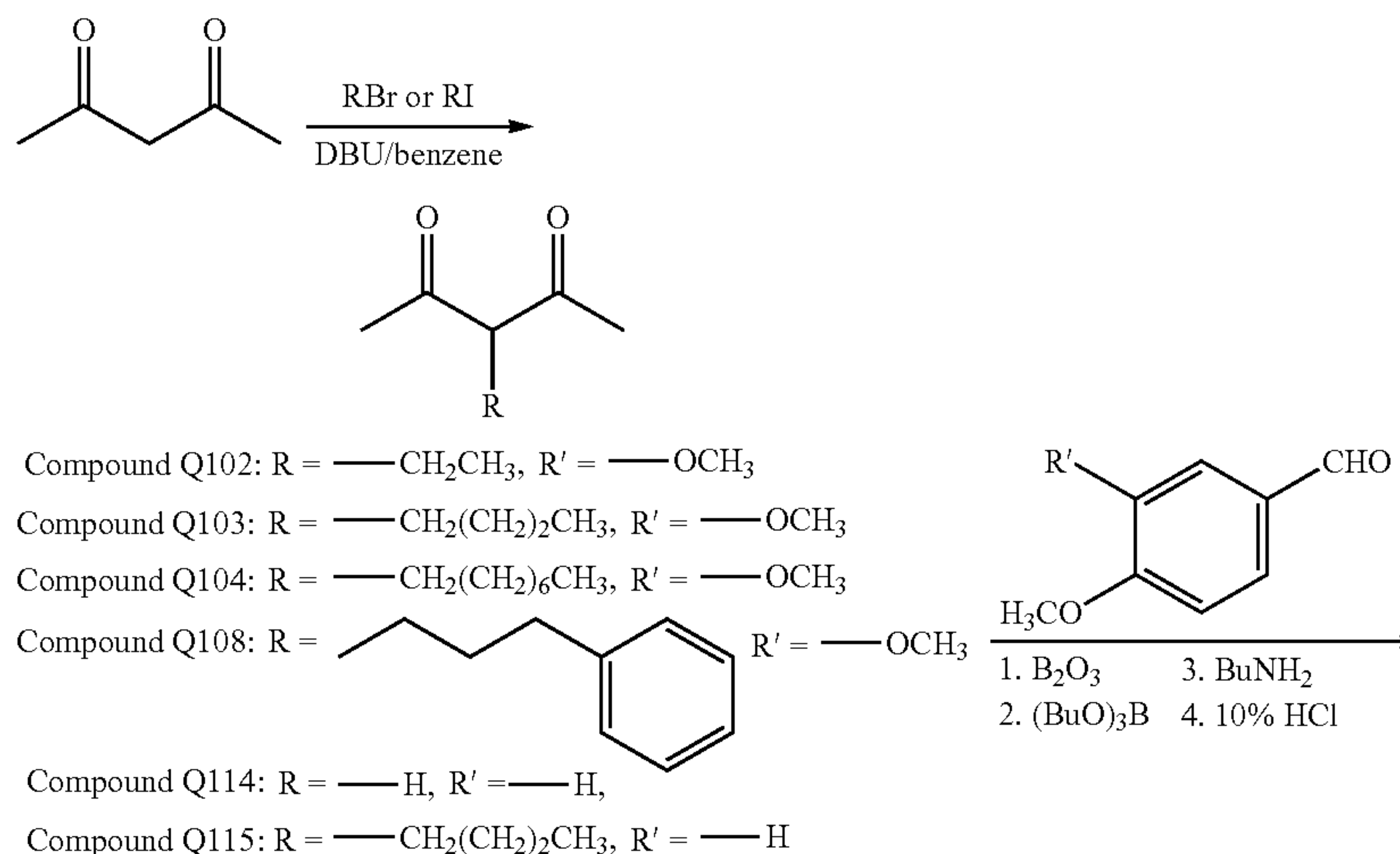
Scheme 10
