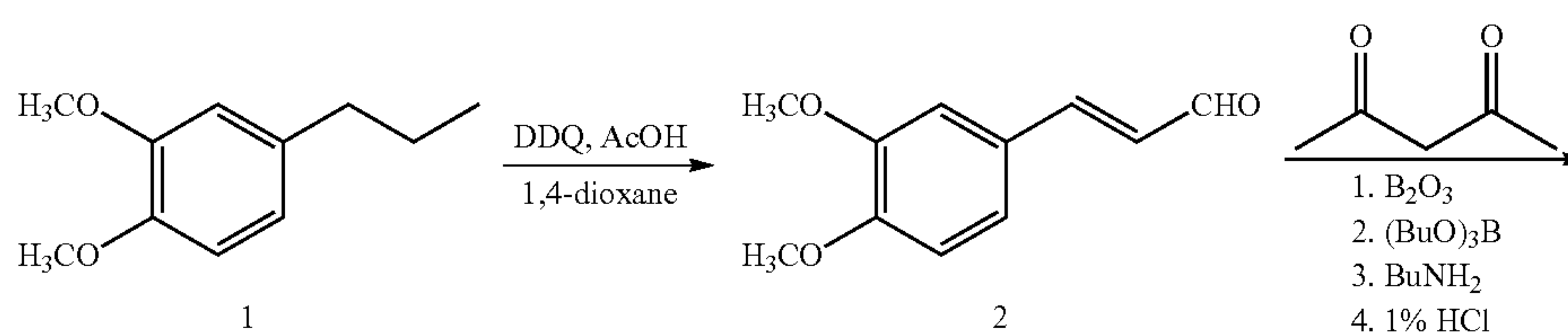
Scheme 13
