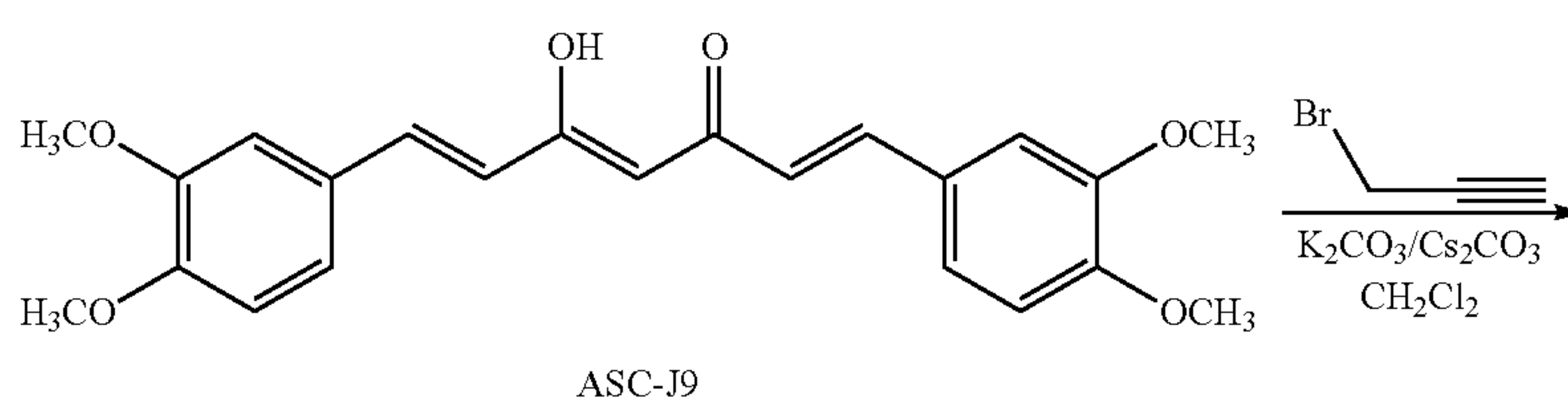
Scheme 8
