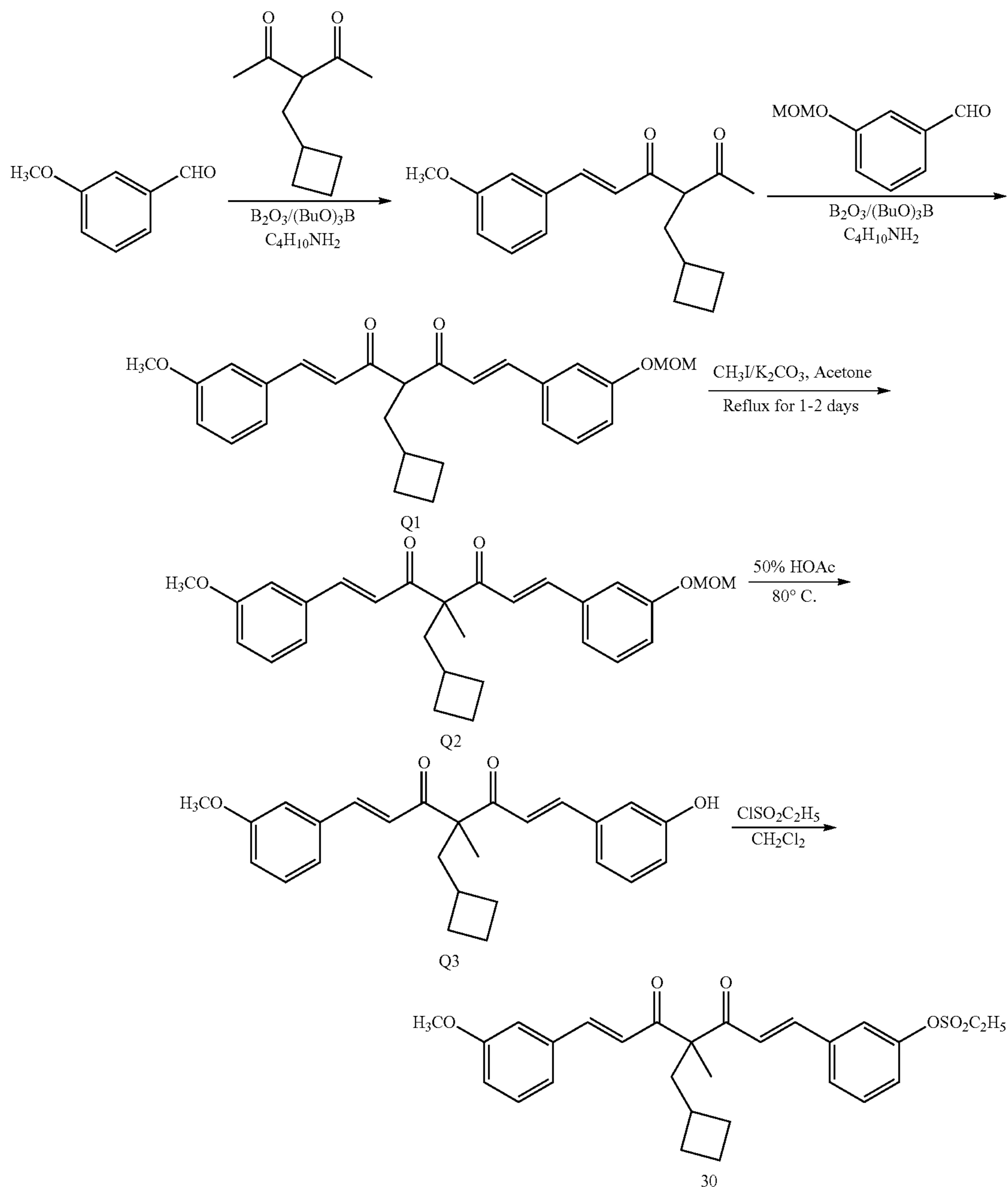
Scheme 19
