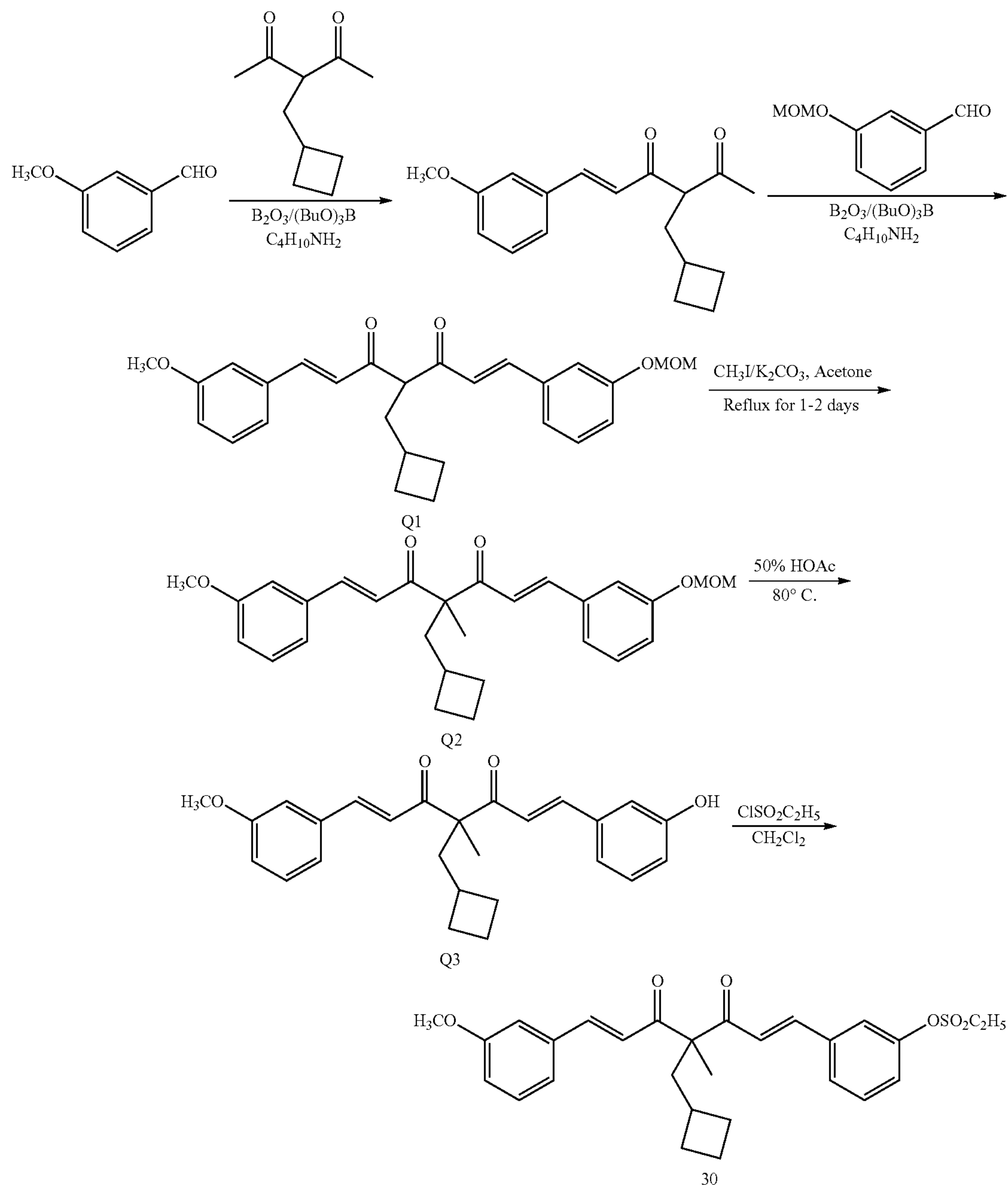
Scheme 19
