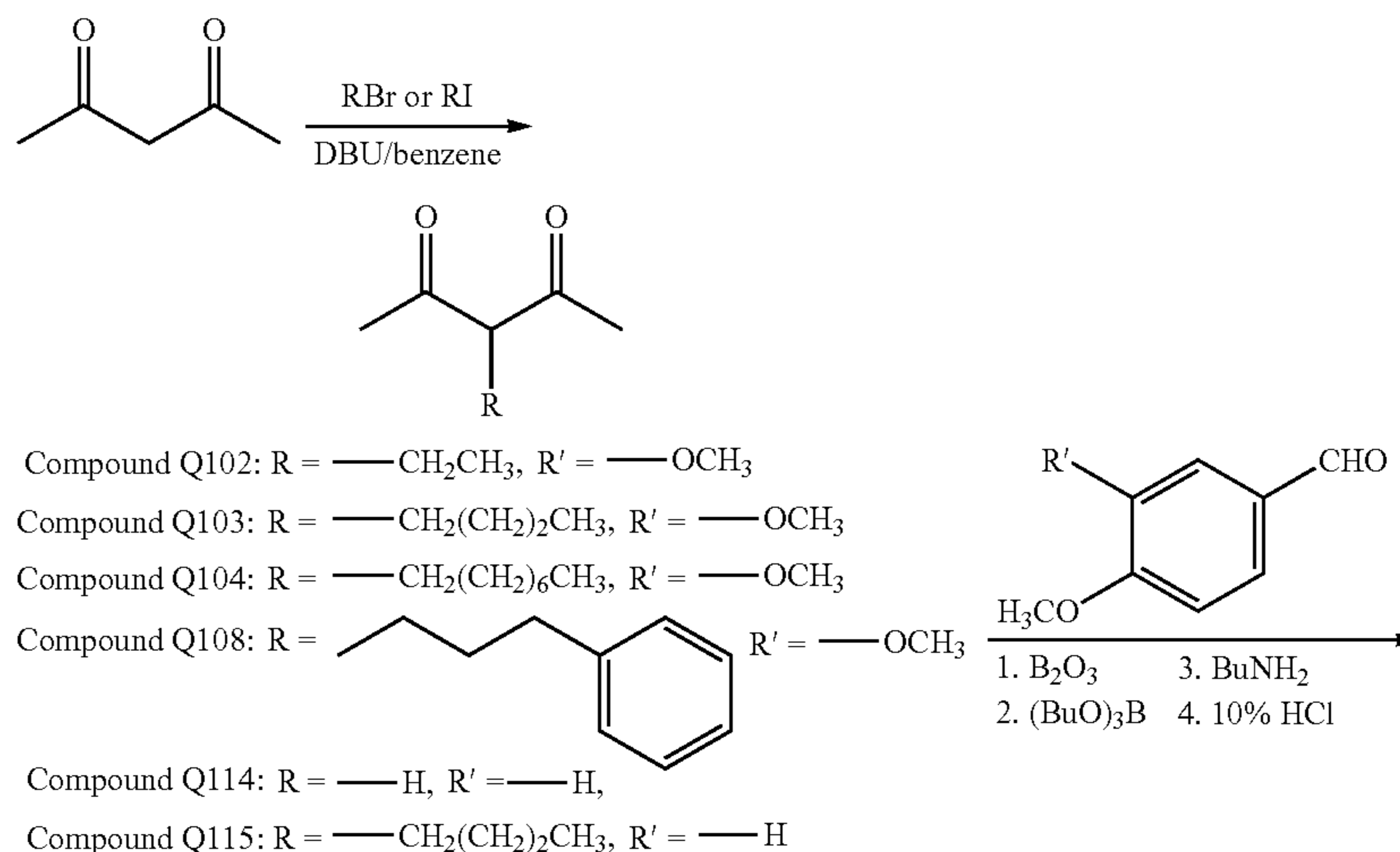
Scheme 10
