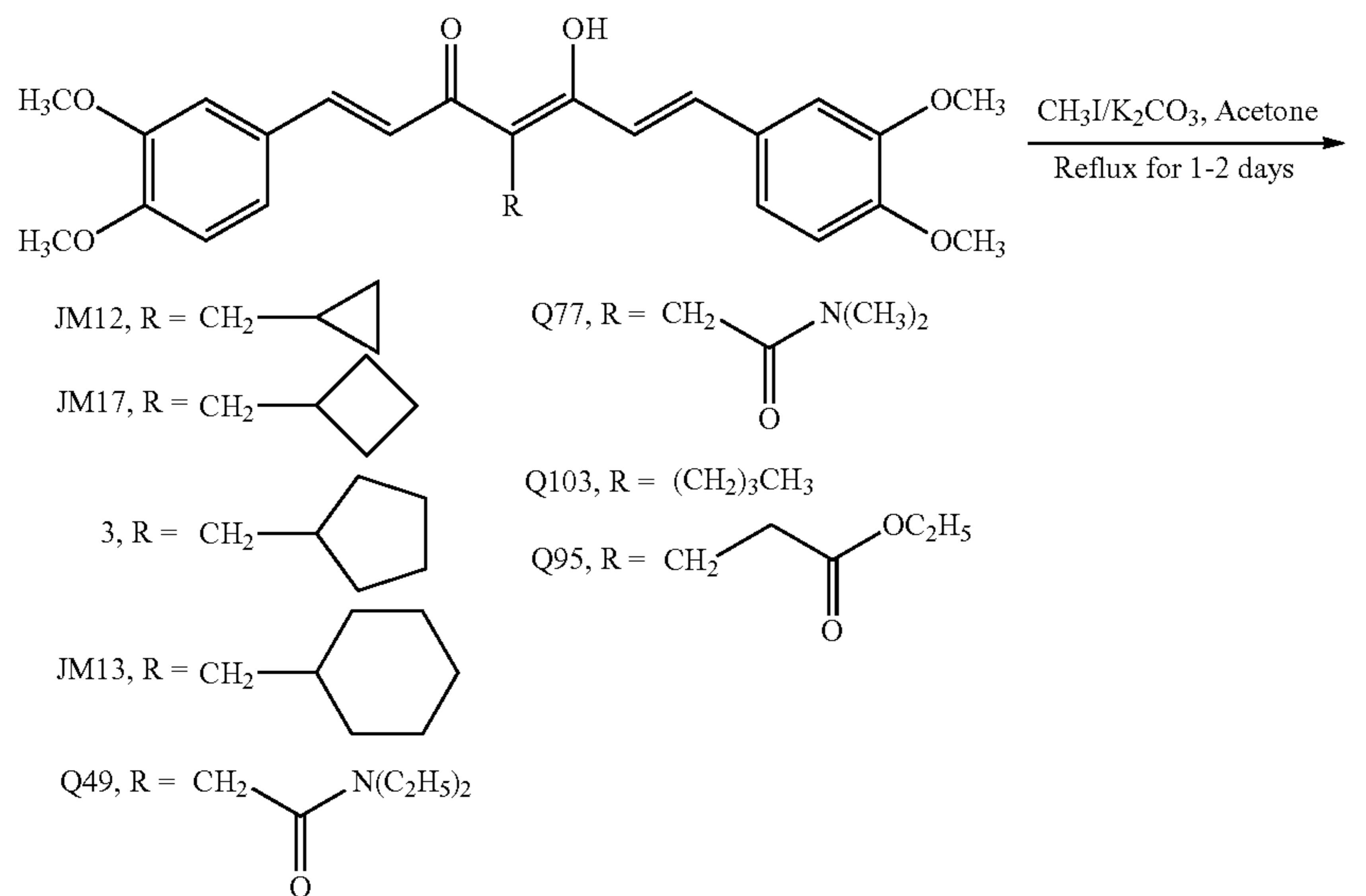
Scheme 14
