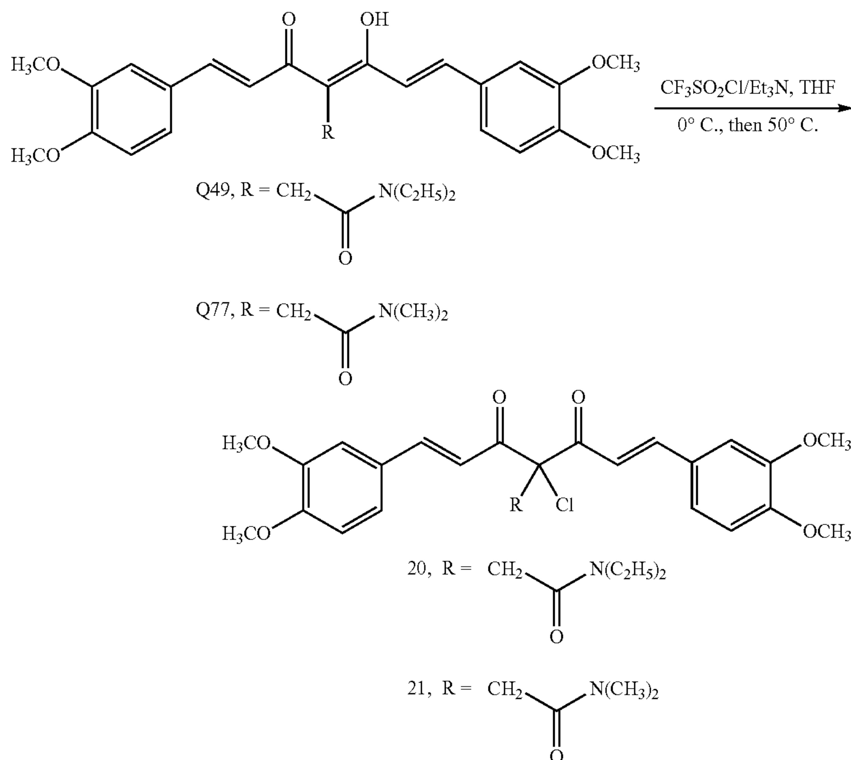
Scheme 17
