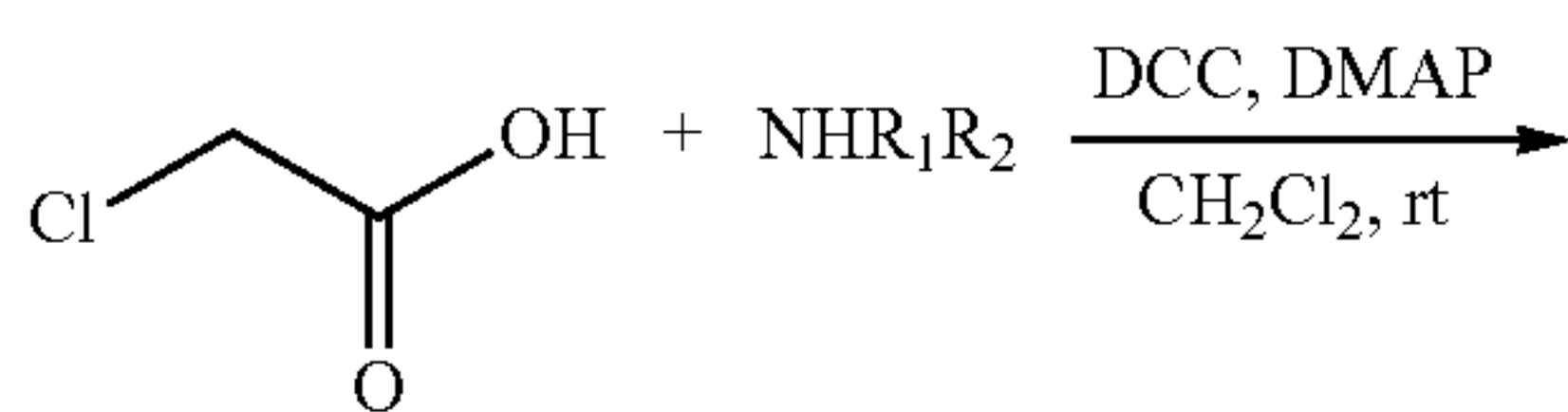
Scheme 15
