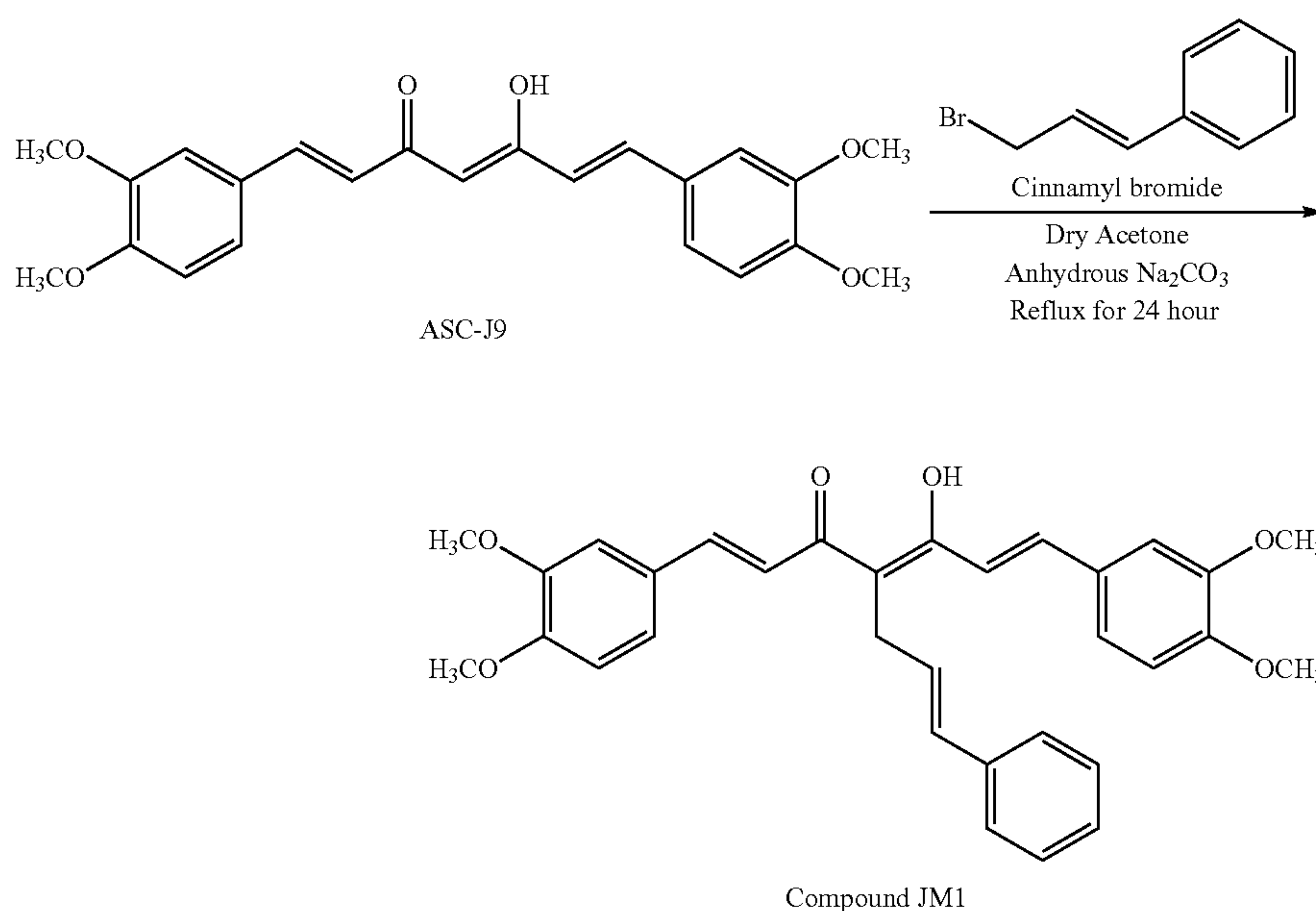
Scheme 9
