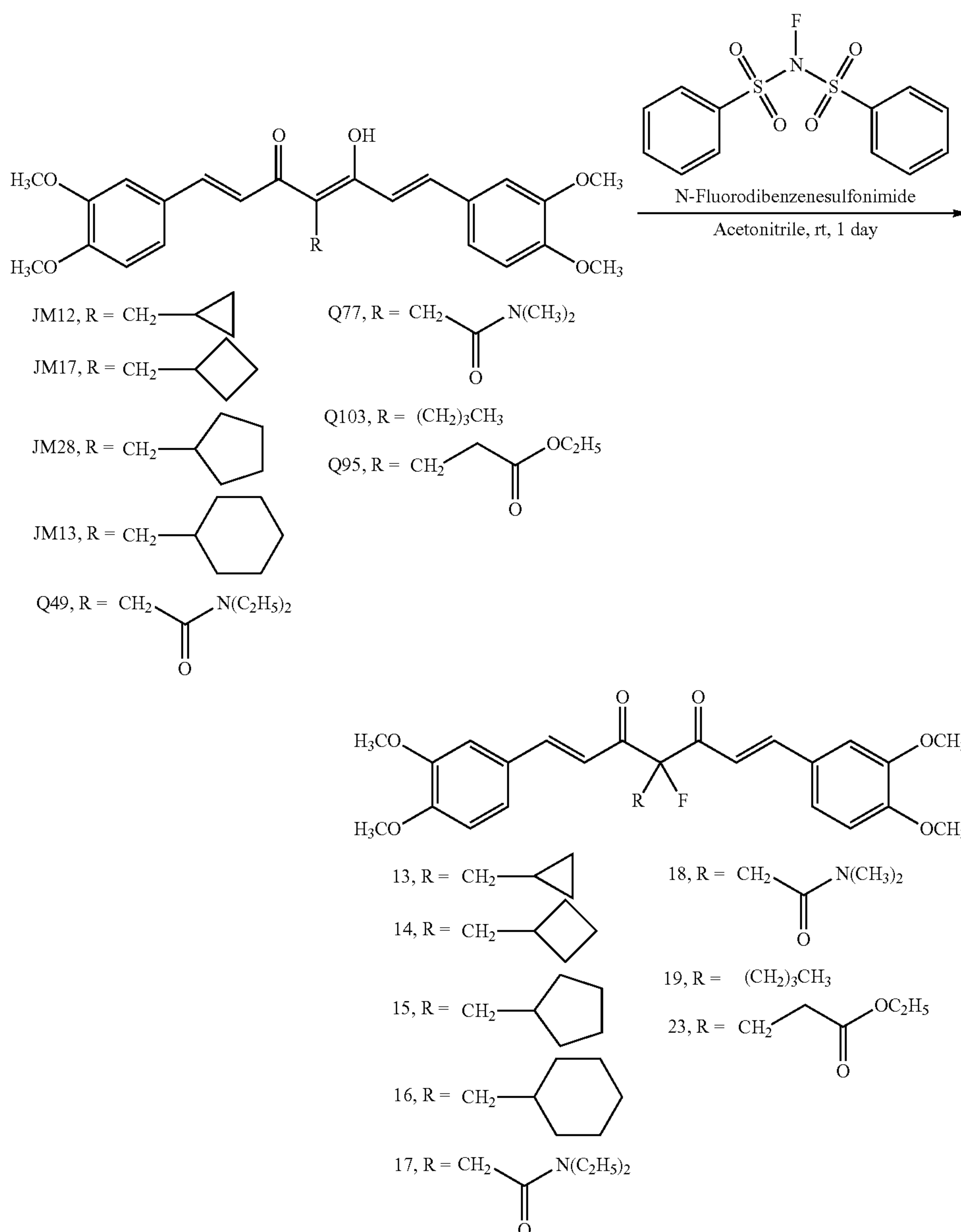
Scheme 16
