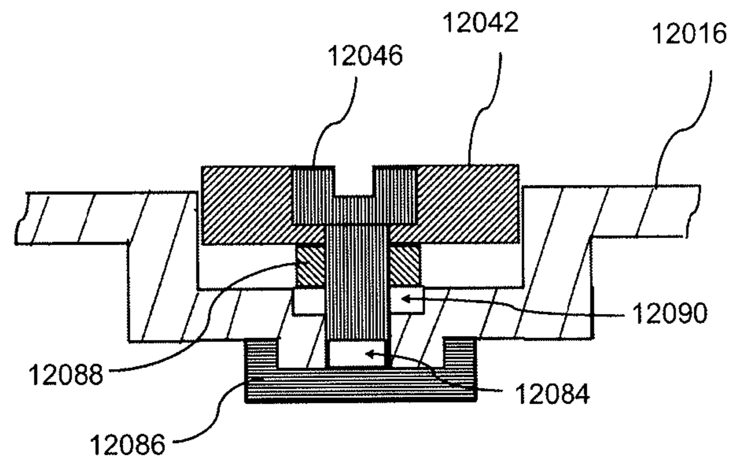
SECTION A
