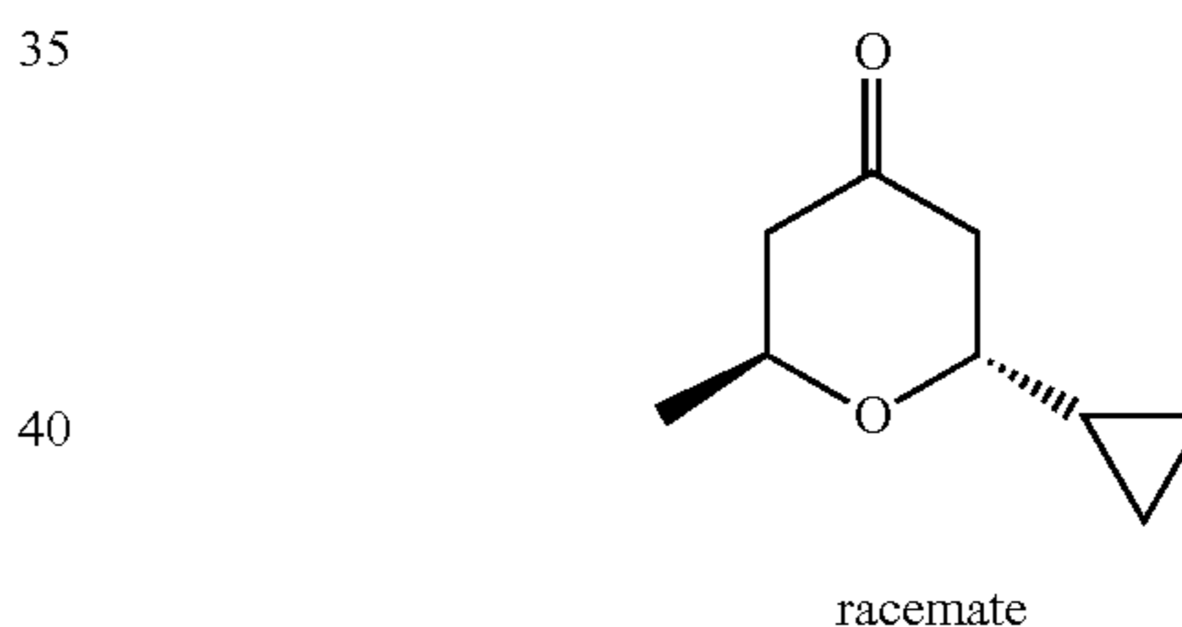
Cap 15, step a
