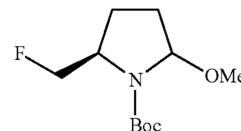
Example 8, Step d
