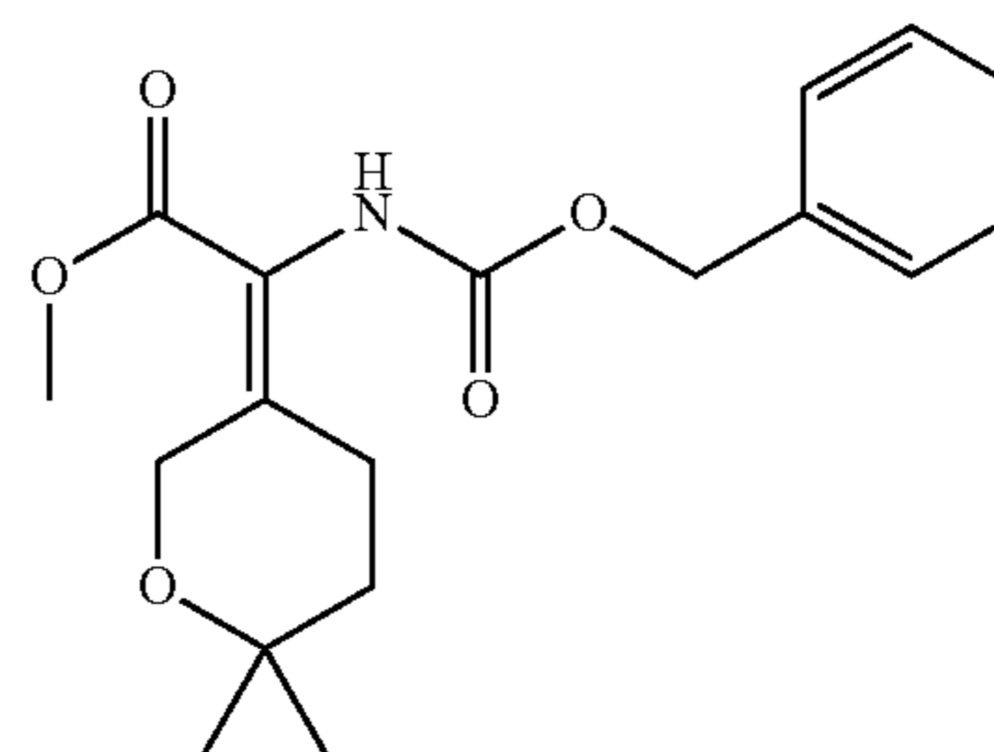
Cap 8, step h
