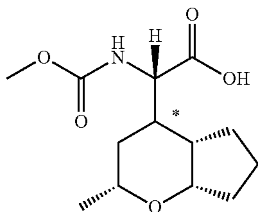
Cap 17:1 Diastereomer-1
