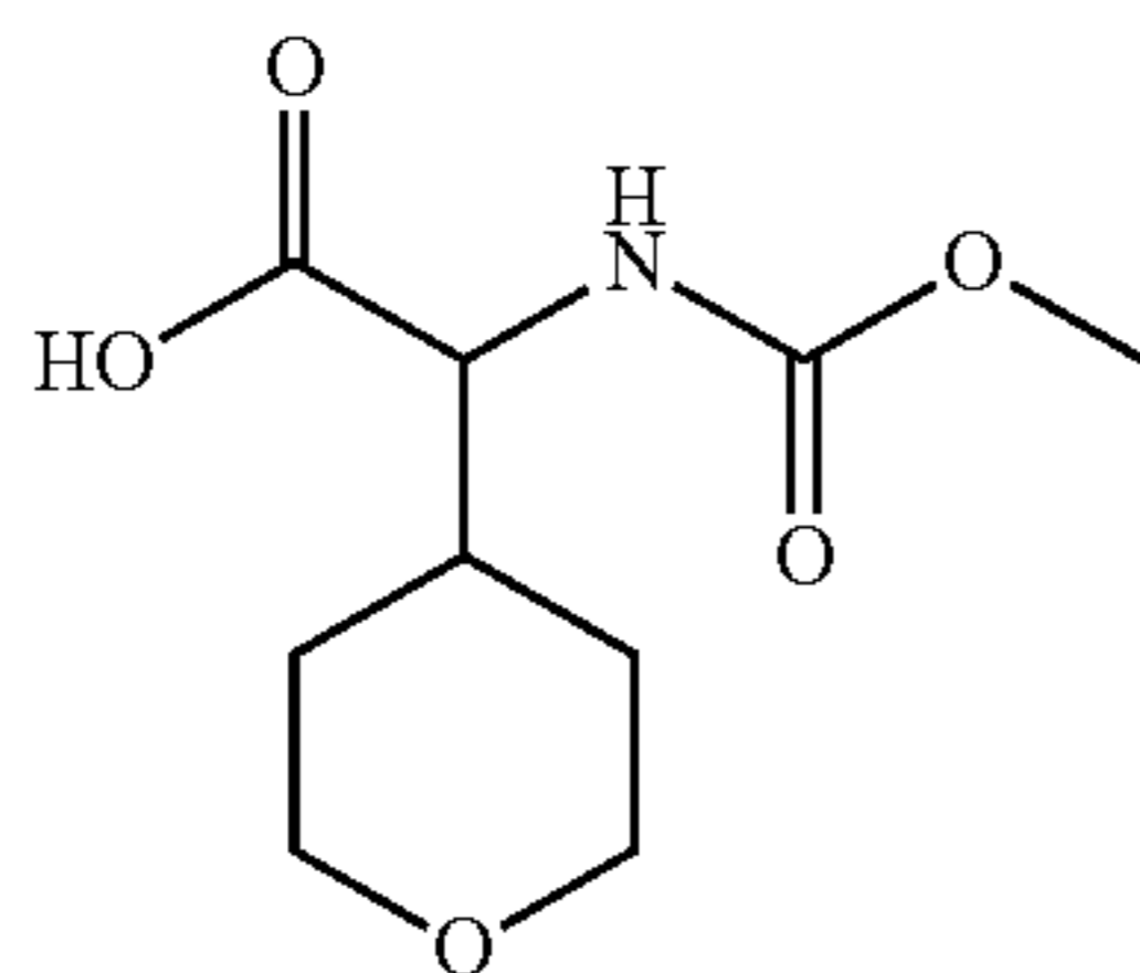
Cap 14, step a
