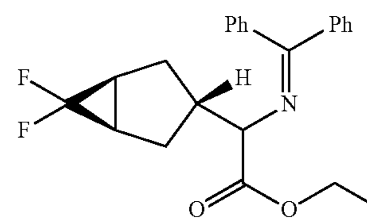
Racemic mixture
