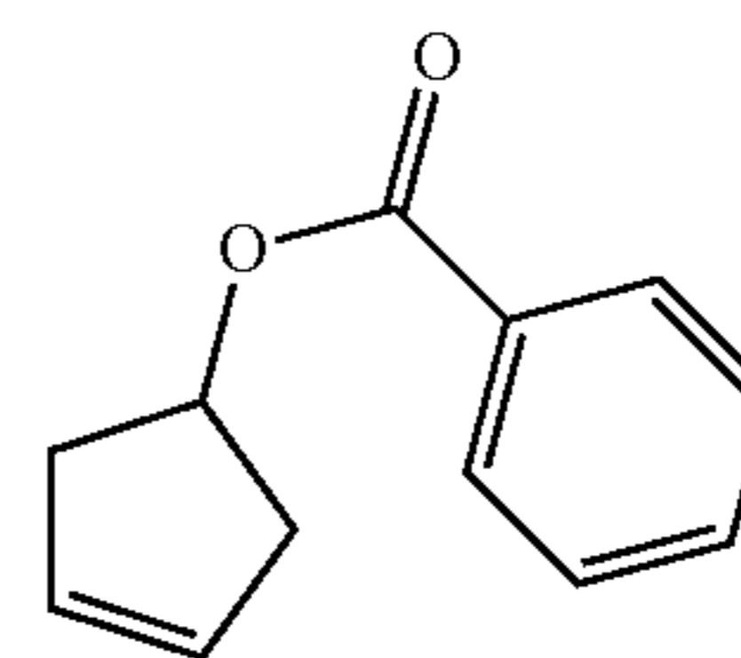
Cap-2 step a
