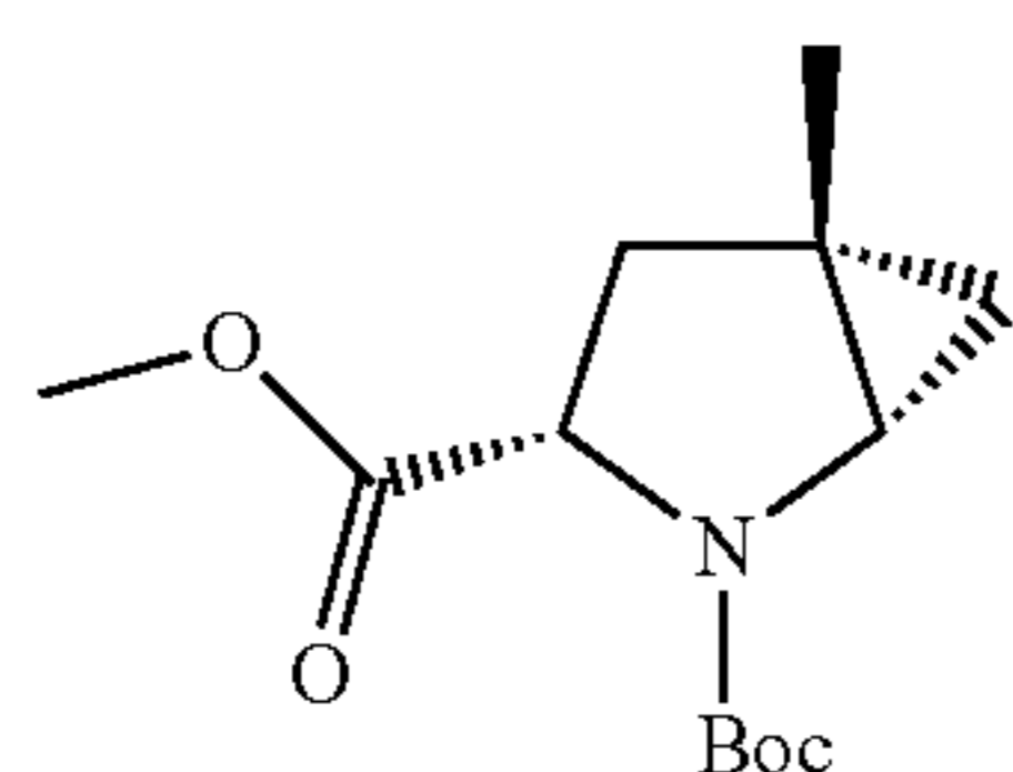
Example QC-19, step c.1
