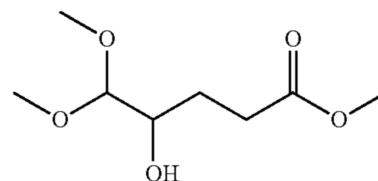
Cap-8, step b
