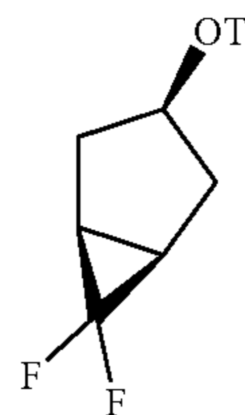
Cap-2 step d
