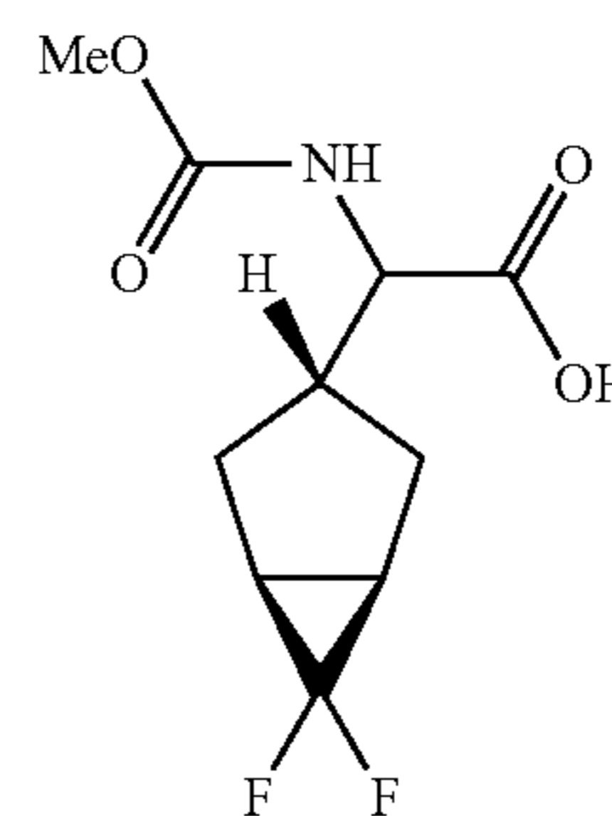
Racemic mixture
