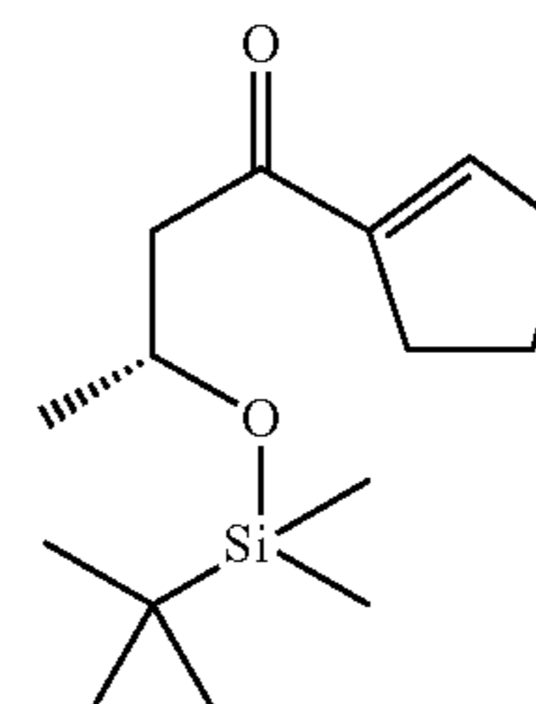
Cap 17, step b
