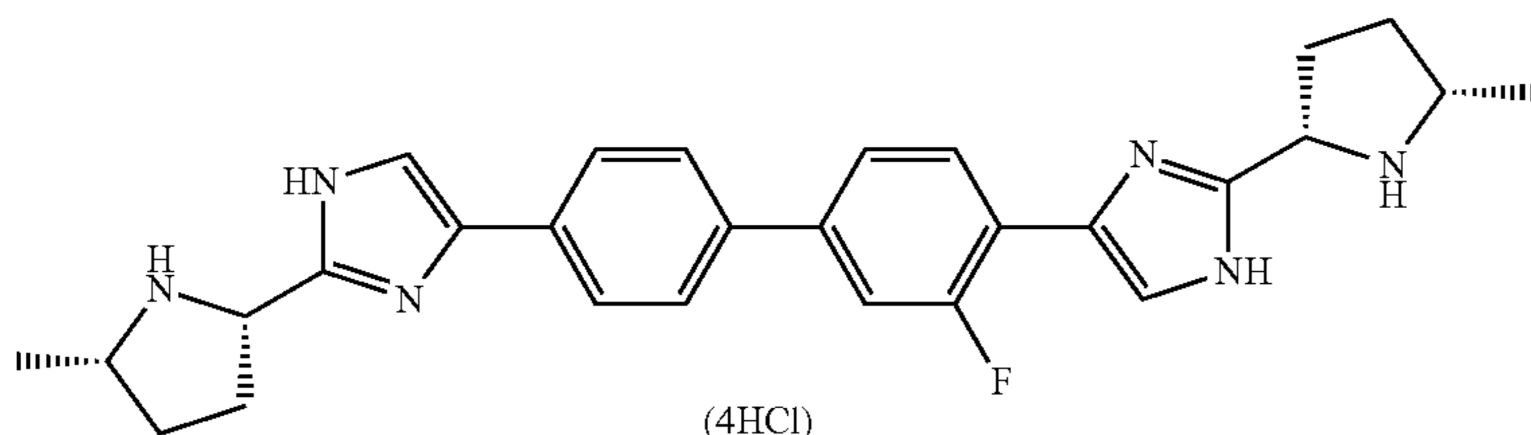
Example QC-18.1, step h
