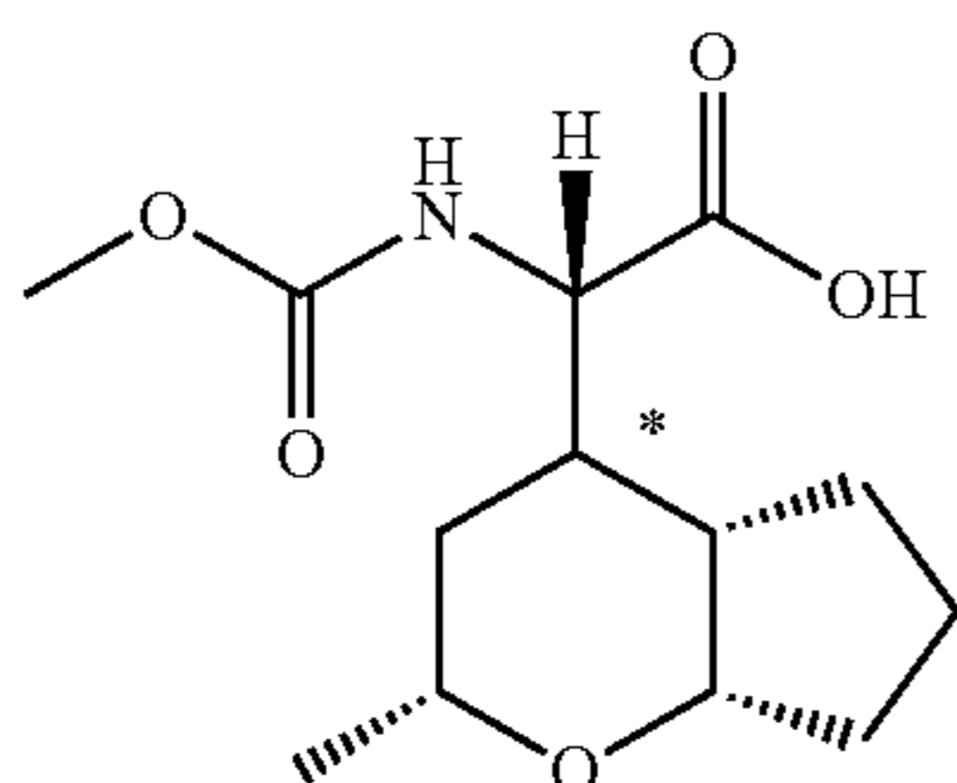
Cap 17:1 Diastereomer-2
