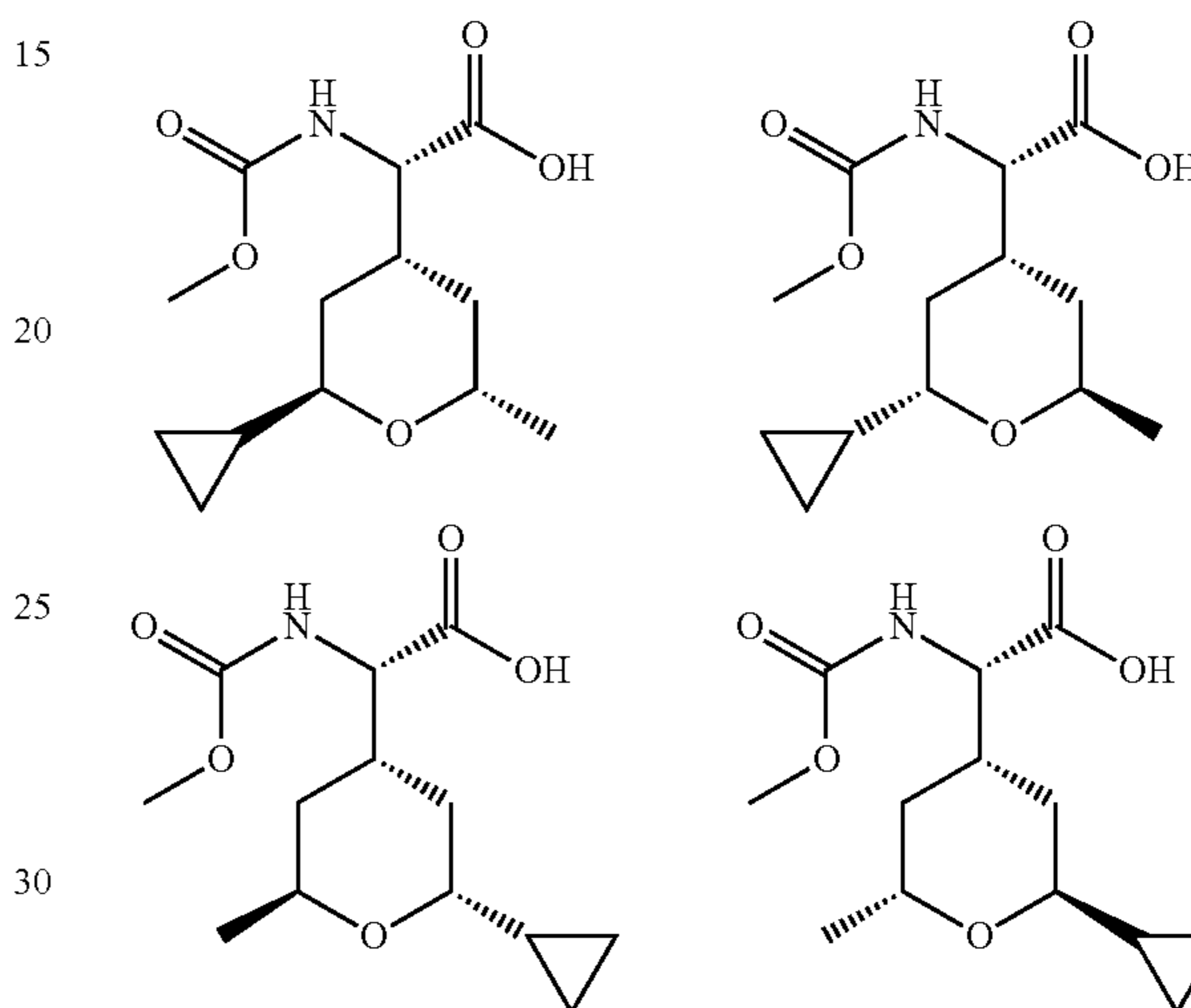
Cap 15, step a
