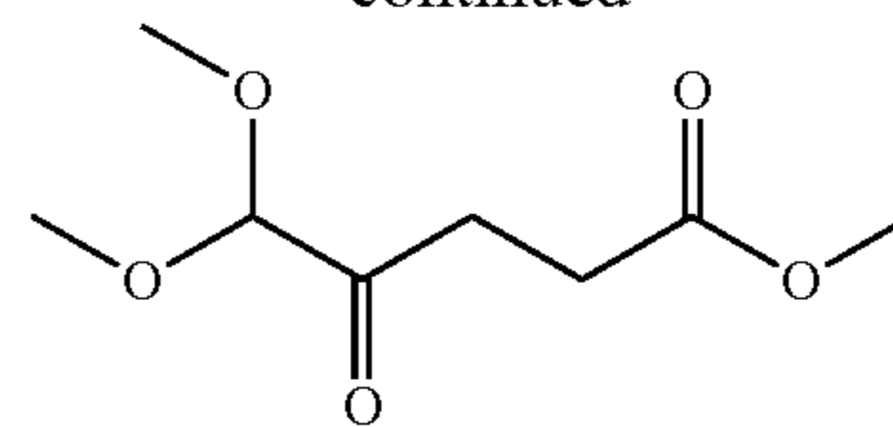
Cap 8, step a
