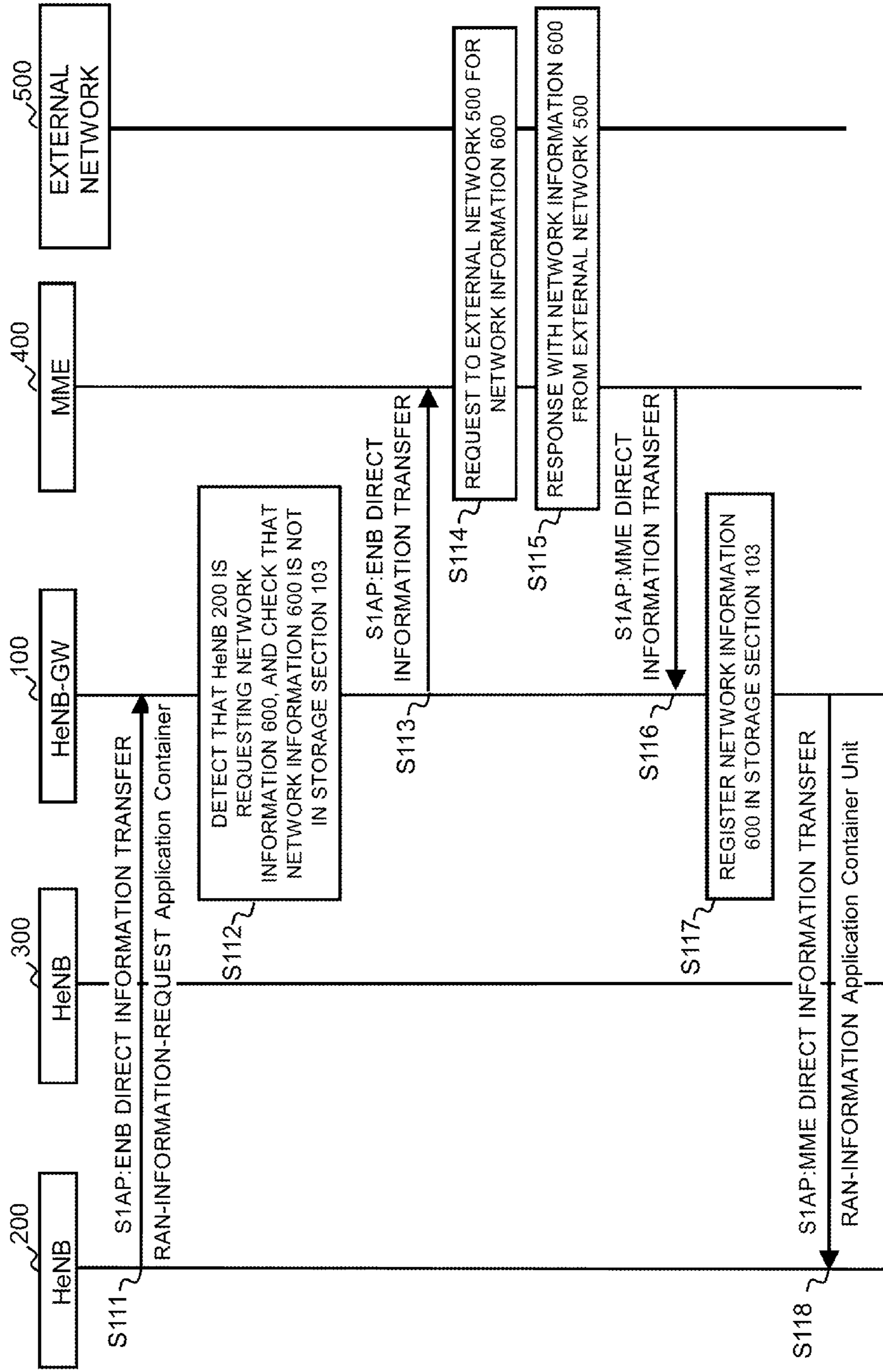
FIG. 11 THIRD EXAMPLE WHERE HeNB-GW 100 DOES NOT RETAIN NETWORK INFORMATION 600
