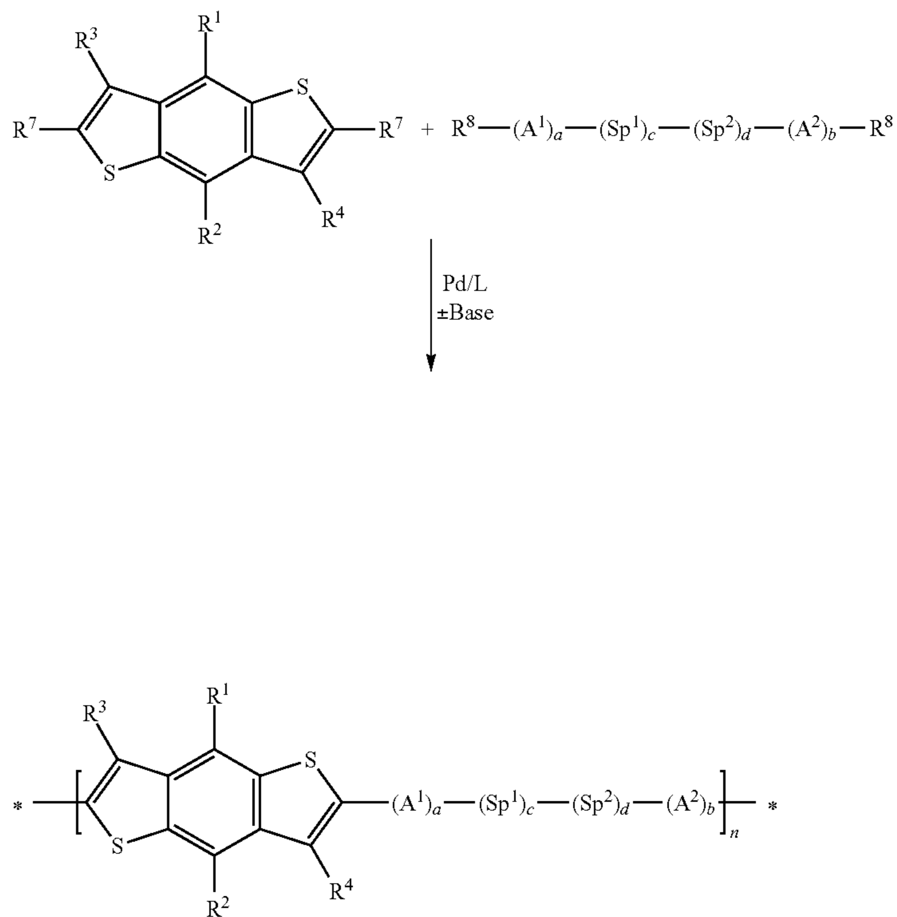
Scheme 1
