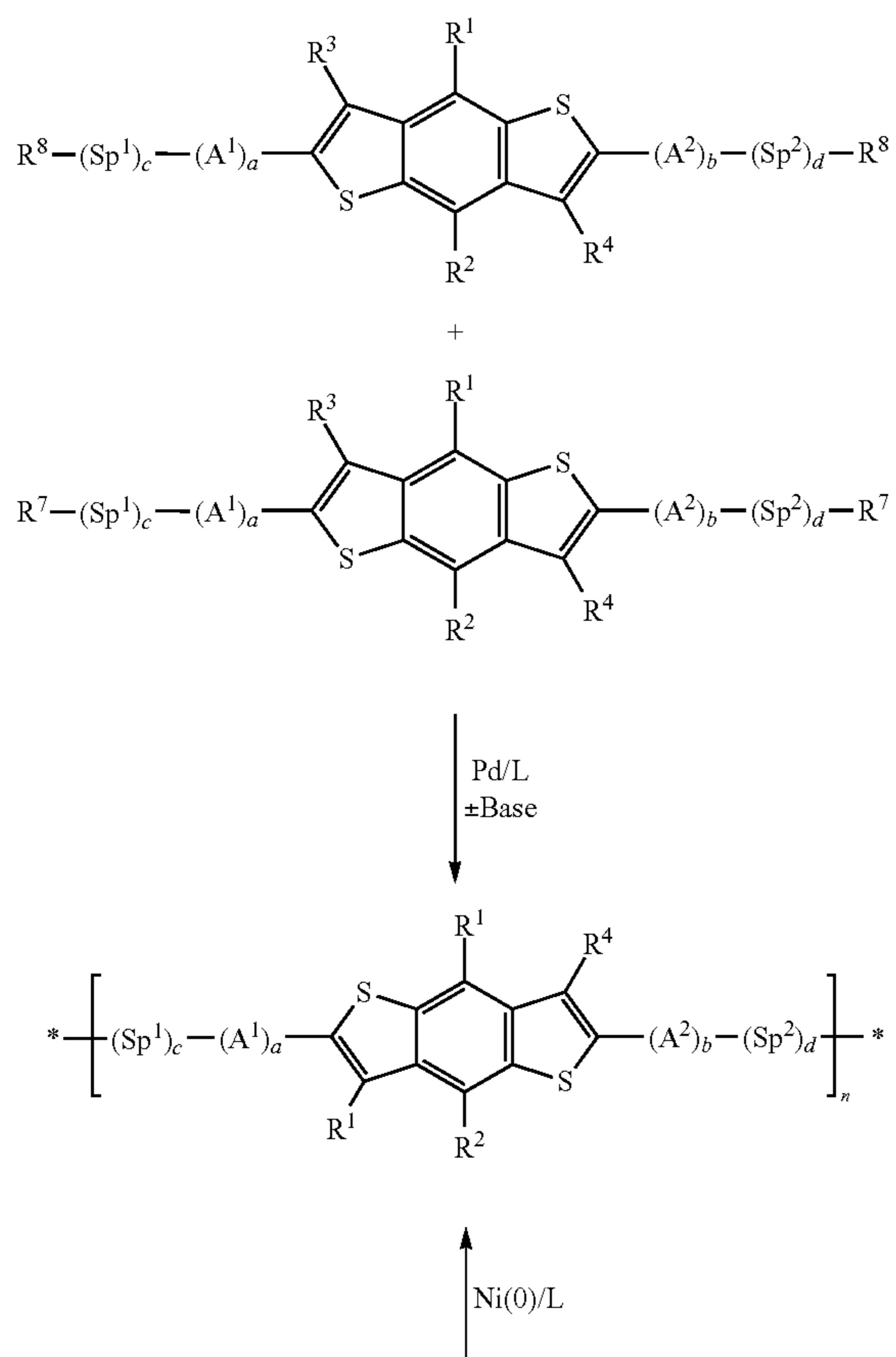
Scheme 3
