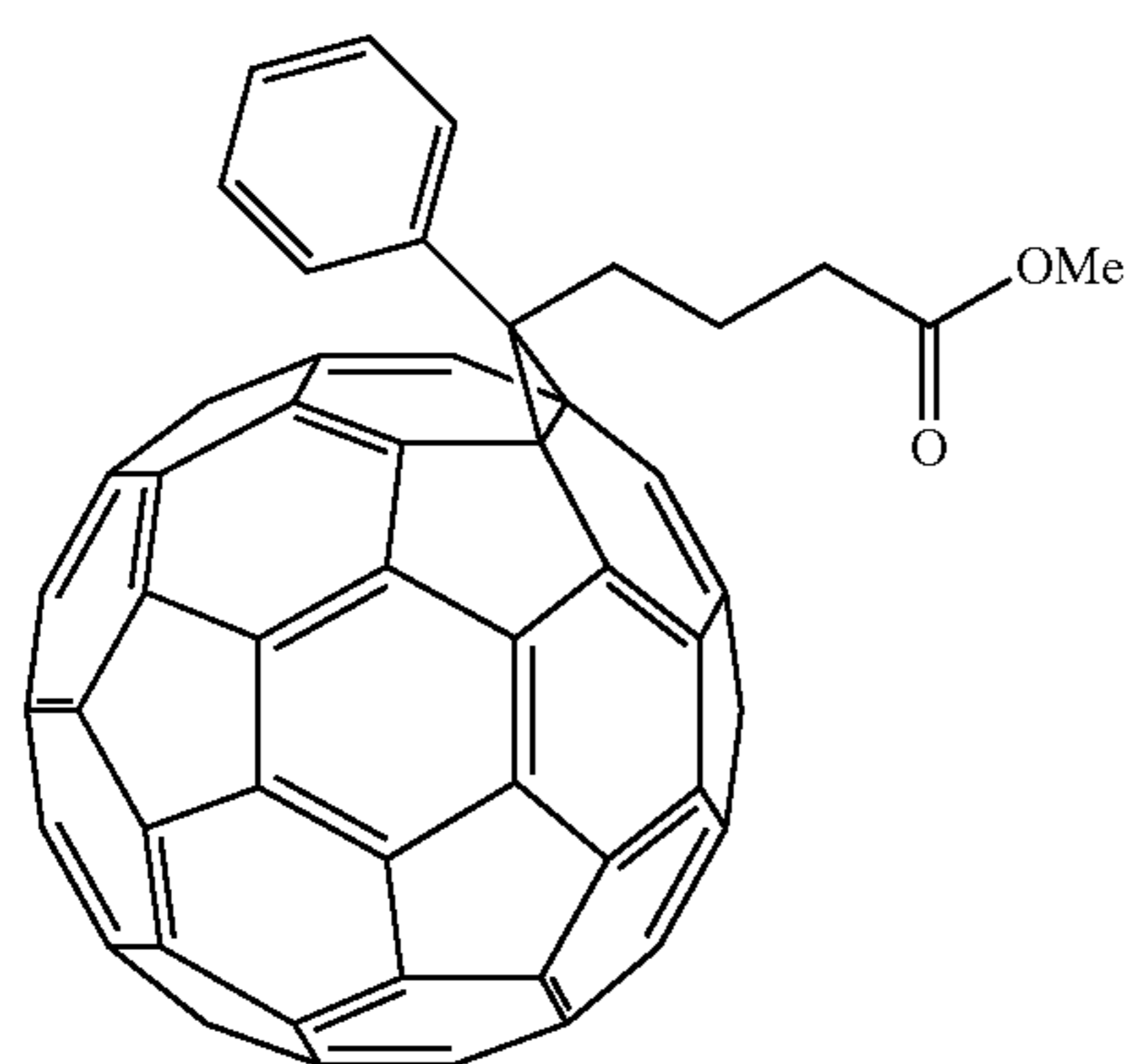
PCBM- C_{60}
