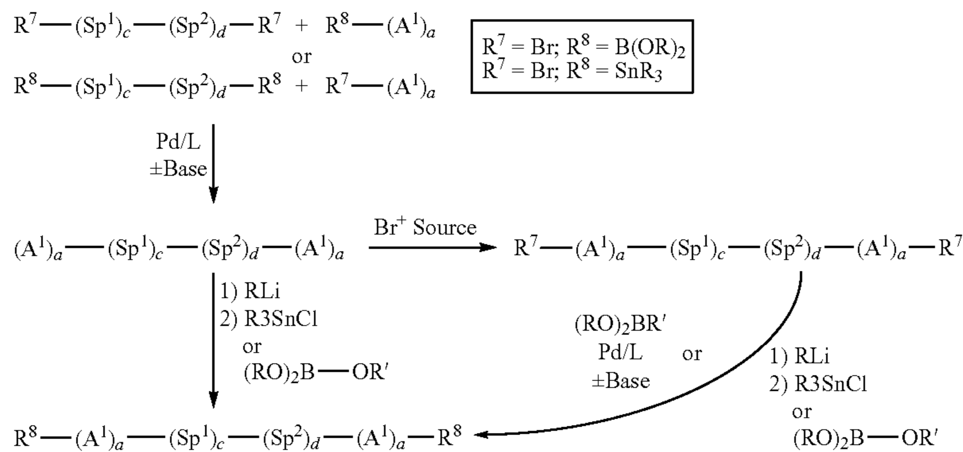
Scheme 6
