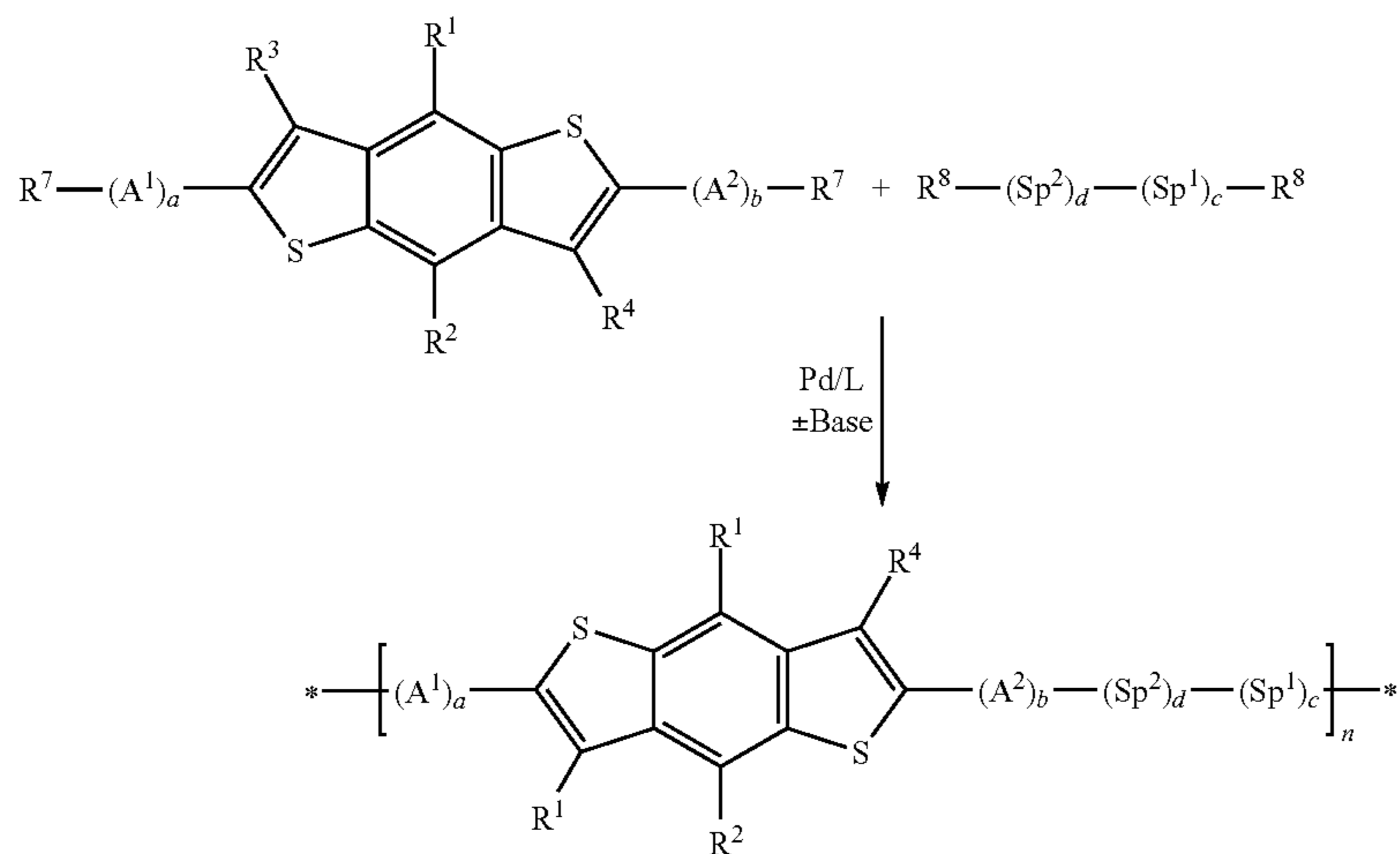
Scheme 2
