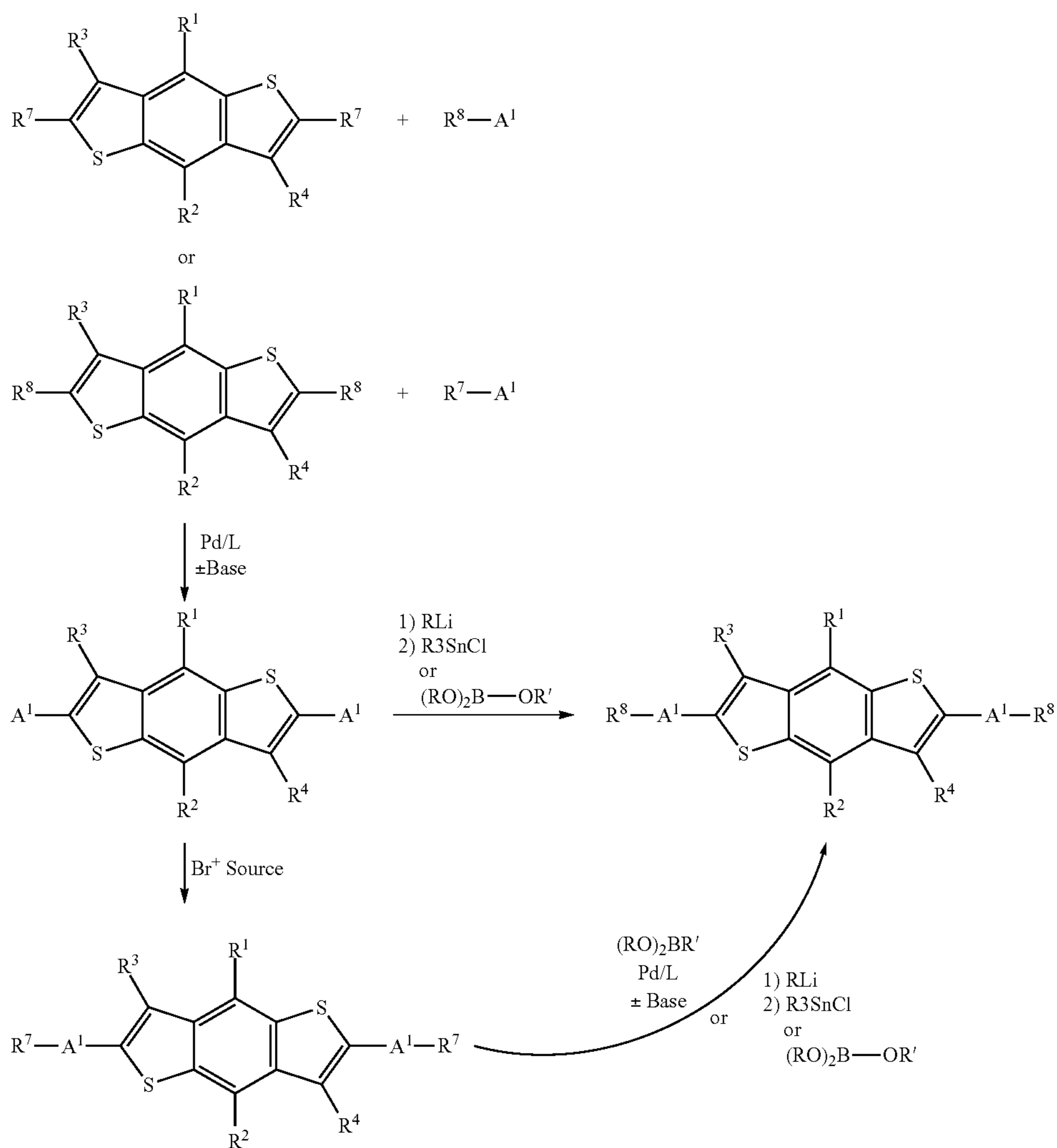
Scheme 5
