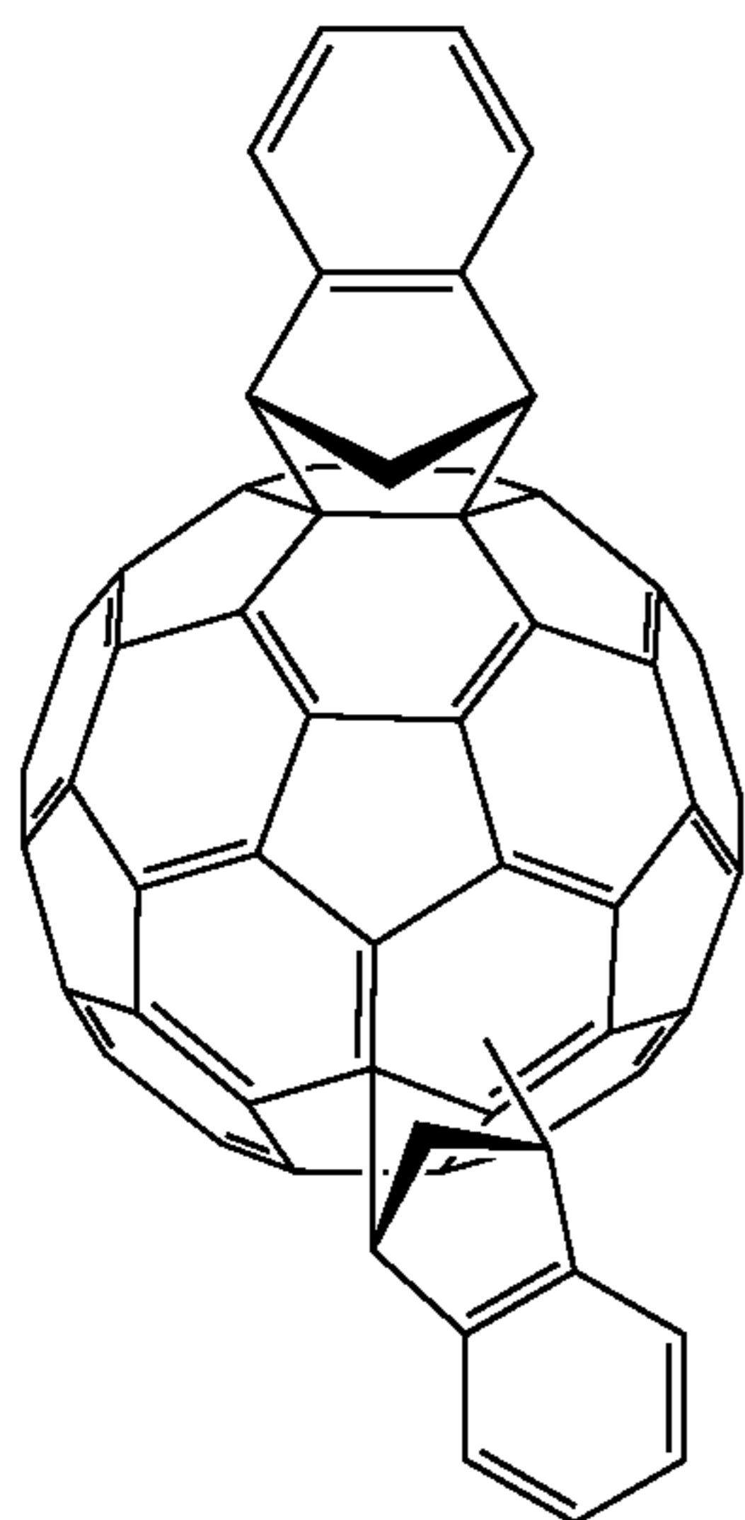
ICBA- C_{60}
