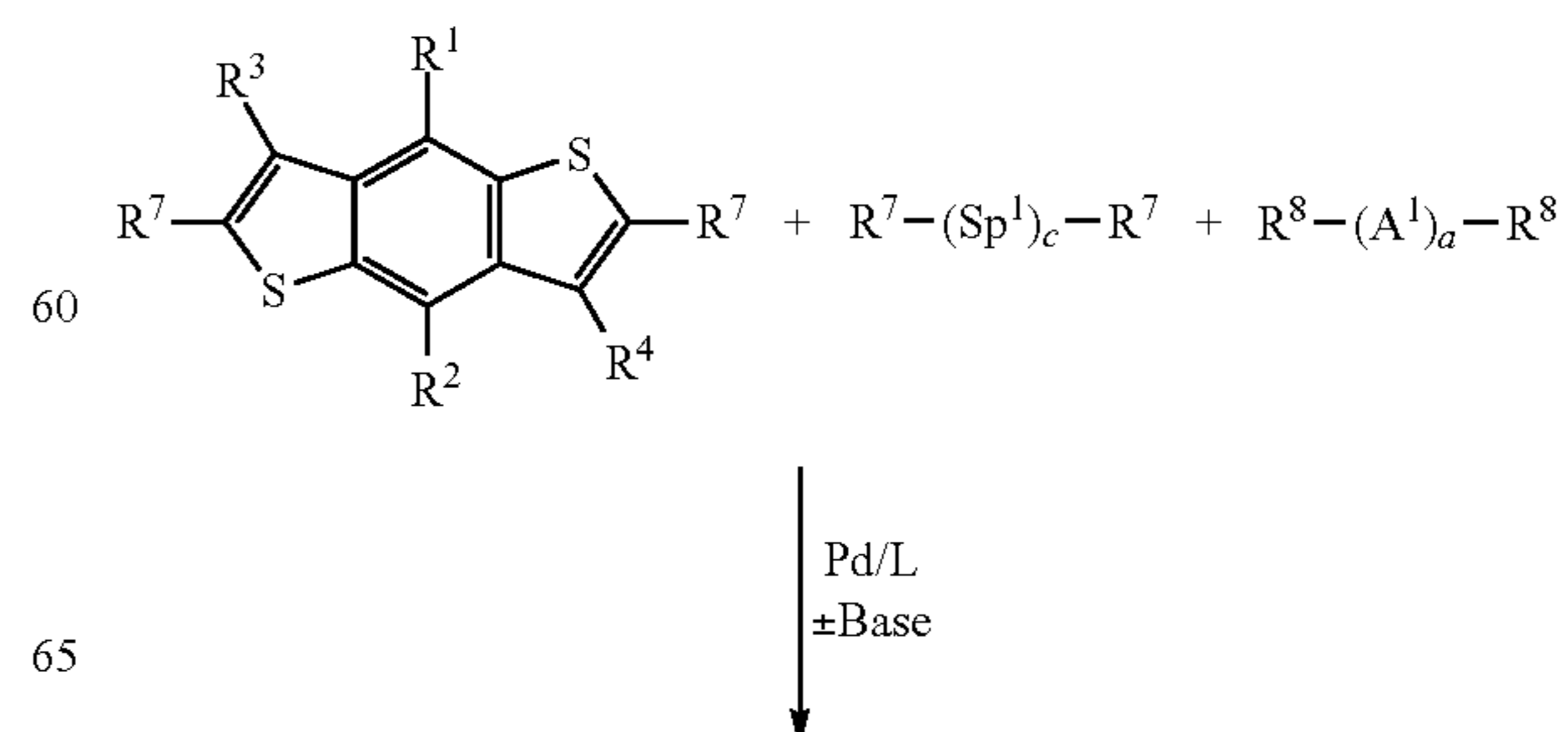
Scheme 4
