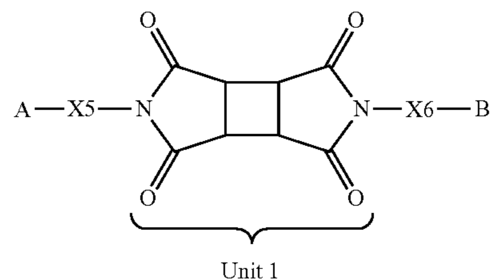
[Chemical Formula 4]
