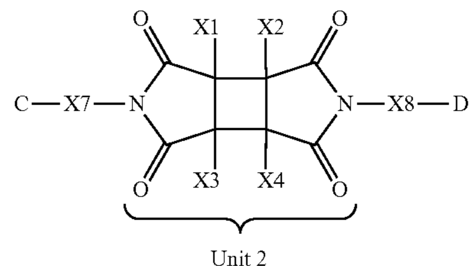
[Chemical Formula 5]
