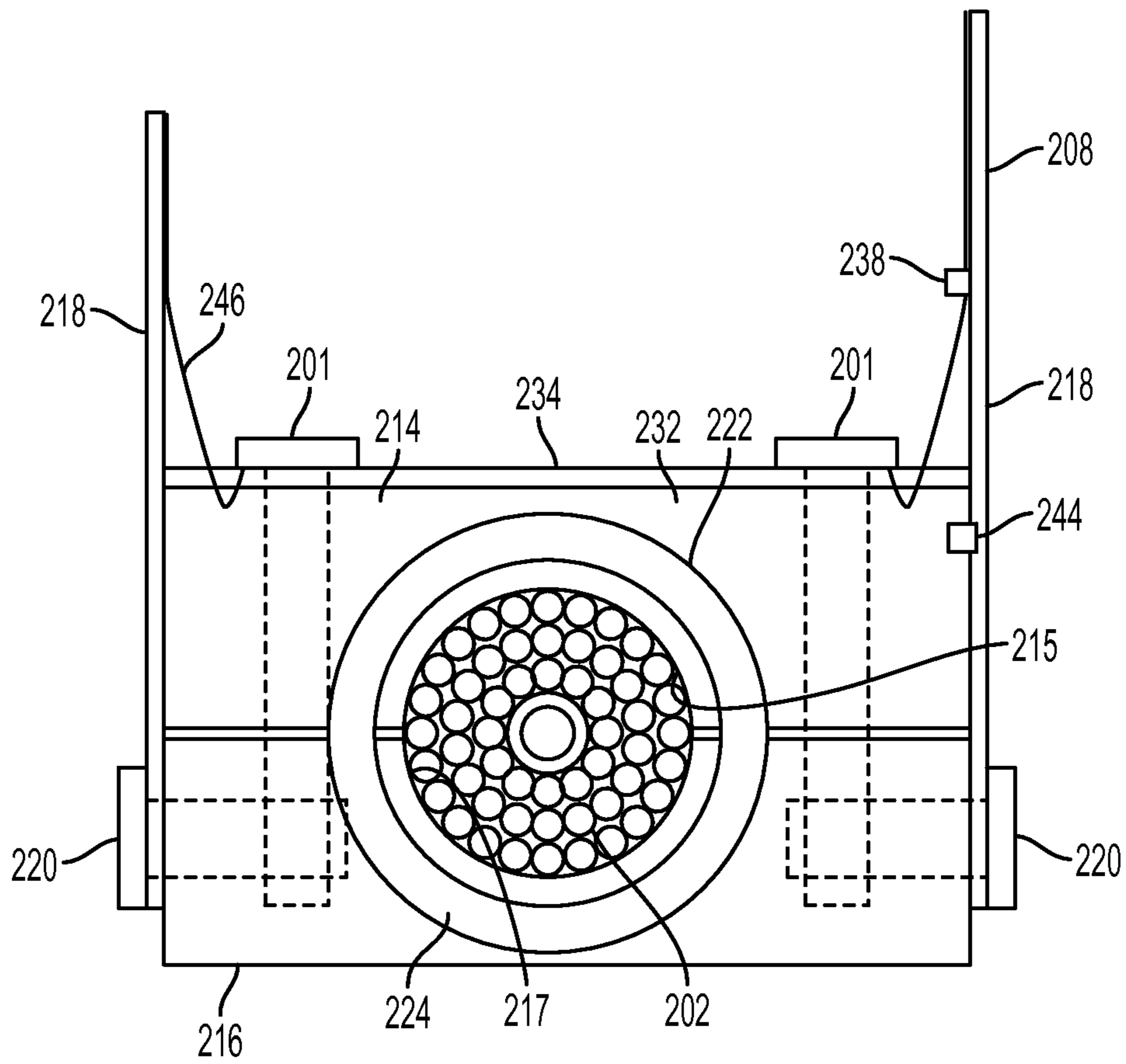
FIG. 3 RELATED ART
