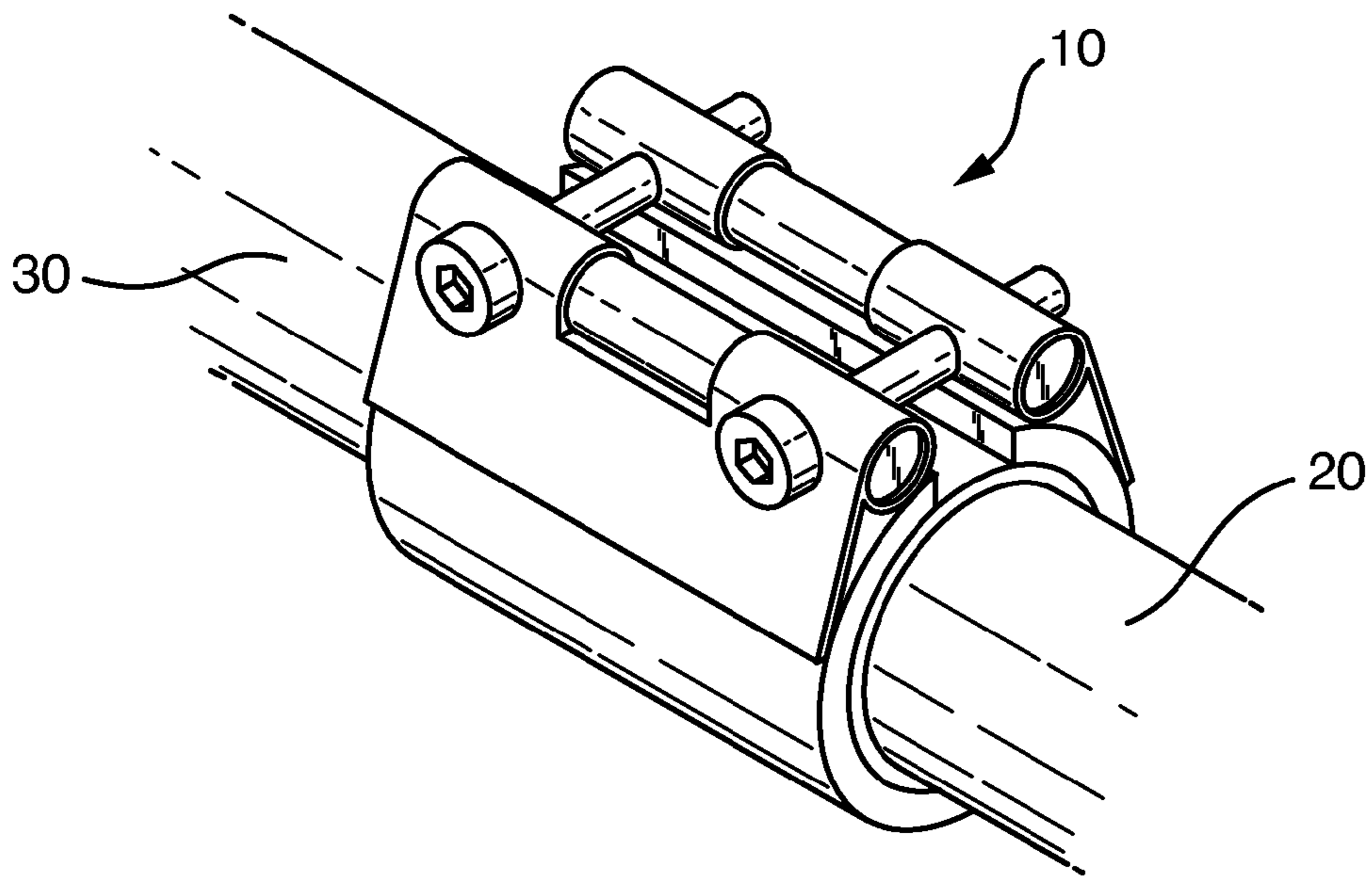
Fig. 1 PRIOR ART
