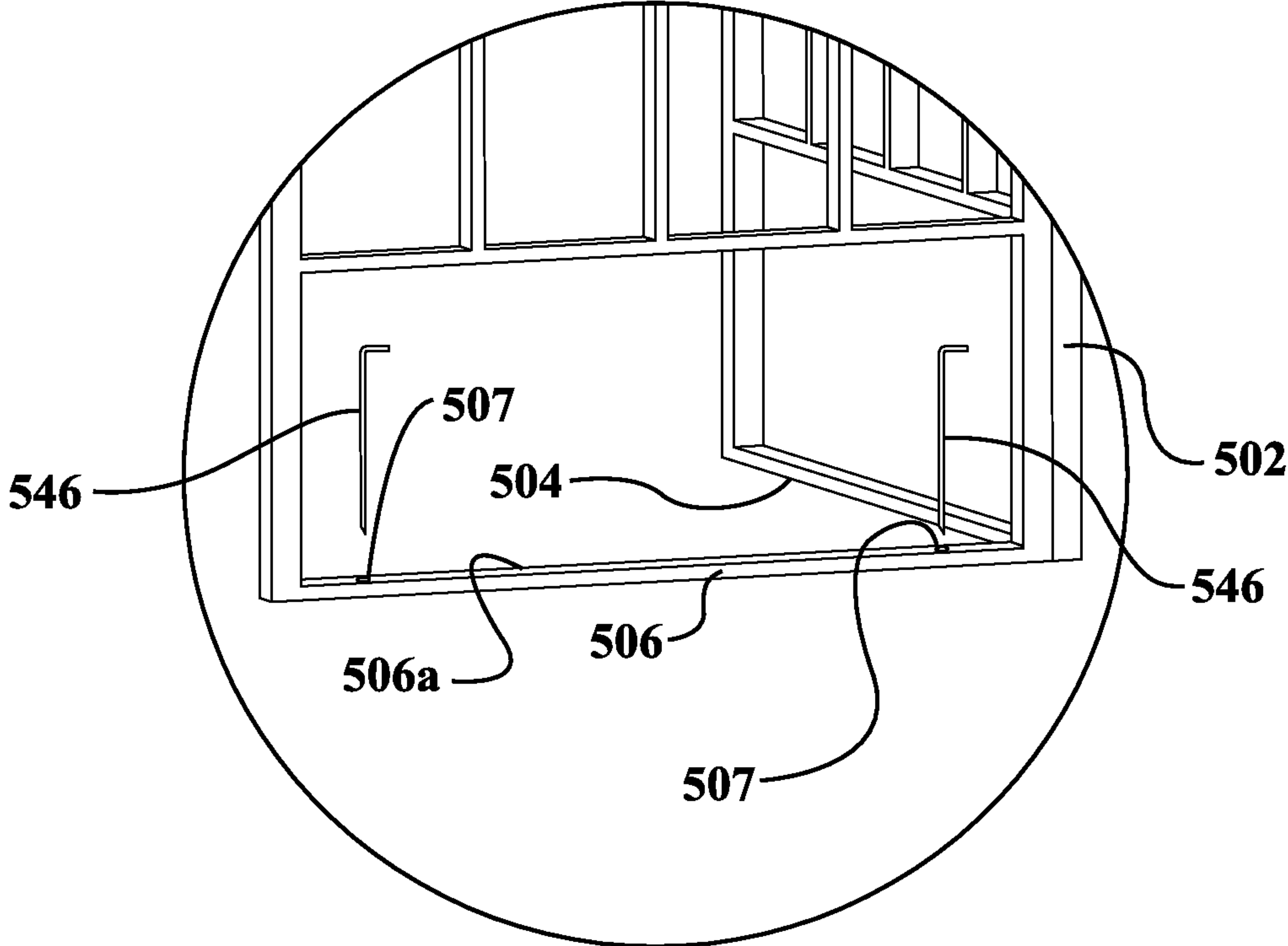
Detail "F"
