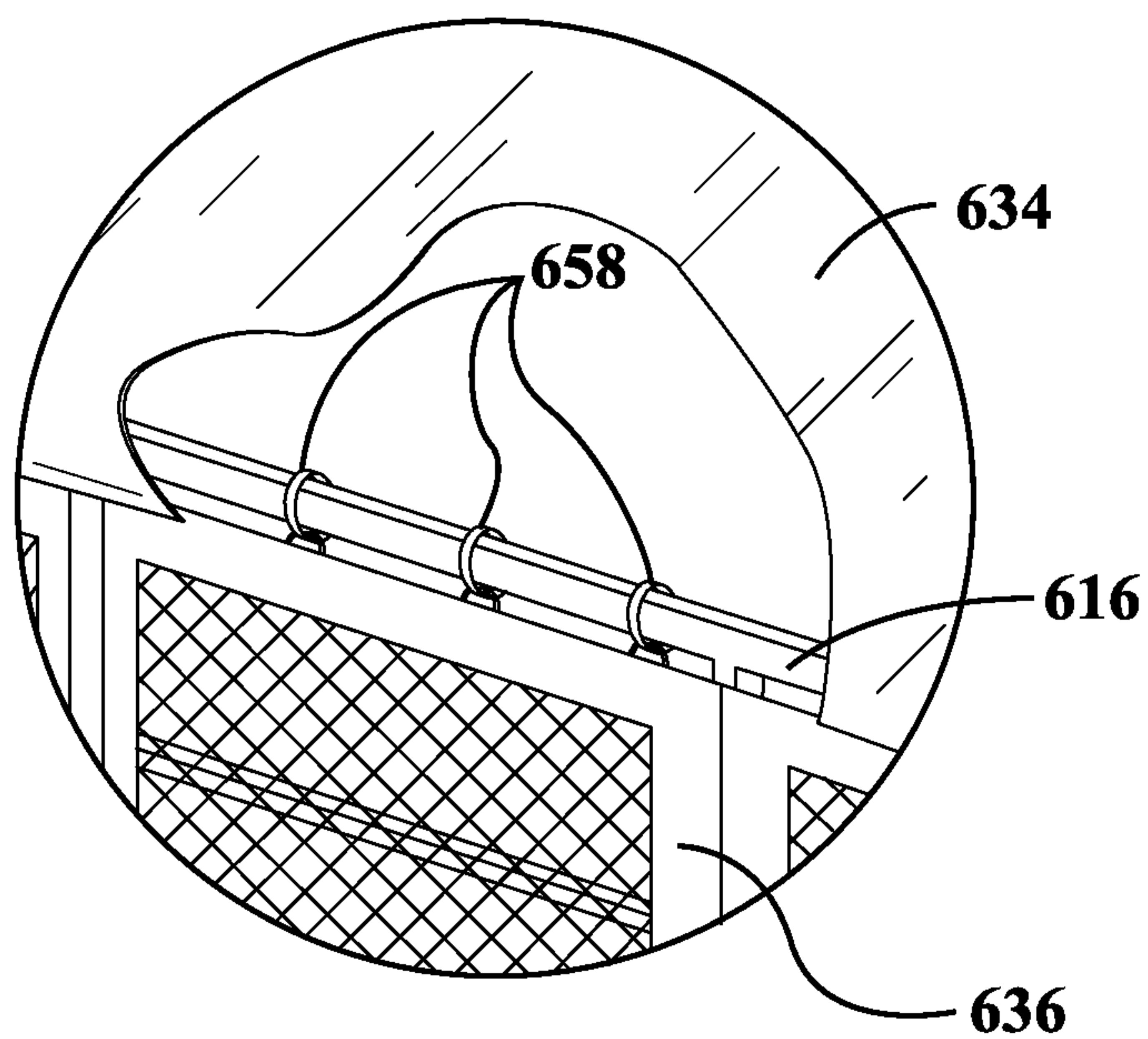
Detail "J" FIG. 46
