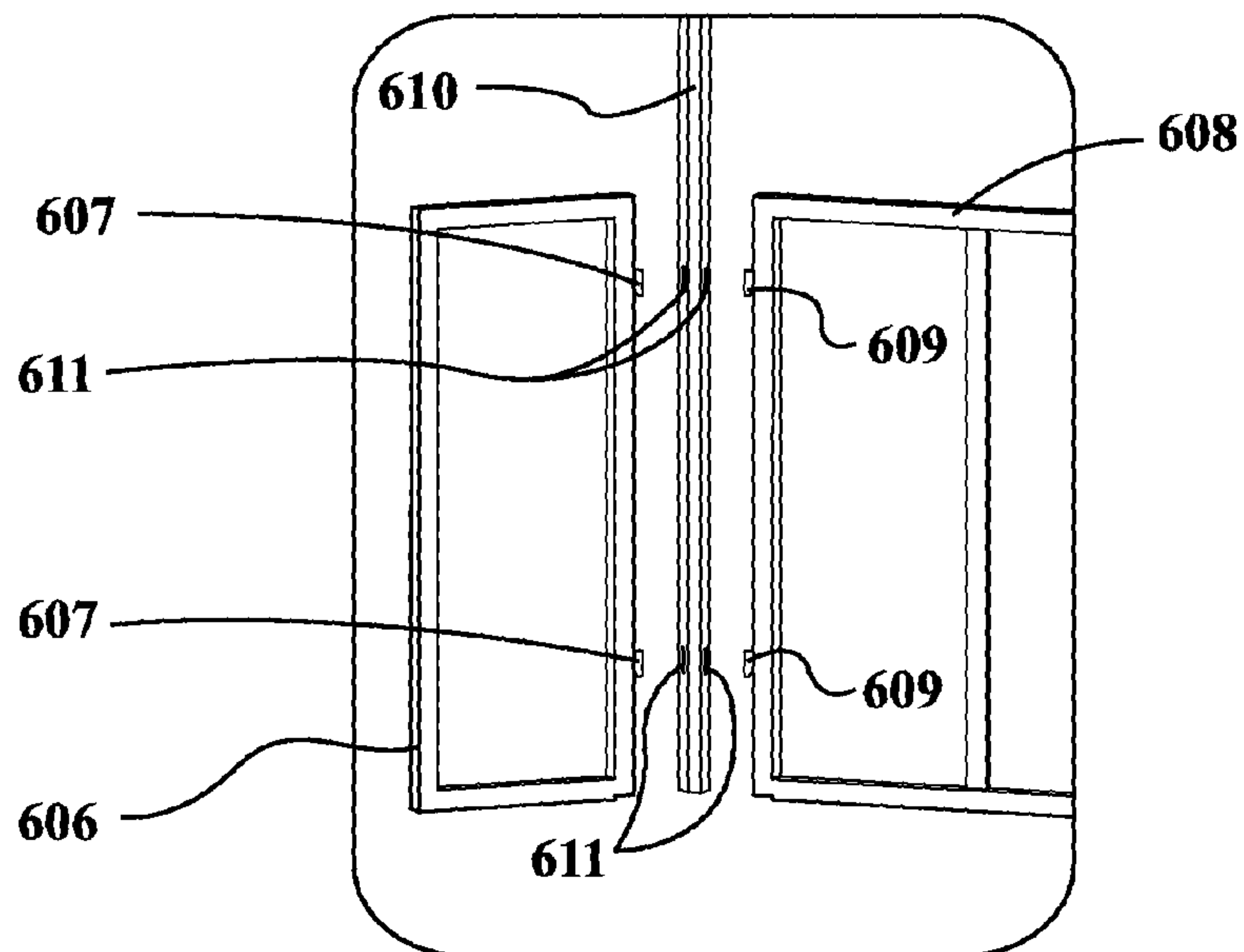
Detail "G" FIG. 43
