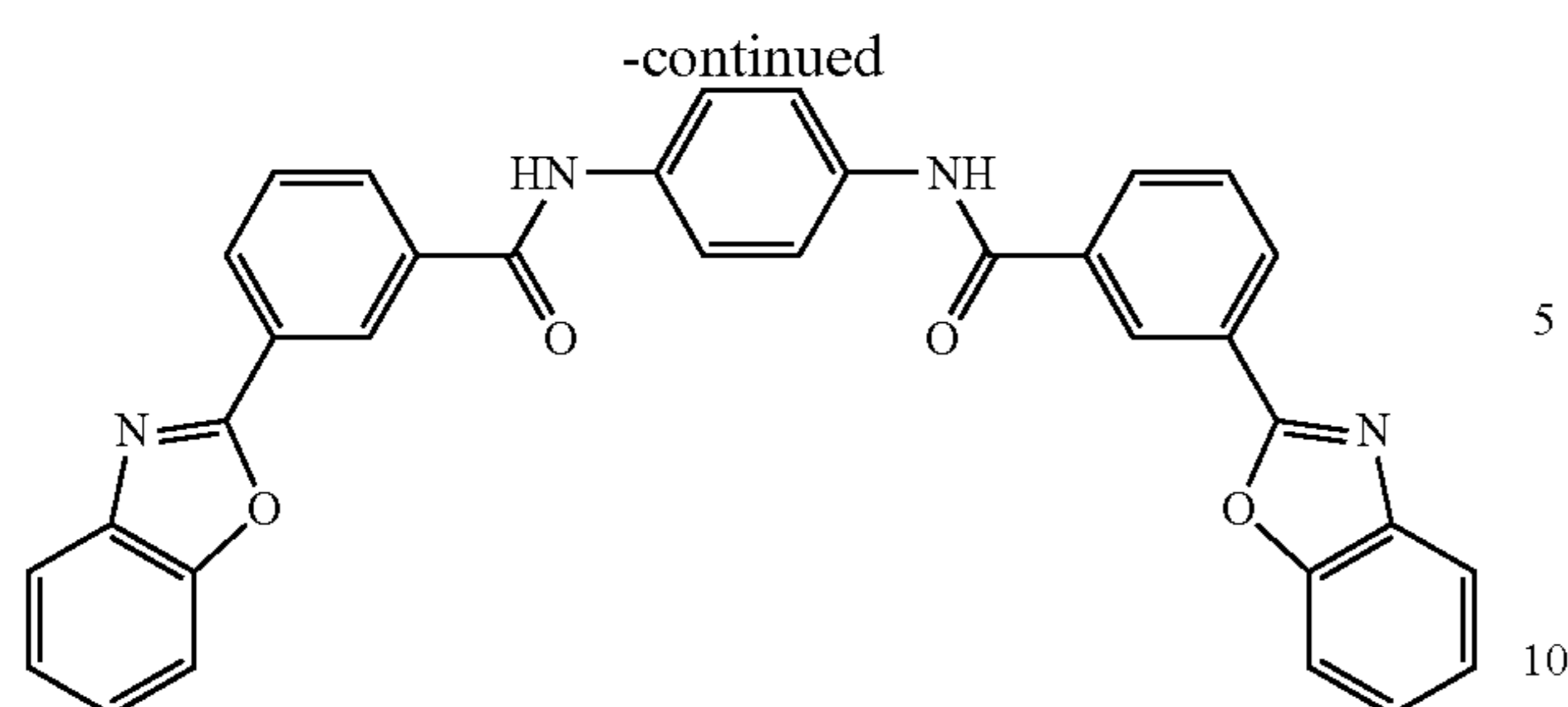
BT-5
