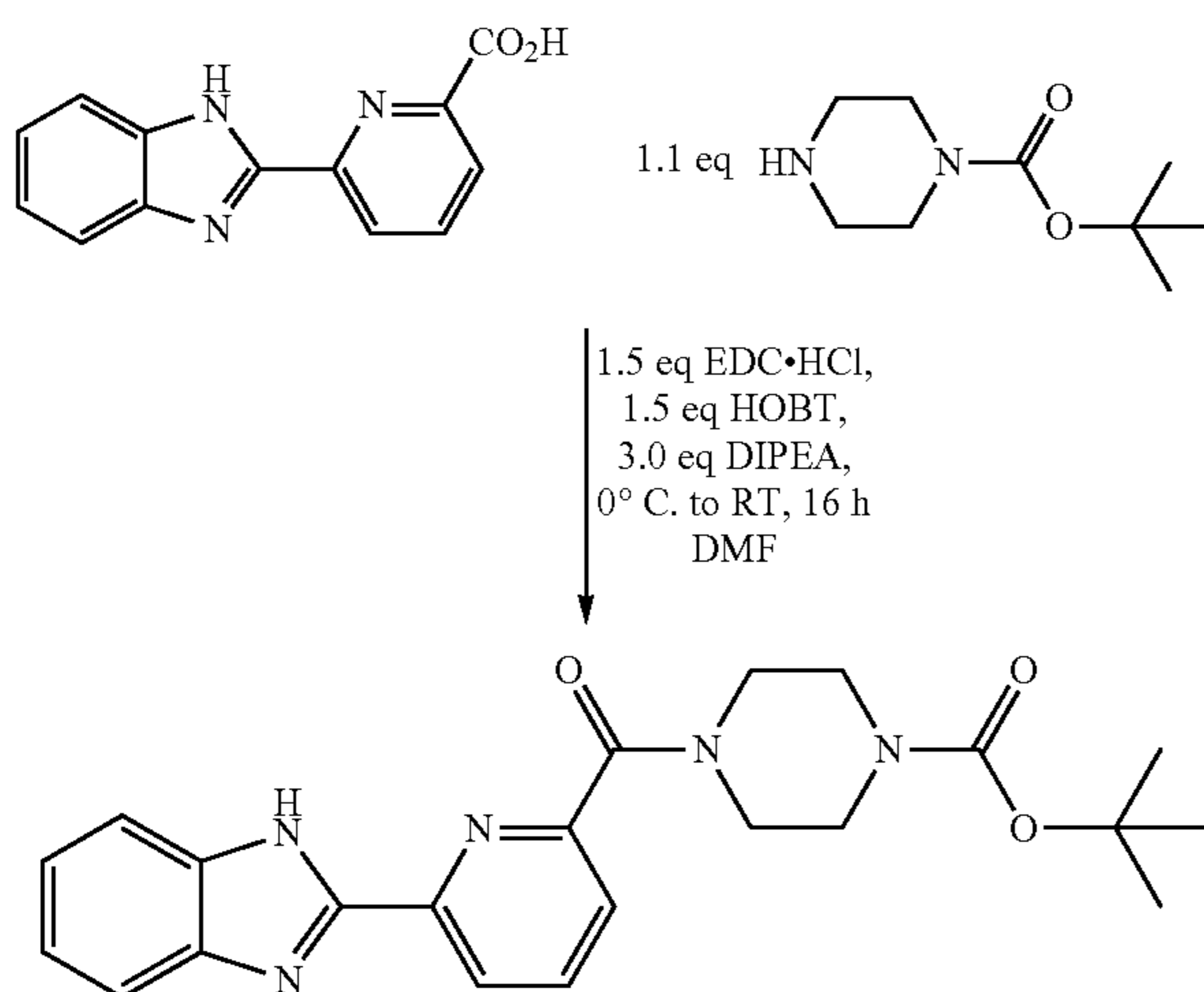
Scheme 6-1
