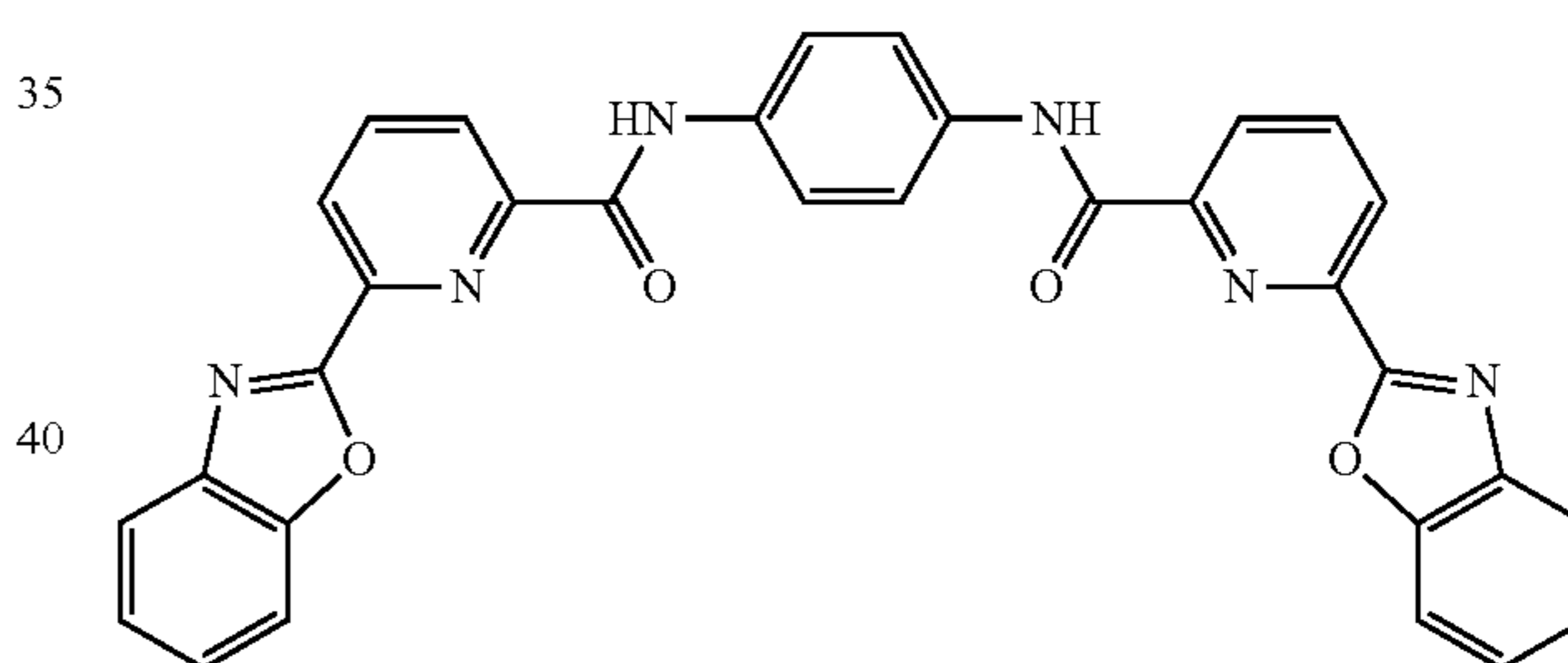
BT-17
