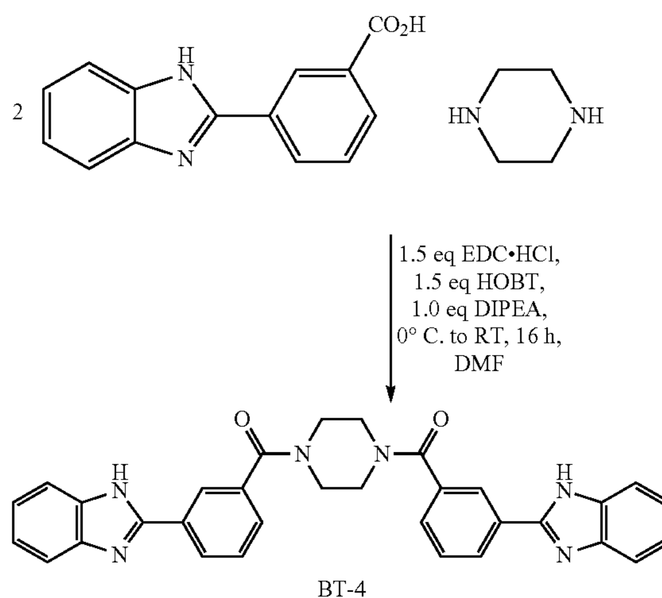
Scheme 7-1
