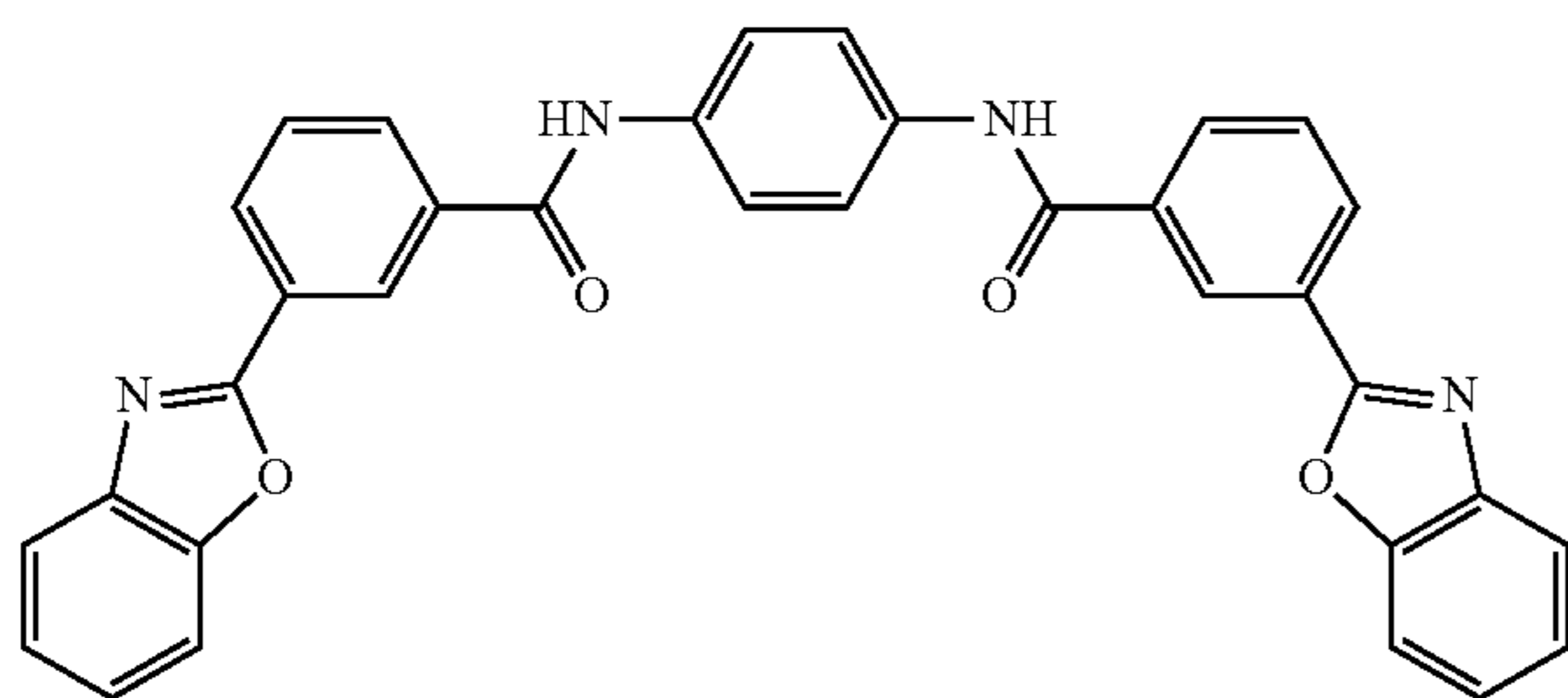
BT-5
