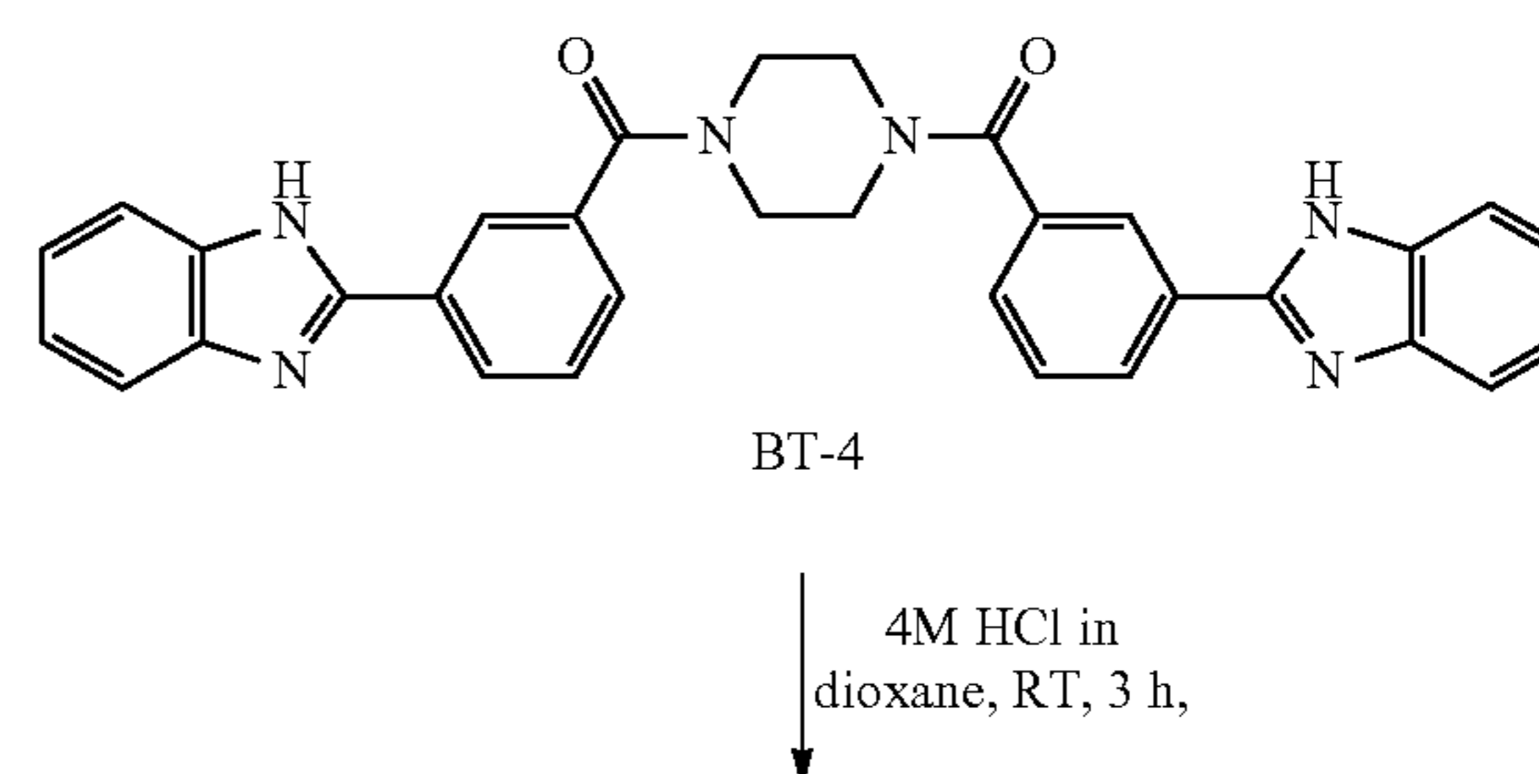
Scheme 7-2
