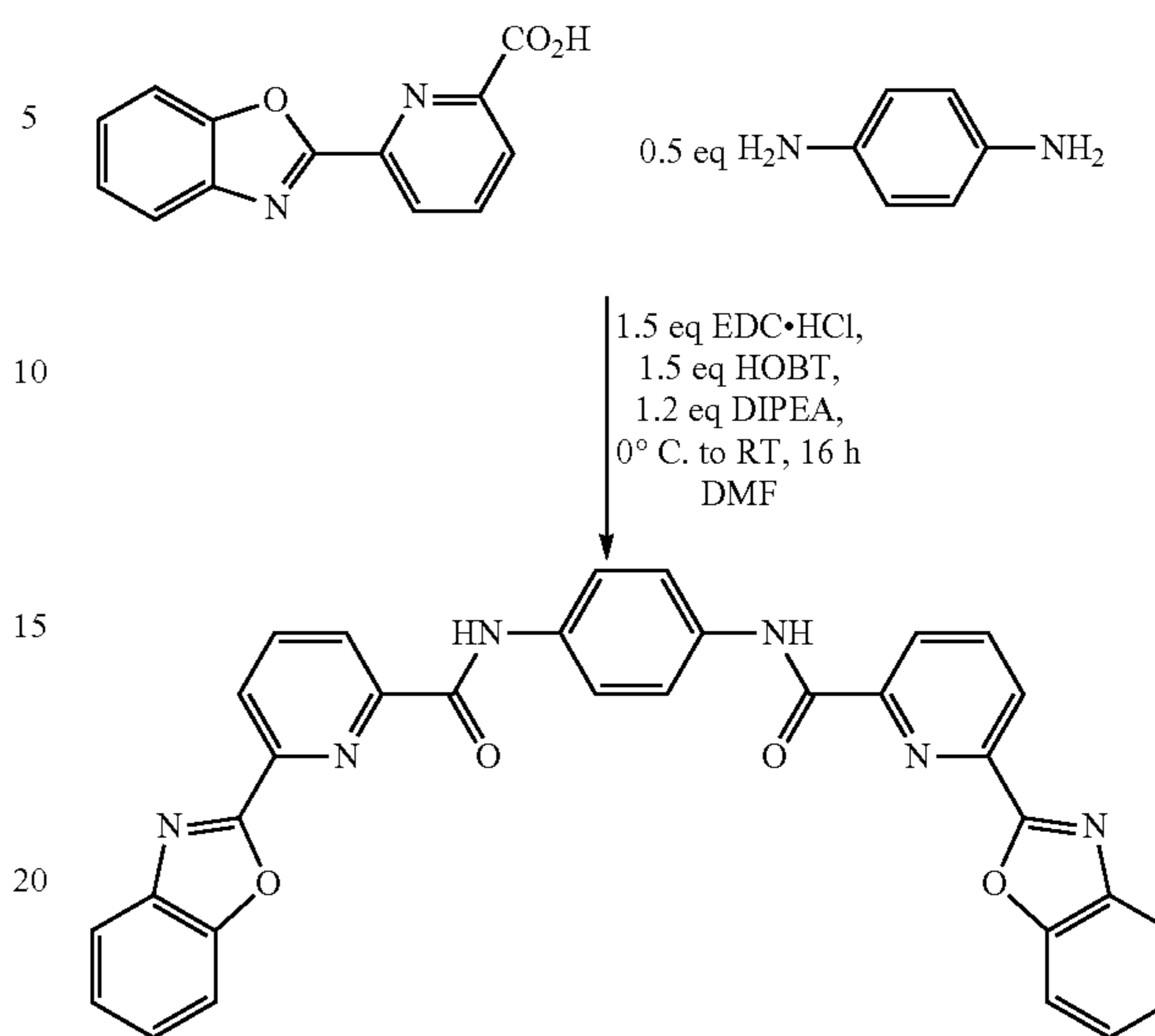
BT-17
