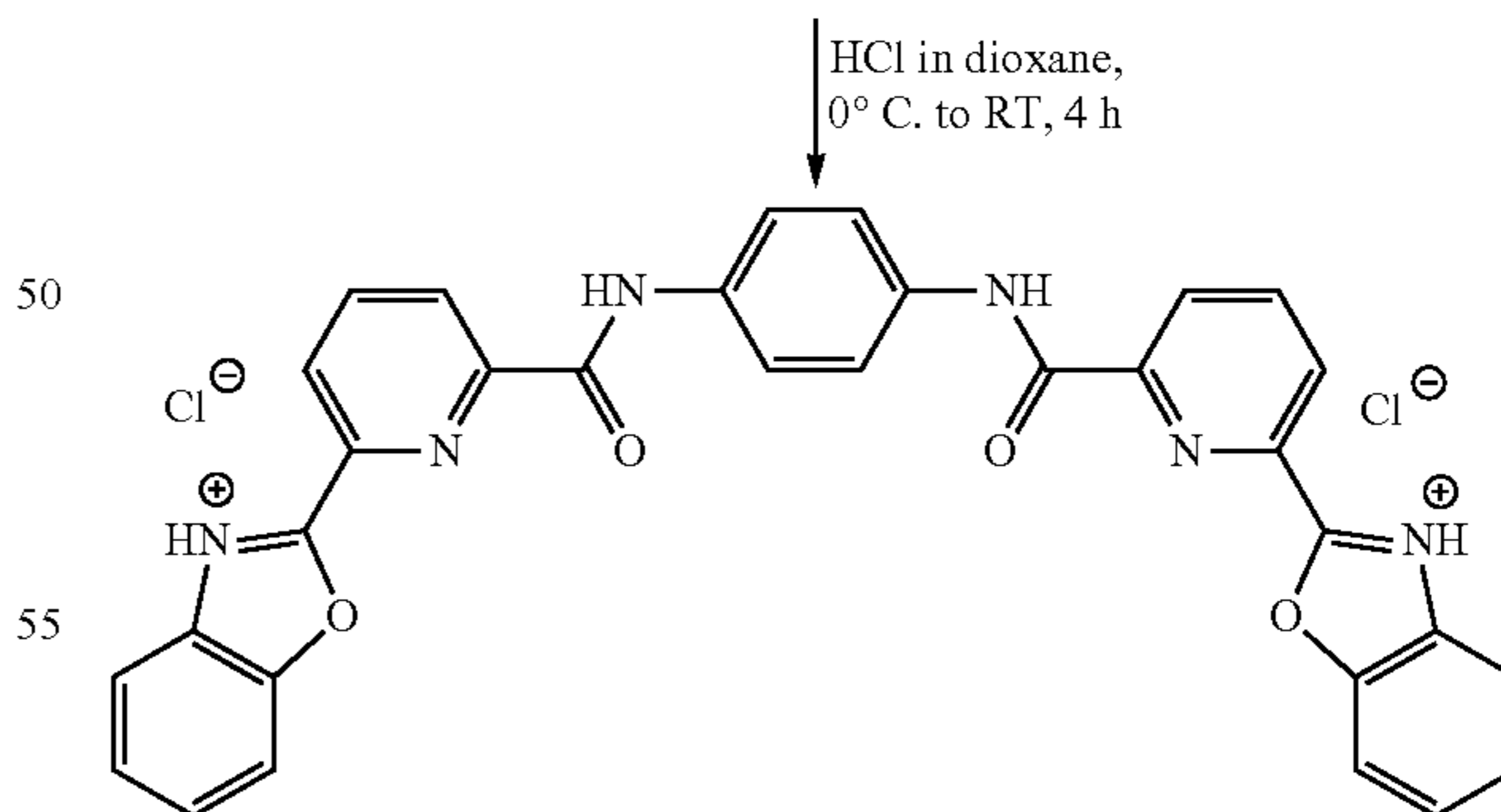
BT-17 salt
