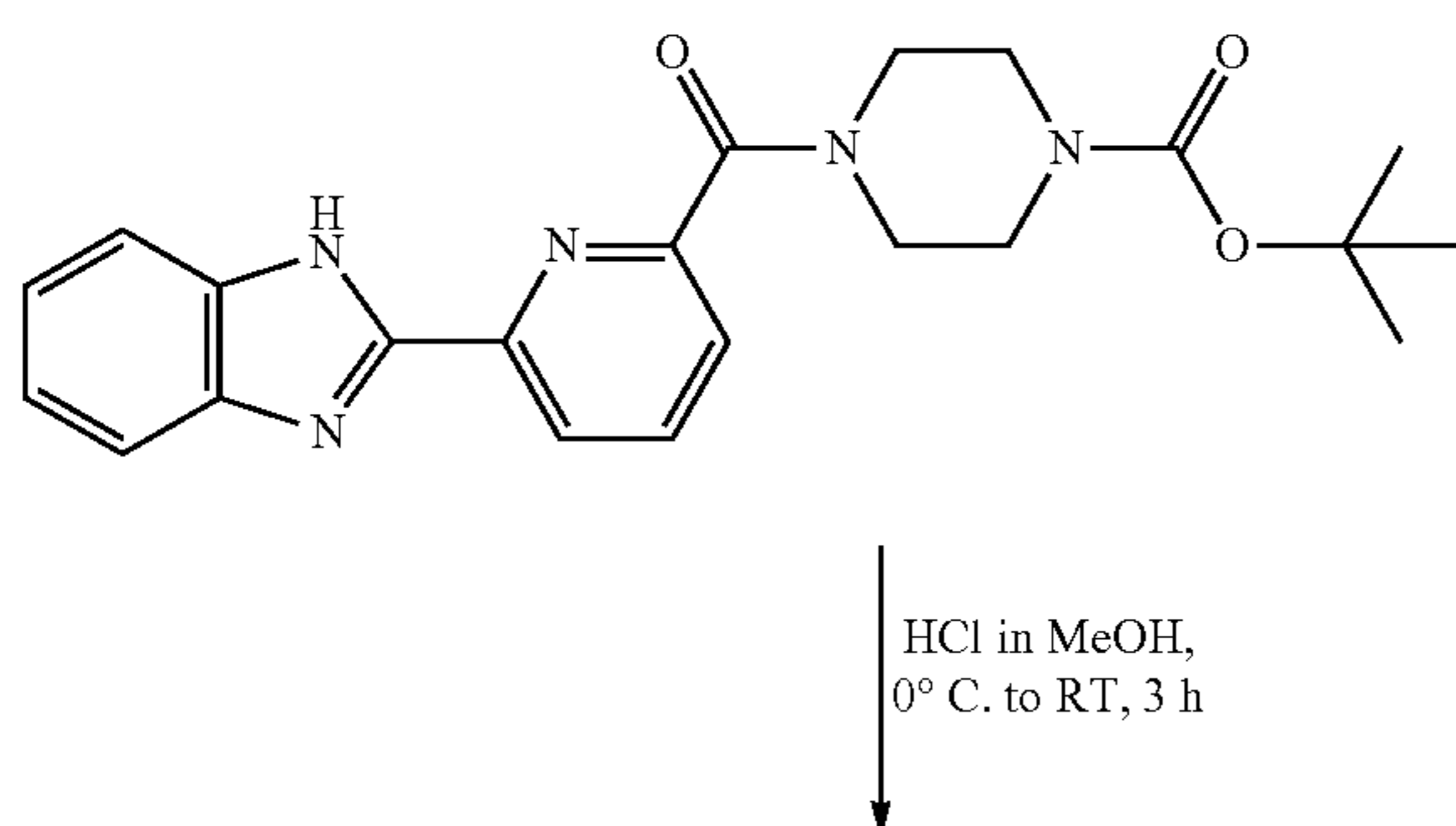
Scheme 6-2
