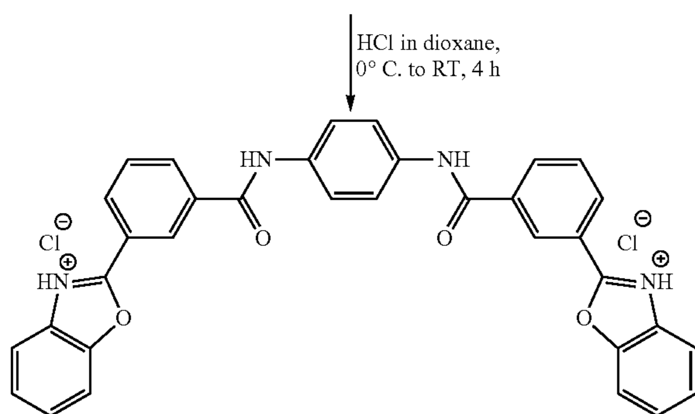
BT-5 salt
