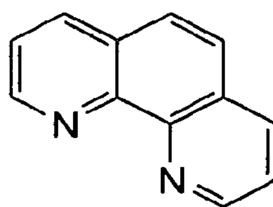
1,10-o-phenanthroline (4,5-diazaphenanthrene)
