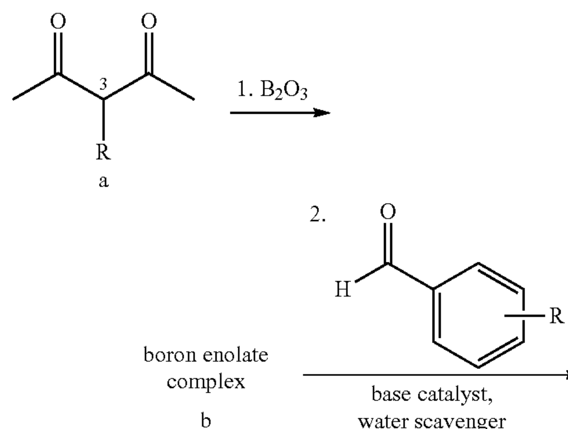
Scheme 1. Synthesis of curcumin analogues.
