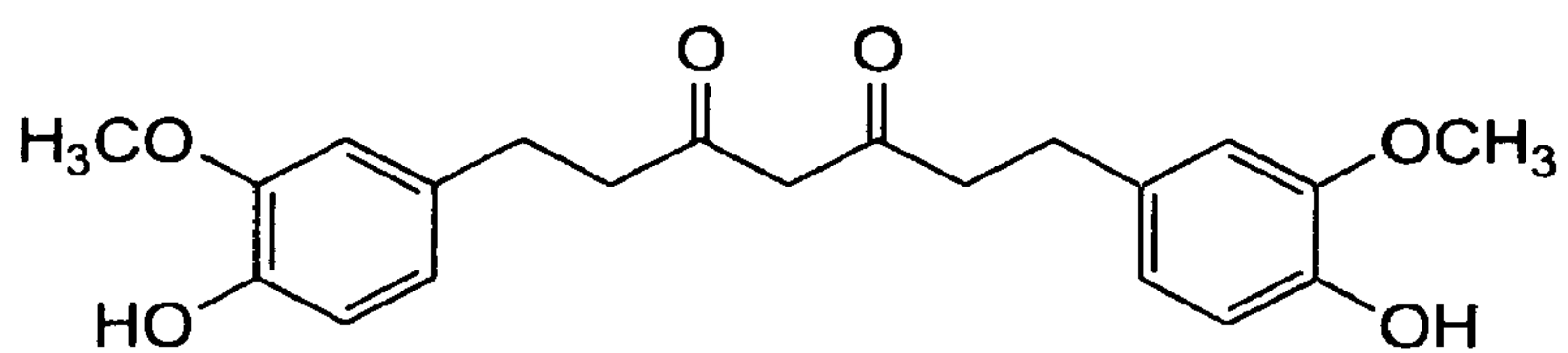
Tetrahydrocurcumin
