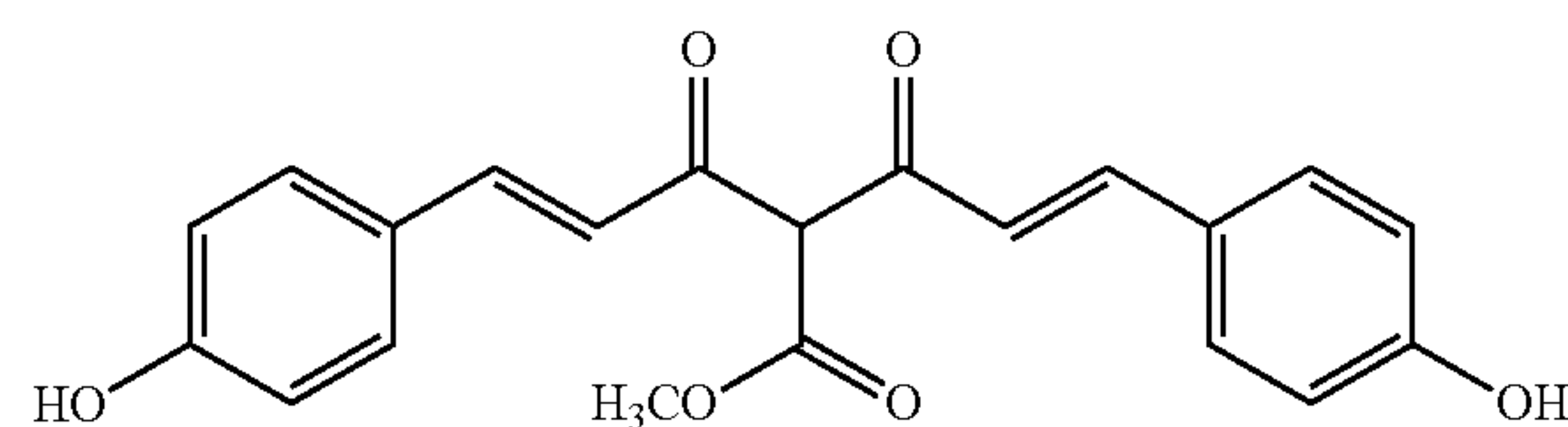
Compound 3
