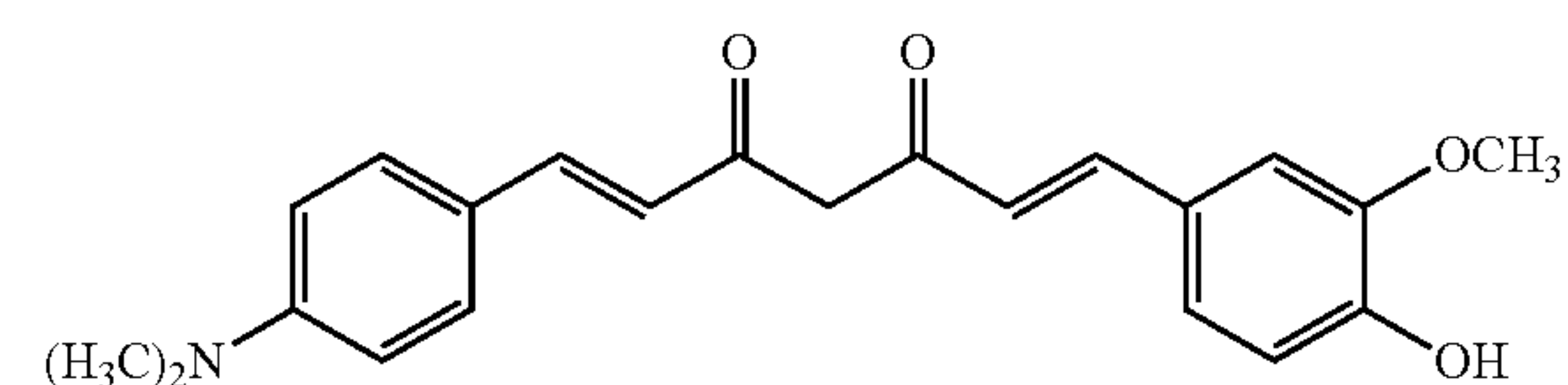
Compound 4
