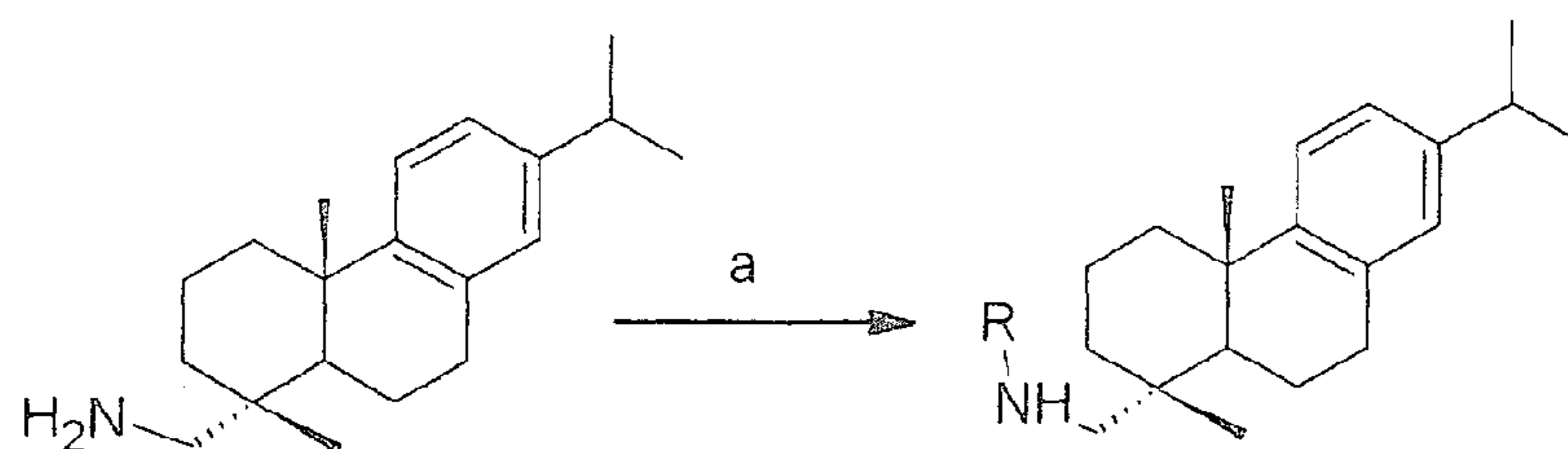
Scheme 3
