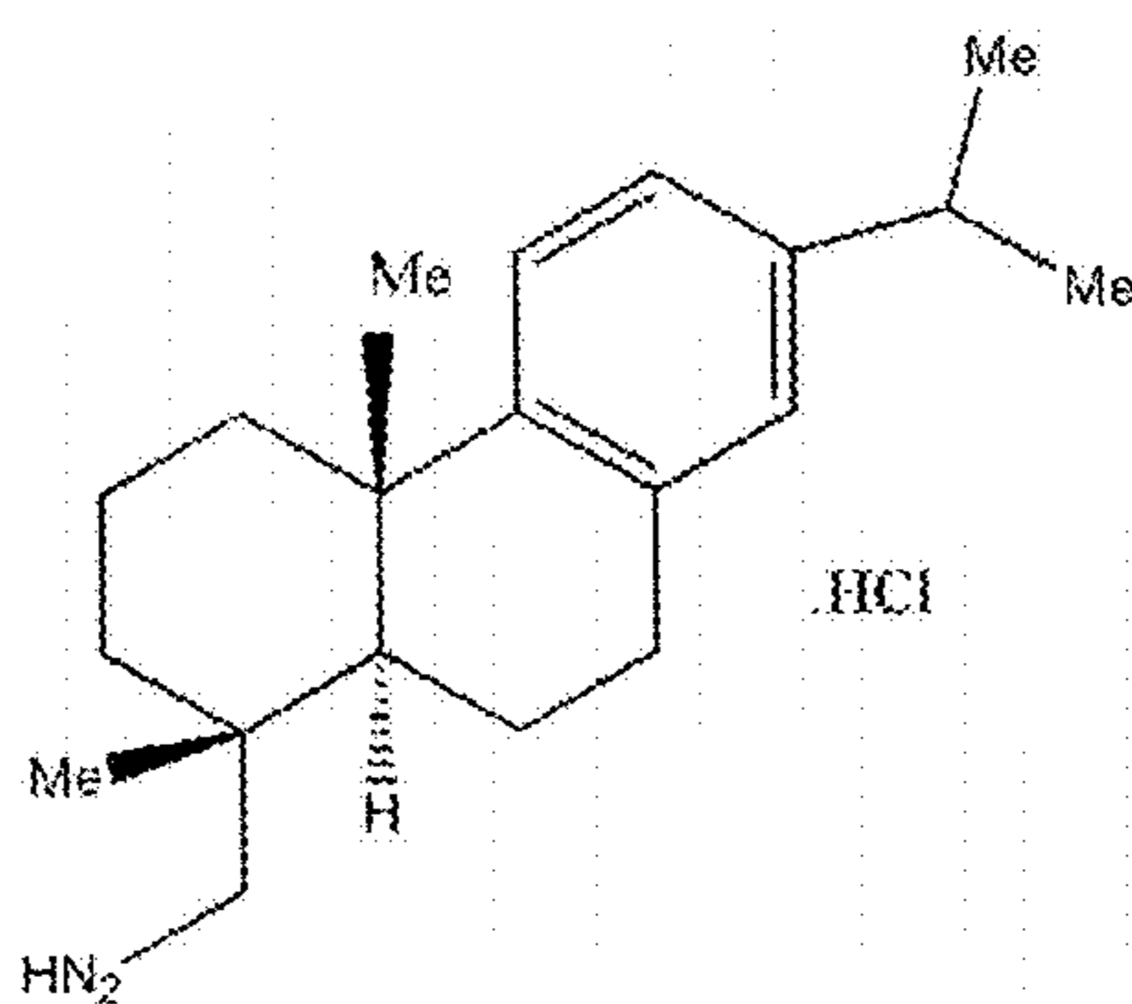
Leelamine hydrochloride
