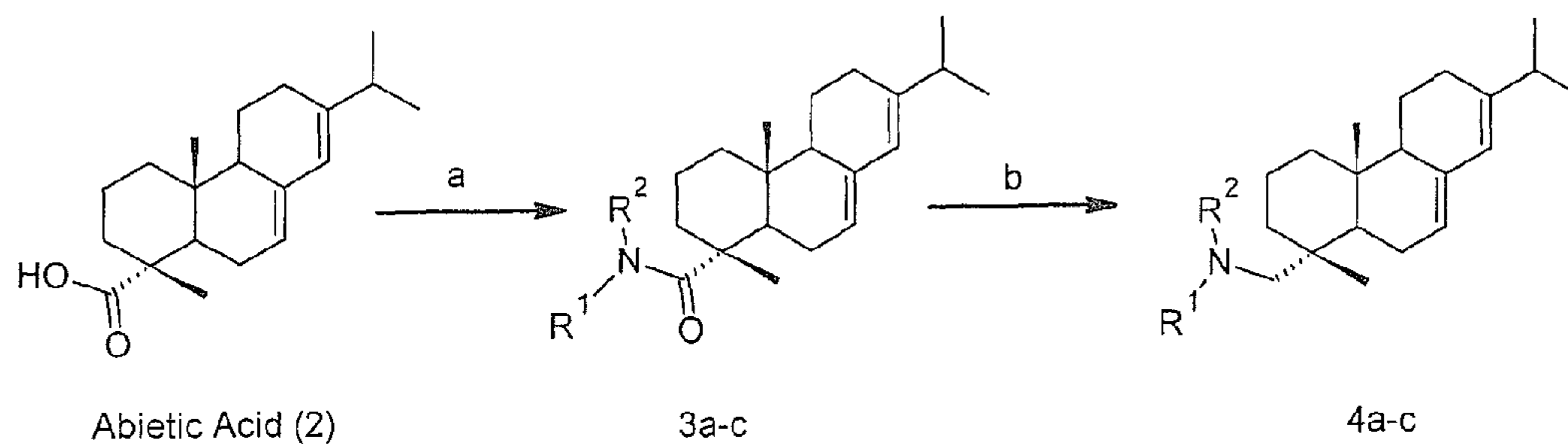
Scheme 2
