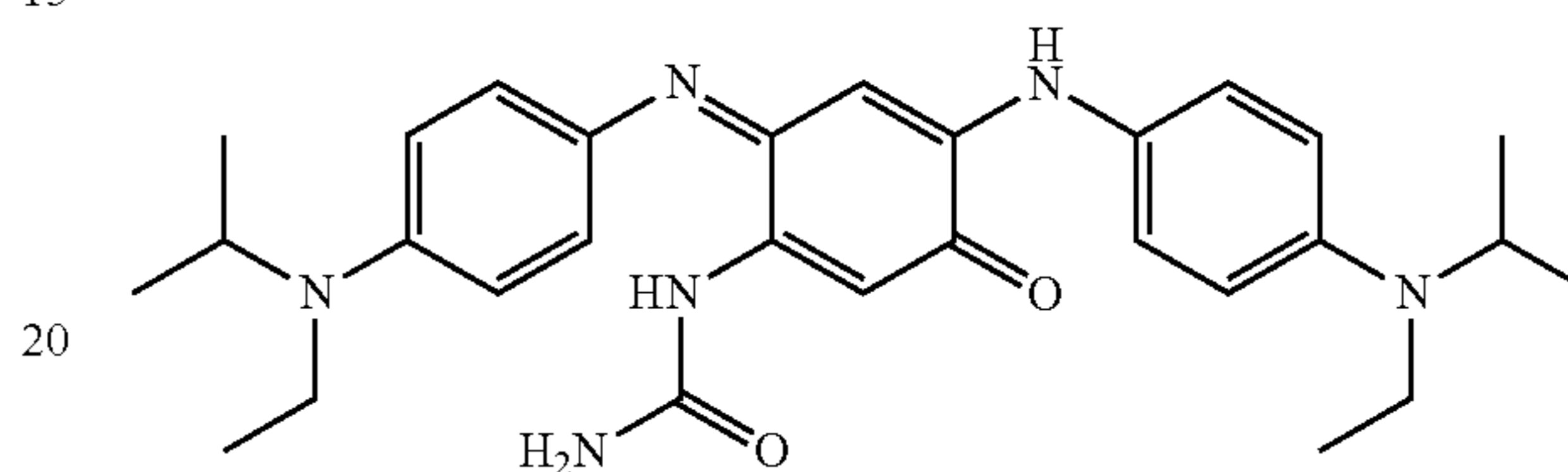
{4-[4-(Ethylisopropylamino)phenylamino]-6-[4-(ethyl-isopropylamino)-phenylimino]-3-oxocyclohexa-1,4-dienyl}urea
