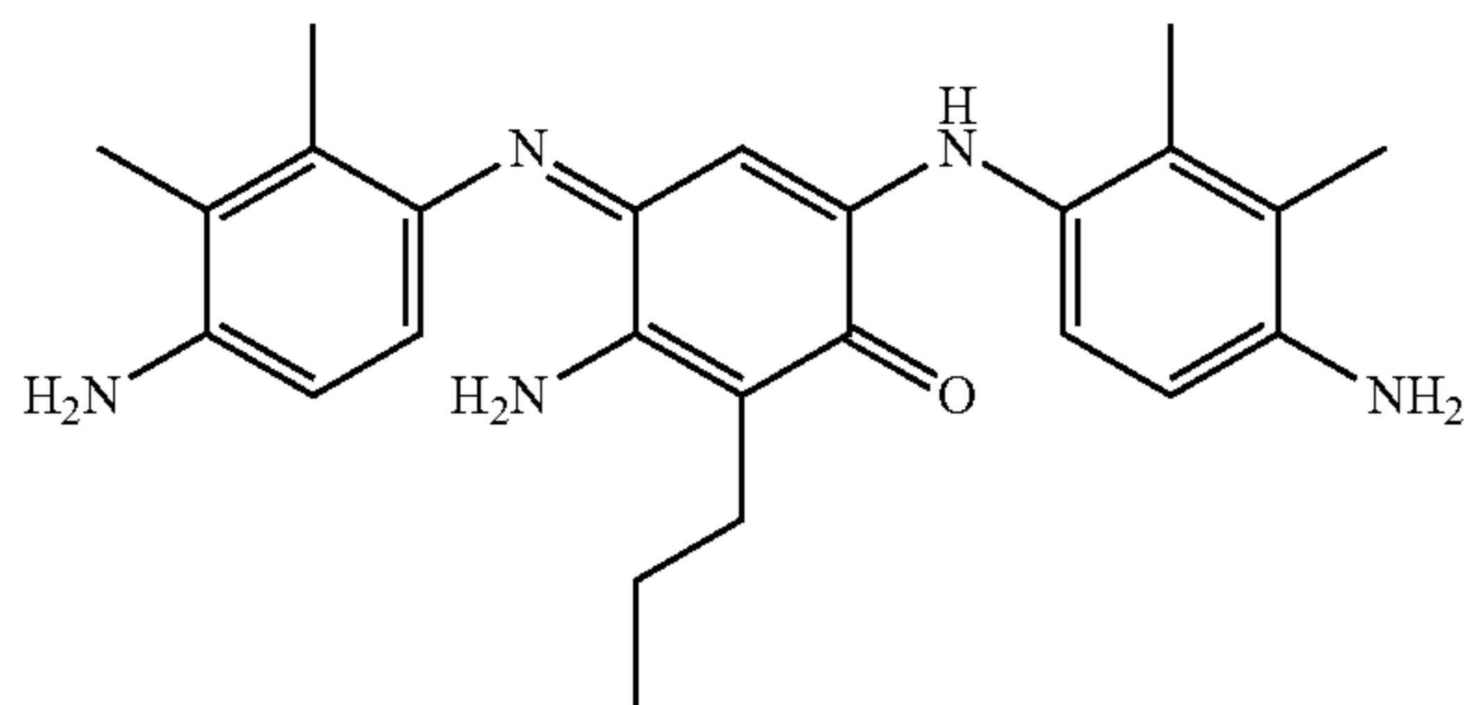
3-Amino-6-(4-amino-2,3-dimethylphenylamino)-4-(4-amino-2,3-dimethyl-phenylimino)-2-propyl-cyclohexa-2,5-dienone
