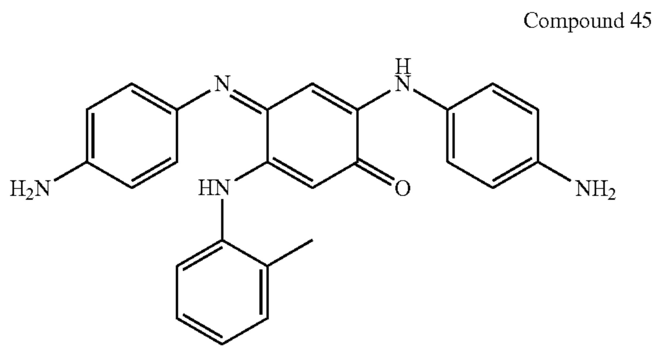
Compound 45 2-(4-Aminophenyl-amino)-4-(4-amino-phenylimino)-5-o-tolylaminocyclohexa-2,5-dienone
