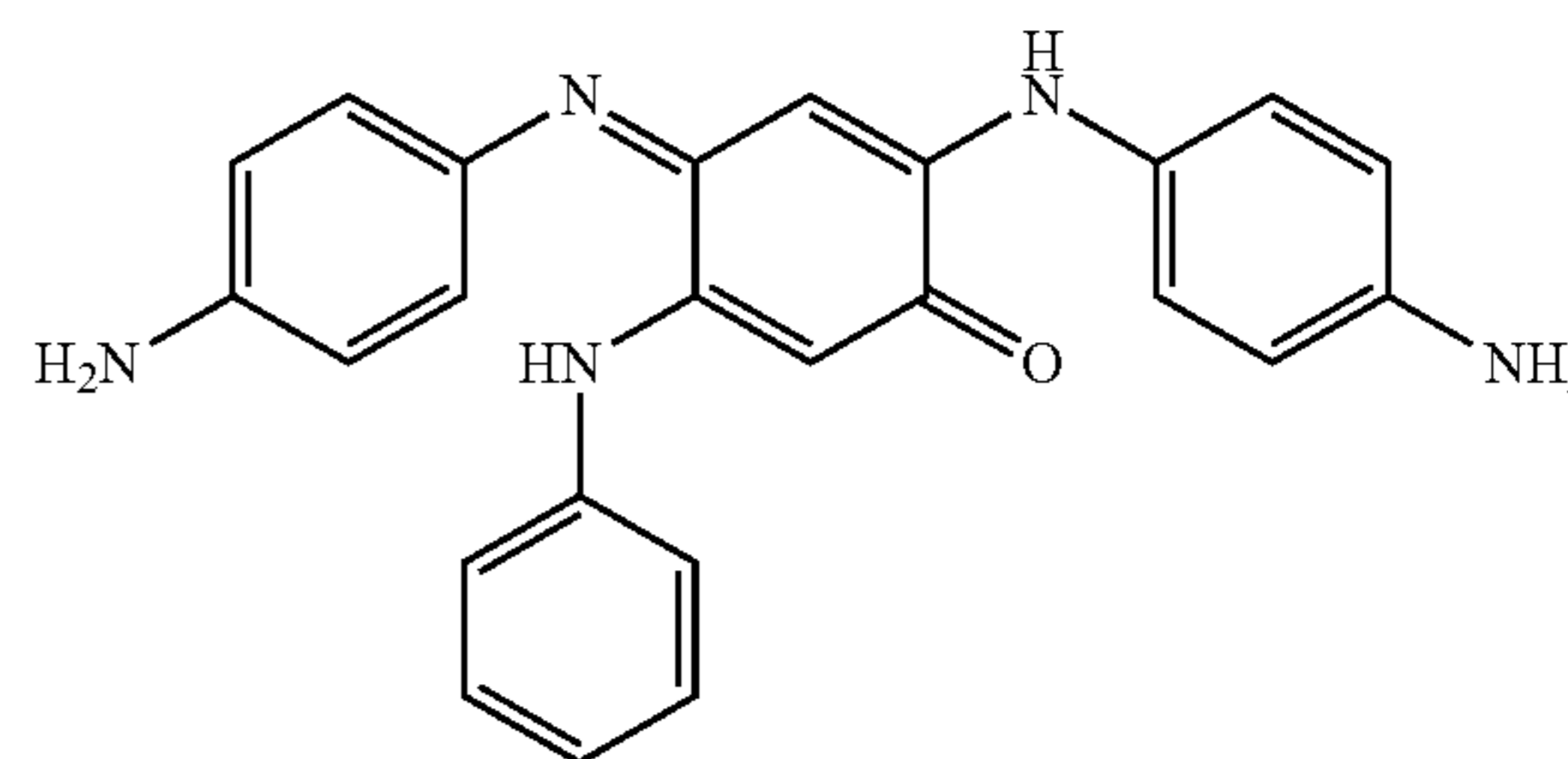
(4-Aminophenylamino)-4-(4-amino-phenylimino)-5-phenylaminocyclohexa-2,5-dienone
