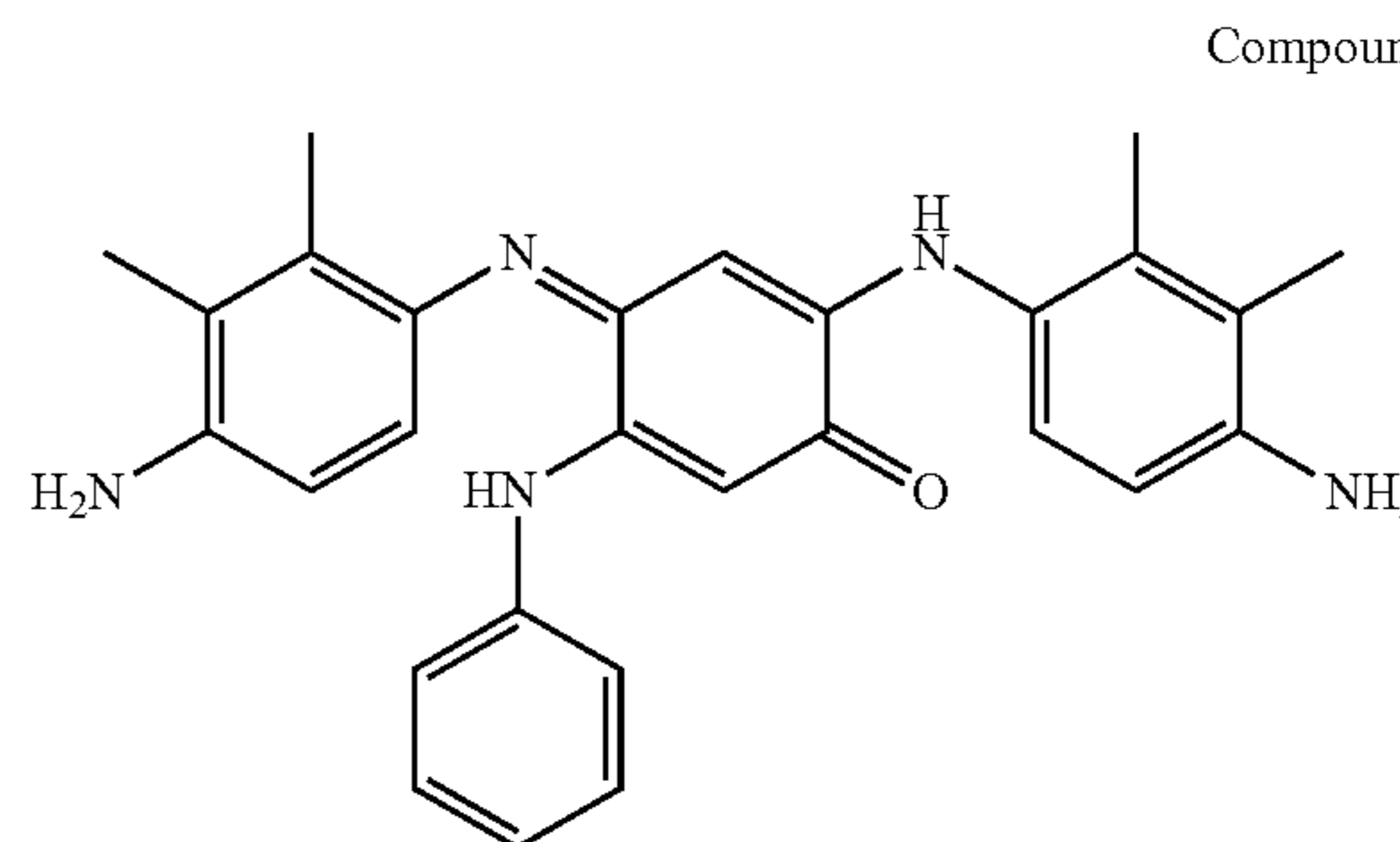
2-(4-Amino-2,3-dimethylphenylamino)-4-(4-amino-2,3-dimethyl-phenylimino)-5-phenylaminocyclohexa-2,5-dienone
