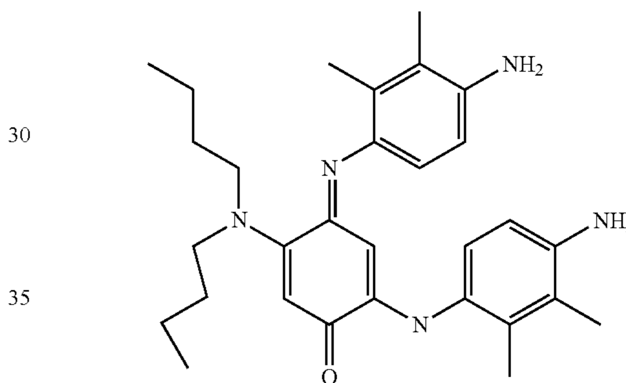
2-(4-Amino-2,3-dimethylphenylamino)-4-(4-amino-2,3-dimethylphenylimino)-5-dibutylamino-cyclohexa-2,5-dienone
