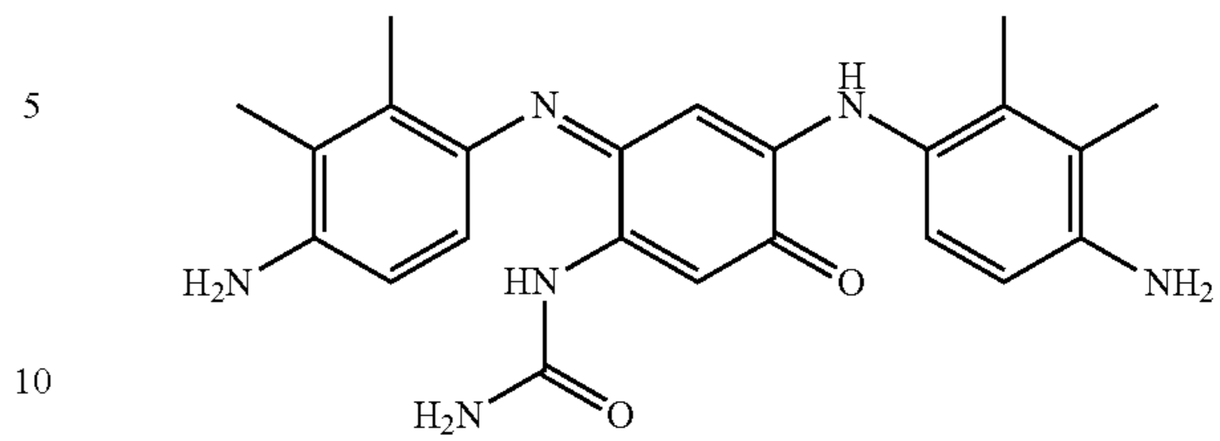
[4-(4-Amino-2,3-dimethylphenylamino)-6-(4-amino-2,3-dimethylphenylimino)-3-oxocyclohexa-1,4-dienyl]urea
