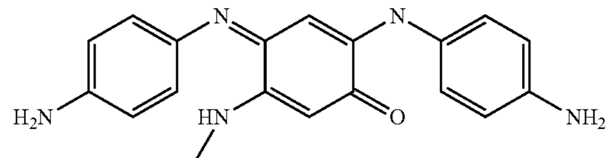
2-(4-Aminophenylamino)-4-(4-amino-phenylimino)-5-methylaminocyclohexa-2,5-dienone
