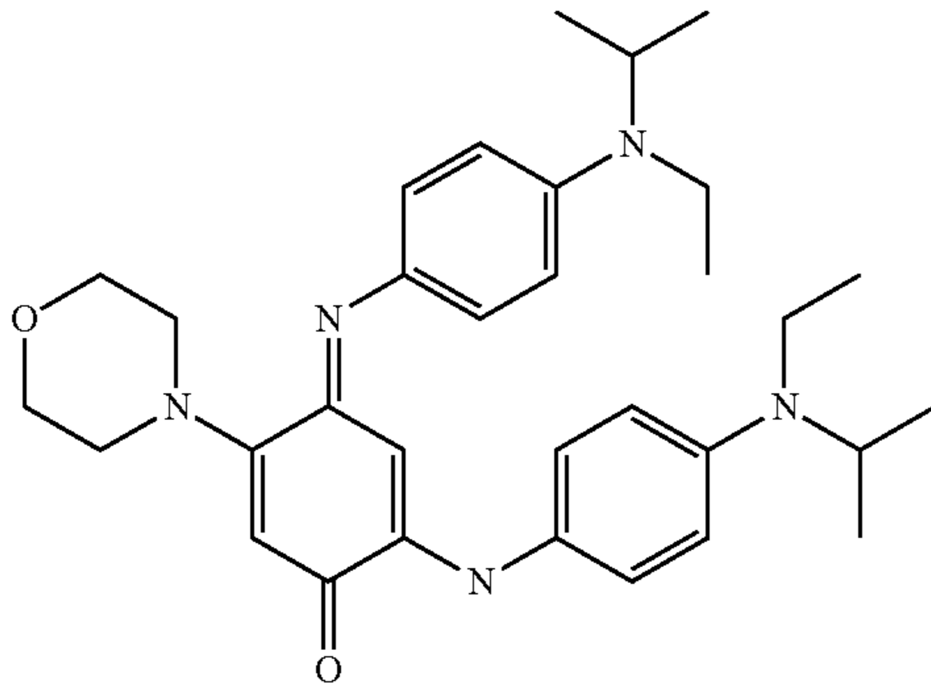
2-[4-(Ethylisopropyl-amino)phenyl-amino]-4-[4-(ethyl-isopropylamino)-phenylimino]-5-morpholin-4-ylcyclohexa-2,5-dienone
