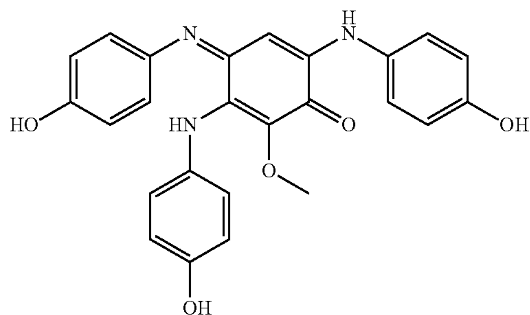
3,6-Bis(4-hydroxy-phenylamino)-4-(4-hydroxy-phenylimino)-2-methoxycyclohexa-2,5-dienone
