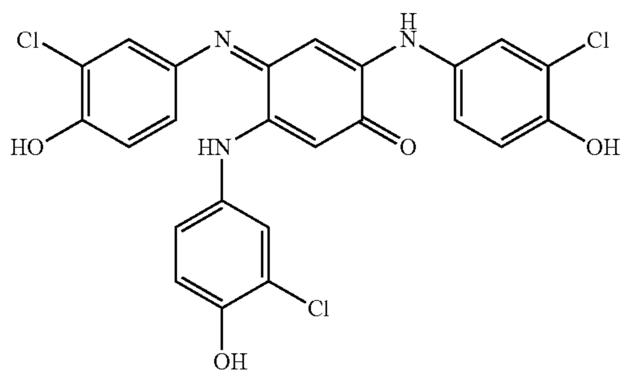
2,5-Bis(3-chloro-4-hydroxyphenylamino)-4-(3-chloro-4-hydroxyphenylimino)cyclohexa-2,5-dienone
