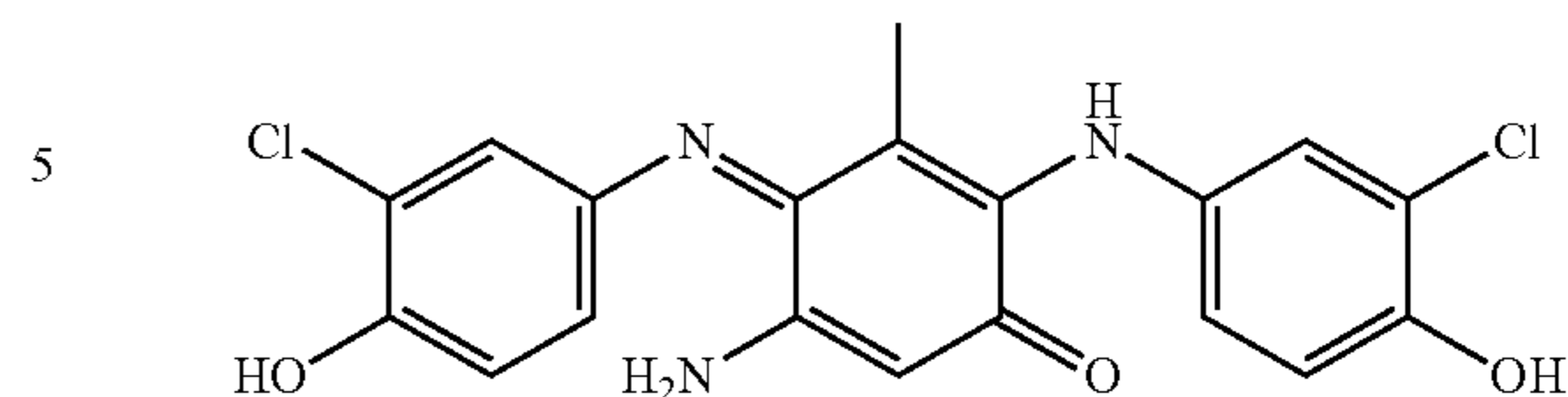
5-Amino-2-(3-chloro-4-hydroxyphenylamino)-4-(3-chloro-4-hydroxy-phenylimino)-3-methyl-cyclohexa-2,5-dienone
