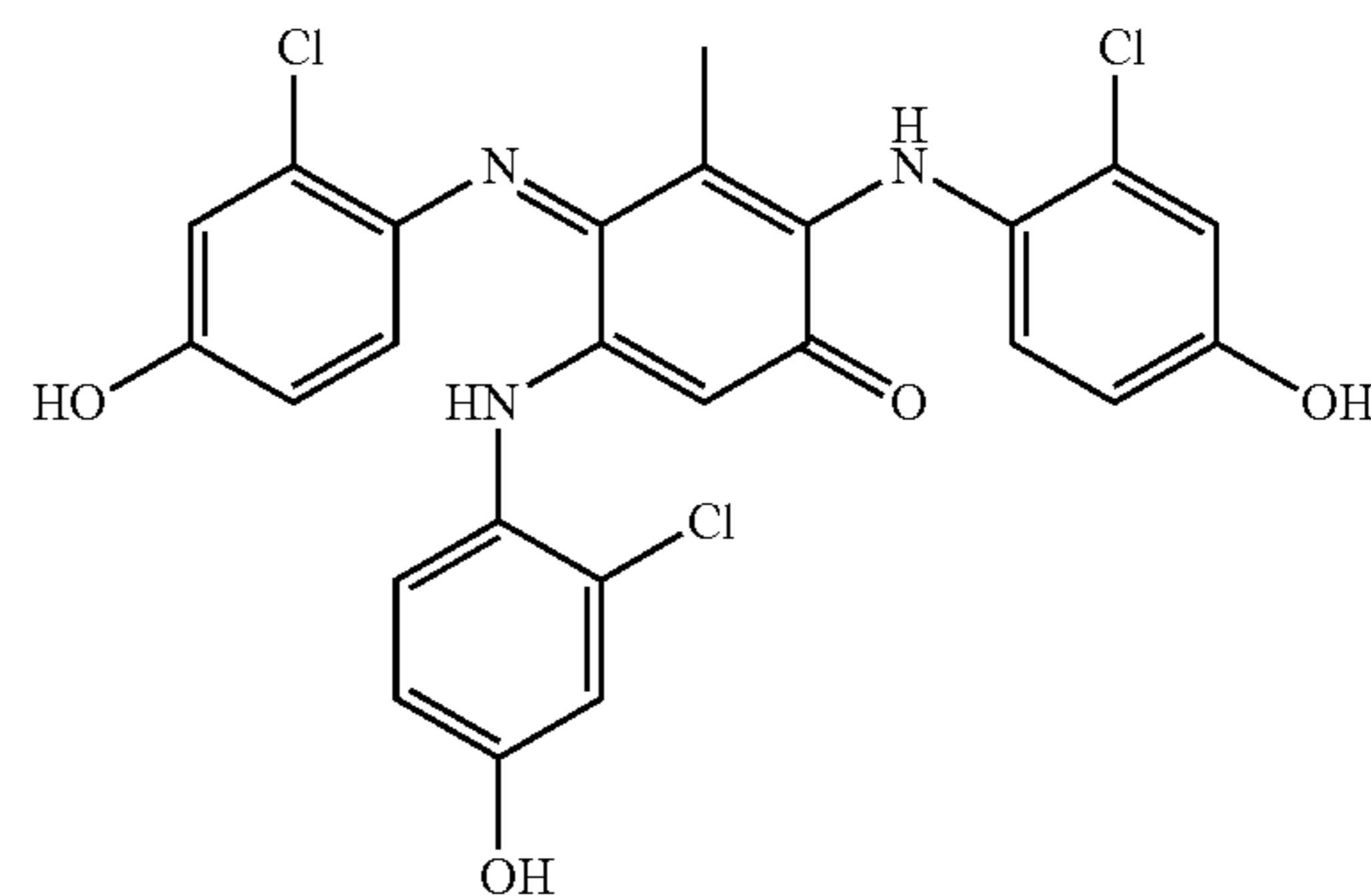
2,5-Bis(2-chloro-4-hydroxyphenylamino)-4-(2-chloro-4-hydroxyphenylimino)-3-methyl-cyclohexa-2,5-dienone
