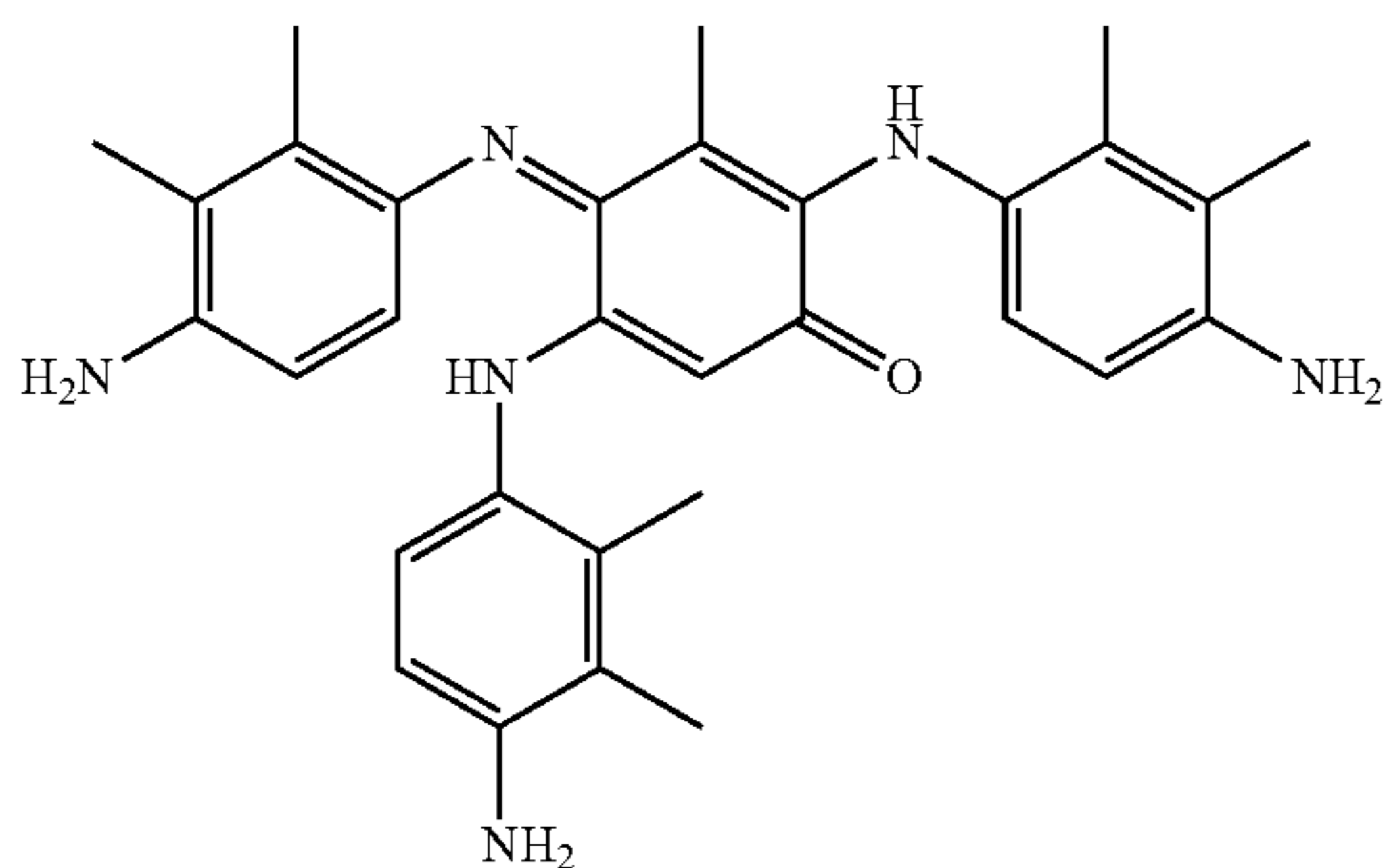
2,5-Bis(4-amino-2,3-dimethylphenylamino)-4-(4-amino-2,3-dimethylphenylimino)-3-methyl-cyclohexa-2,5-dienone
