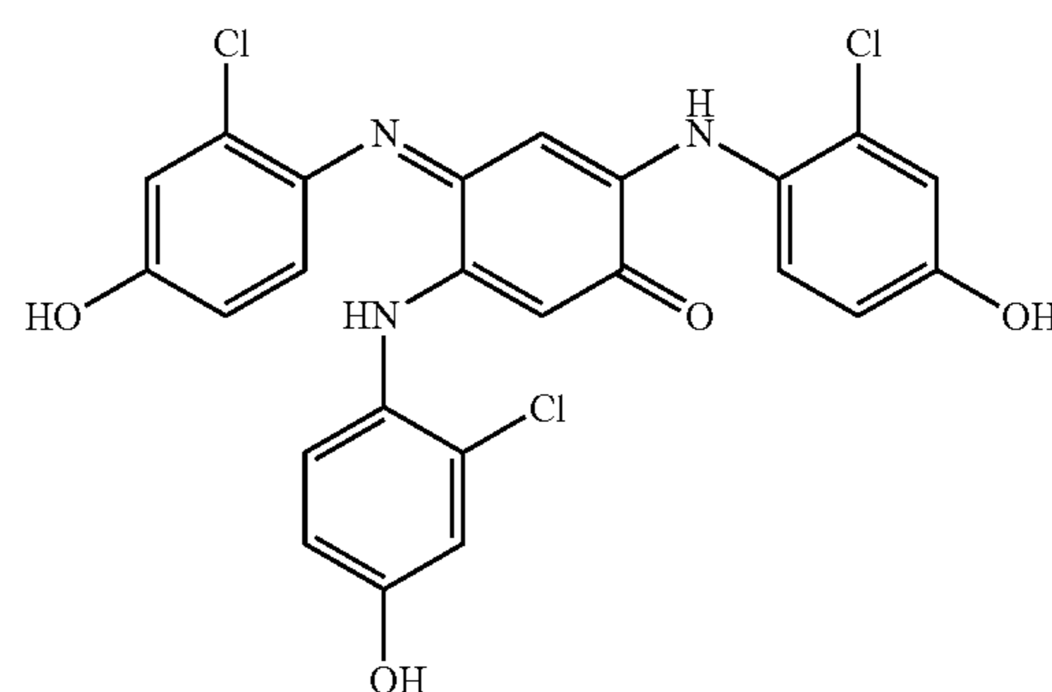
2,5-Bis(2-chloro-4-hydroxyphenylamino)-4-(2-chloro-4-hydroxyphenylimino)cyclohexa-2,5-dienone
