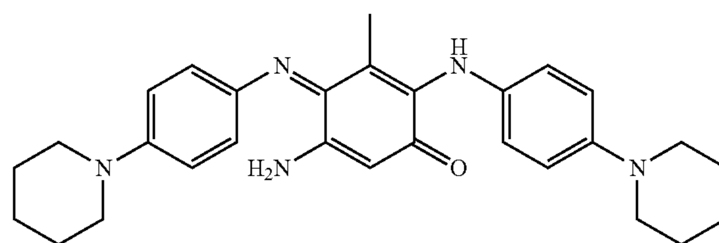
5-Amino-3-methyl-2-(4-piperidin-1-yl-phenylamino)-4-[4-piperidin-1-ylphenylimino]cyclohexa-2,5-dienone
