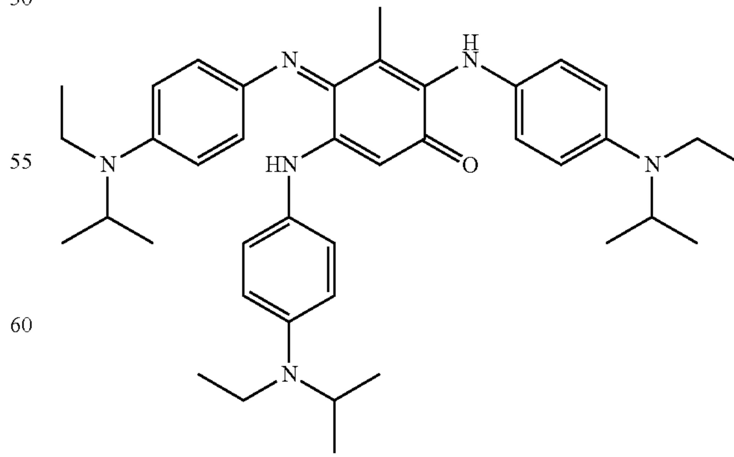
2,5-Bis[4-(ethylisopropyl-amino)-phenylamino]-4-[4-(ethyl-isopropyl-amino)phenylimino]-3-methylcyclohexa-2,5-dienone
