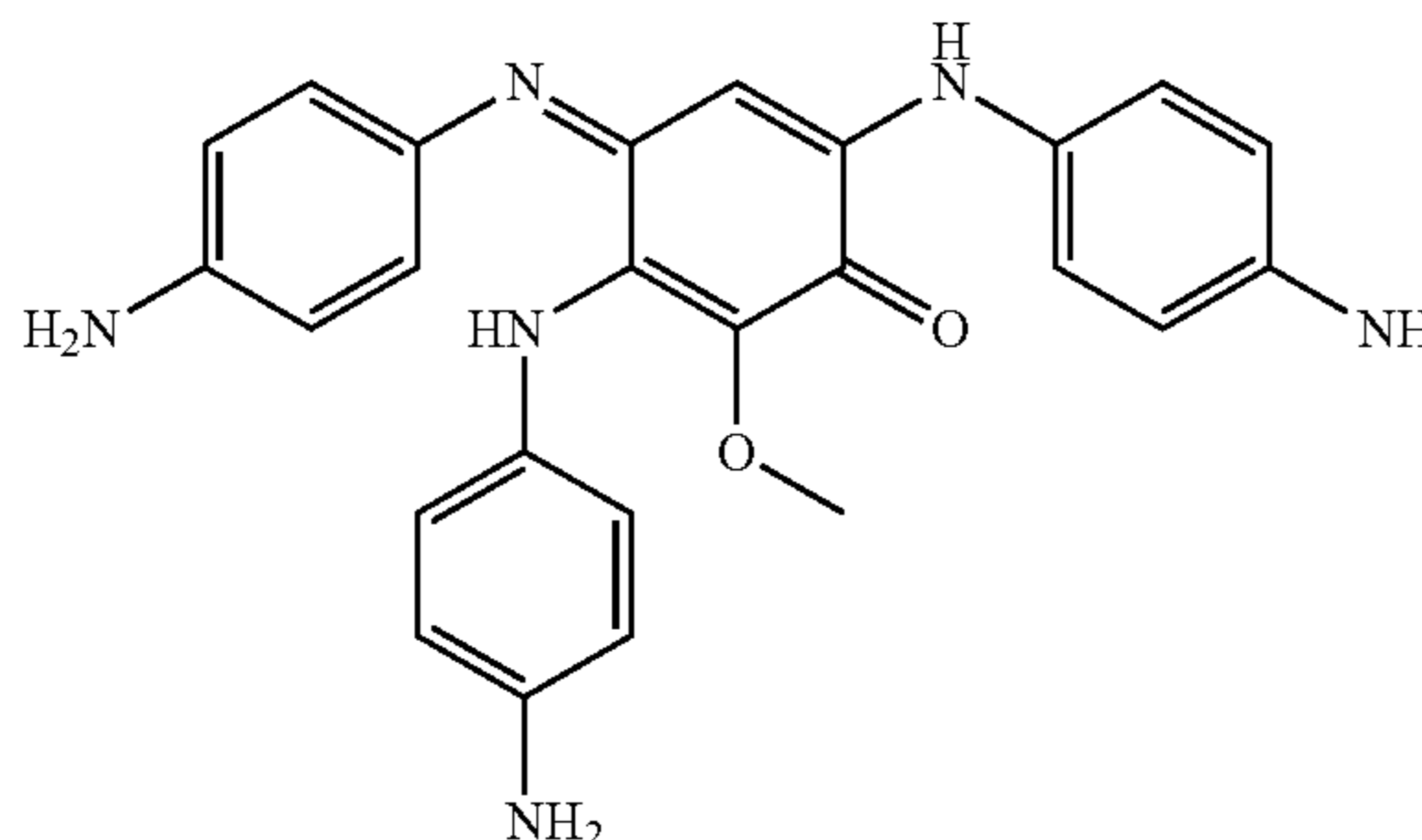
3,6-Bis(4-aminophenylamino)-4-(4-aminophenylimino)-2-methoxycyclohexa-2,5-dienone
