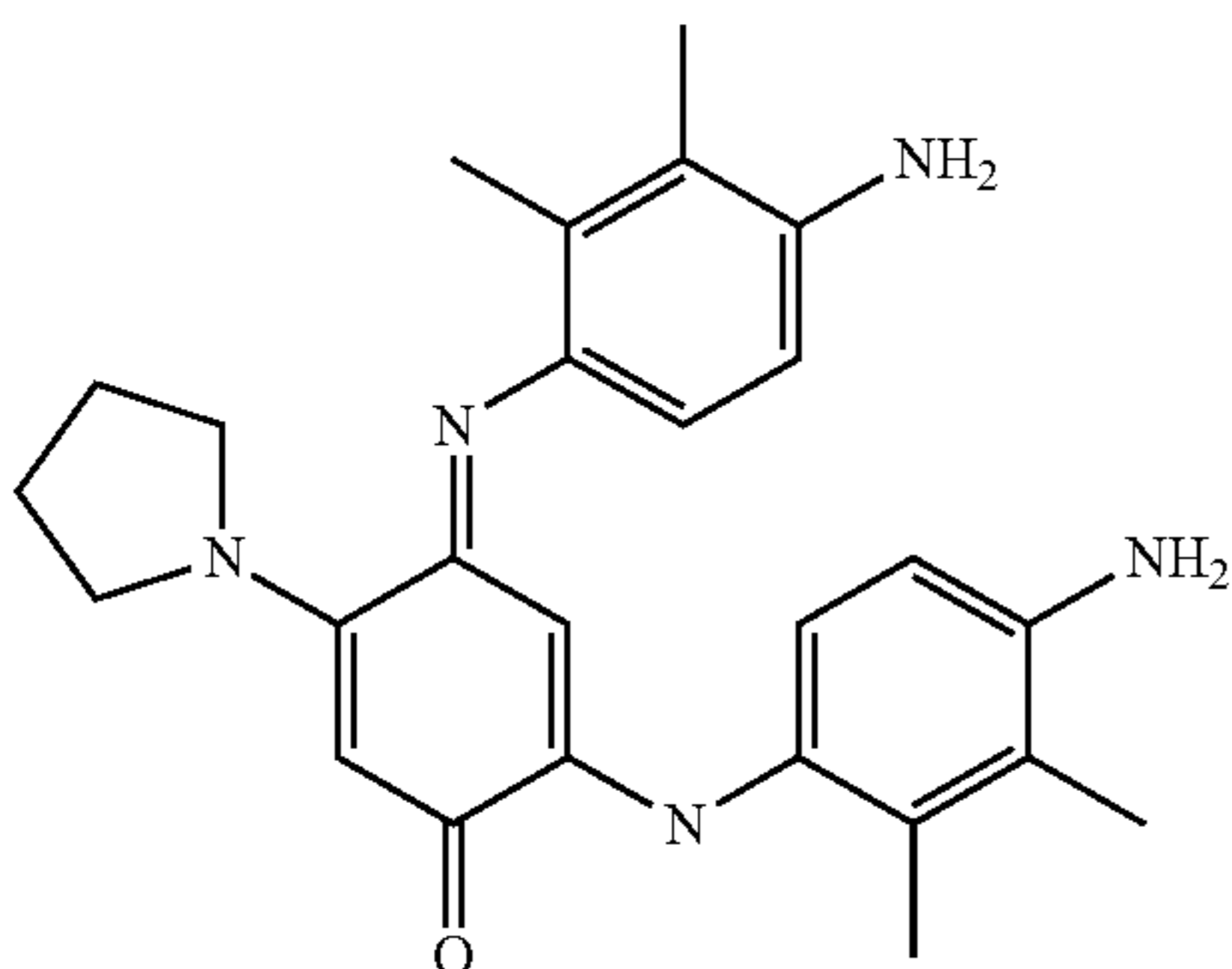
2-(4-Amino-2,3-dimethylphenylamino)-4-(4-amino-2,3-diethylphenylimino)-5-pyrrolidin-1-ylcyclohexa-2,5-dienone
