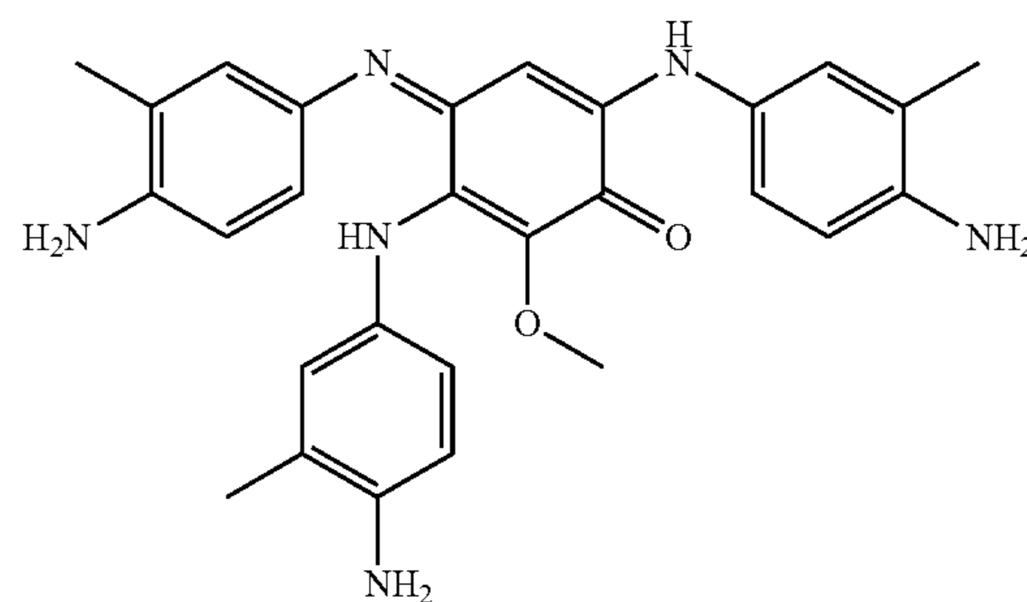
3,6-Bis(4-amino-3-methylphenylamino)-4-(4-amino-3-methylphenylimino)-2-methoxy-cyclohexa-2,5-dienone
