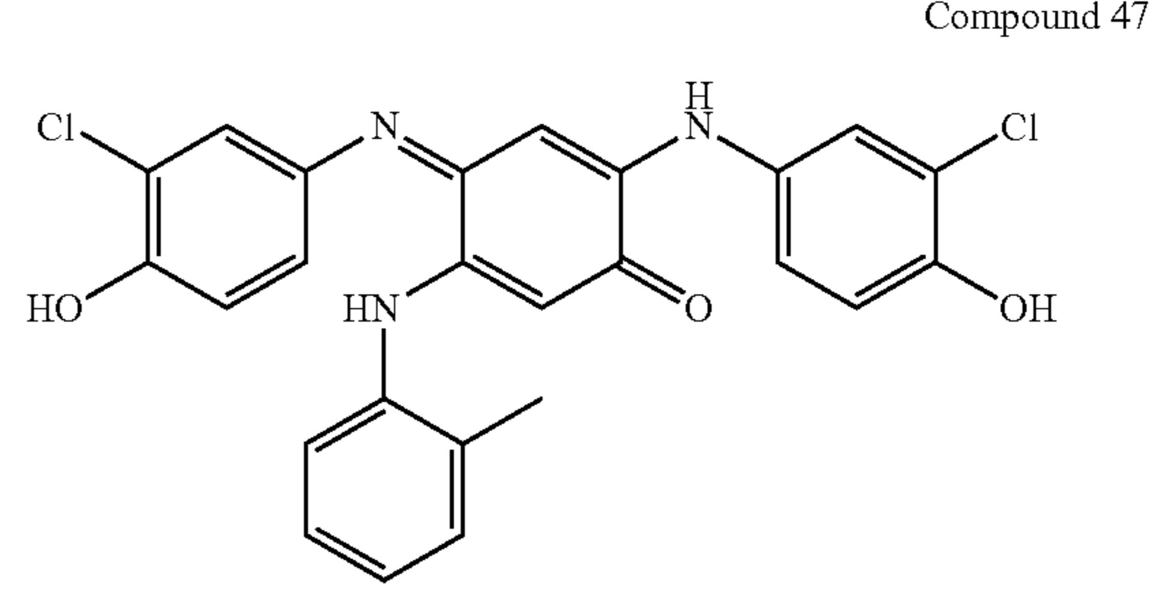
Compound 47 2-(3-Chloro-4-hydroxyphenylamino)-4-(3-chloro-4-hydroxy-phenylimino)-5-o-tolylaminocyclohexa-2,5-dienone
