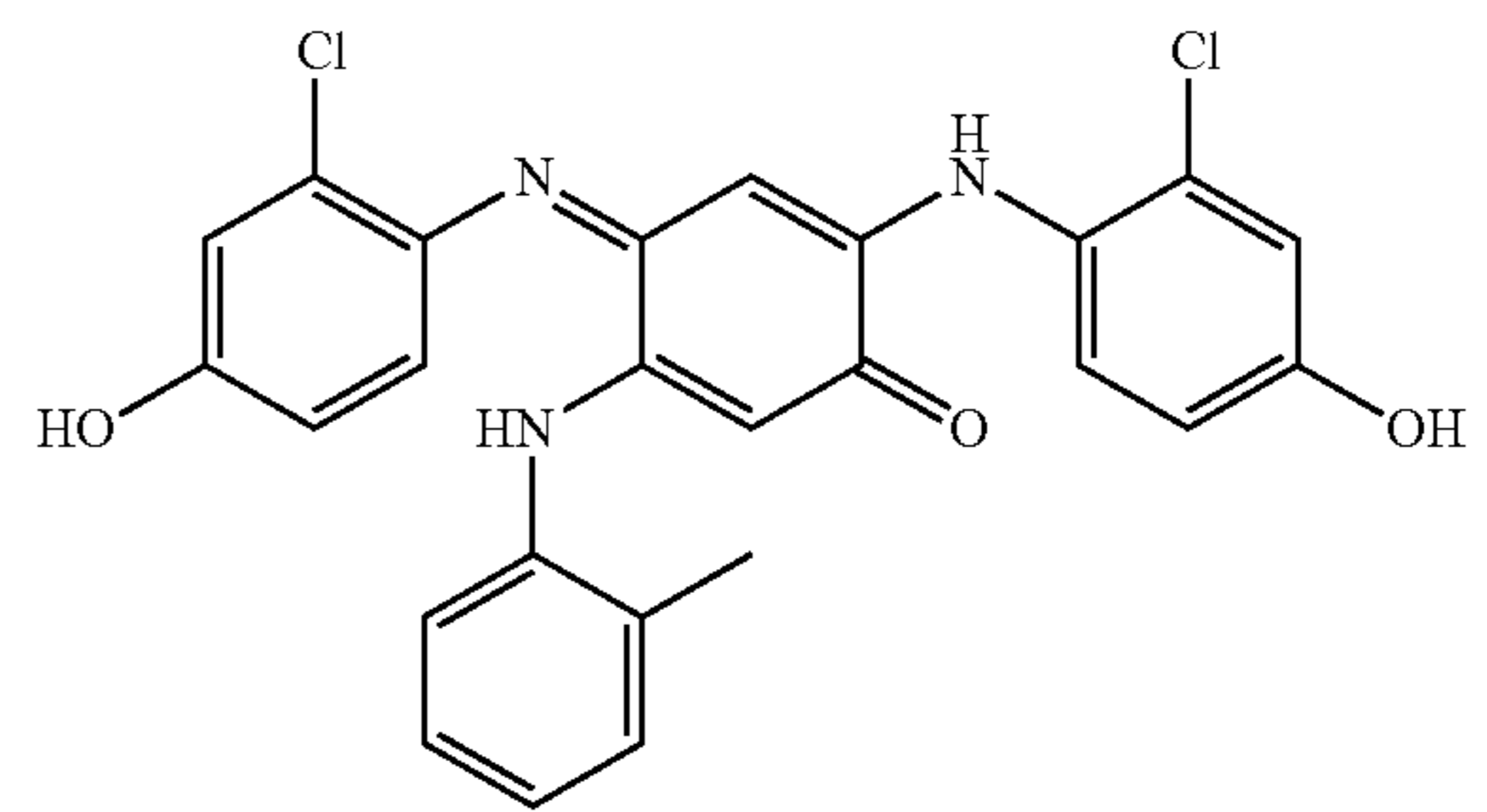
Compound 48 2-(2-Chloro-4-hydroxy-phenylamino)-4-(2-chloro-4-hydroxy-phenylimino)-5-o-tolylaminocyclohexa-2,5-dienone
