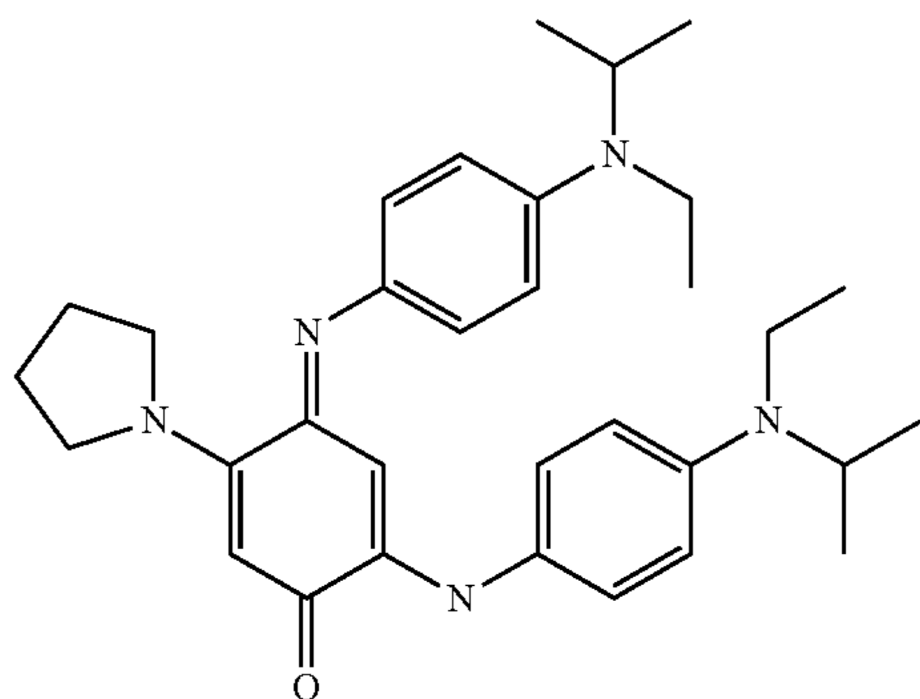
2-[4-(Ethylisopropylamino)-phenyl-amino]-4-[4-(ethylisopropyl-amino)]phenylimino-5-pyrrolidin-1-ylcyclohexa-2,5-dienone
