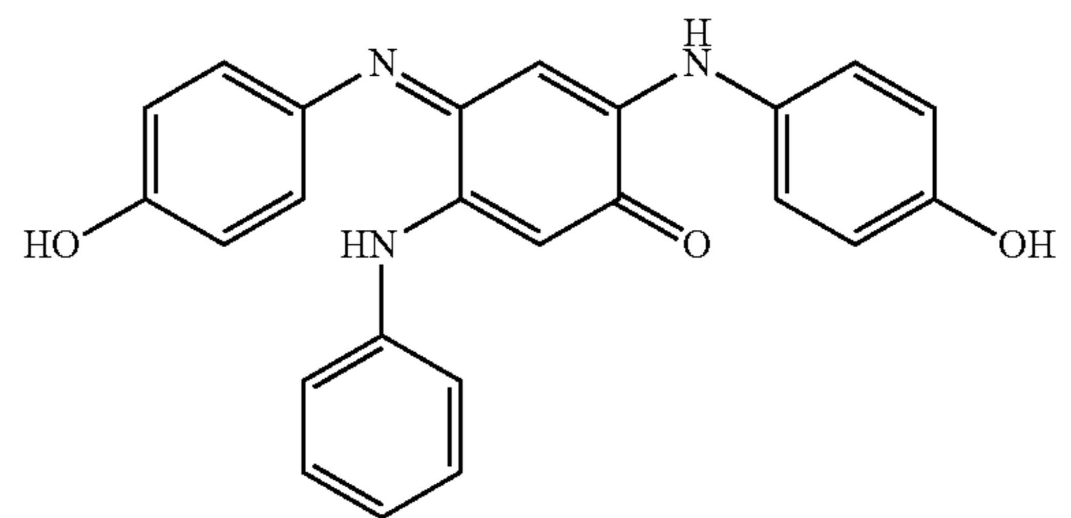
2-(4-Hydroxy-phenylamino)-4-(4-hydroxyphenylimino)-5-phenylaminocyclohexa-2,5-dienone
