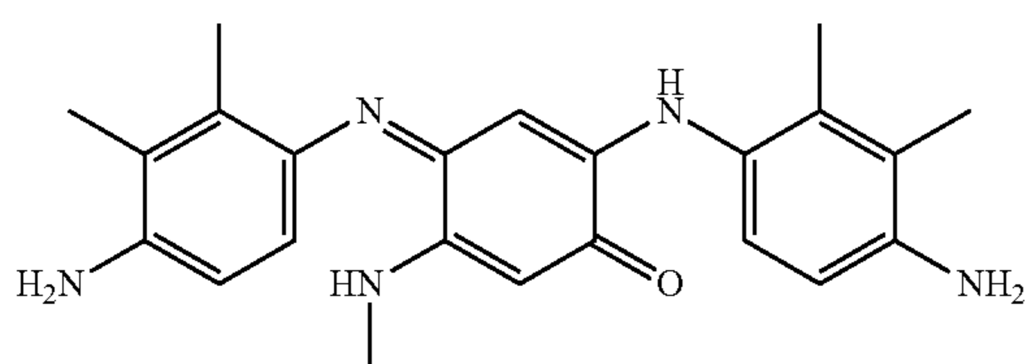
2-(4-Amino-2,3-dimethyl-phenylamino)-4-(4-amino-2,3-dimethylphenylimino)-5-methylaminocyclohexa-2,5-dienone
