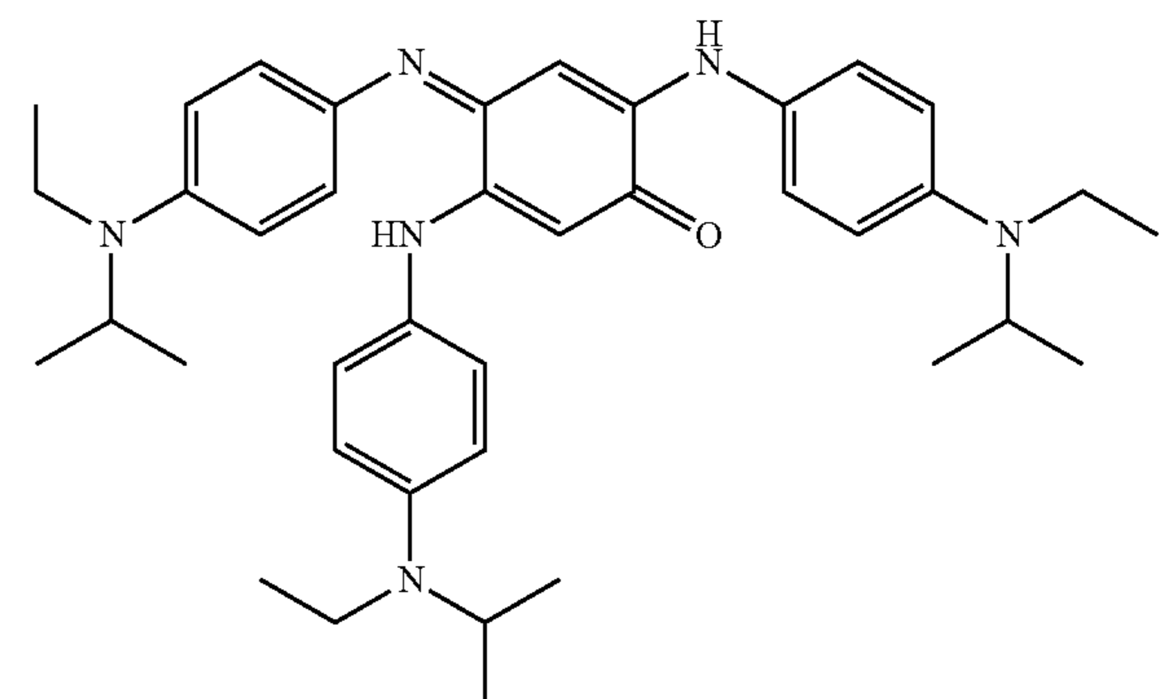
2,5-Bis[4-(ethylisopropyl-amino)-phenylamino]-4-[4-(ethylisopropylamino)-phenylimino]cyclohexa-2,5-dienone
