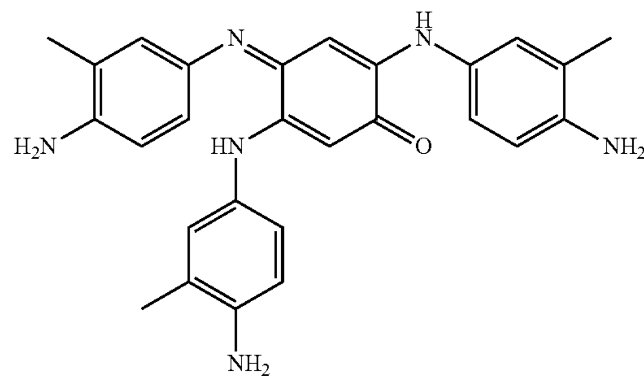
2,5-Bis(4-amino-3-methyl-phenylamino)-4-(4-amino-3-methylphenylimino)cyclohexa-2,5-dienone
