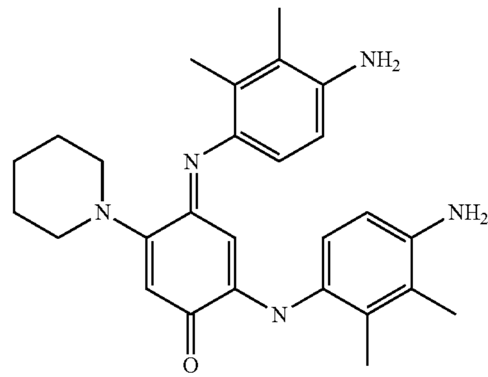
2-(4-Amino-2,3-dimethylphenylamino)-4-(4-amino-2,3-dimethylphenylimino)-5-piperidin-1-ylcyclohexa-2,5-dienone
