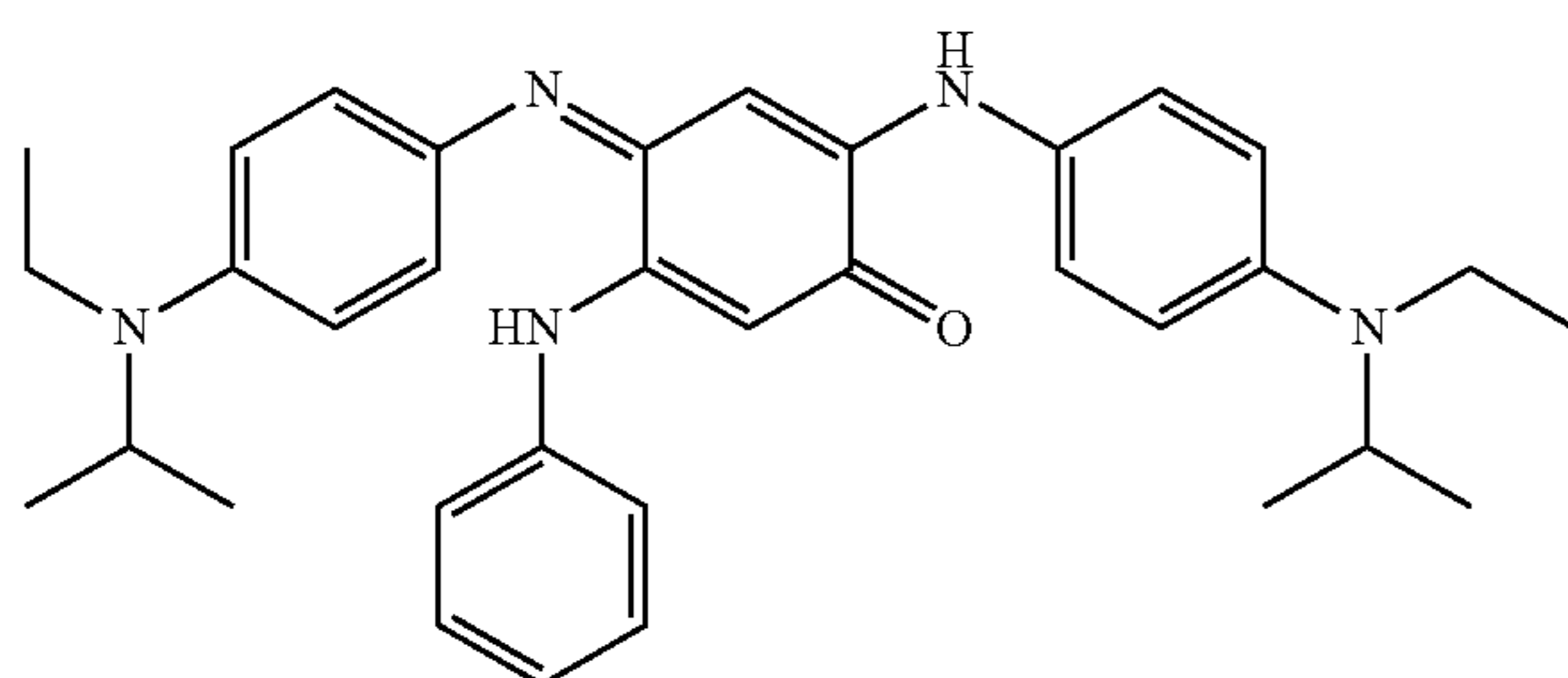
2-[4-Ethylisopropylamino]-phenyl-amino]-4-[4-(ethyl-isopropylamino)-phenylimino]-5-phenylaminocyclohexa-2,5-dienone
