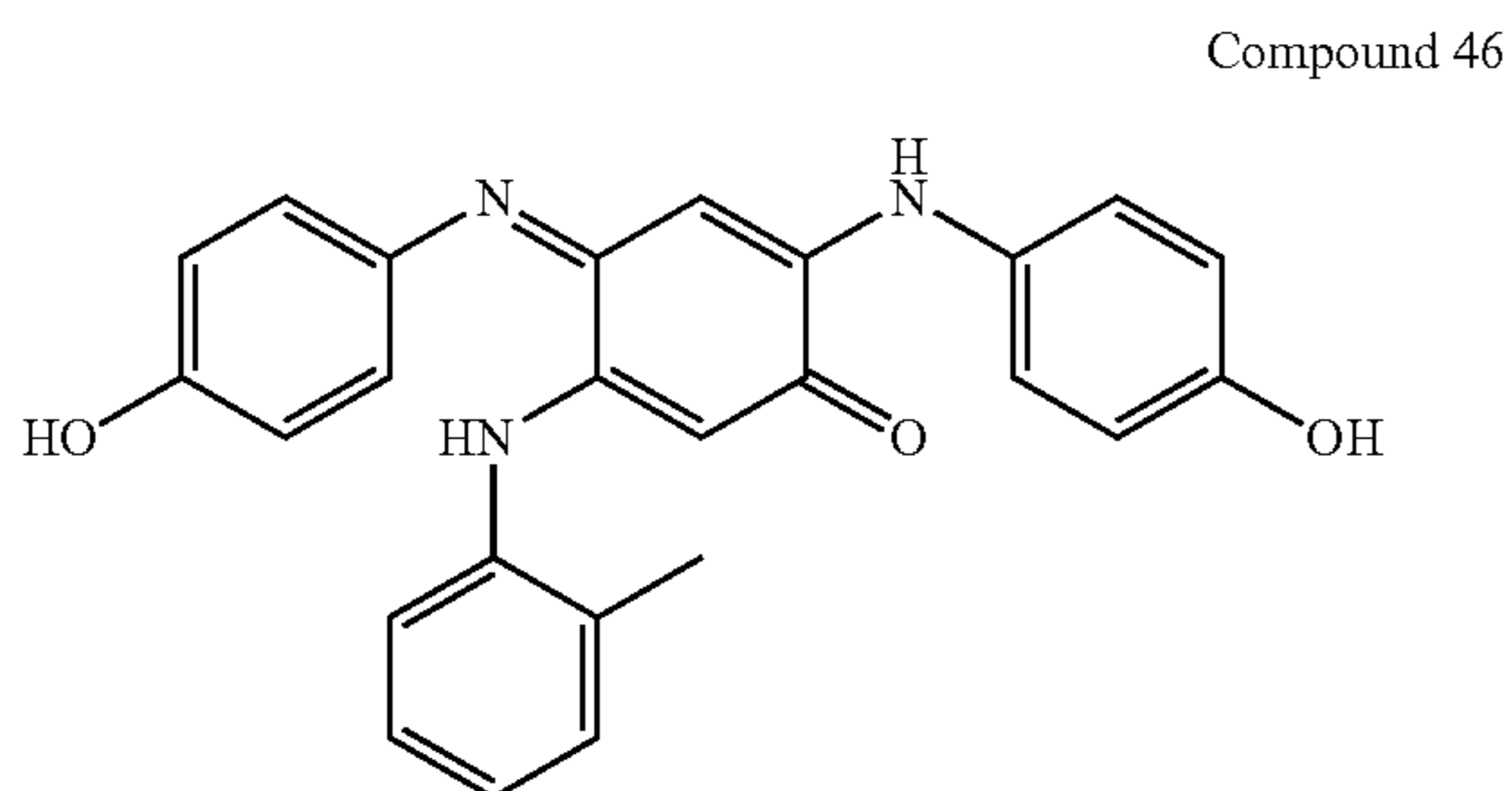
Compound 46 2-(4-Hydroxy-phenylamino)-4-(4-hydroxyphenylimino)-5-o-tolylamino-cyclohexa-2,5-dienone
