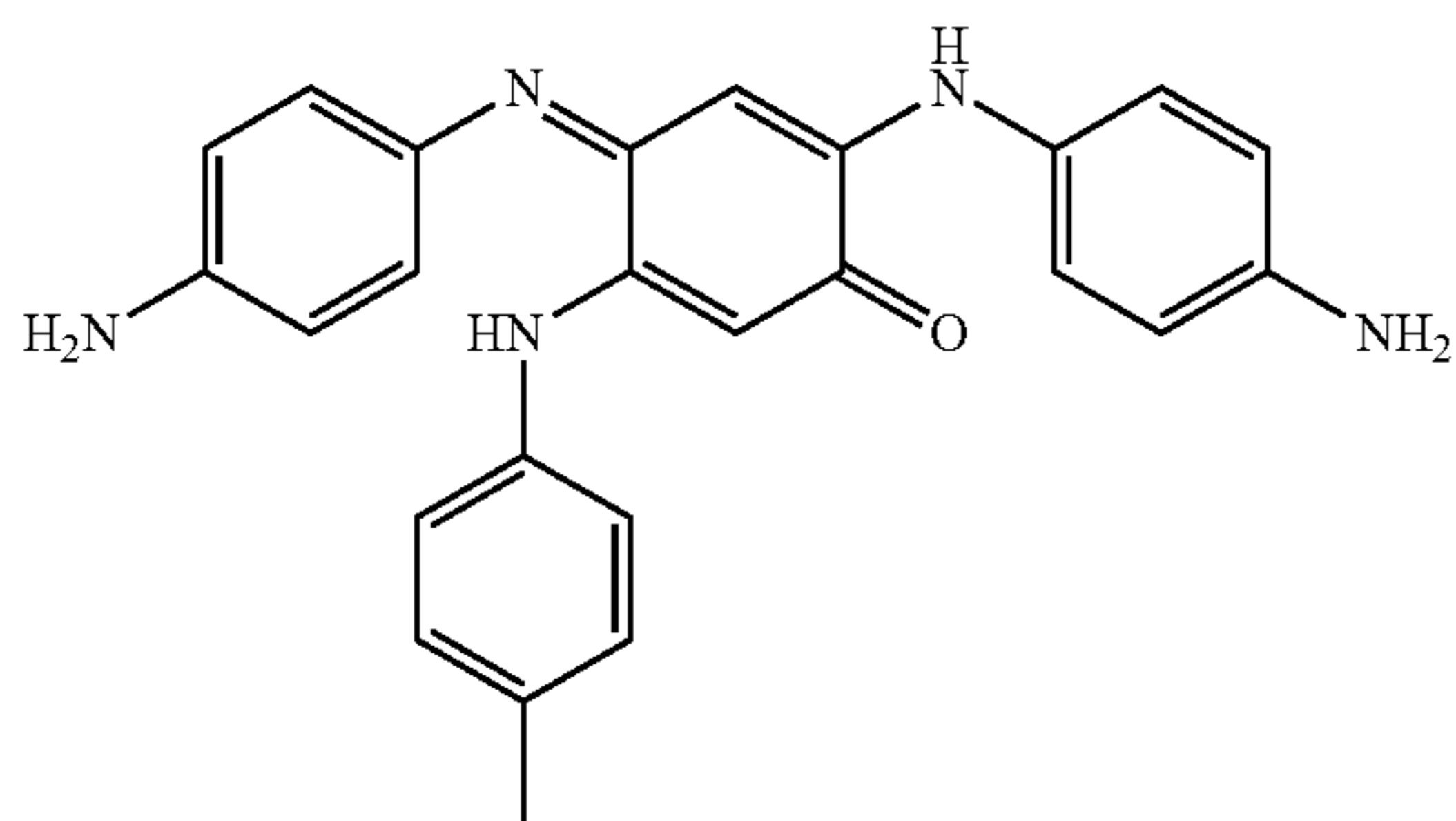
2-(4-Aminophenylamino)-4-(4-amino-phenylimino)-5-p-tolylaminocyclohexa-2,5-dienone
