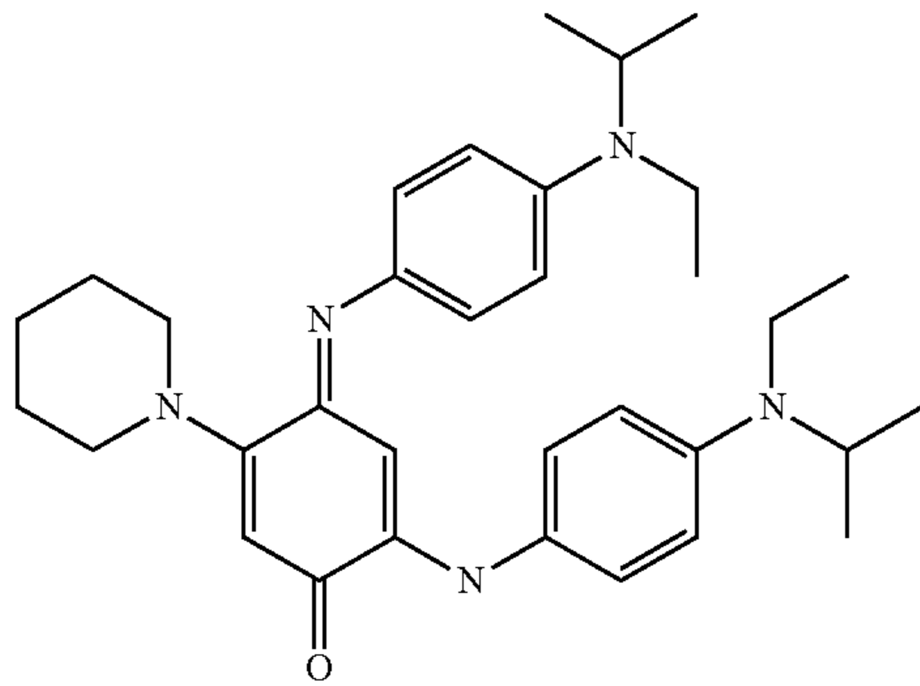
2-[4-(Ethylisopropyl-amino)phenyl-amino]-4-[4-(ethyl-isopropylamino)-phenylimino]-5-piperidin-1-ylcyclohexa-2,5-dienone
