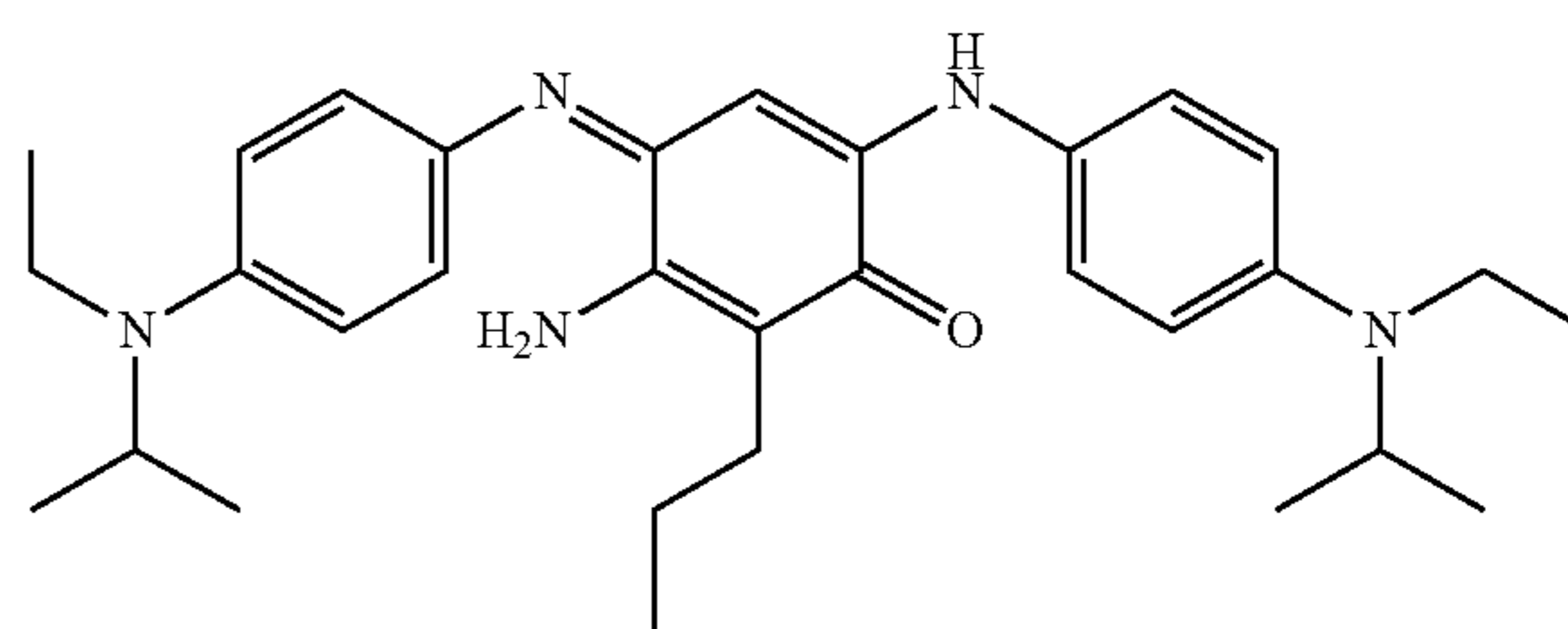
3-Amino-6-[4-(ethyl-isopropylamino)-phenylamino]-4-[4-ethyl-isopropylamino)-phenylimino]-2-propyl-cyclohexa-2,5-dienone
