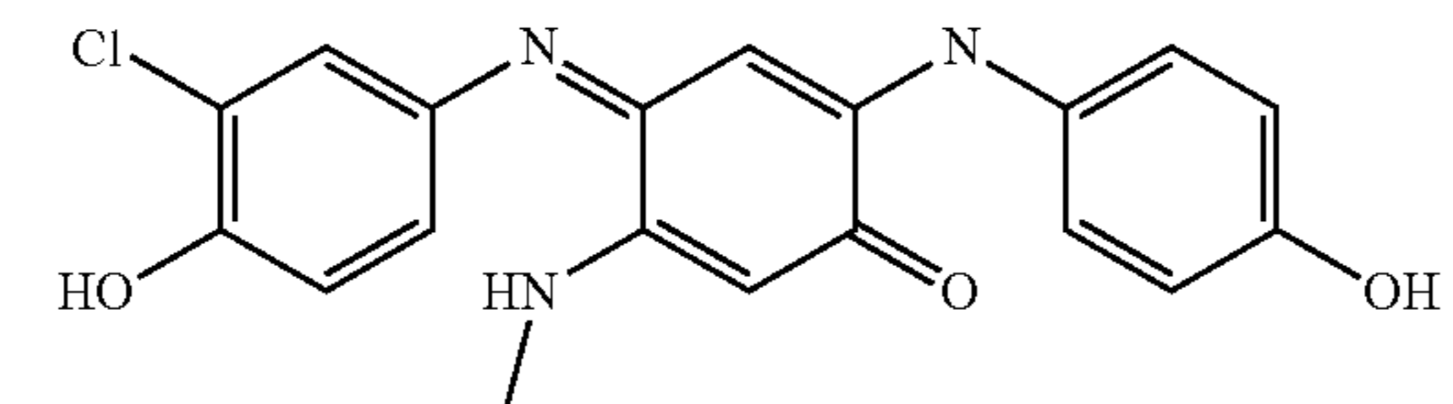
4-(3-Chloro-4-hydroxy-phenylimino)-2-(4-hydroxyphenylamino)-5-methylaminocyclohexa-2,5-dienone
