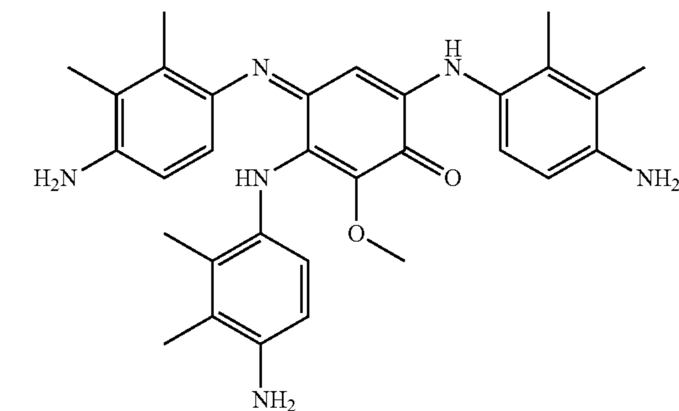
3,6-Bis(4-amino-2,3-dimethylphenylamino)-4-(4-amino-2,3-dimethylphenylimino)-2-methoxy-cyclohexa-2,5-dienone
