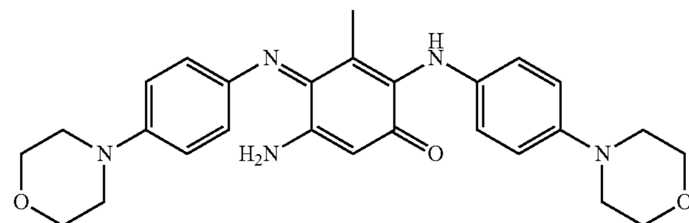
5-Amino-3-methyl-2-(4-morpholin-4-ylphenylamino)-4-[4-morpholin-4-ylphenylimino]cyclohexa-2,4-dienone
