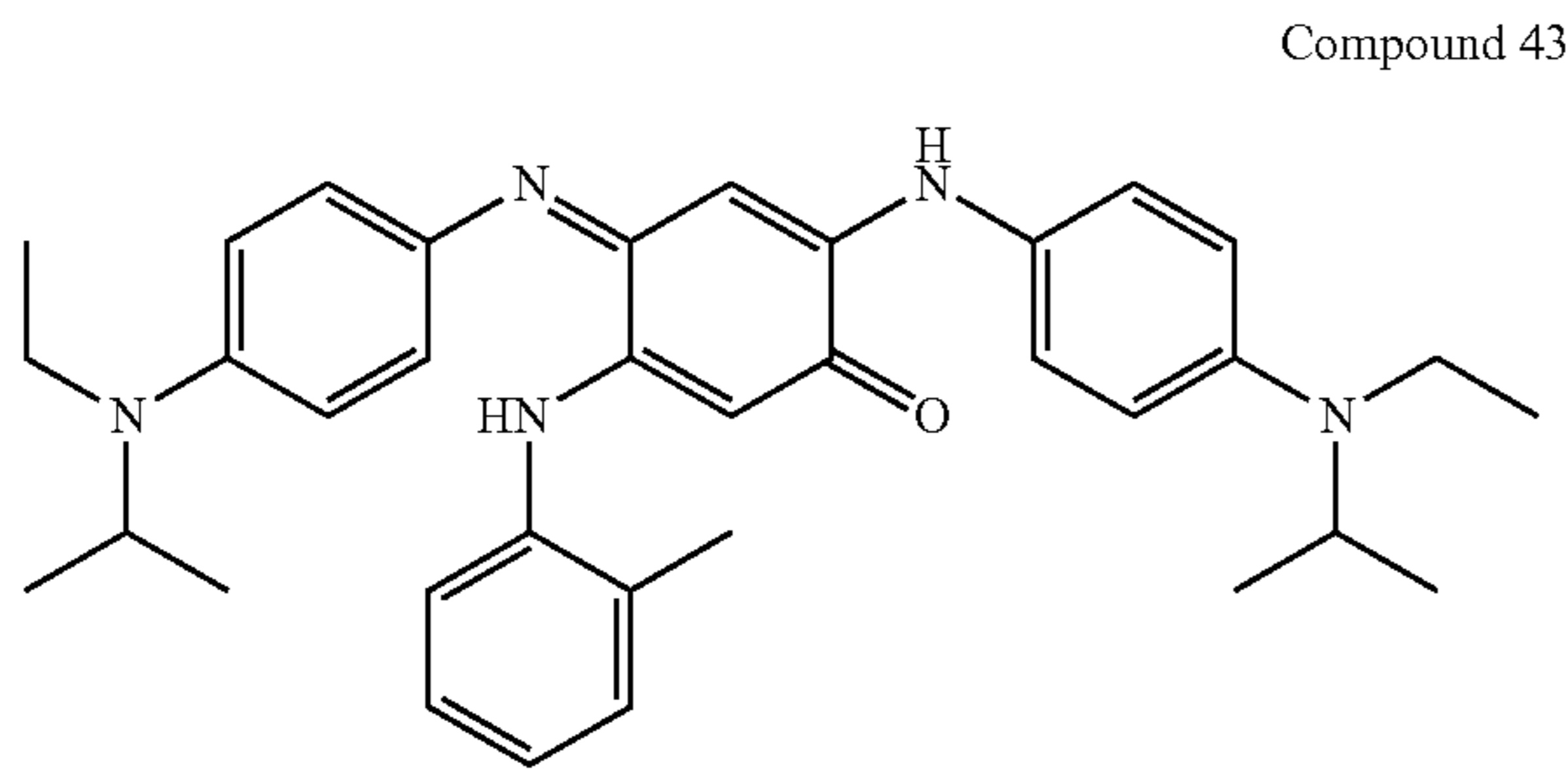
Compound 43 2-[4-(Ethylisopropyl-amino)phenyl-amino]-4-[4-ethyl-isopropylamino)-phenylimino]-5-o-tolyaminocyclohexa-2,5-dienone
