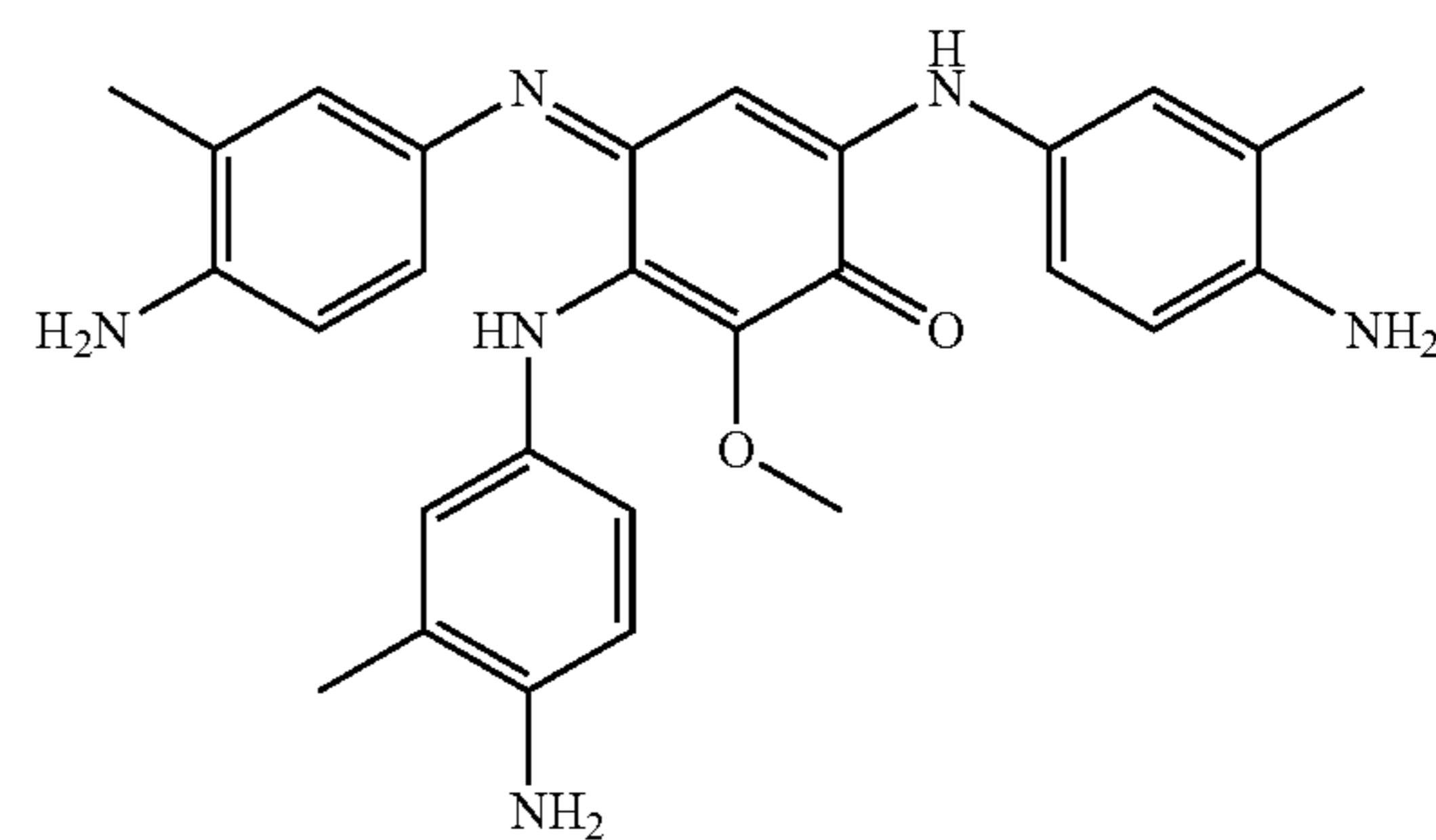
3,6-Bis(4-amino-3-methyl-phenylamino)-4-(4-amino-3-methylphenylimino)-2-methoxycyclohexa-2,5-dienone
