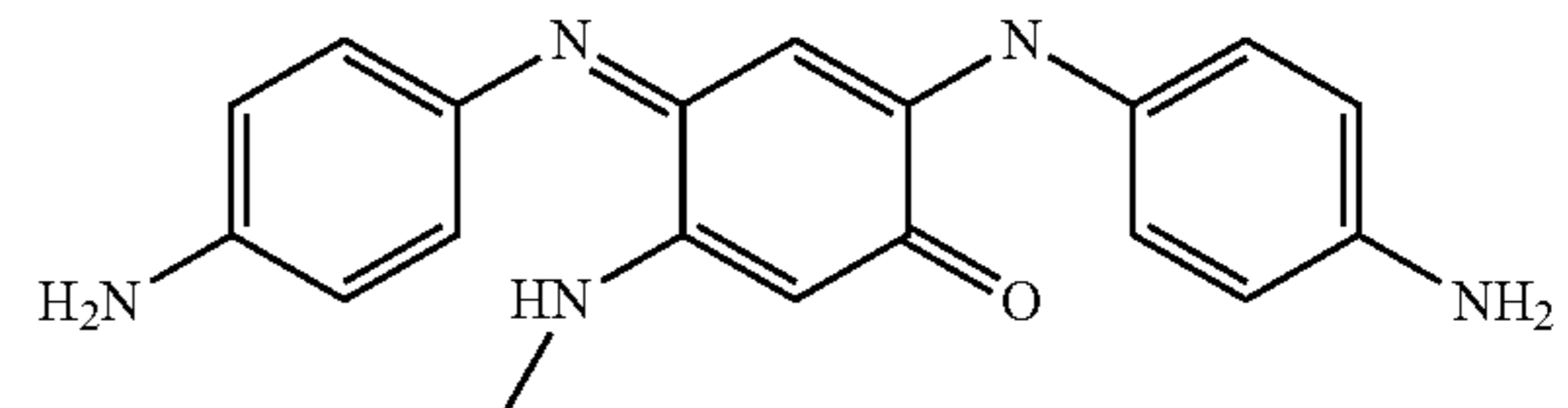
2-(4-Aminophenylamino)-4-(4-amino-phenylimino)-5-methylaminocyclohexa-2,5-dienone
