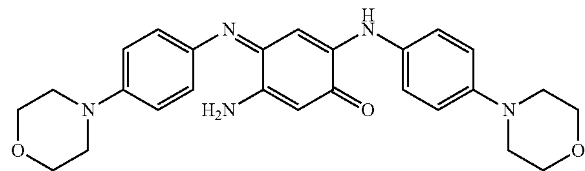
Compound 50 5-Amino-2-(4-morpholin-4-ylphenylamino)-4-[4-morpholin-4-yl-phenylimino]cyclohexa-2,5-dienone
