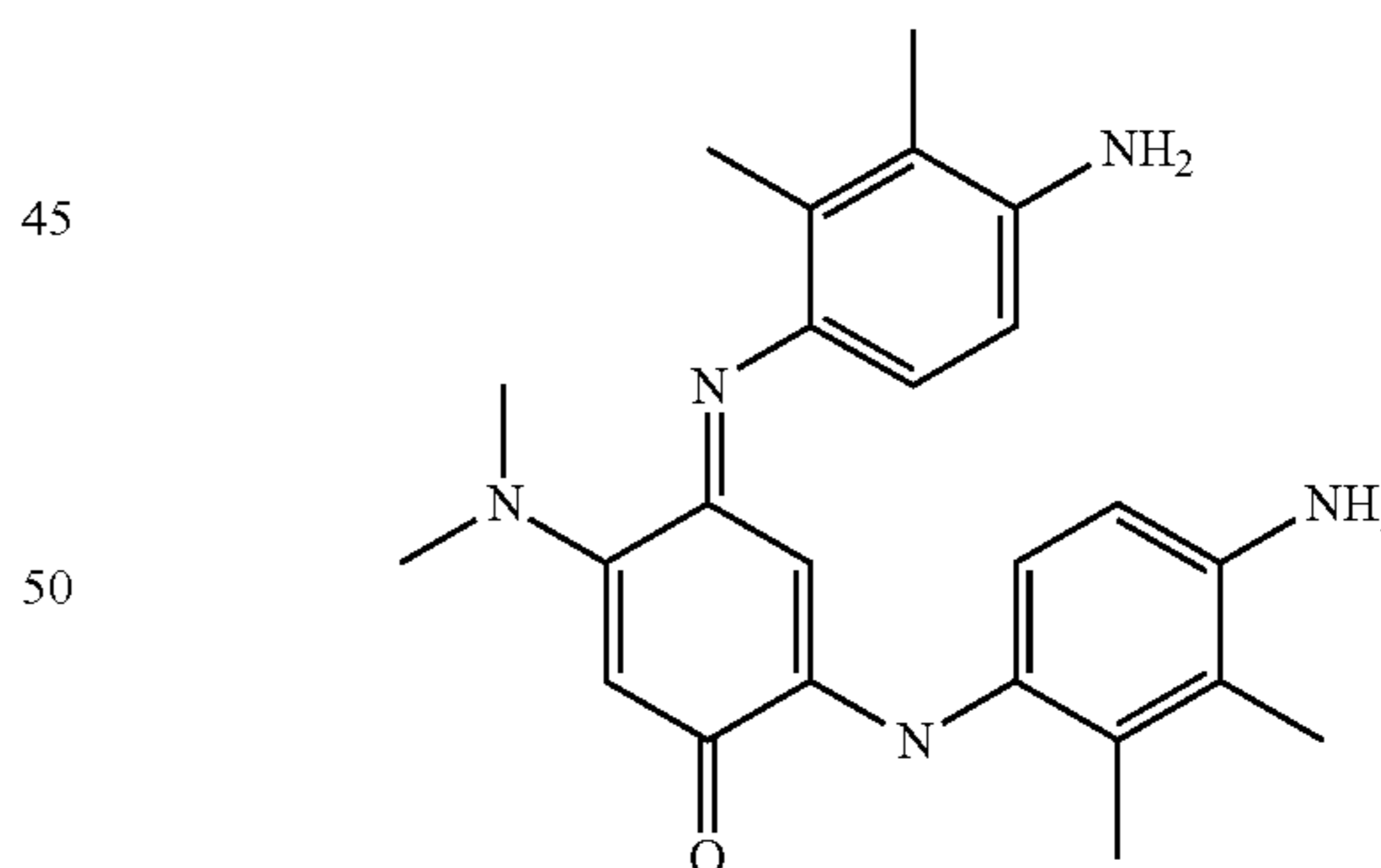
2-(4-Amino-2,3-dimethyl-phenylamino)-4-(4-amino-2,3-dimethylphenylimino)-5-dimethylaminocyclohexa-2,5-dienone
