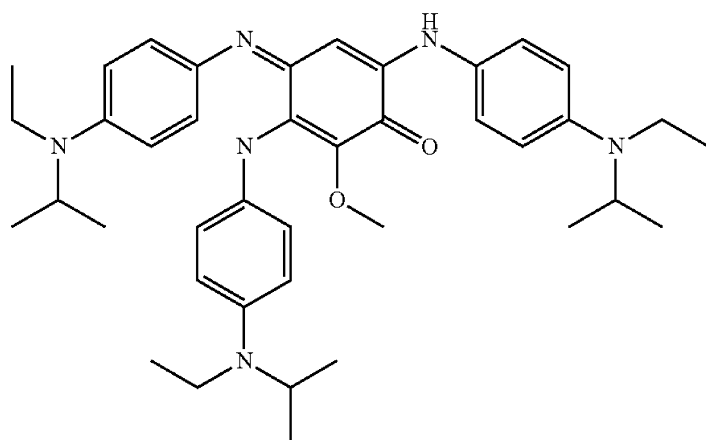
3,6-Bis[4-(ethylisopropyl-amino)-phenylamino]-4-[4-(ethylisopropyl-amino)phenylimino]-2-methoxycyclohexa-2,5-dienone
