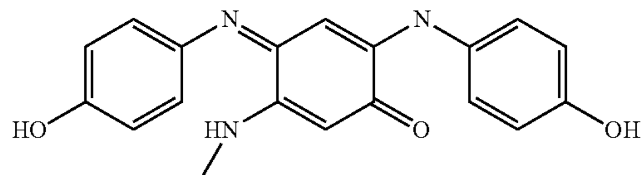
2-(4-Hydroxyphenylamino)-4-(4-hydroxyphenylimino)-5-methylaminocyclohexa-2,5-dienone
