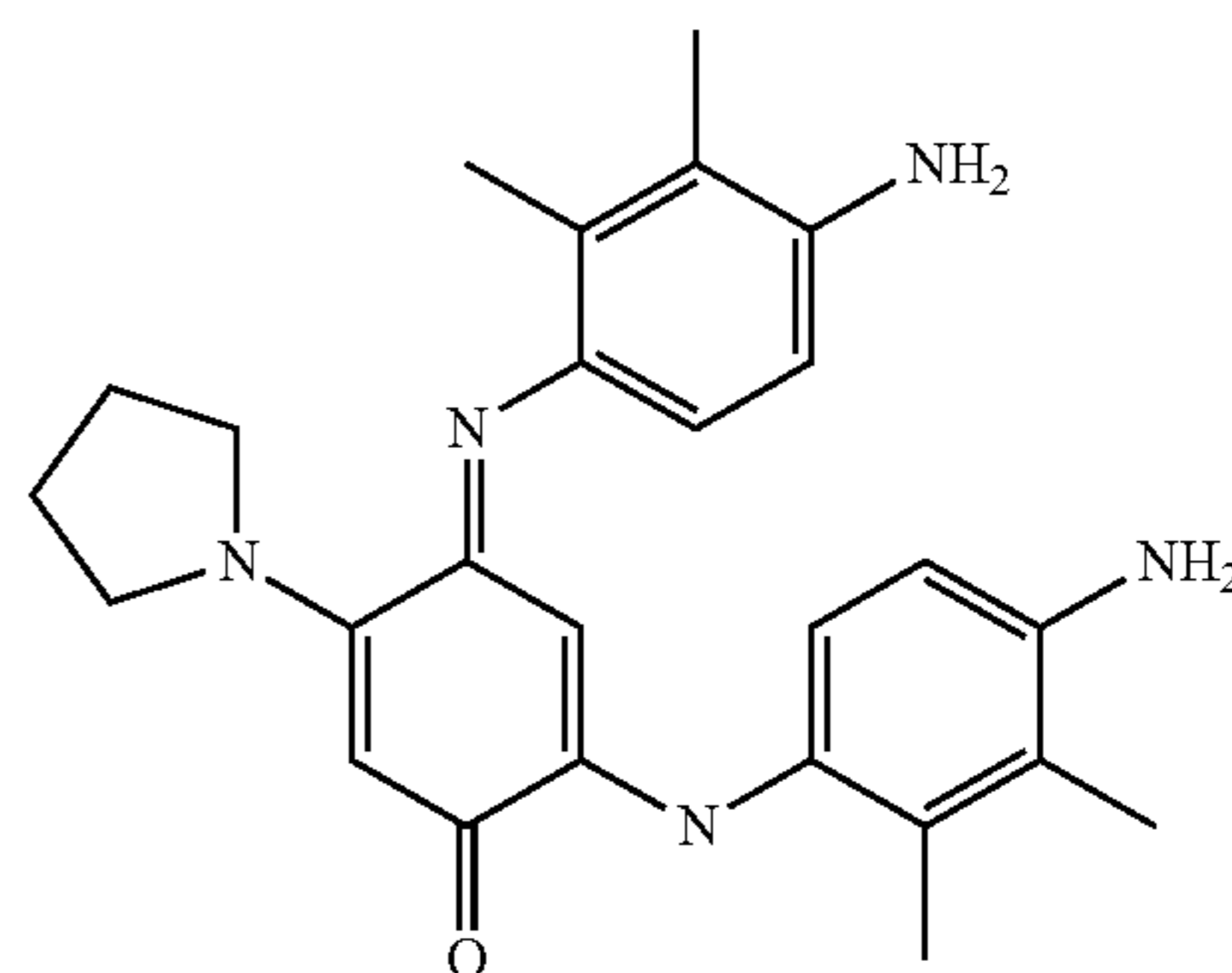
2-(4-Amino-2,3-dimethyl-phenylamino)-4-(4-amino-2,3-diethylphenylimino)-5-pyrrolidin-1-ylcyclohexa-2,5-dienone
