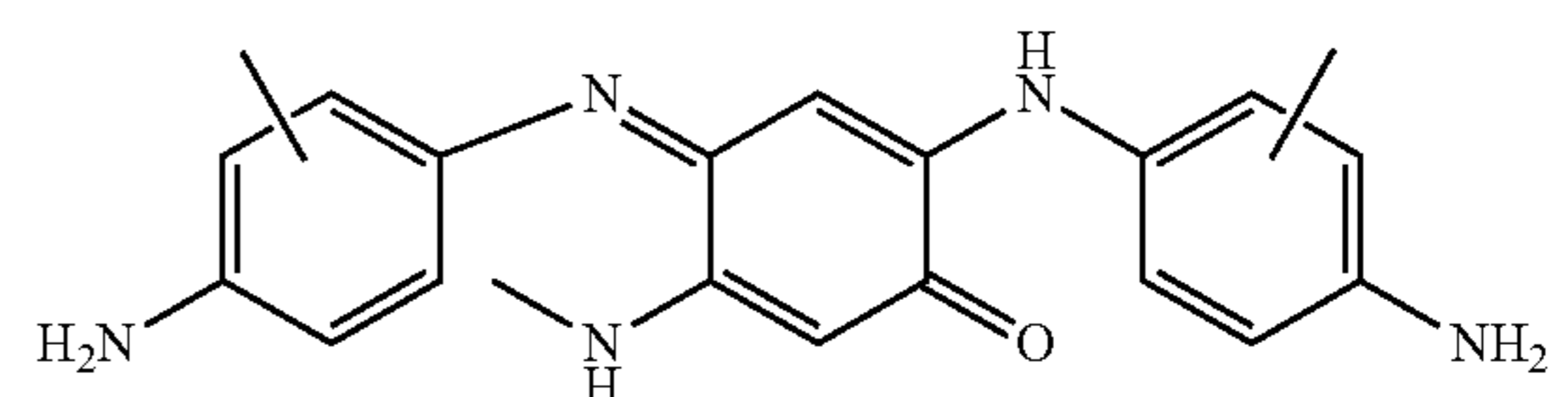
2-(4-Amino-3(or 2)-methyl-phenylamino)-4-(4-amino-3-methylphenylimino)-5-methylaminocyclohexa-2,5-dienone
