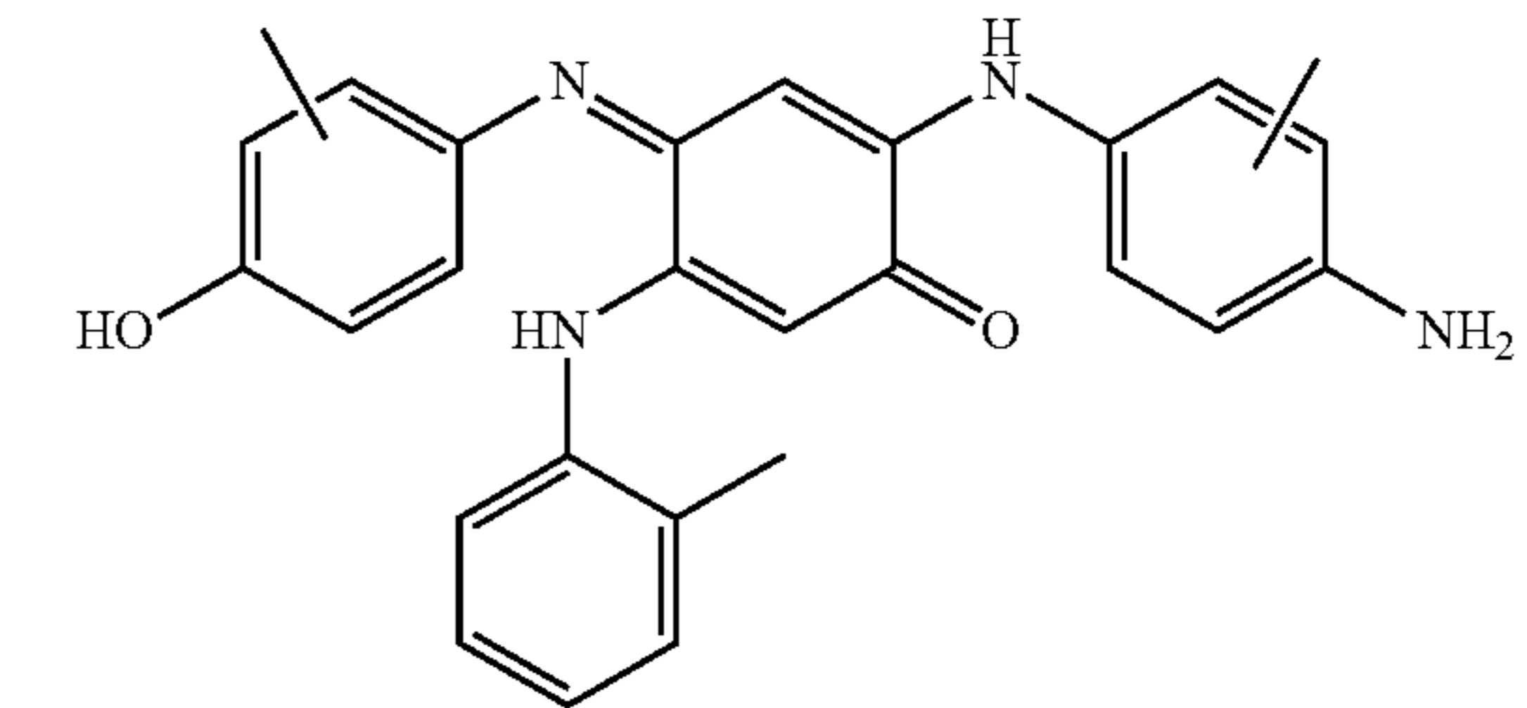
Compound 49 2-(4-Amino-3(or 2)-methylphenylamino)-4-(4-amino-3(or 2)-methyl-phenylimino)-5-o-tolylaminocyclohexa-2,5-dienone
