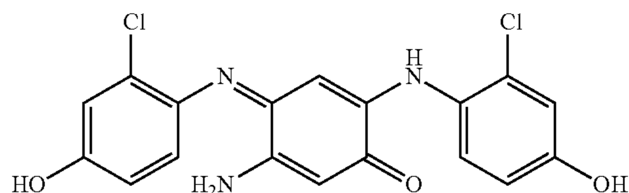
5-Amino-2-(2-chloro-4-hydroxyphenylamino)-4-[2-chloro-4-hydroxyphenylimino]cyclohexa-2,5-dienone
