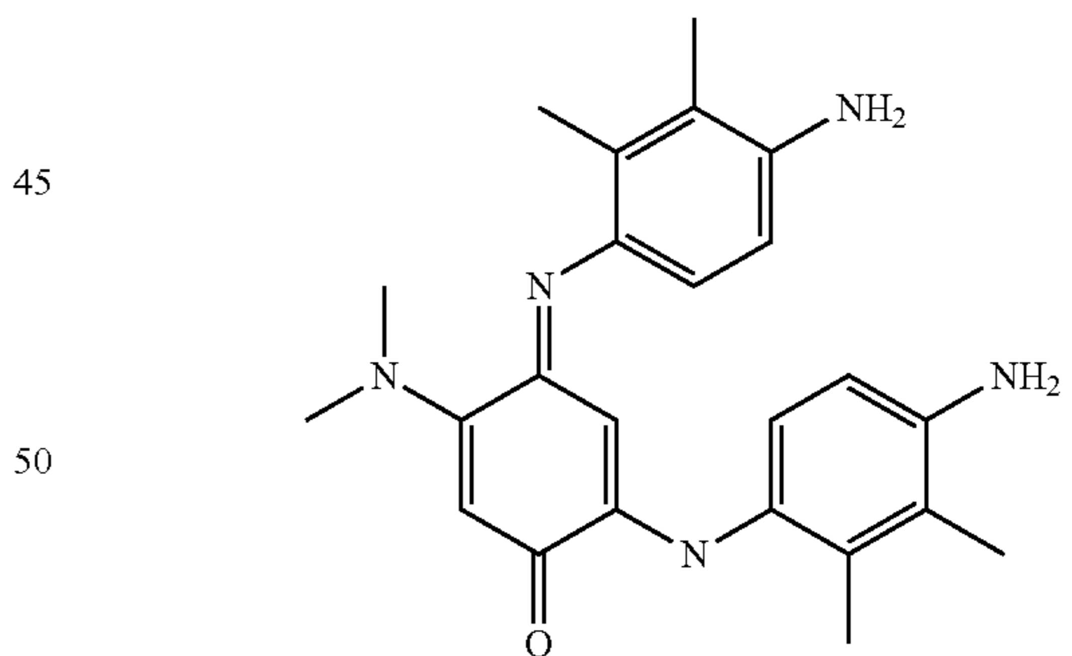
2-(4-Amino-2,3-dimethyl-phenylamino)-4-(4-amino-2,3-dimethylphenylimino)-5-dimethylamino-cyclohexa-2,5-dienone
