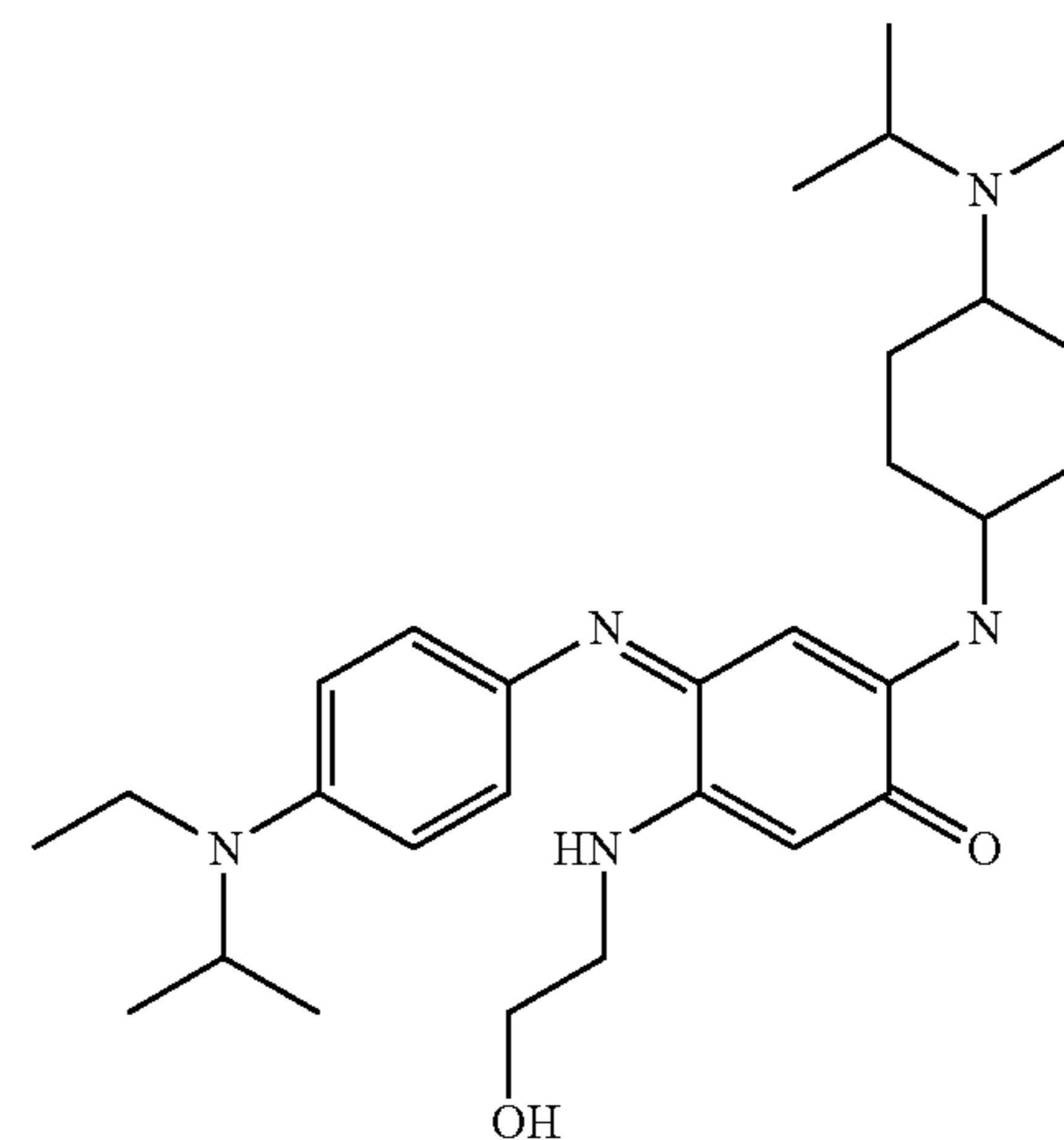
2-[4-(Ethylisopropyl-amino)phenyl-amino]-4-[4-(ethyl-isopropylamino)-phenylimino]-5-(2-hydroxyethylamino)-cyclohexa-2,5-dienone
