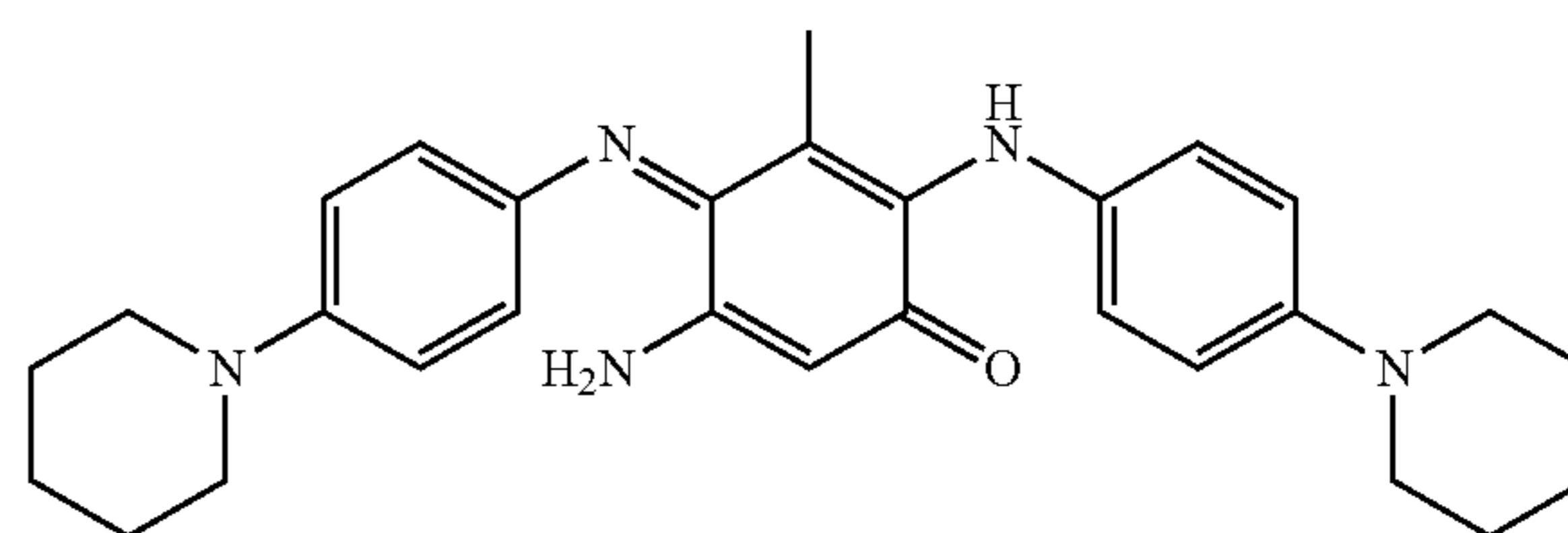
5-Amino-3-methyl-2-(4-piperidin-1-yl-phenylamino)-4-[4-piperidin-1-ylphenylimino]cyclohexa-2,5-dienone
