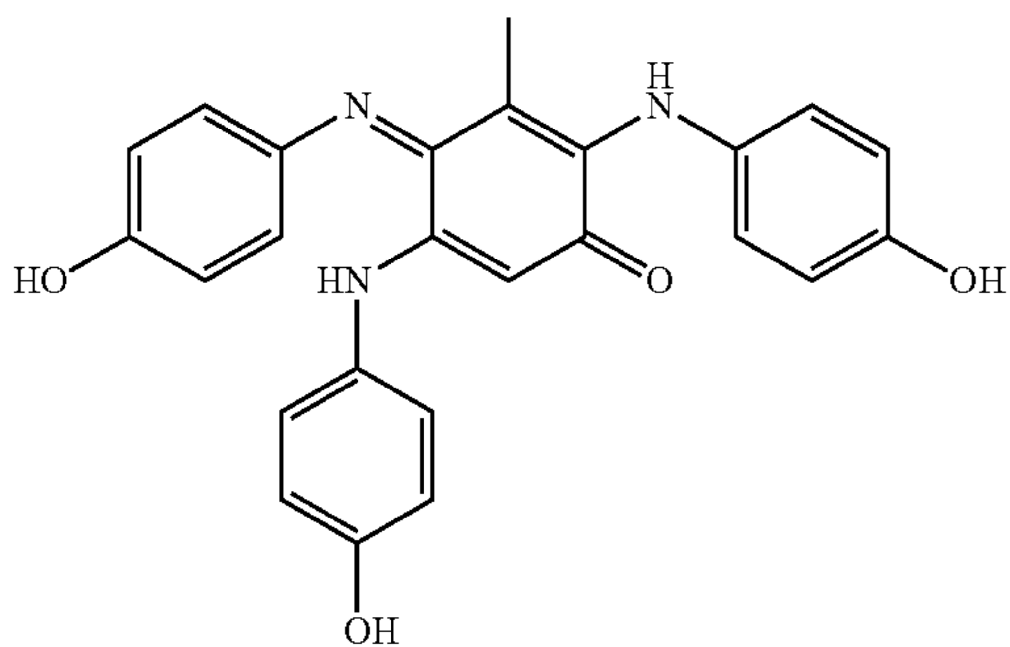
2,5-Bis(4-hydroxy-phenylamino)-4-(4-hydroxyphenylimino)-3-methylcyclohexa-2,5-dienone
