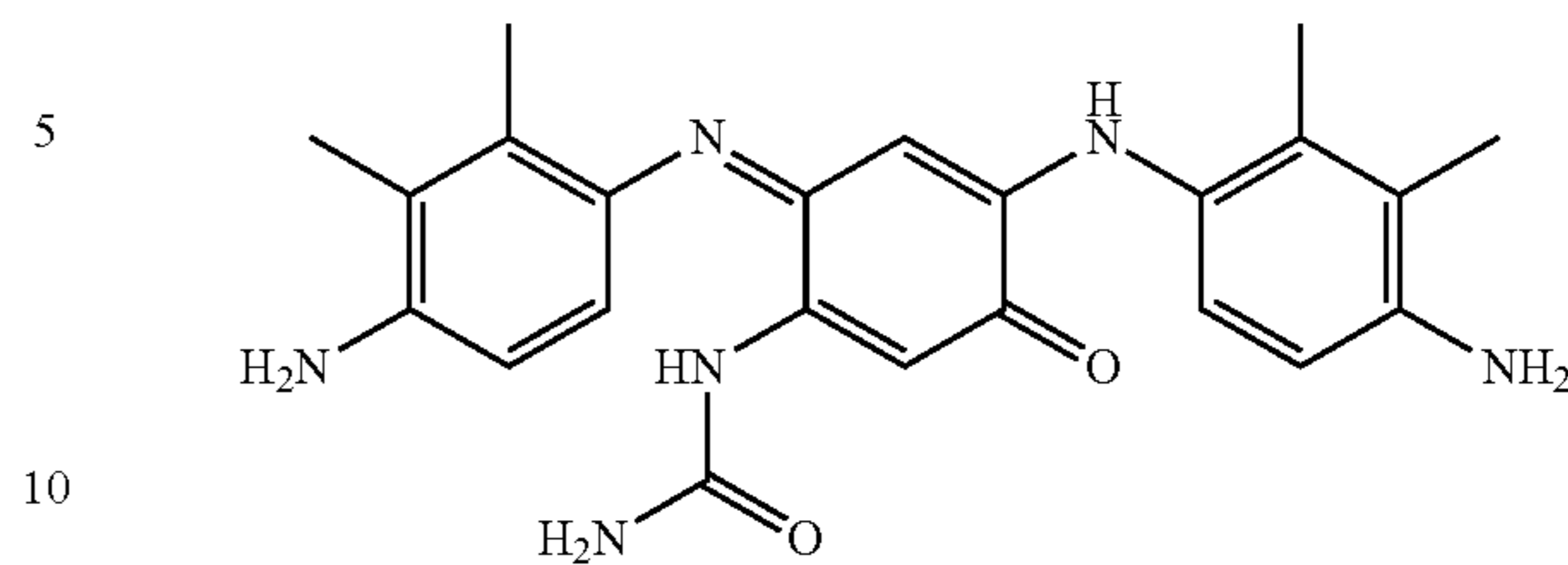
[4-(4-Amino-2,3-dimethyl-phenylamino)-6-(4-amino-2,3-dimethylphenylimino)-3-oxocyclohexa-1,4-dienyl]-urea
