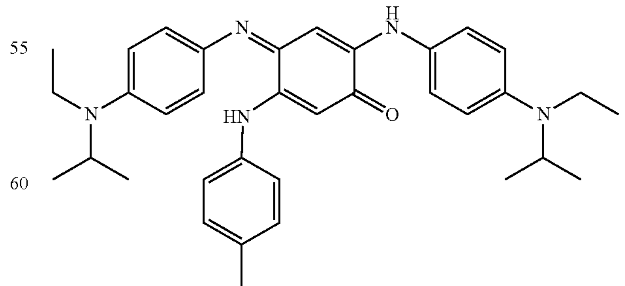
Compound 51 2-[4-(Ethylisopropyl-amino)phenyl-amino]-4-[4-(ethylisopropylamino)-phenylimino]-5-p-tolyaminocyclohexa-2,5-dienone
