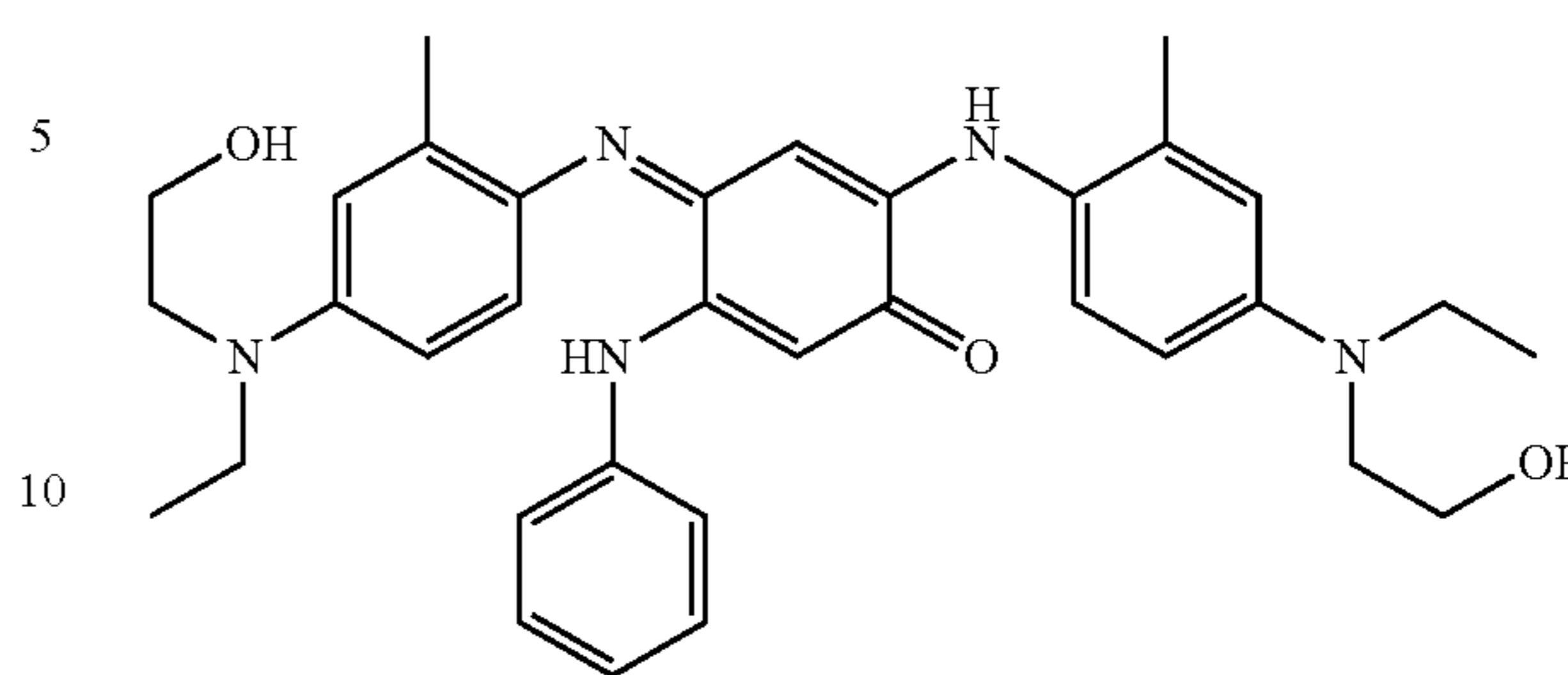
2-{4-[ethyl-(2-hydroxy-ethyl)amino]-2-methyl-phenylamino}-4-{4-[ethyl-(2-hydroxyethyl)amino]-2-methyl-phenylimino}-5-phenylaminocyclohexa-2,5-dienone
