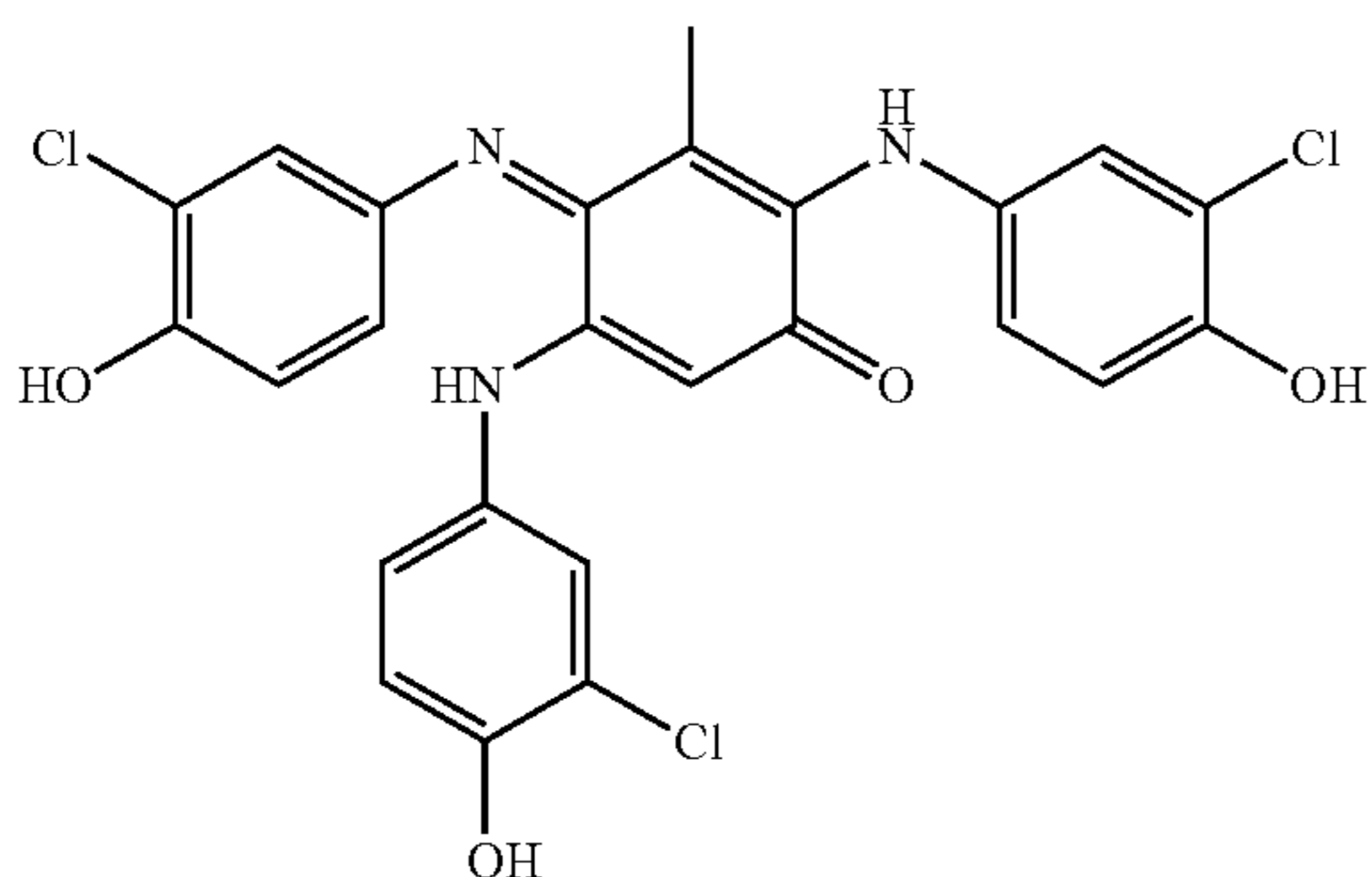
2,5-Bis(3-chloro-4-hydroxy-phenylamino)-4-(3-chloro-4-hydroxyphenylimino)-3-methylcyclohexa-2,5-dienone
