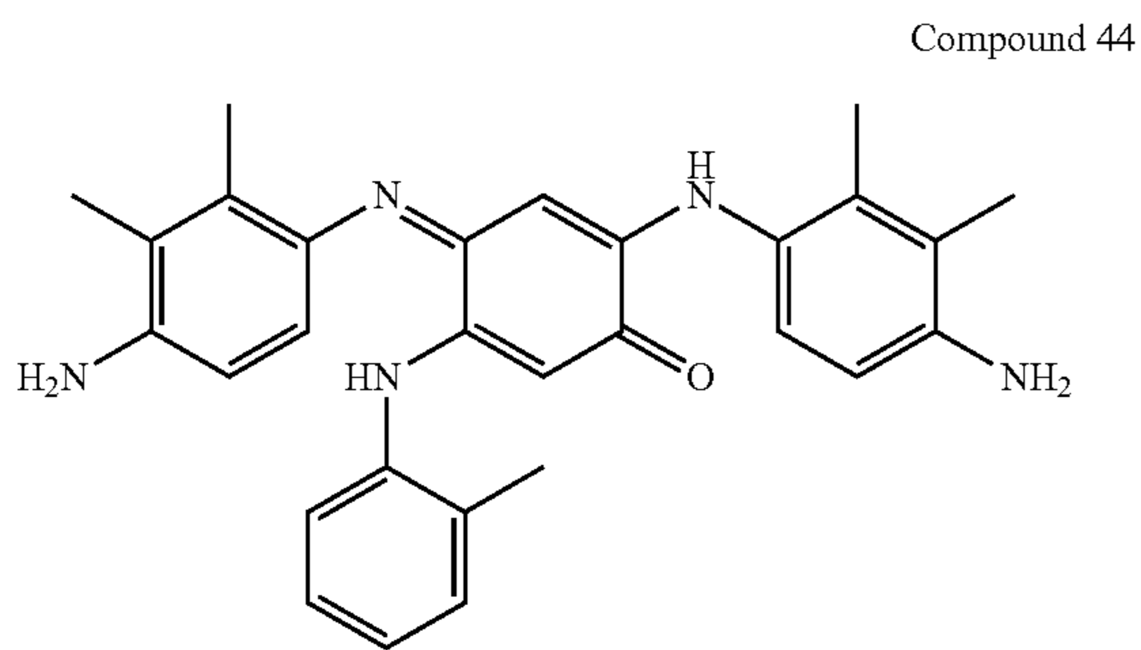
Compound 44 2-(4-Amino-2,3-dimethylphenylamino)-4-(4-amino-2,3-dimethylphenylimino)-5-o-tolylaminocyclohexa-2,5-dienone
