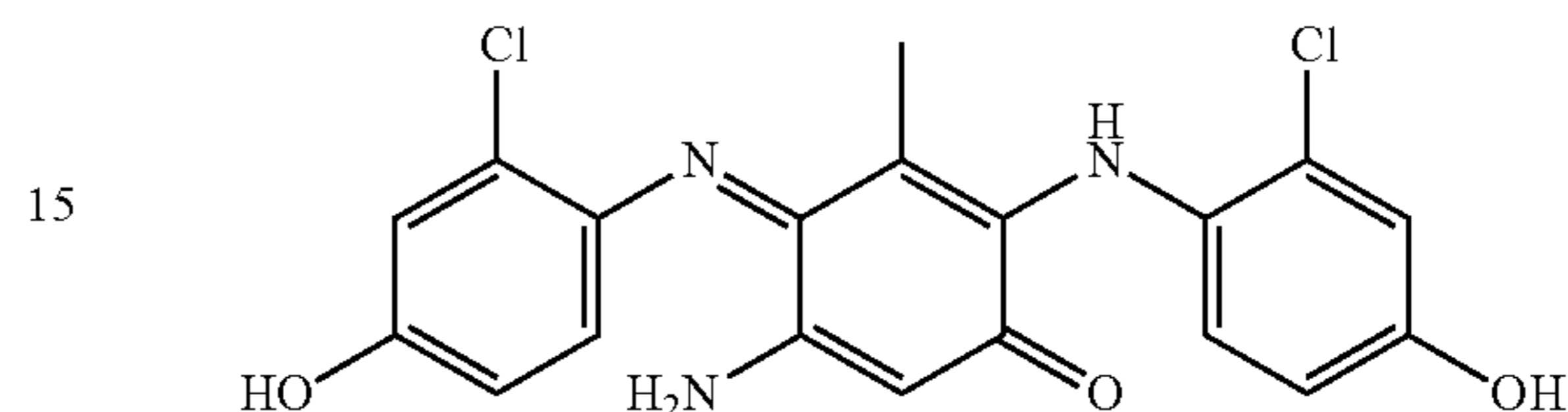
5-Amino-2-(2-chloro-4-hydroxyphenylamino)-4-(2-chloro-4-hydroxy-phenylimino)-3-methyl-cyclohexa-2,5-dienone
