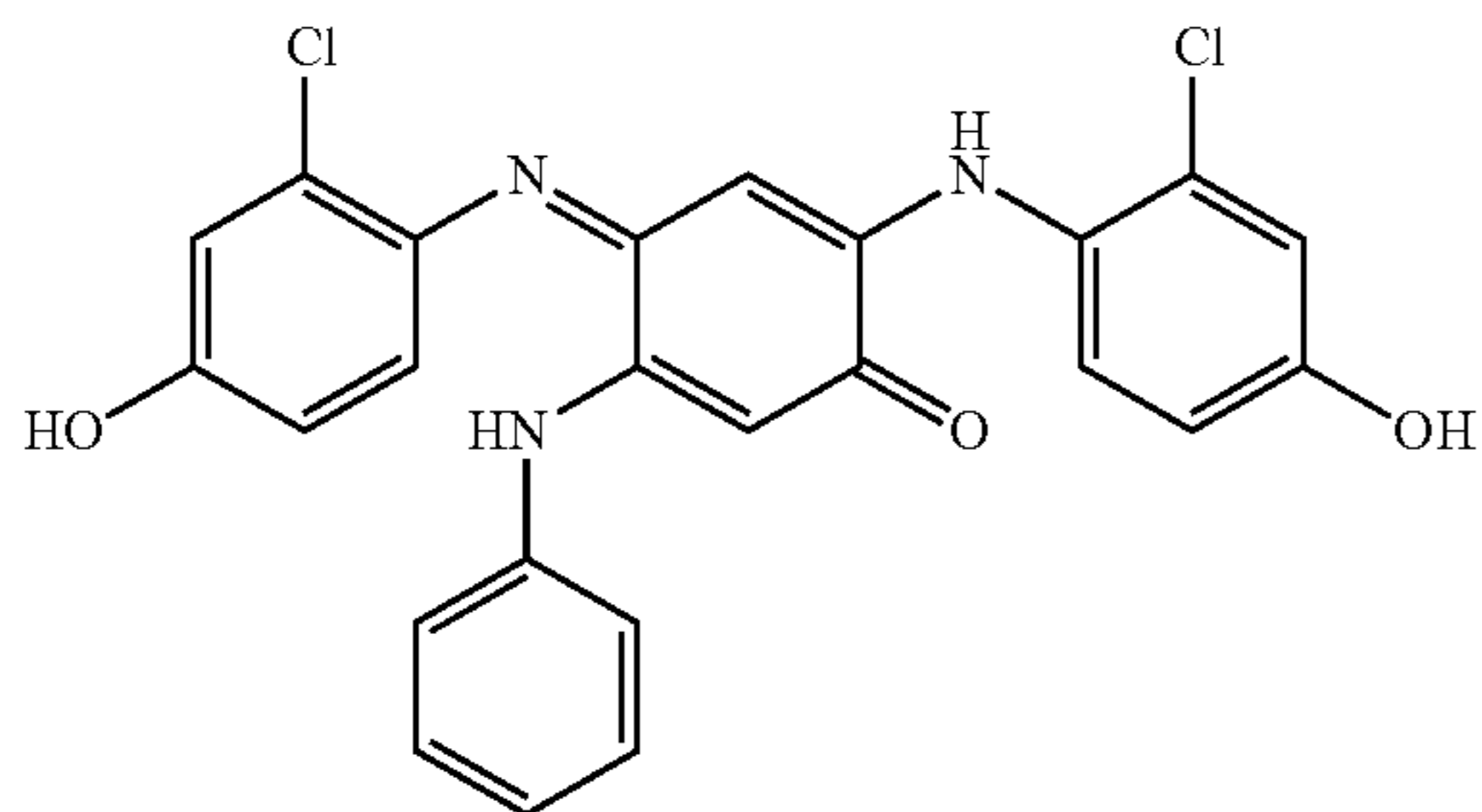
2-(2-Chloro-4-hydroxy-phenylamino)-4-(2-chloro-4-hydroxy-phenylimino)-5-phenylaminocyclohexa-2,5-dienone
