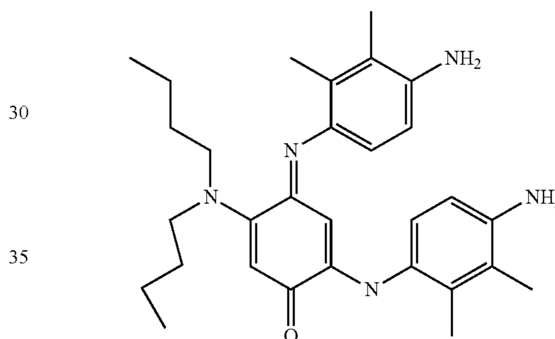
2-(4-Amino-2,3-dimethyl-phenylamino)-4-(4-amino-2,3-dimethylphenylimino)-5-dibutylaminocyclohexa-2,5-dienone
