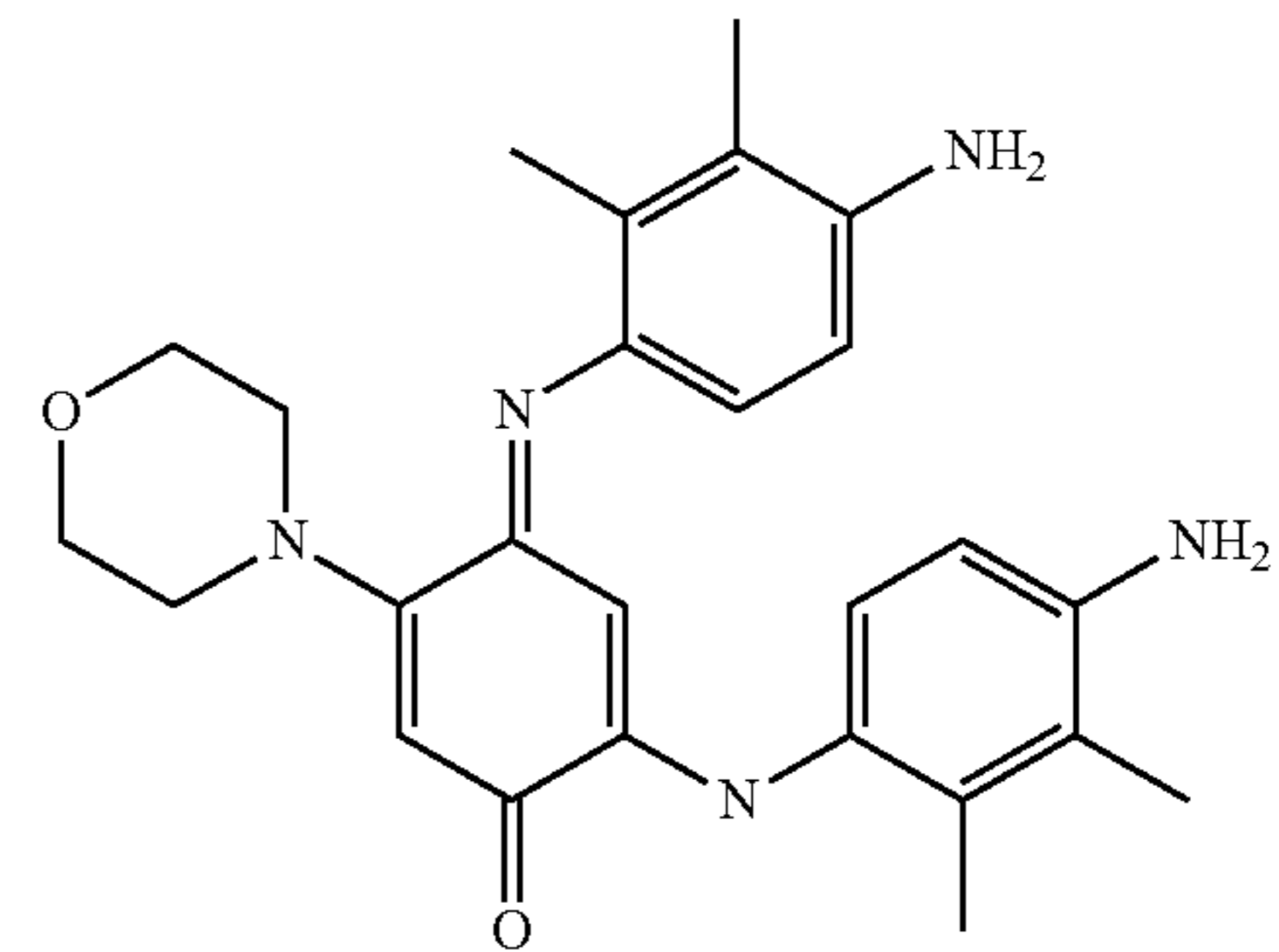
2-(4-Amino-2,3-dimethylphenylamino)-4-(4-amino-2,3-dimethylphenylimino)-5-morpholin-4-ylcyclohexa-2,5-dienone
