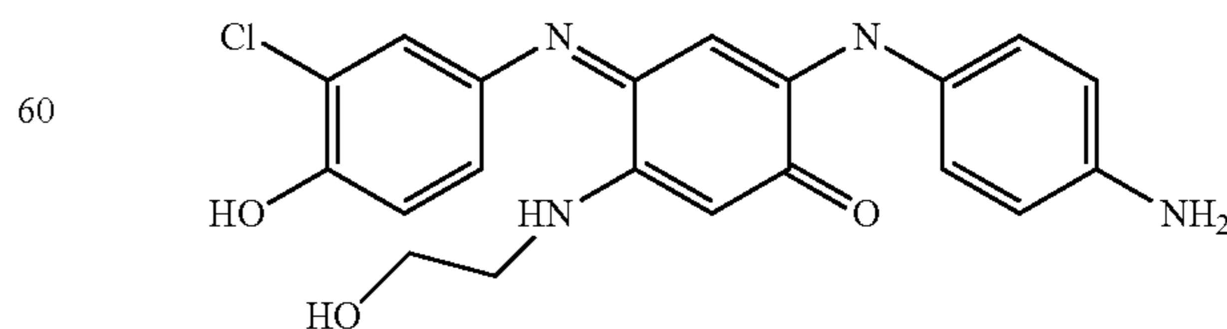
2-(4-Aminophenylamino)-4-(3-chloro-4-hydroxyphenylamino)-5-(2-hydroxyethylamino)-cyclohexa-2,5-dienone
