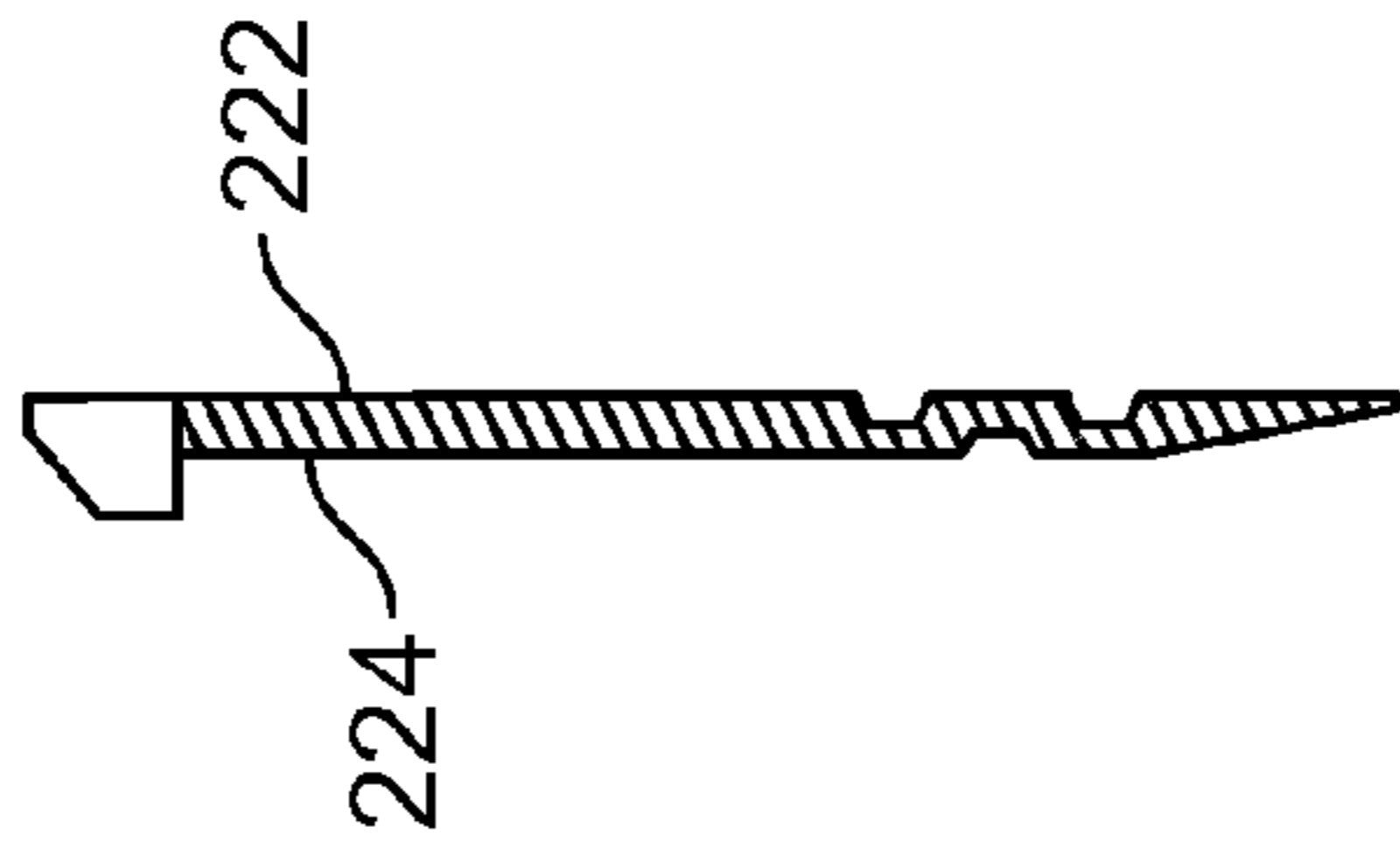
FIG. 8D (SECTION A1-A2)
