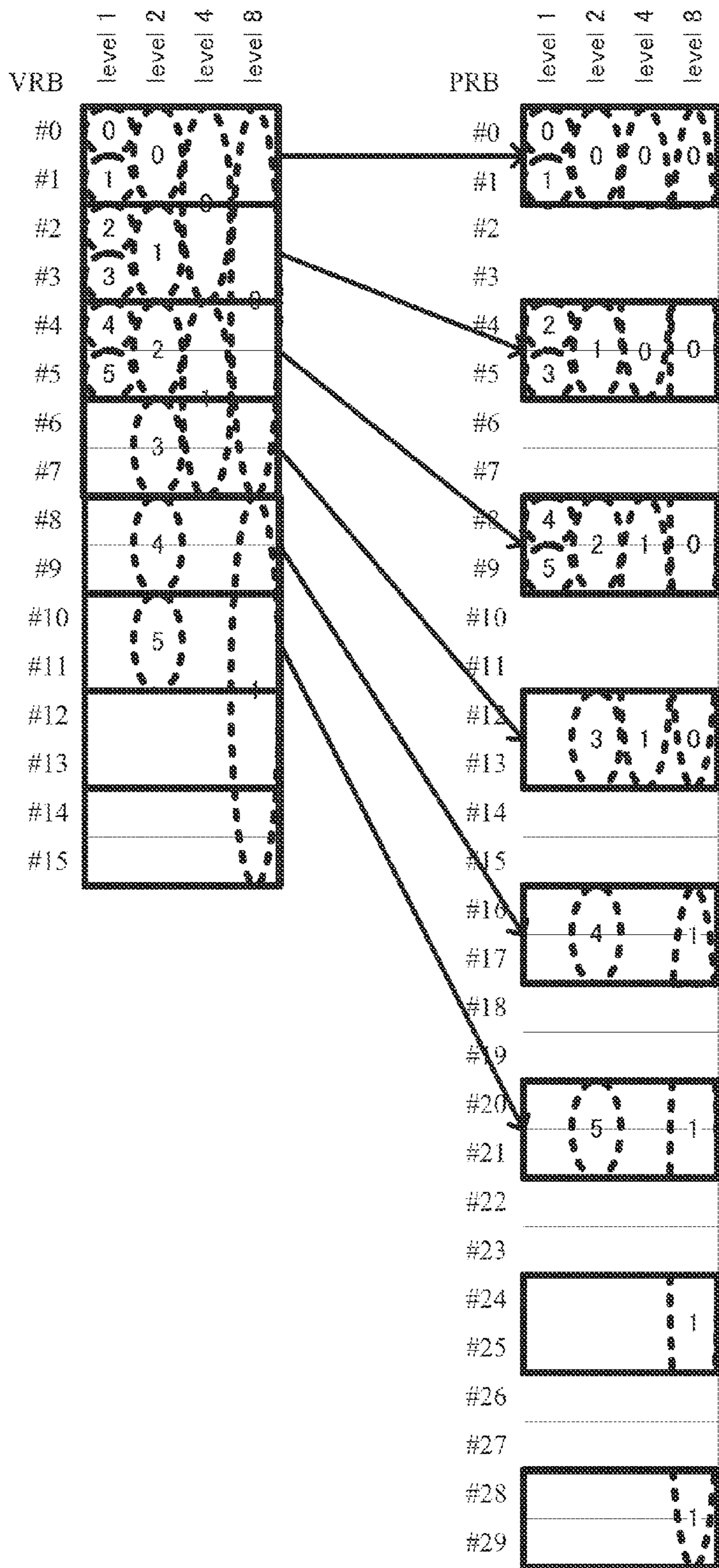
FIG. 2 (PRIOR ART)
