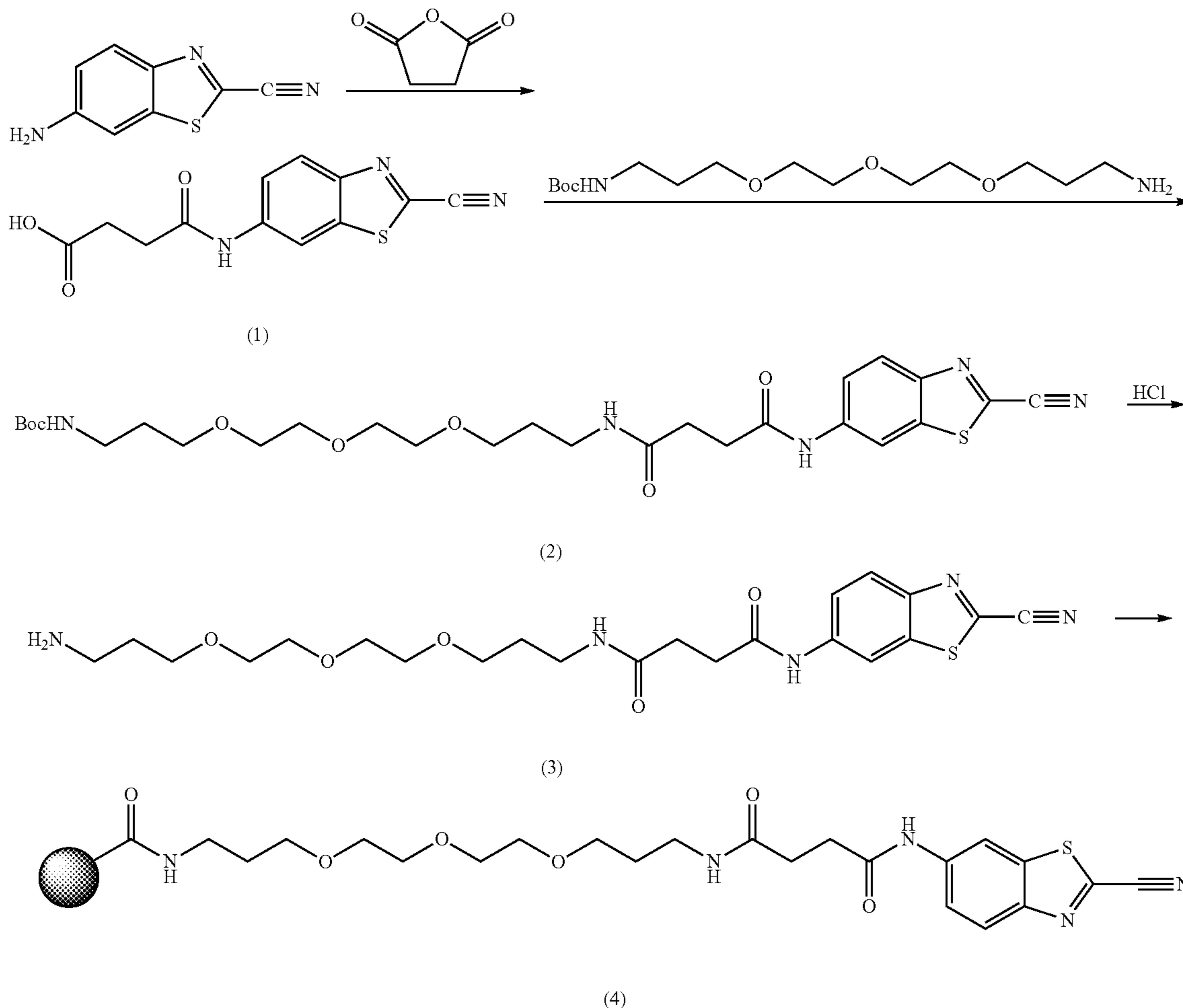
4-((2-cyanobenzo[d]thiazol-6-yl)amino)-4-oxobutanoic acid (1)
