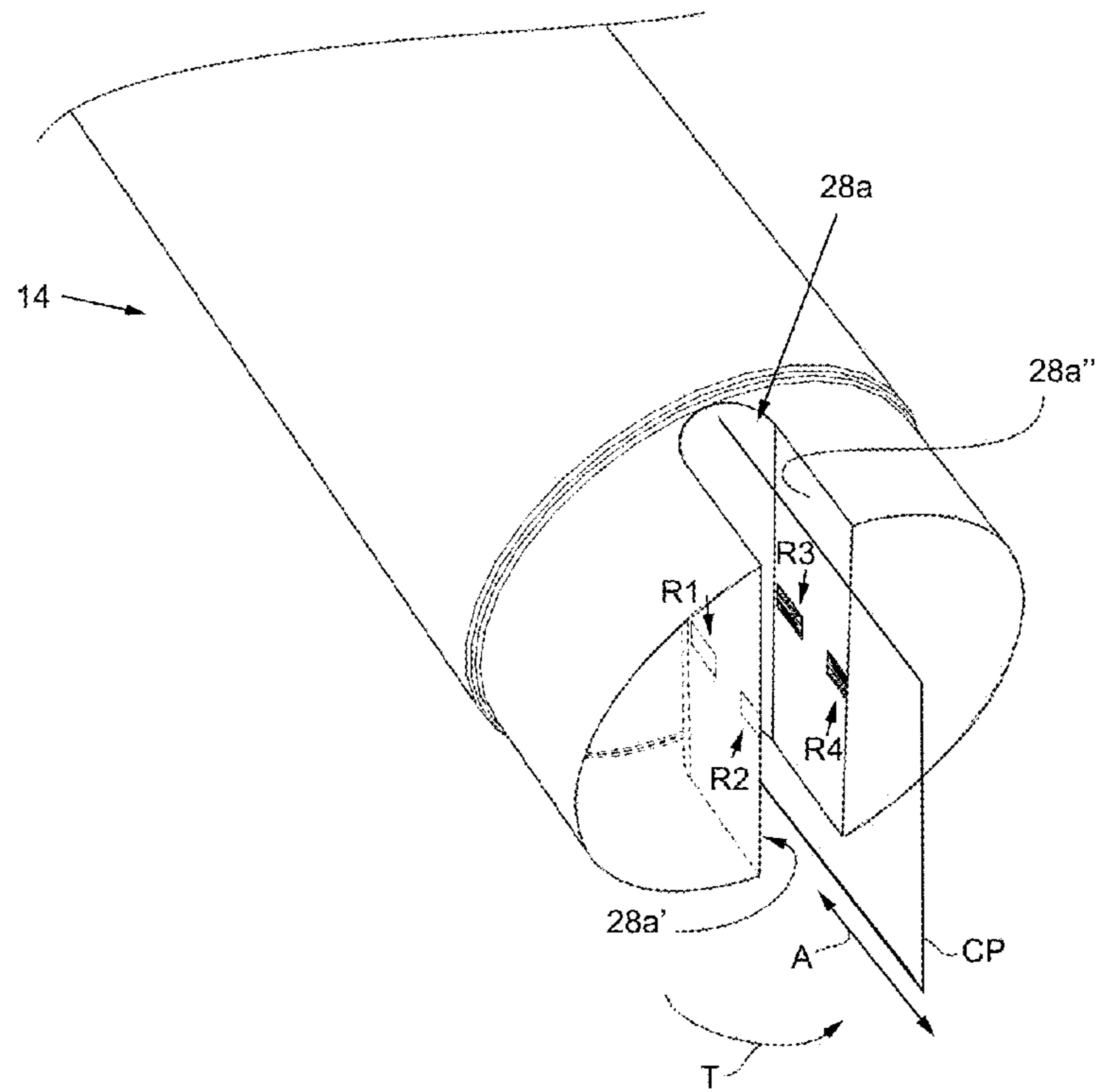
Fig. 11a - Torque (counter-clockwise)
