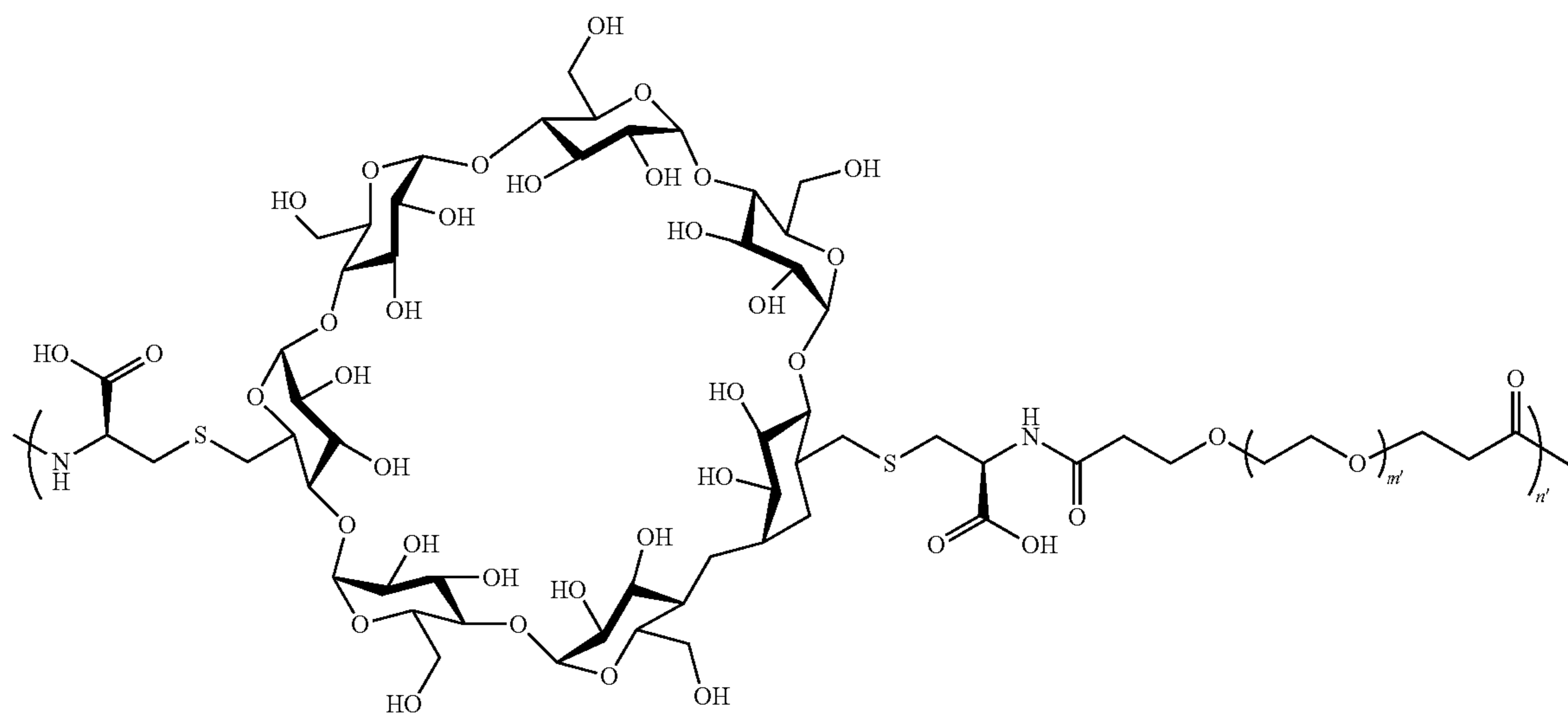
36a-f Poly(CDDCys-PA-PEG) Abbr: PA = propanoamide bond between PEG and CD
