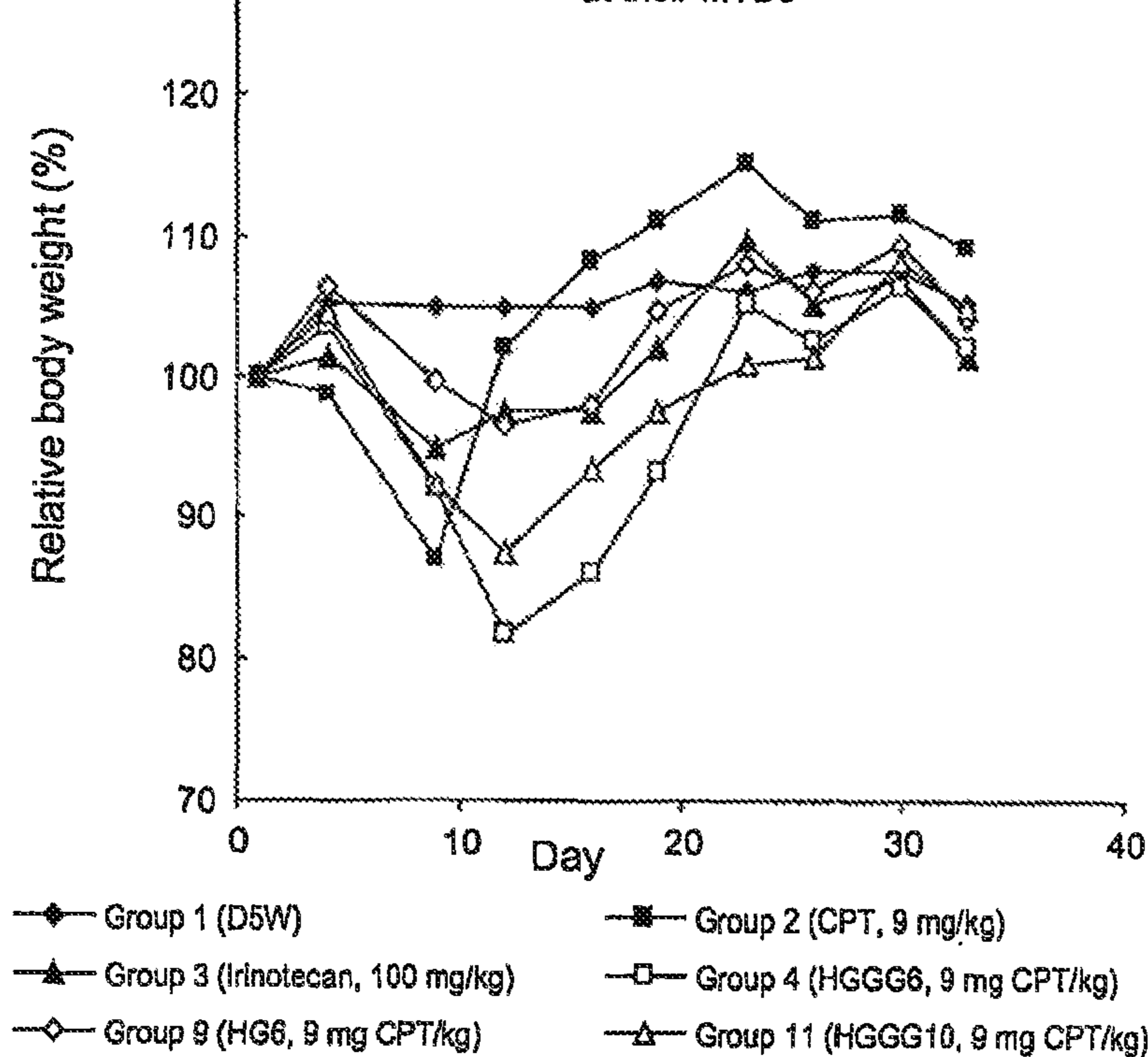
Mean body weight (MBW) losses as a function of time plotted for D5W, CPT, Irinotecan and the three conjugates containing high MW polymer at their MTDs
