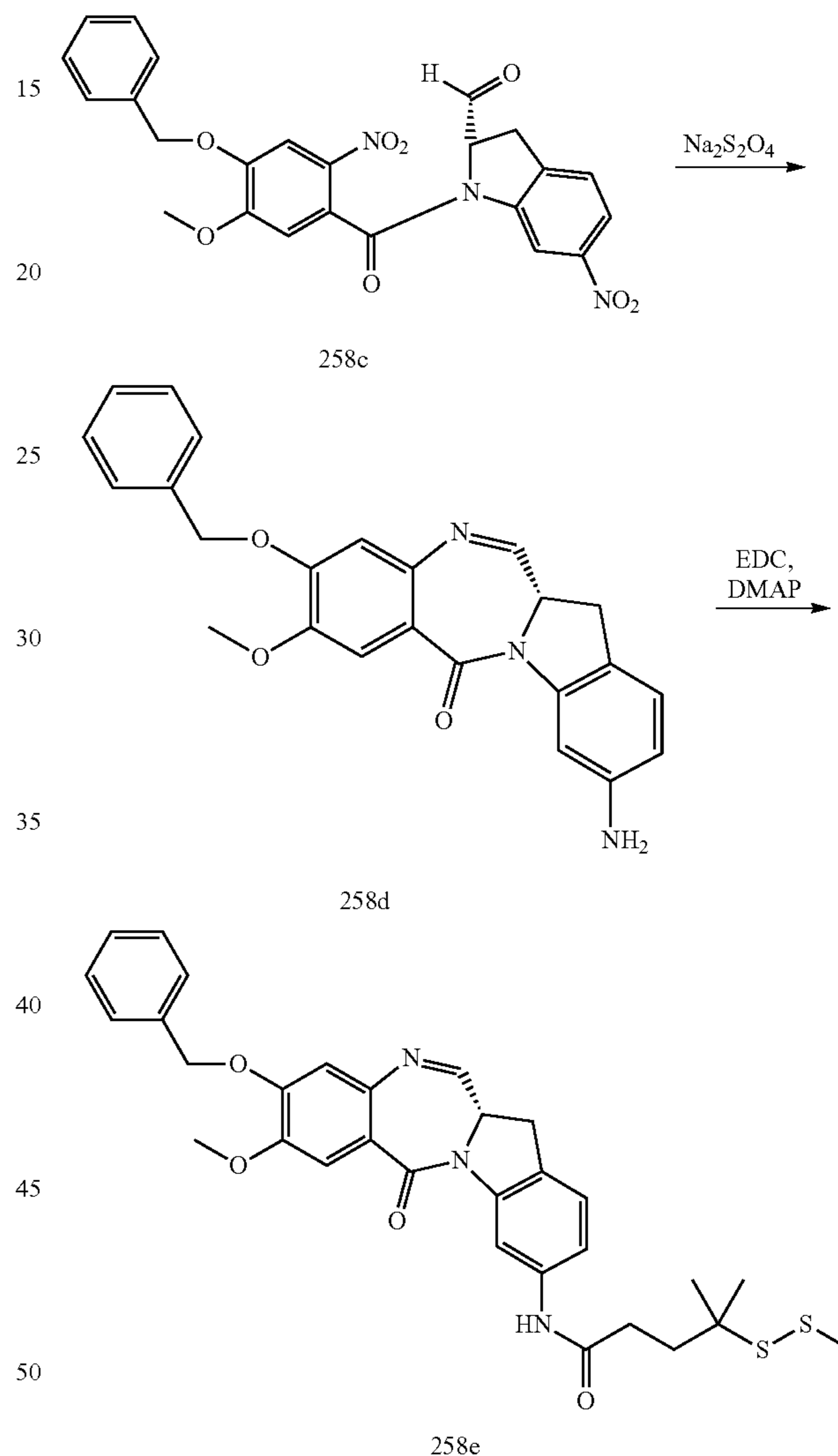
1-(4-(benzyloxy)-5-methoxy-2-nitrobenzoyl)-6-nitroindoline-2-carbaldehyde (258c)
