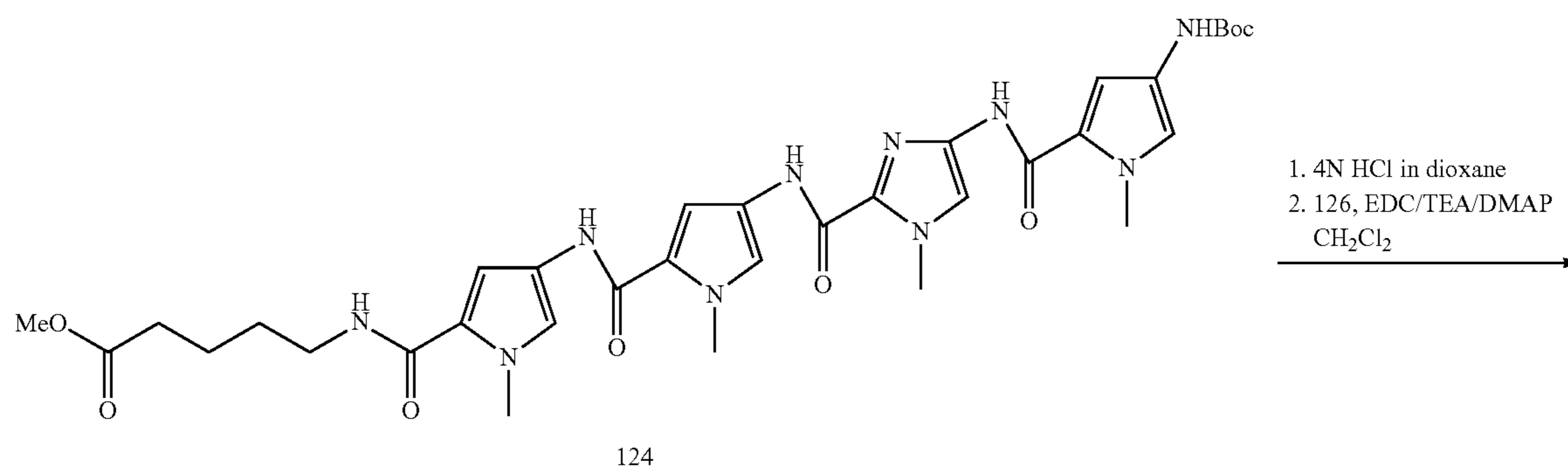
Compound 127 (IGN-11)
