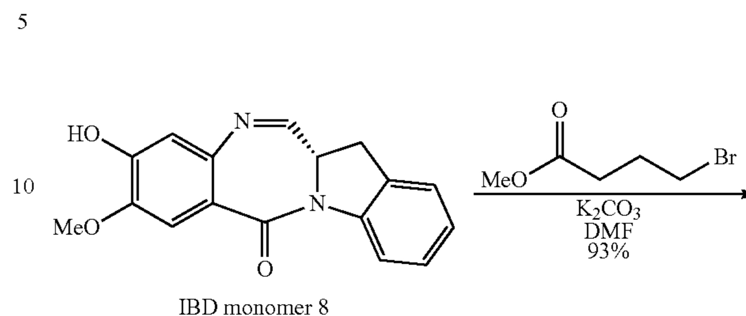
Compound 125
