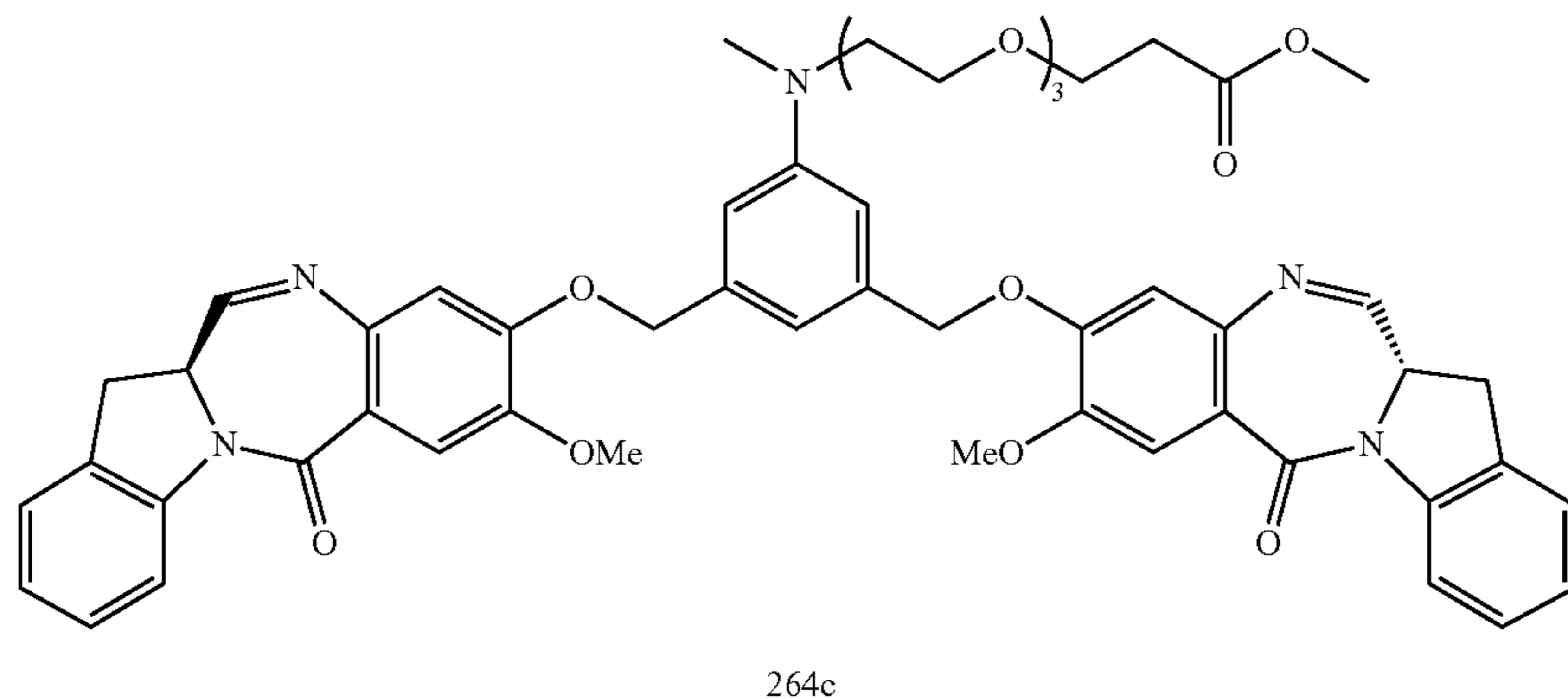
Compound 264c
