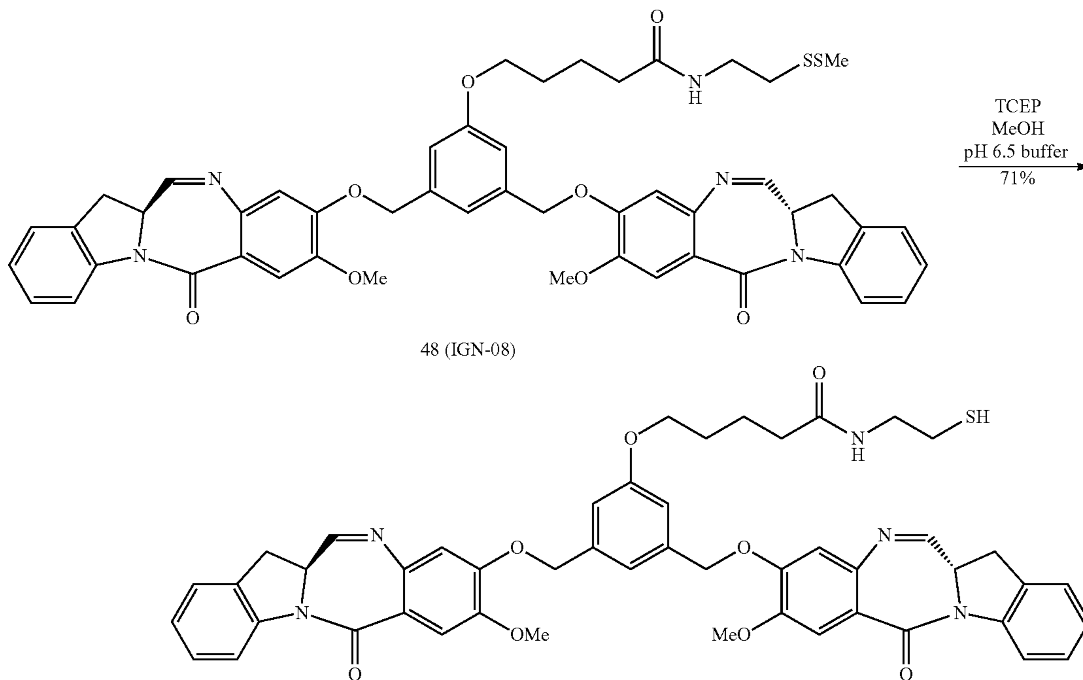
Compound 49
