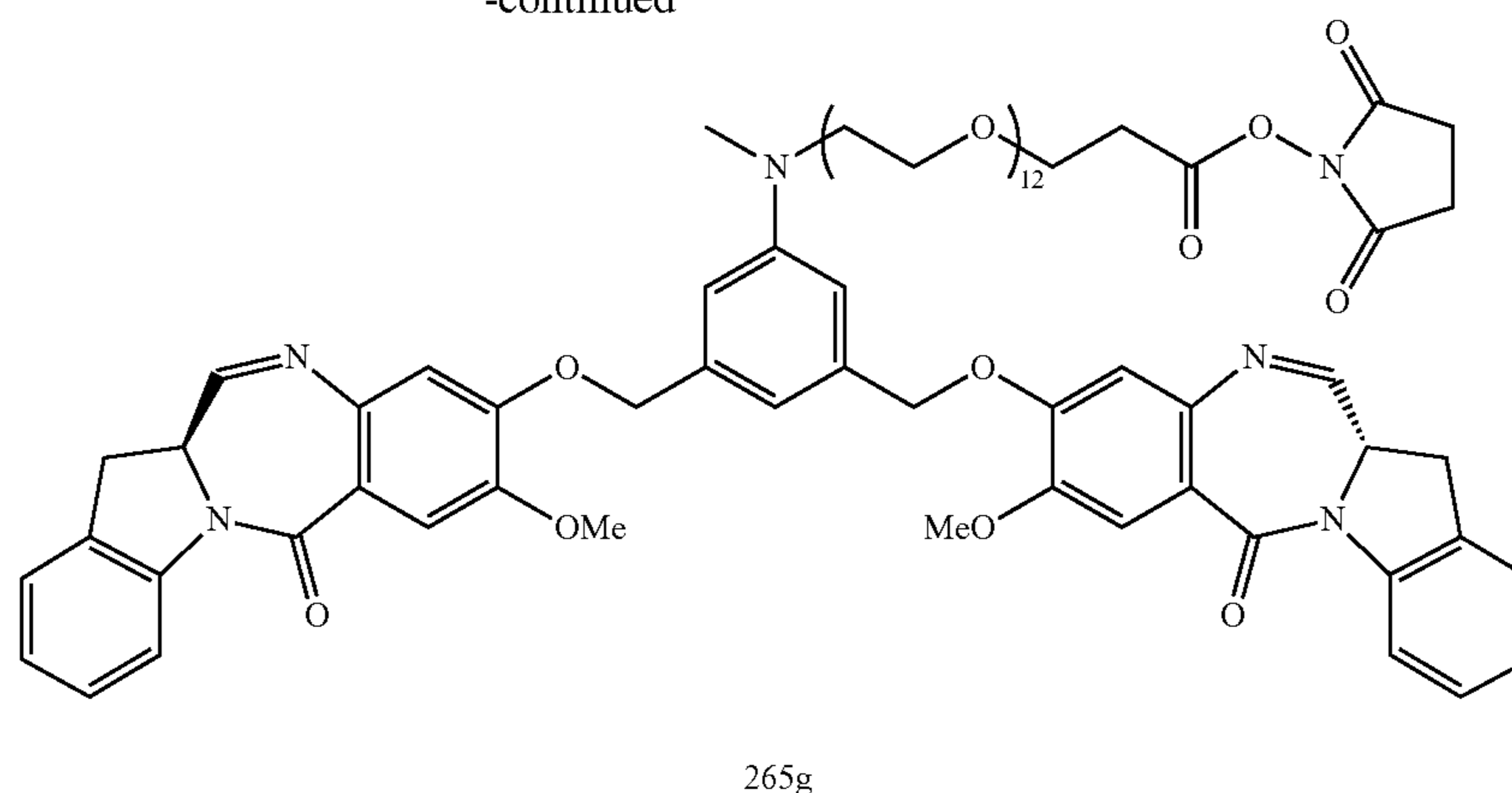
Compound 265g
