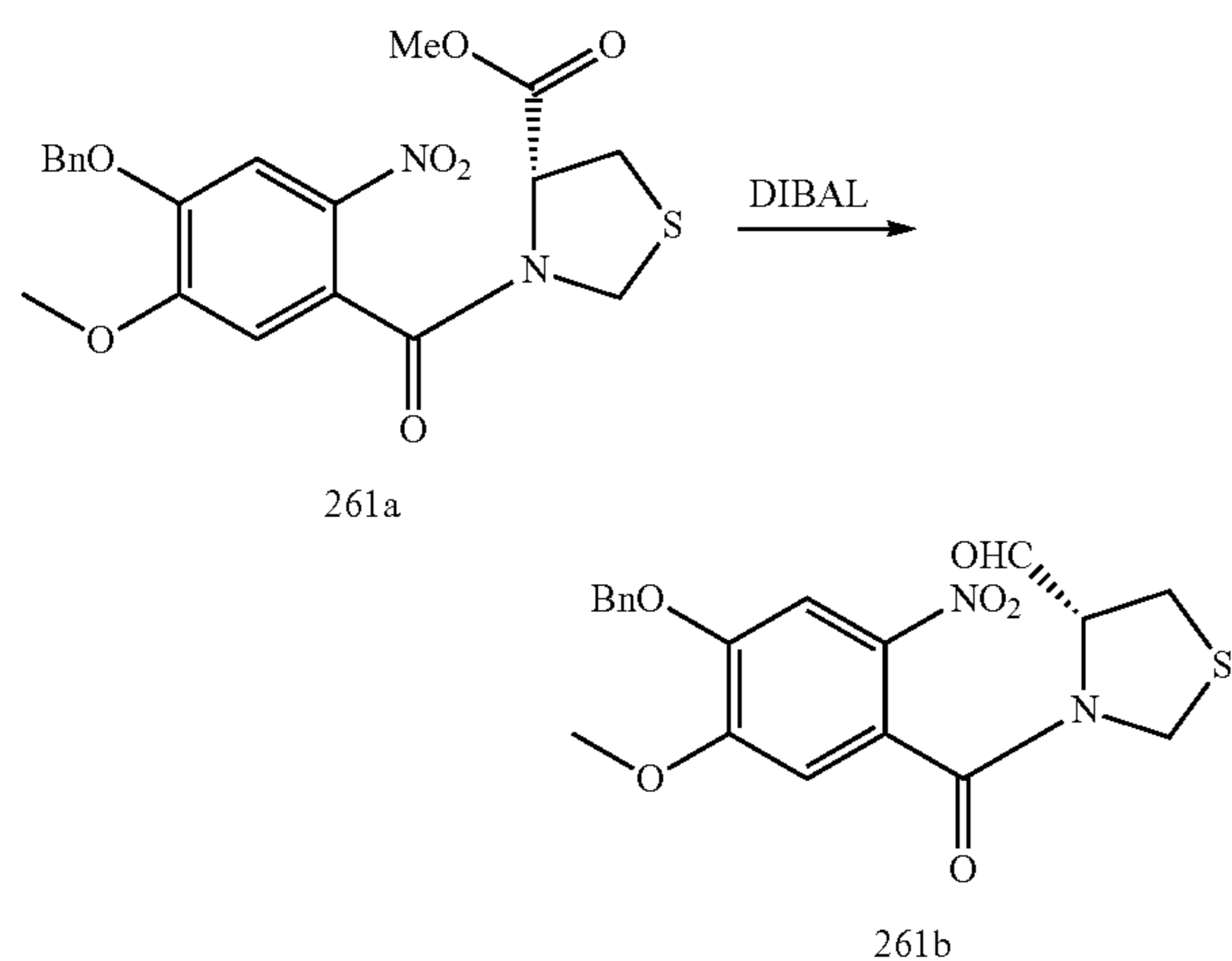
Compound 261b
