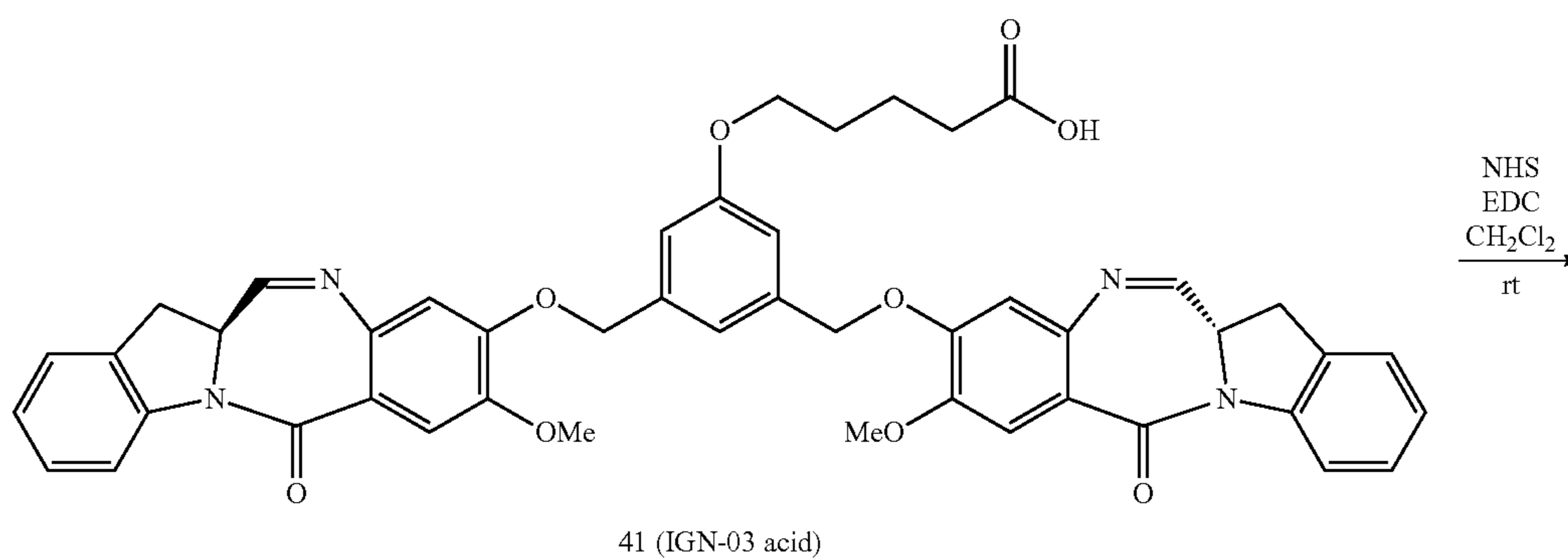
Compound 43
