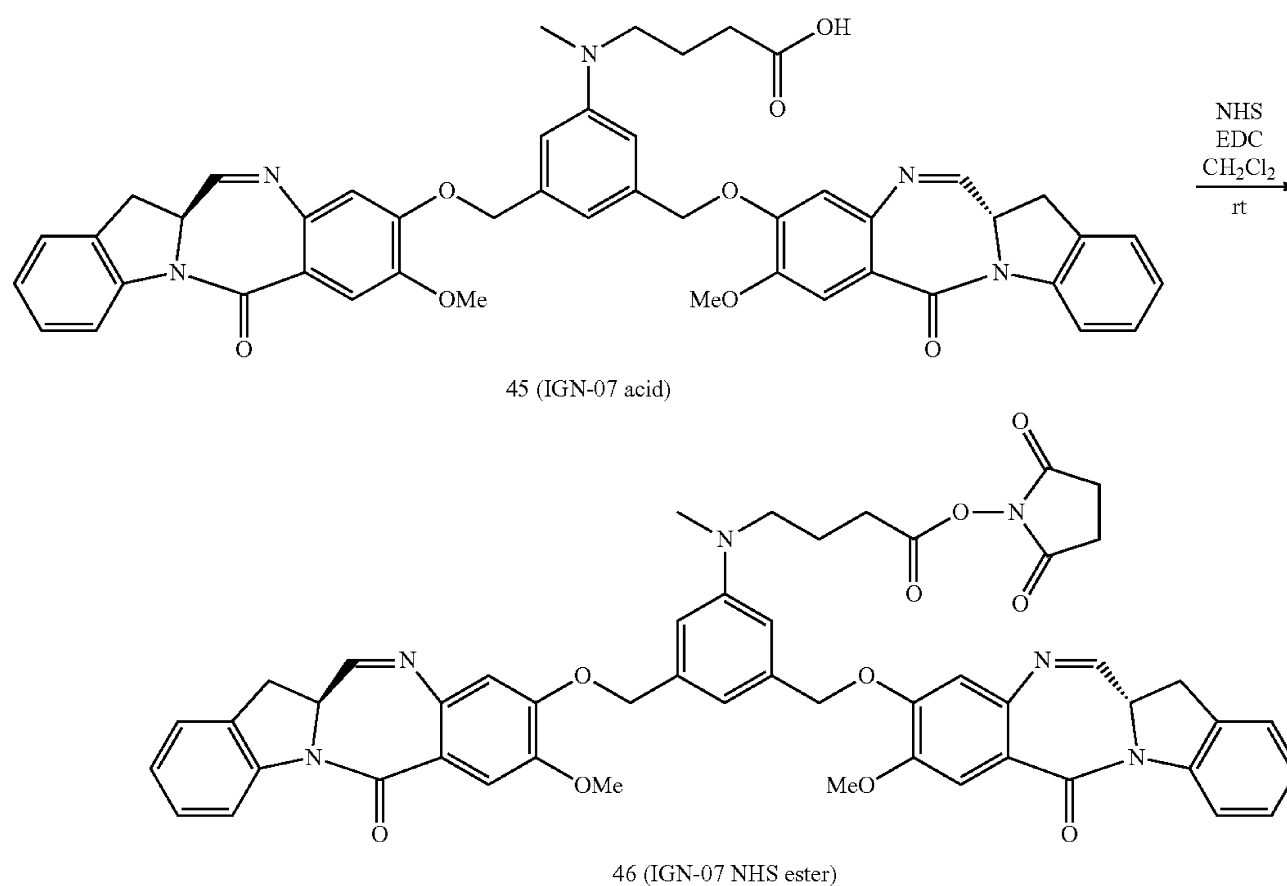
Compound 46
