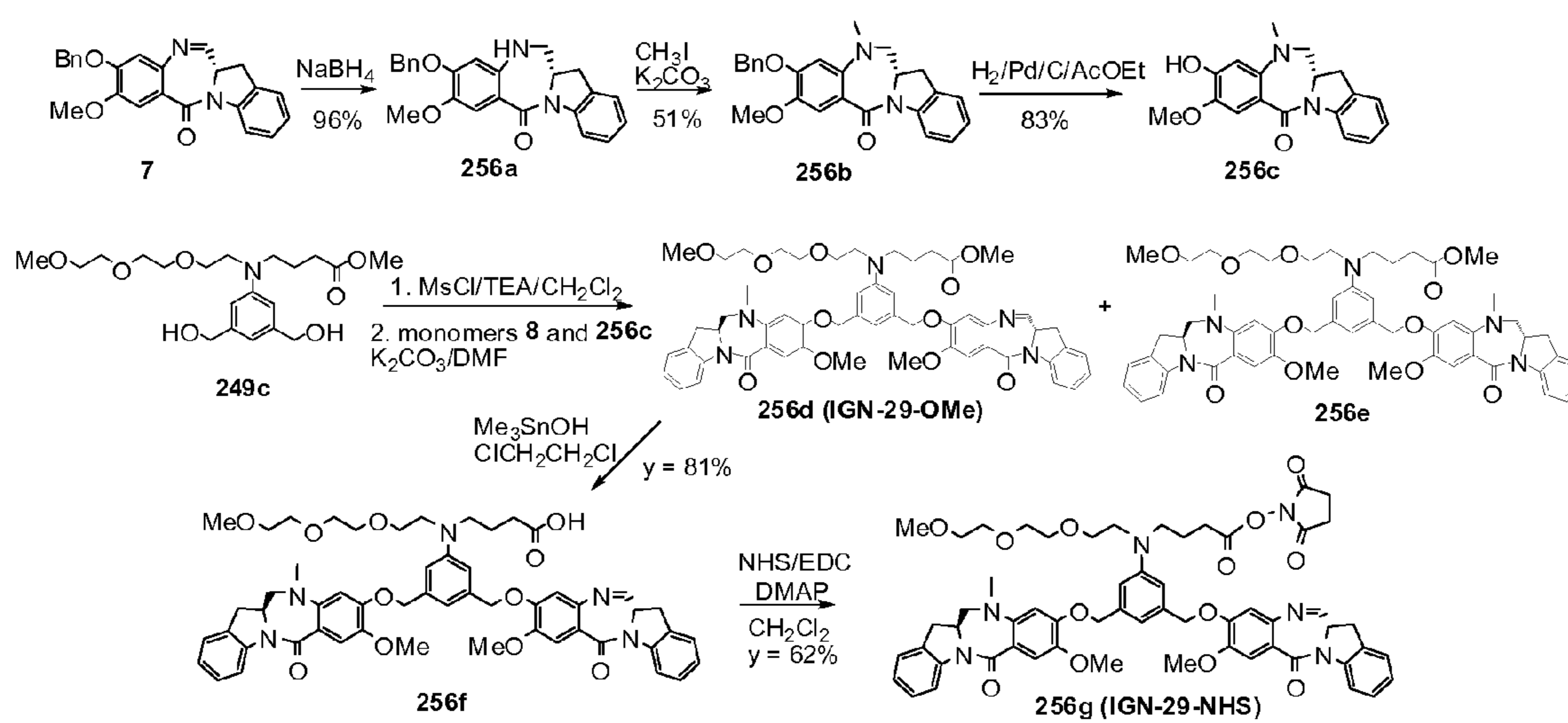
FIG. 40 Synthetic scheme of compound 256g (IGN-29-NHS) .
