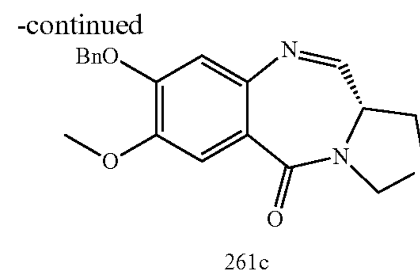
Compound 261c
