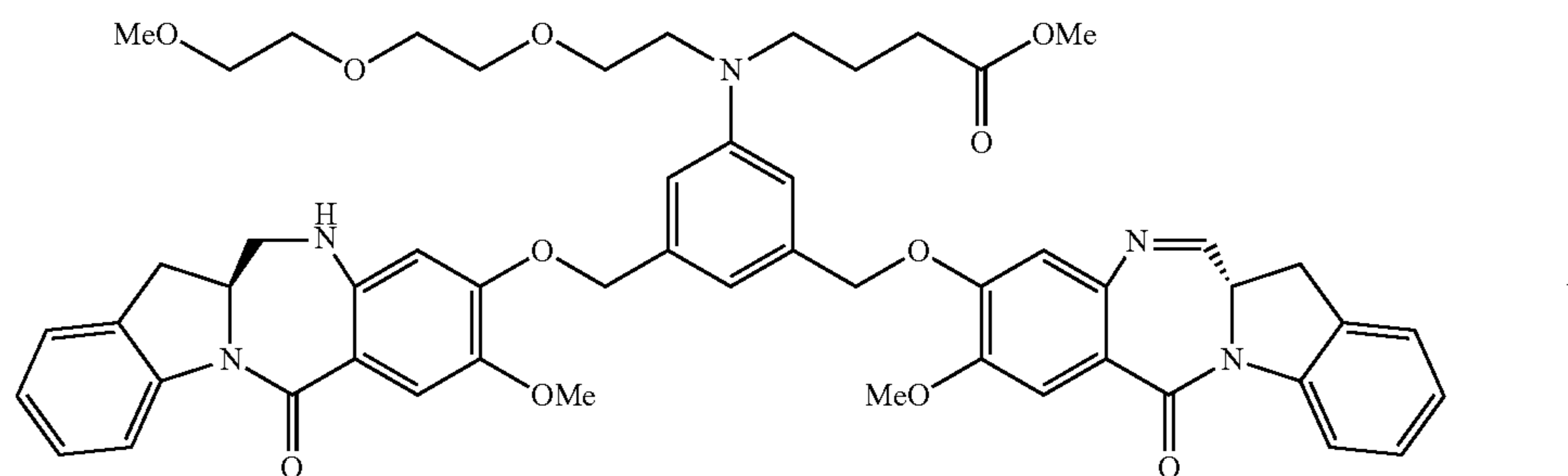
254a (IGN-23-OMe) y = 24.5%
