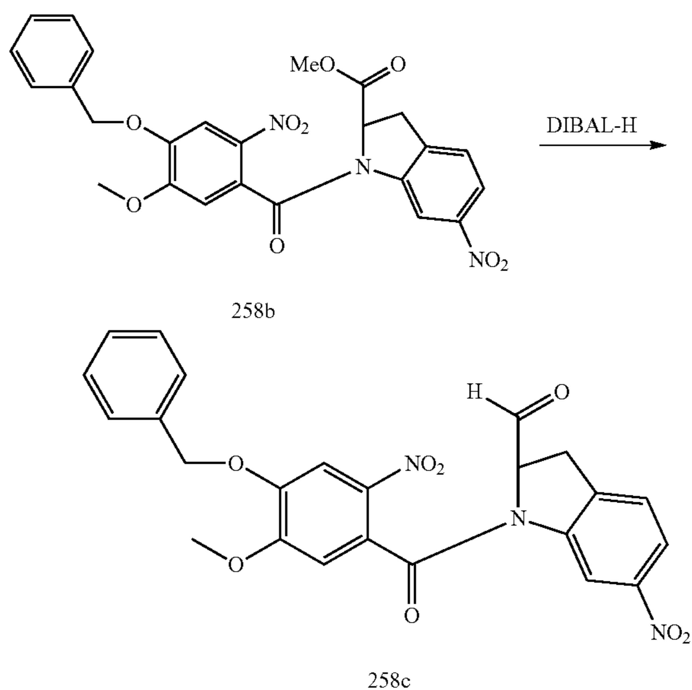
1-(4-(benzyloxy)-5-methoxy-2-nitrobenzoyl)-6-nitroindoline-2-carbaldehyde (258c)
