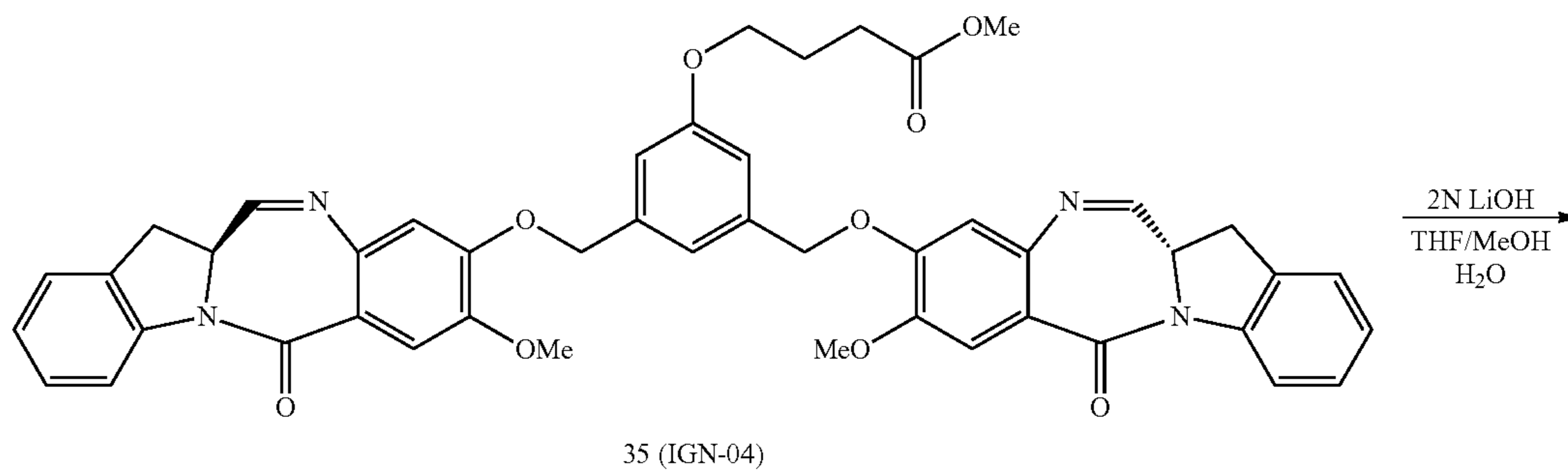
Compound 42
