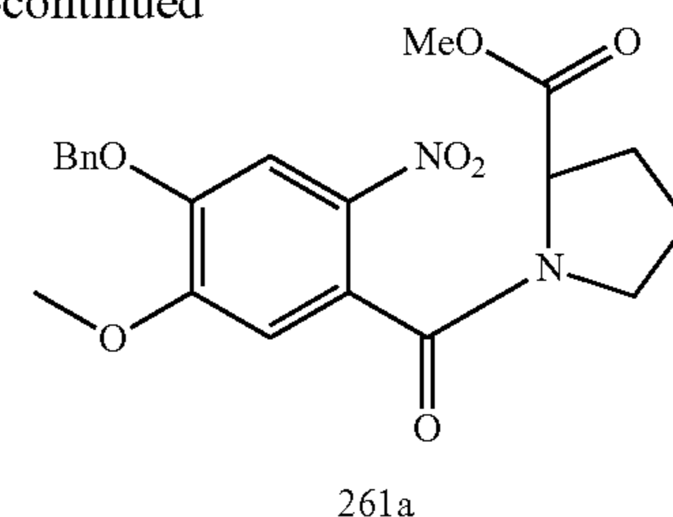
Compound 261a
