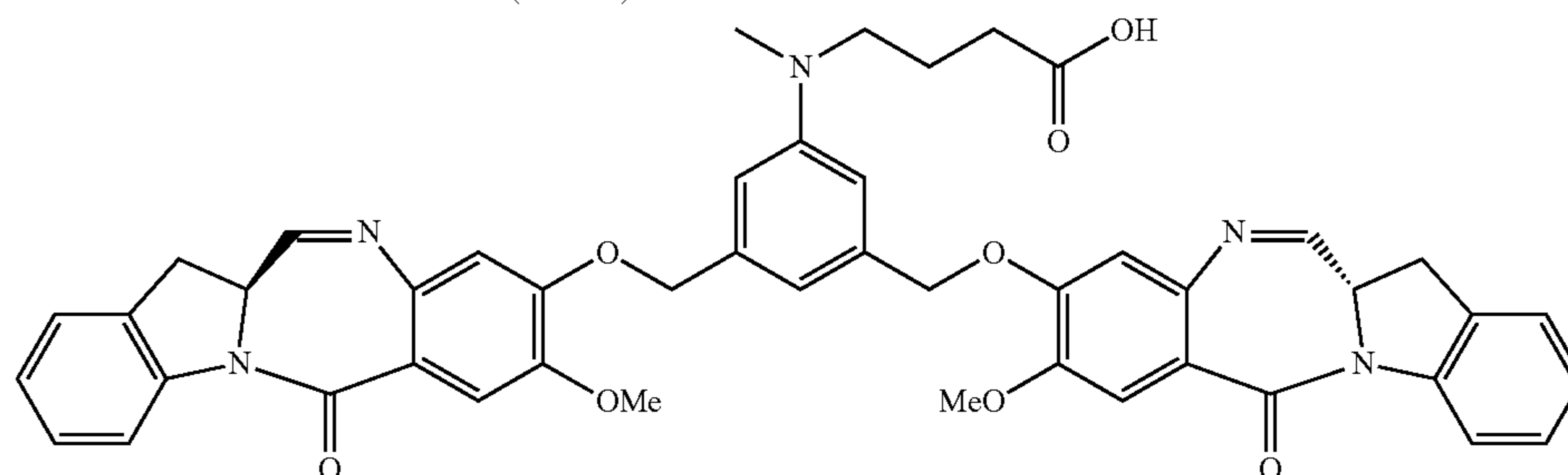
45 (IGN-07 acid)
