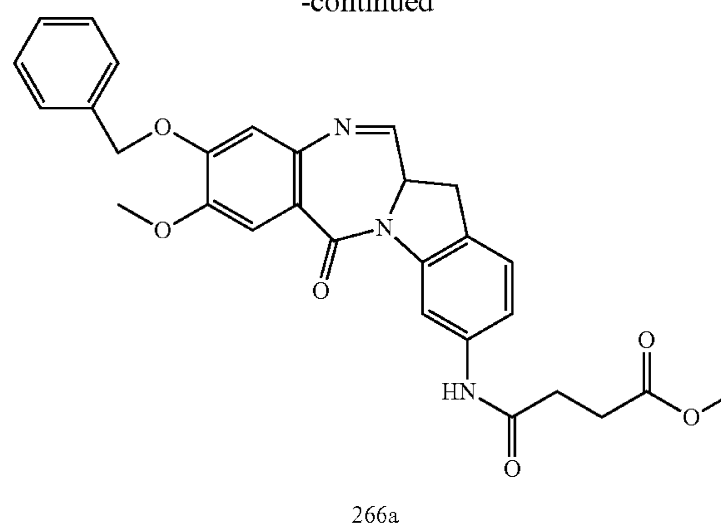
Compound 266a
