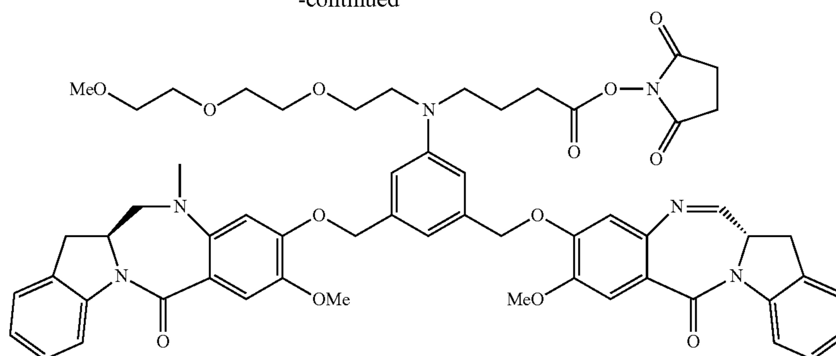
256g (IGN-29-NHS)
