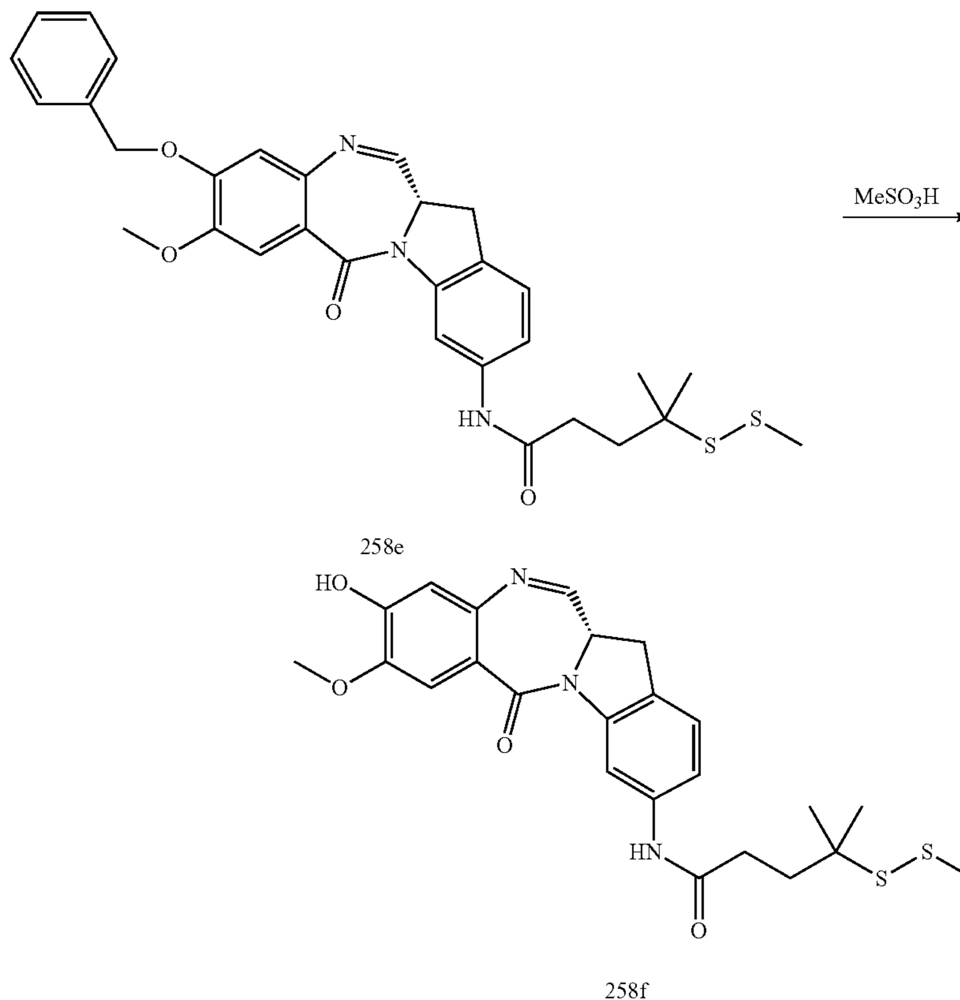
Compound 258f
