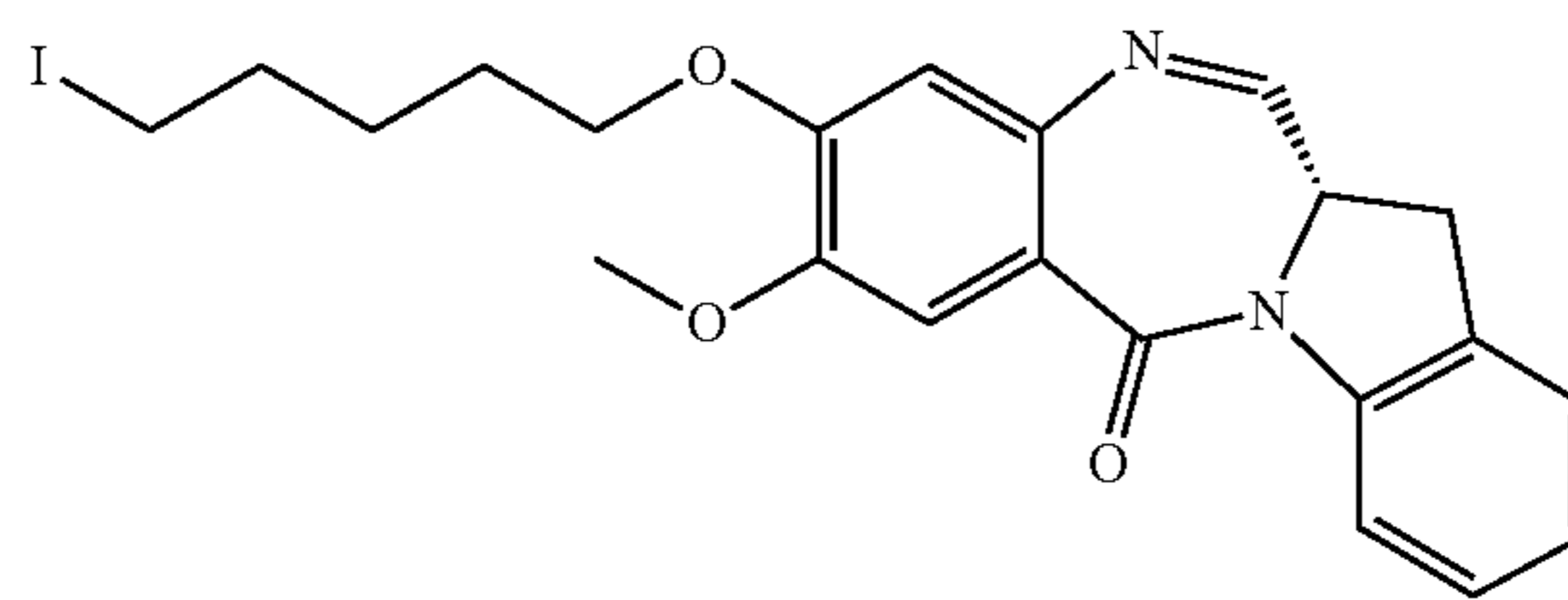
259a
