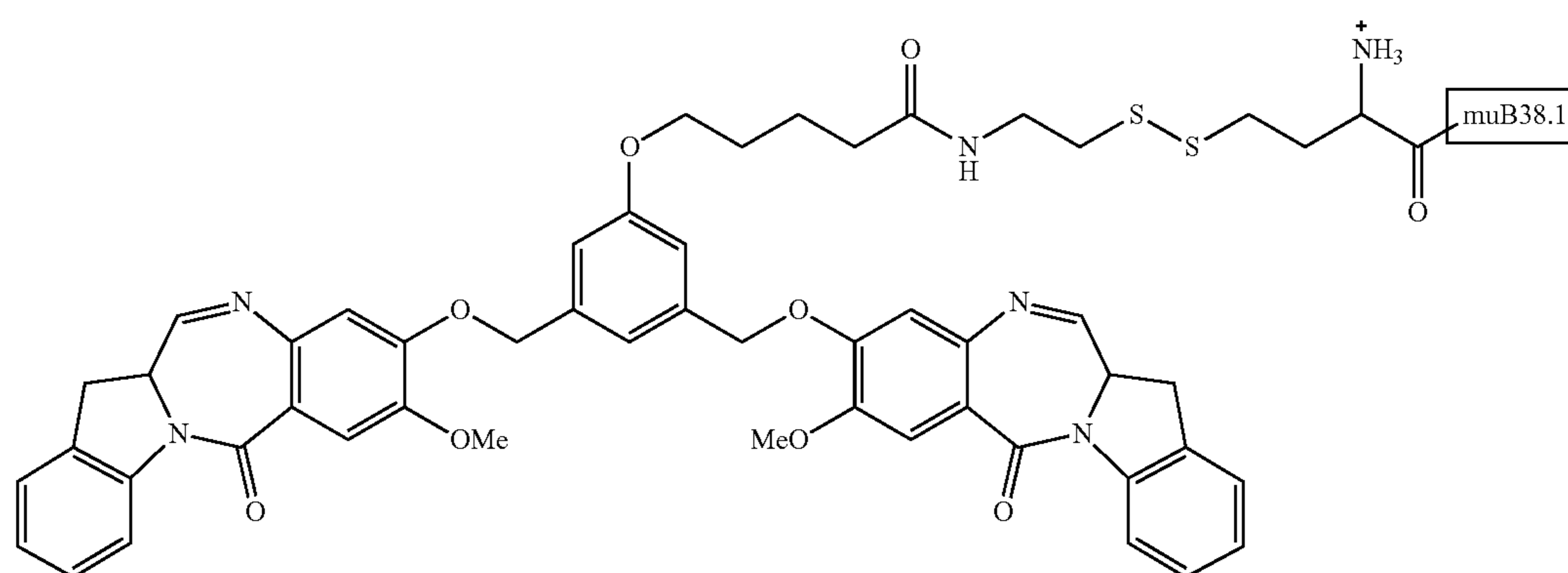
B38.1-IGN-10
