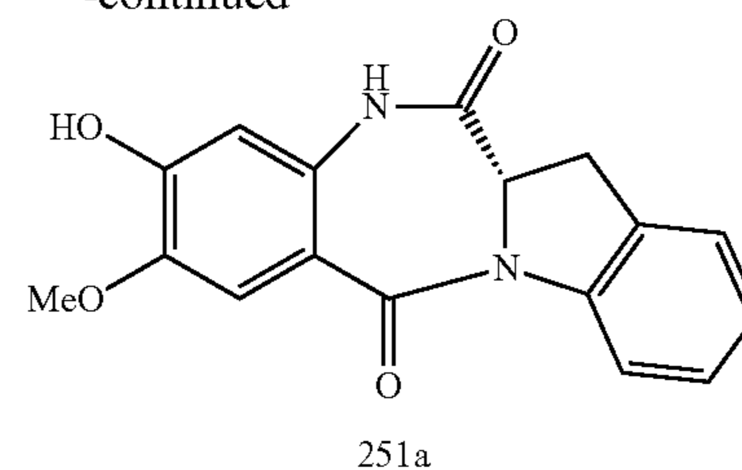
Compound 251a
