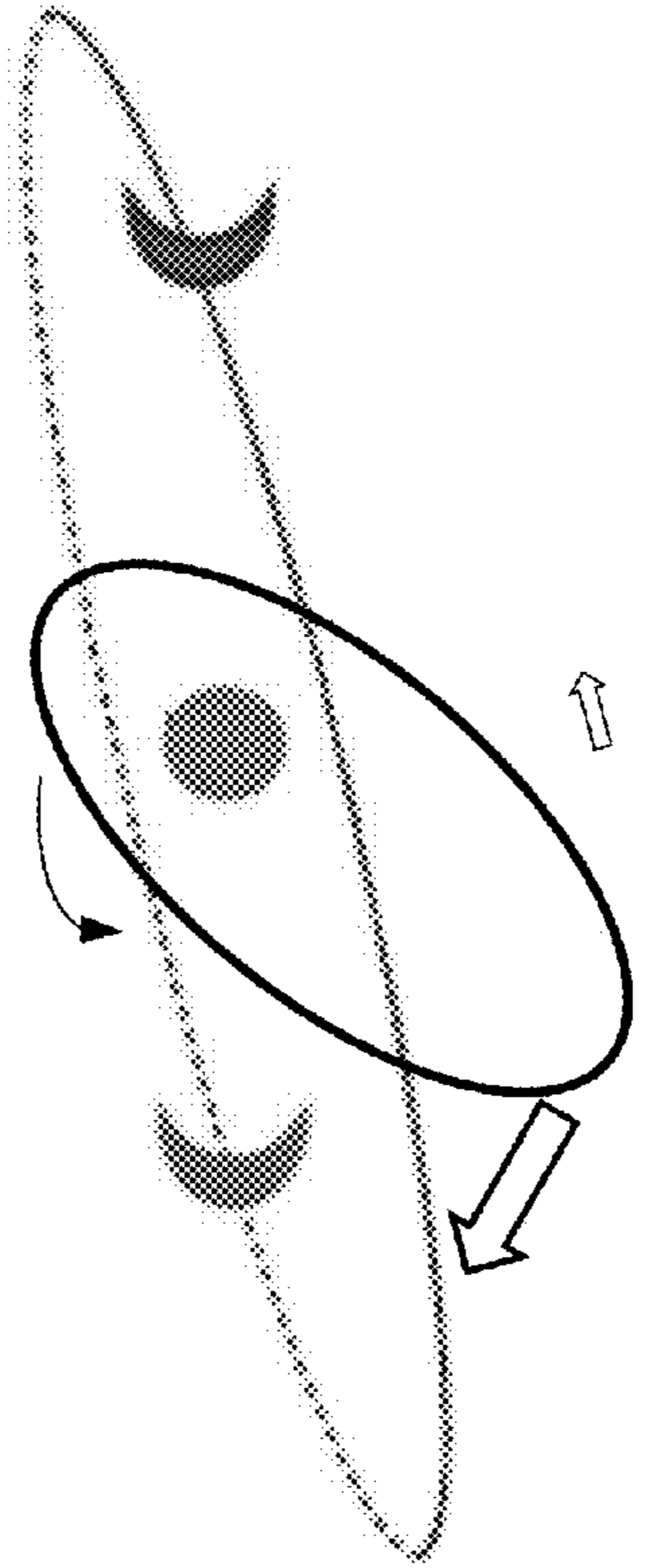
Detail D: Argument of perigee between 90 and 0 (360) degrees
