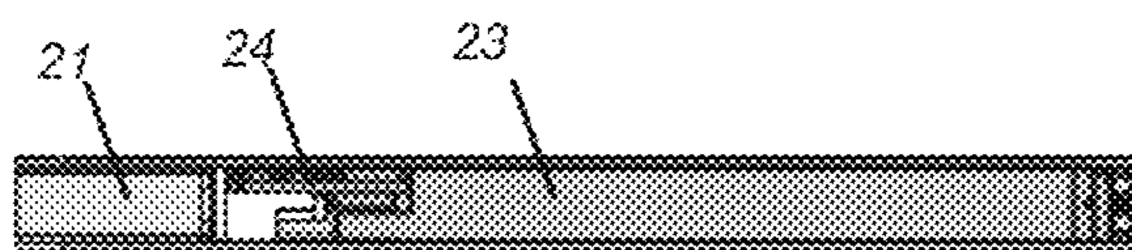
Section B-B
