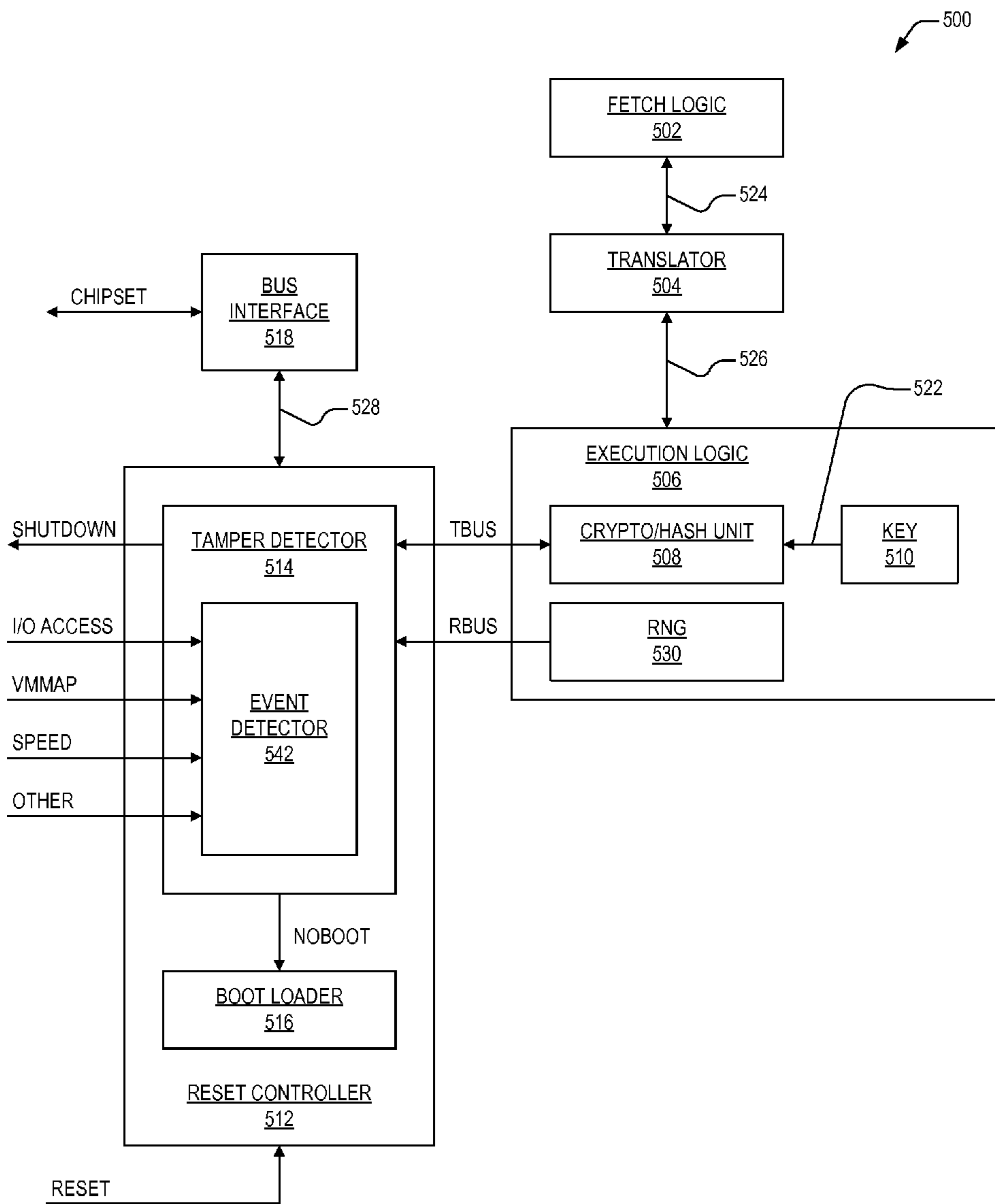
EVENT-BASED MECHANISM FOR SECURING BIOS
