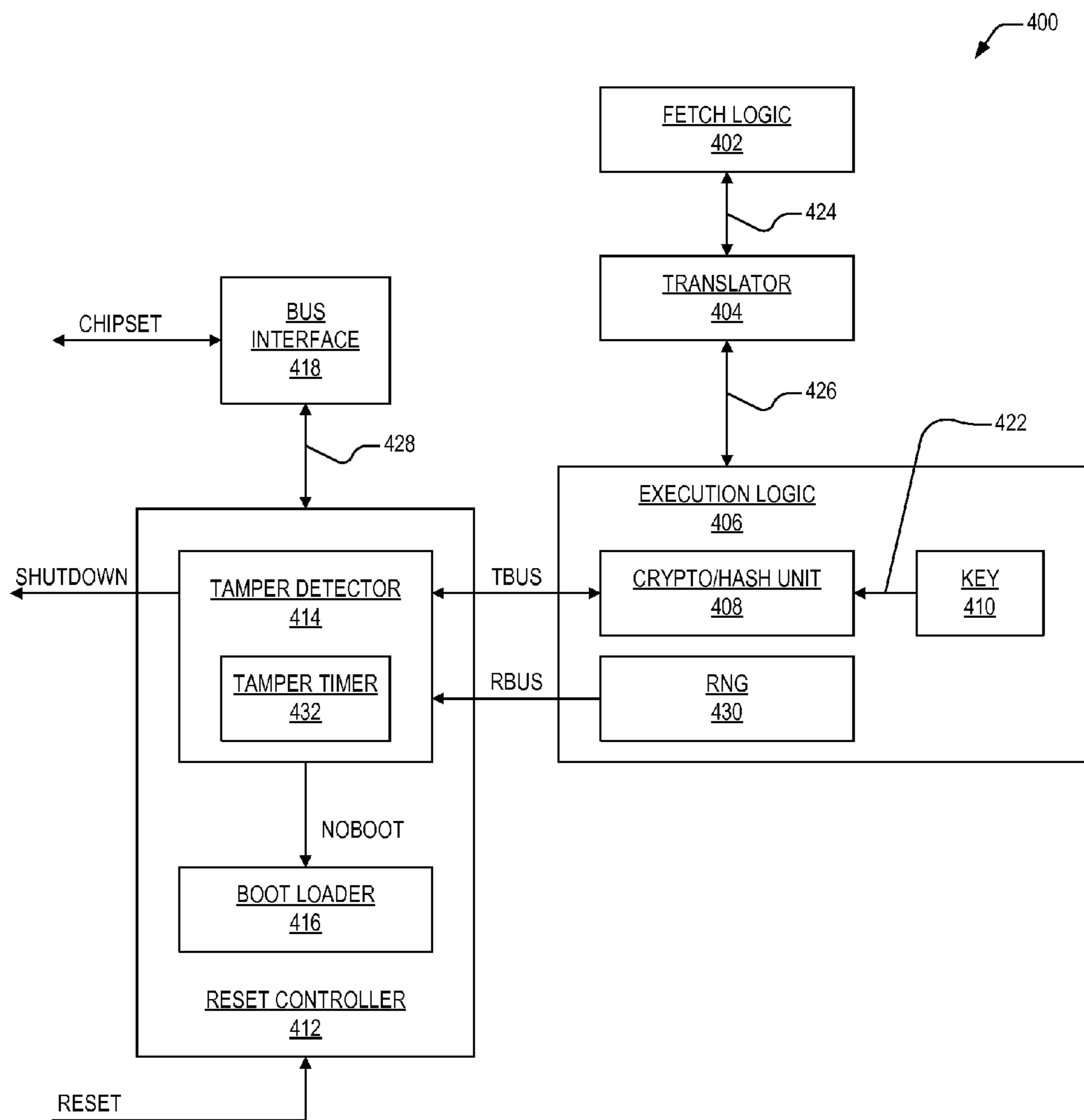
PERIODIC MECHANISM FOR SECURING BIOS
