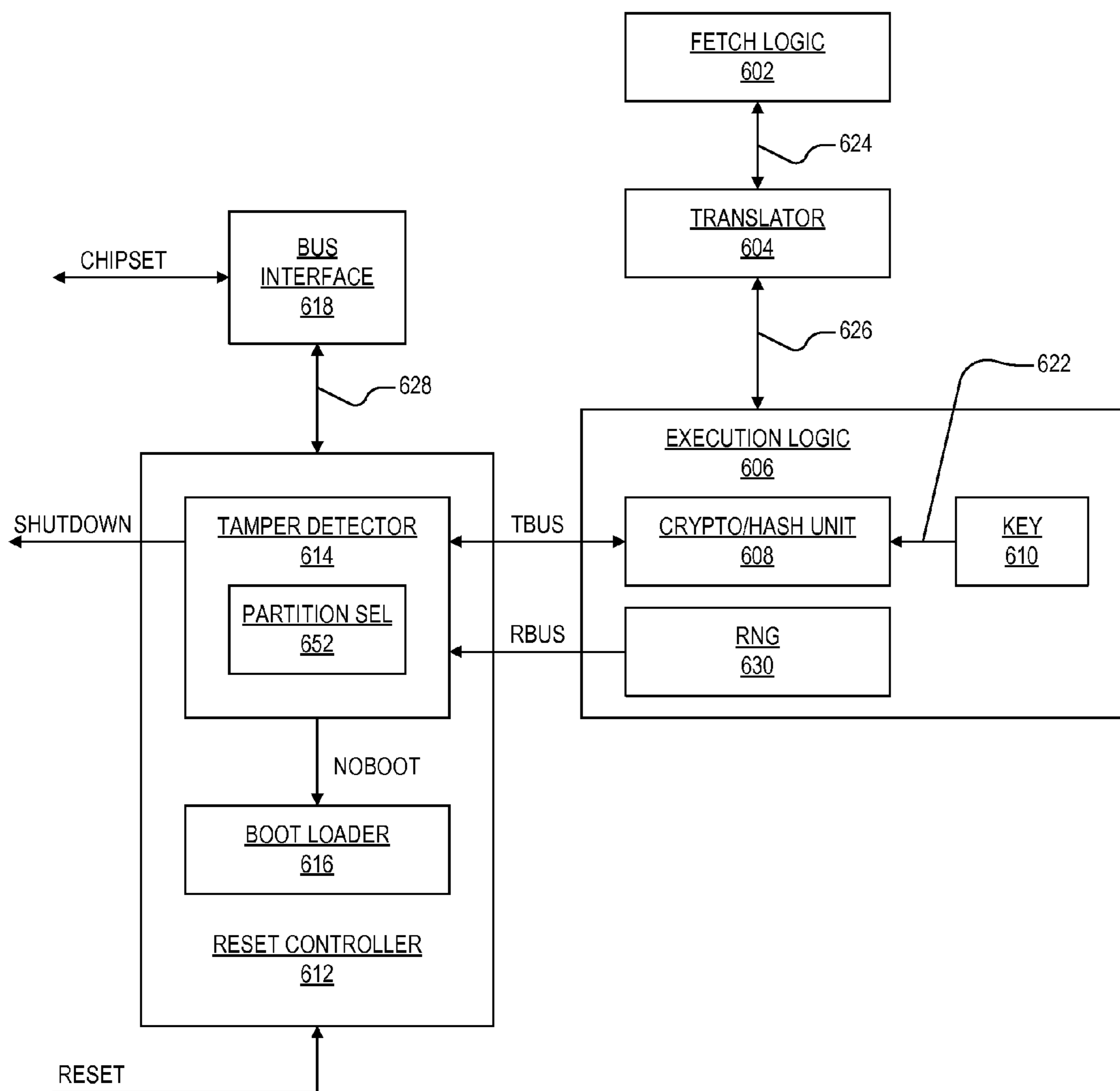
PARTITION-BASED MECHANISM FOR SECURING BIOS
