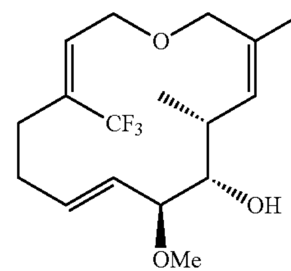
Z-Trifluoromethyl dehydromigraether
