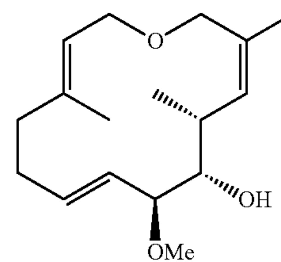
Methyl-trans-dehydromigraether
