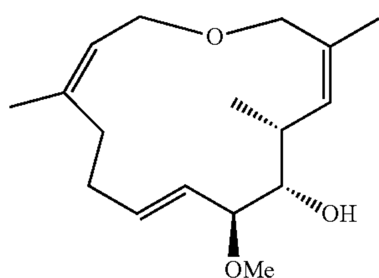
Methyl-cis-dehydromigraether
