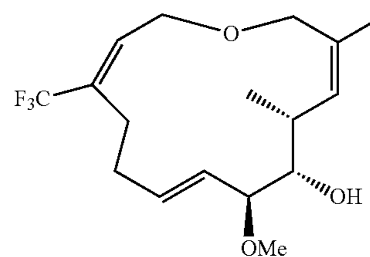
E-Trifluoromethyl dehydromigraether
