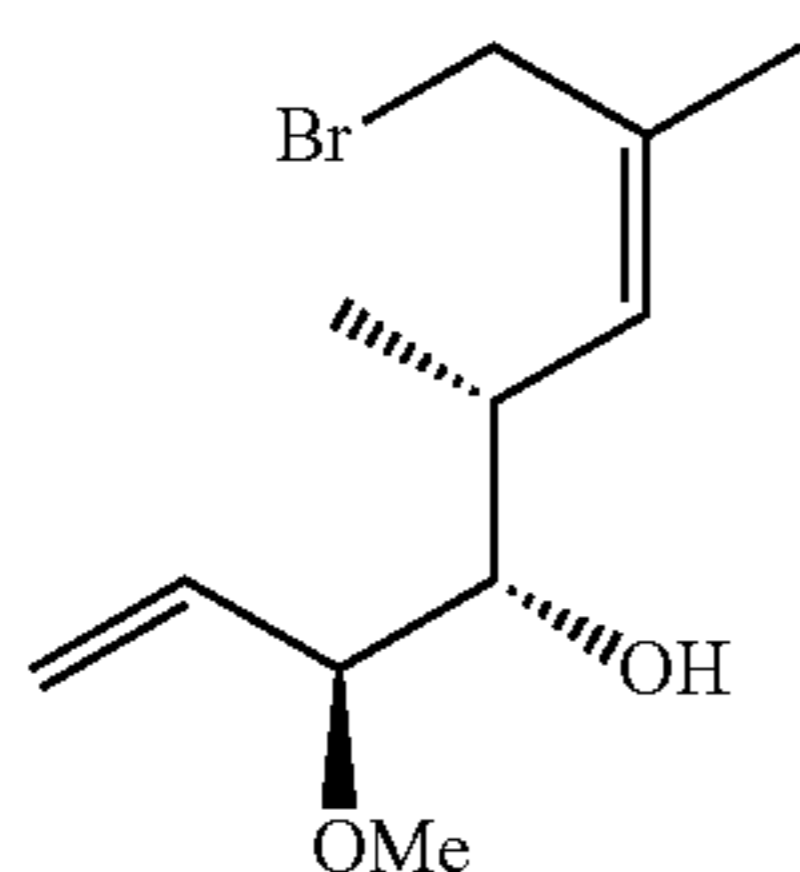
(3S,4S,5R,Z)-8-Bromo-3-methoxy-5,7-dimethylocta-1,6-dien-4-ol (12)
