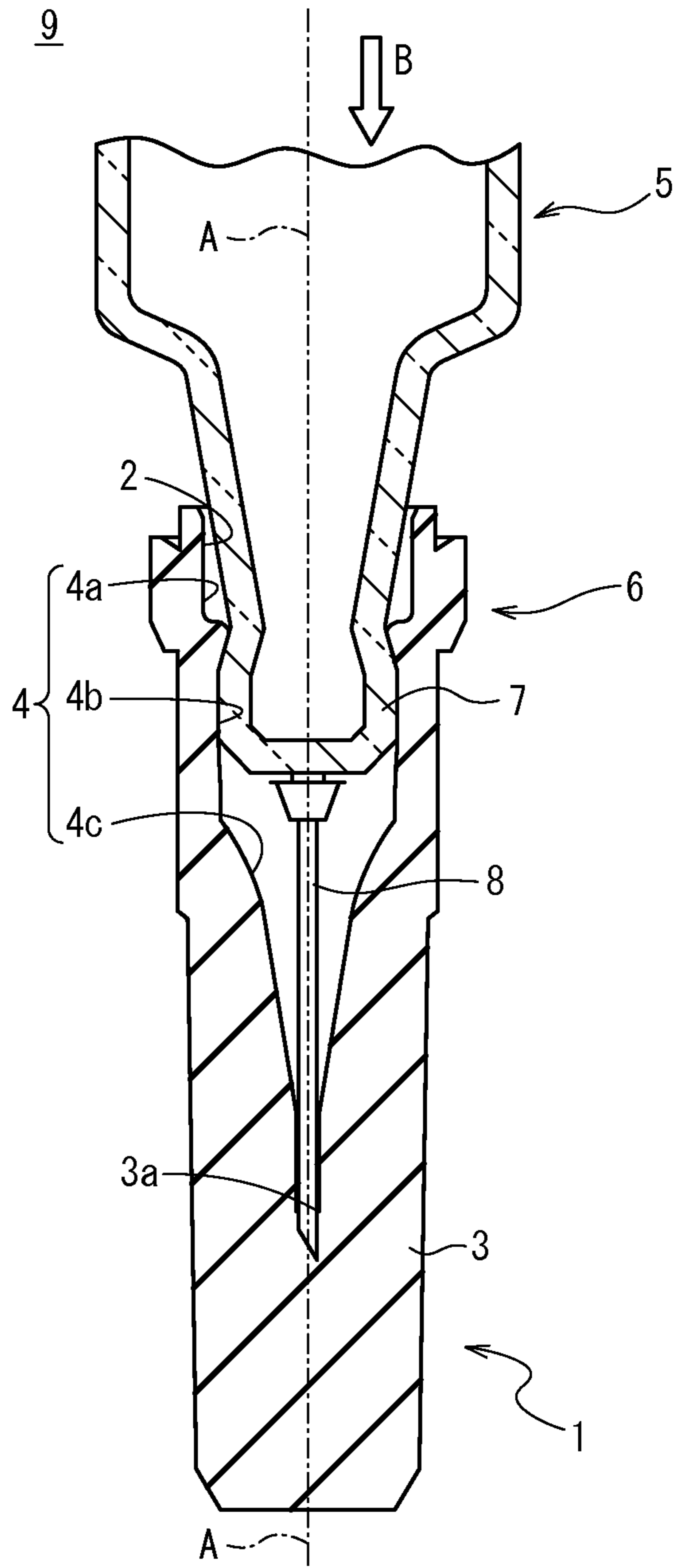
FIG. 5 (Prior Art)
