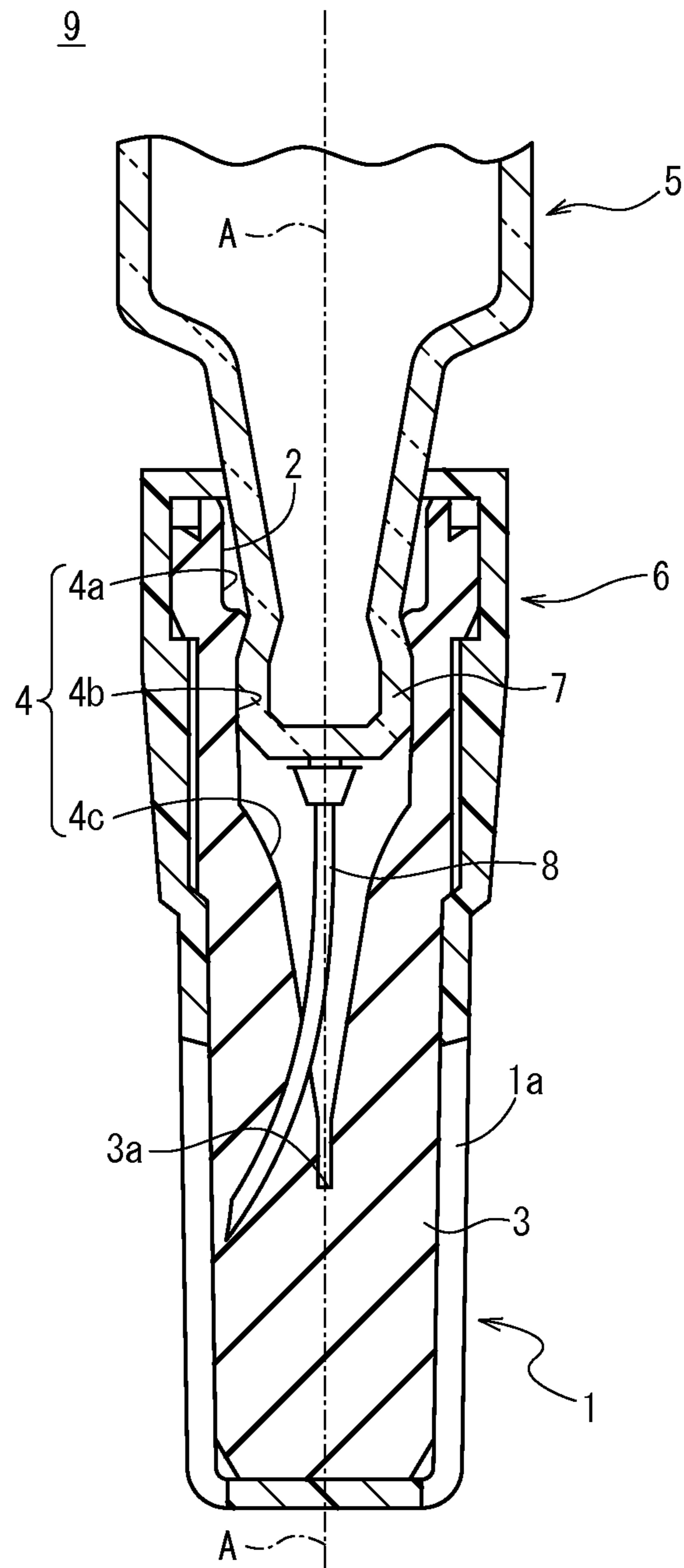
FIG. 8 (Prior Art)
