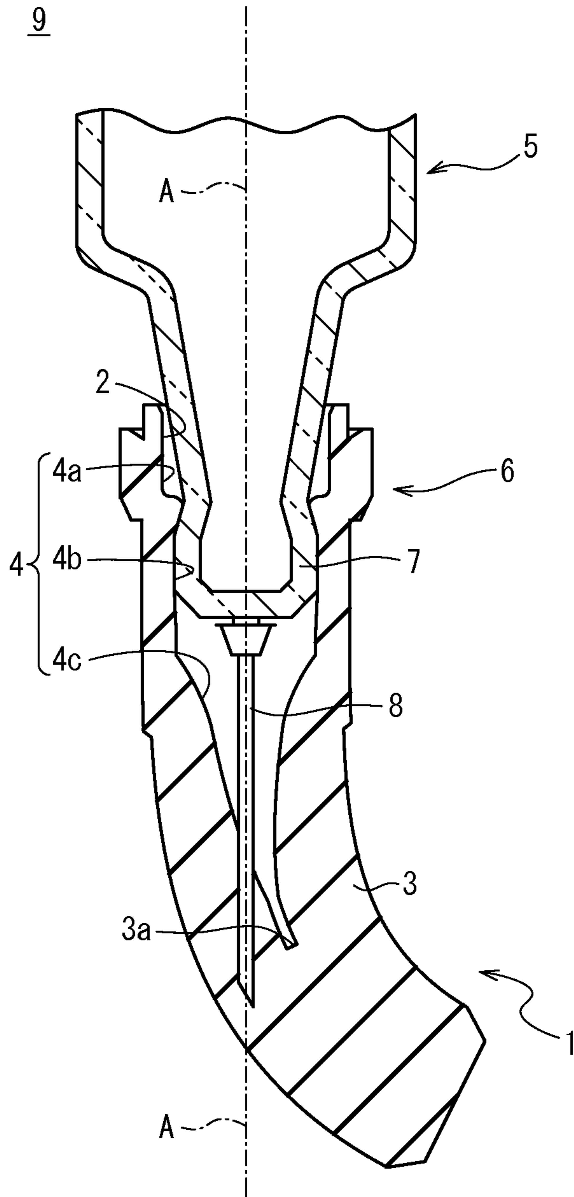
FIG. 6 (Prior Art)
