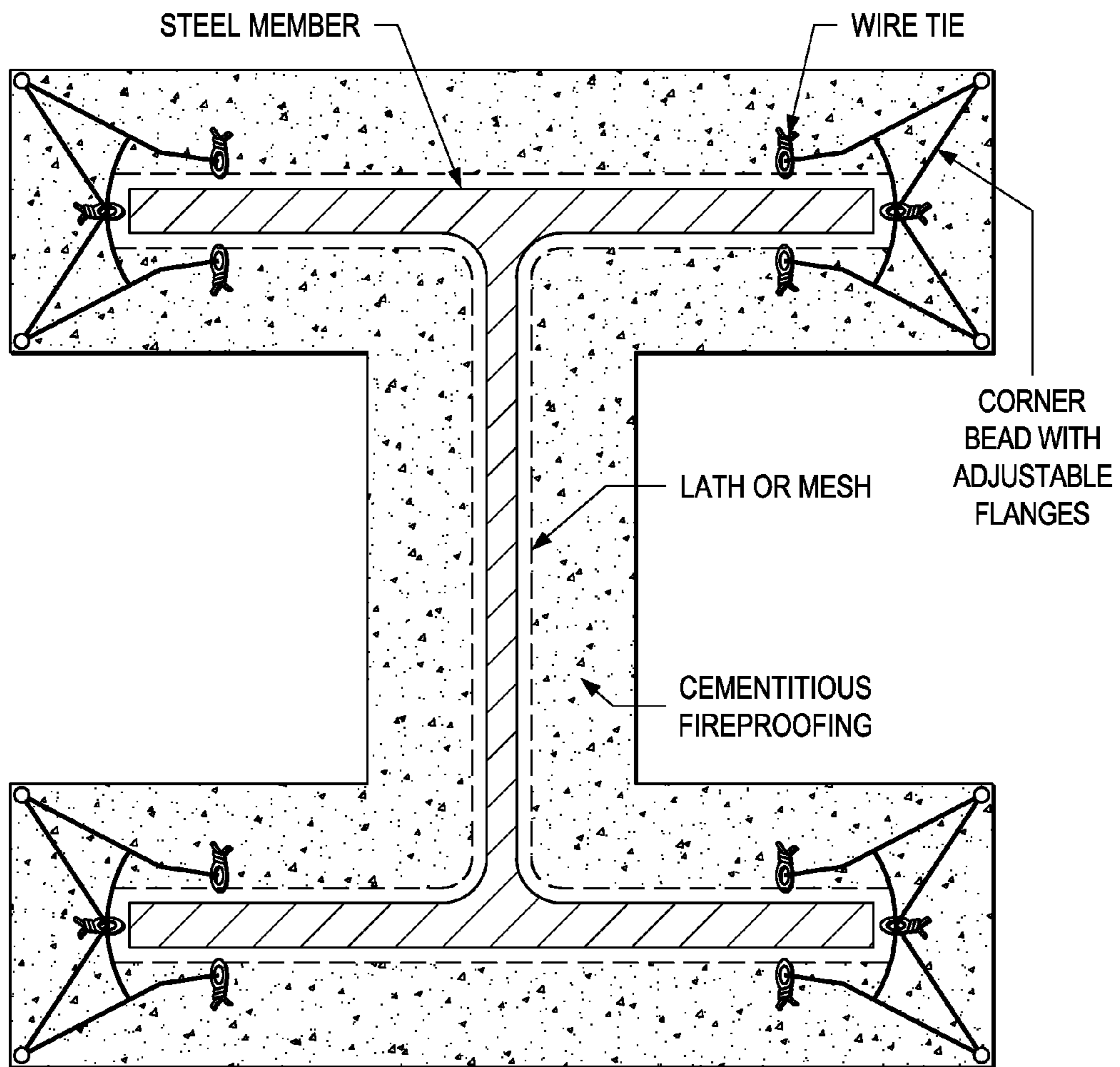
FIG. 2 (PRIOR ART)
