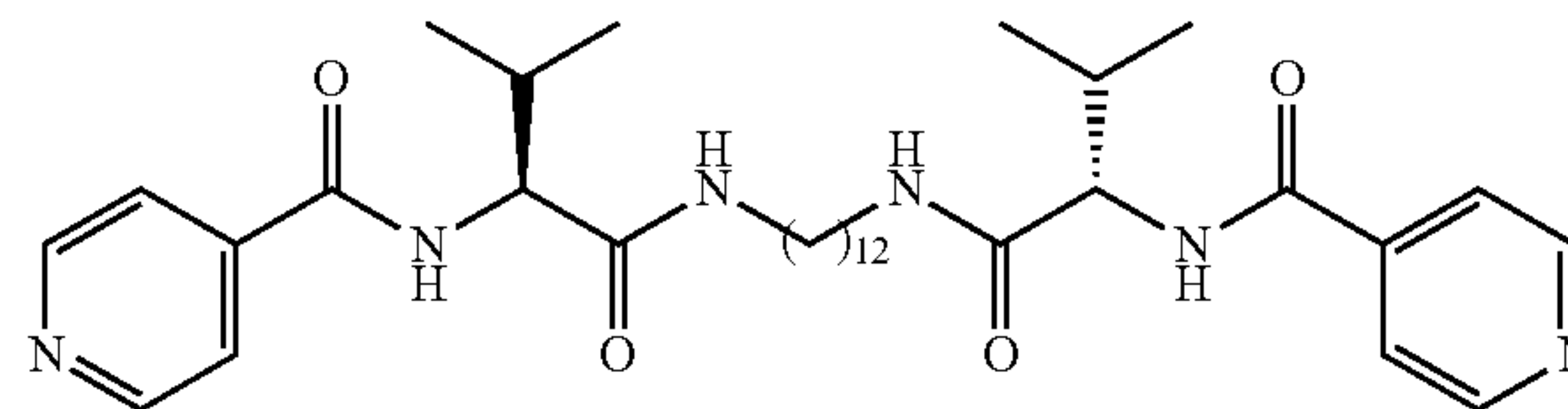
N,N'-(2S,2'S)-1,1'-(dodecane-1,12-diylbis(azanediyl))bis(3-methyl-1-oxobutane-2,1-diyl)diisonicotinamide
