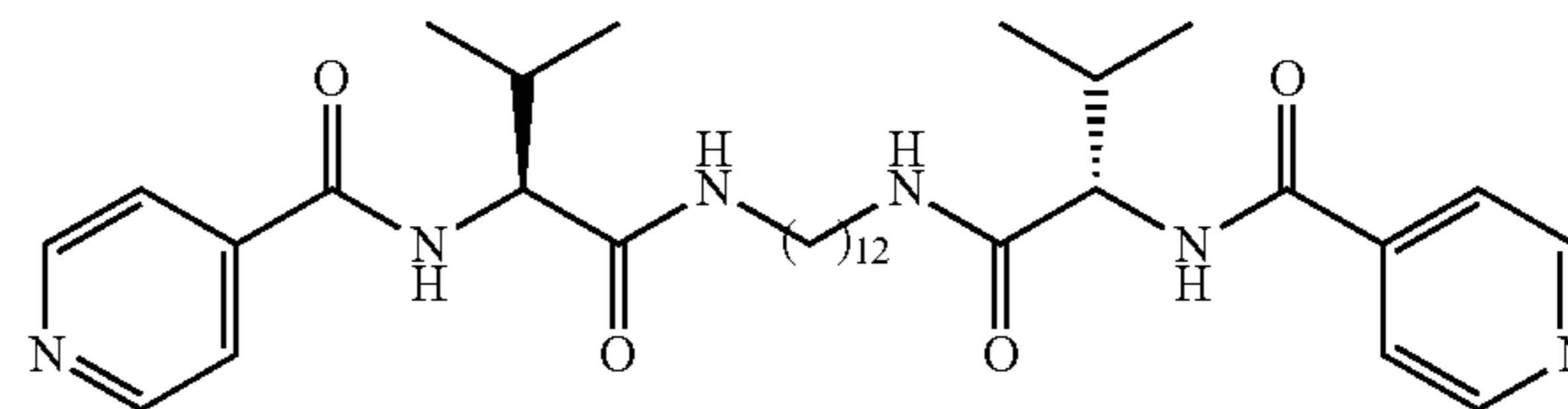
5 10 N,N'-(2S,2'S)-1,1'-(dodecane-1,12-diylbis(azanediyl))bis(3-methyl-1-oxobutane-2,1-diyl)diisonicotinamide
