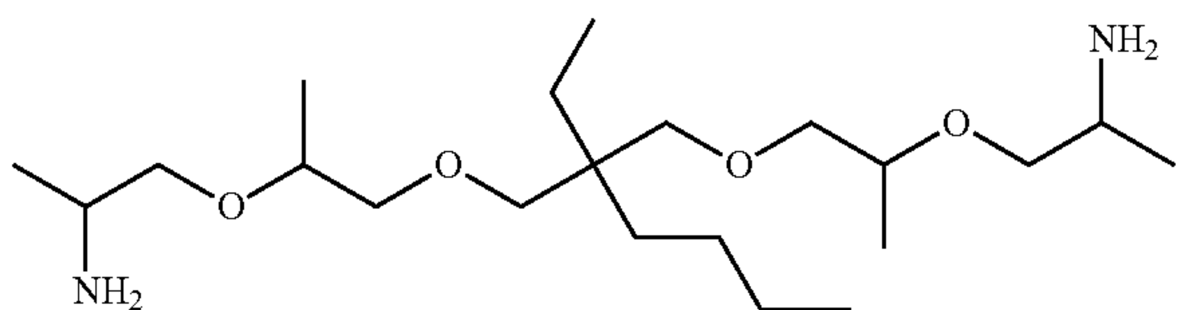
Formula B
