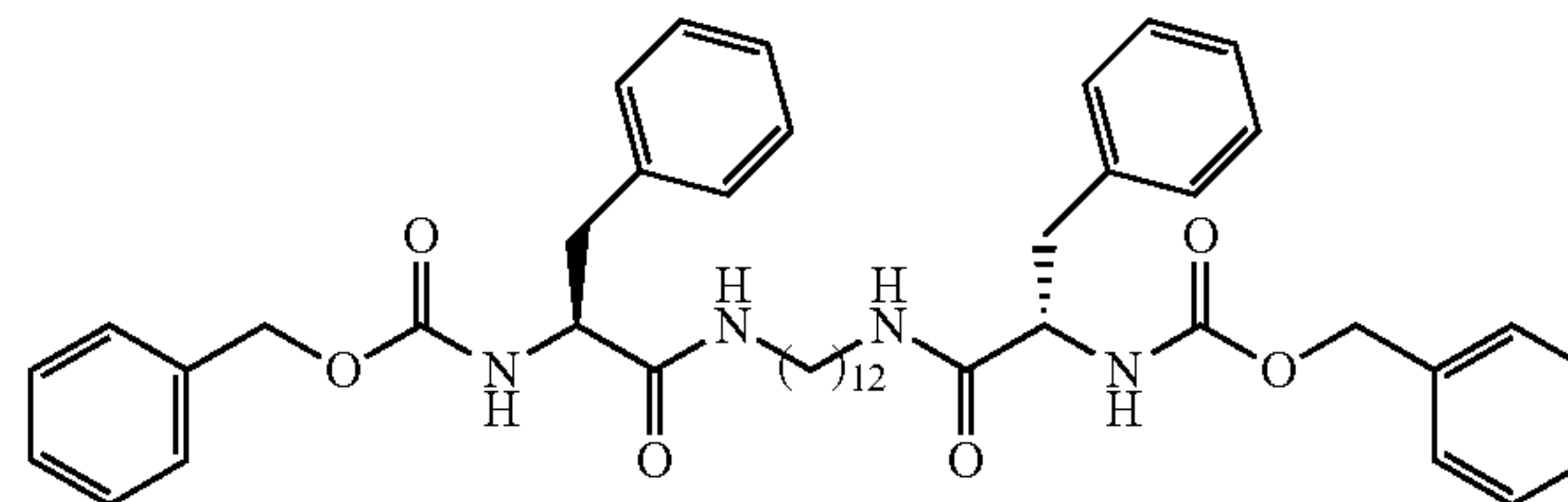
dibenzyl (2S,2'S)-1,1'-(propane-1,3-diylbis(azanediyl))bis(3-methyl-1-oxobutane-2,1-diyl)dicarbamate
