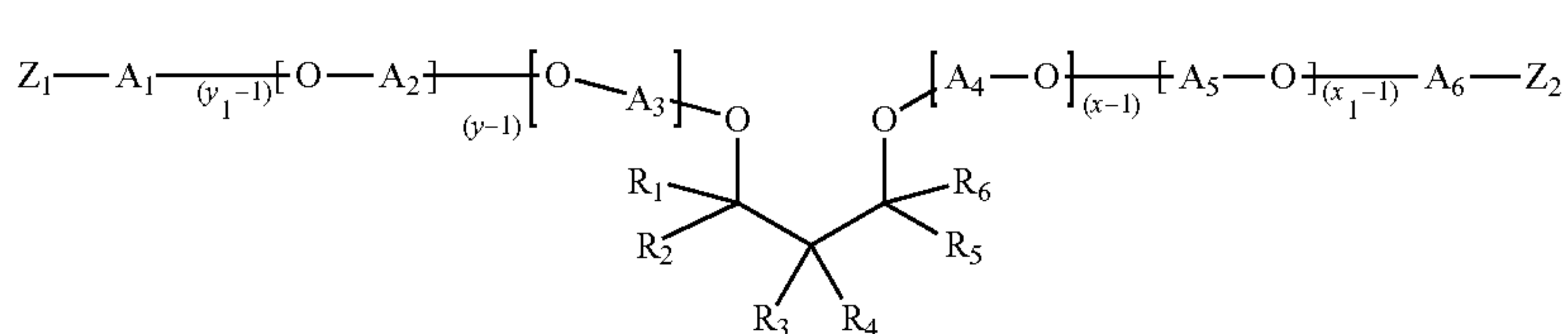
Formula (I)
