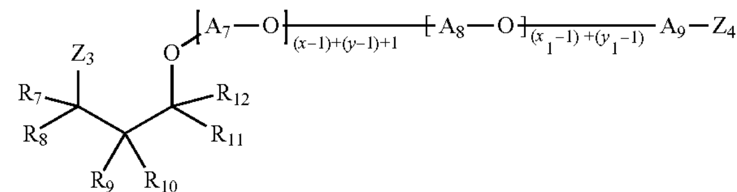
Formula (II)
