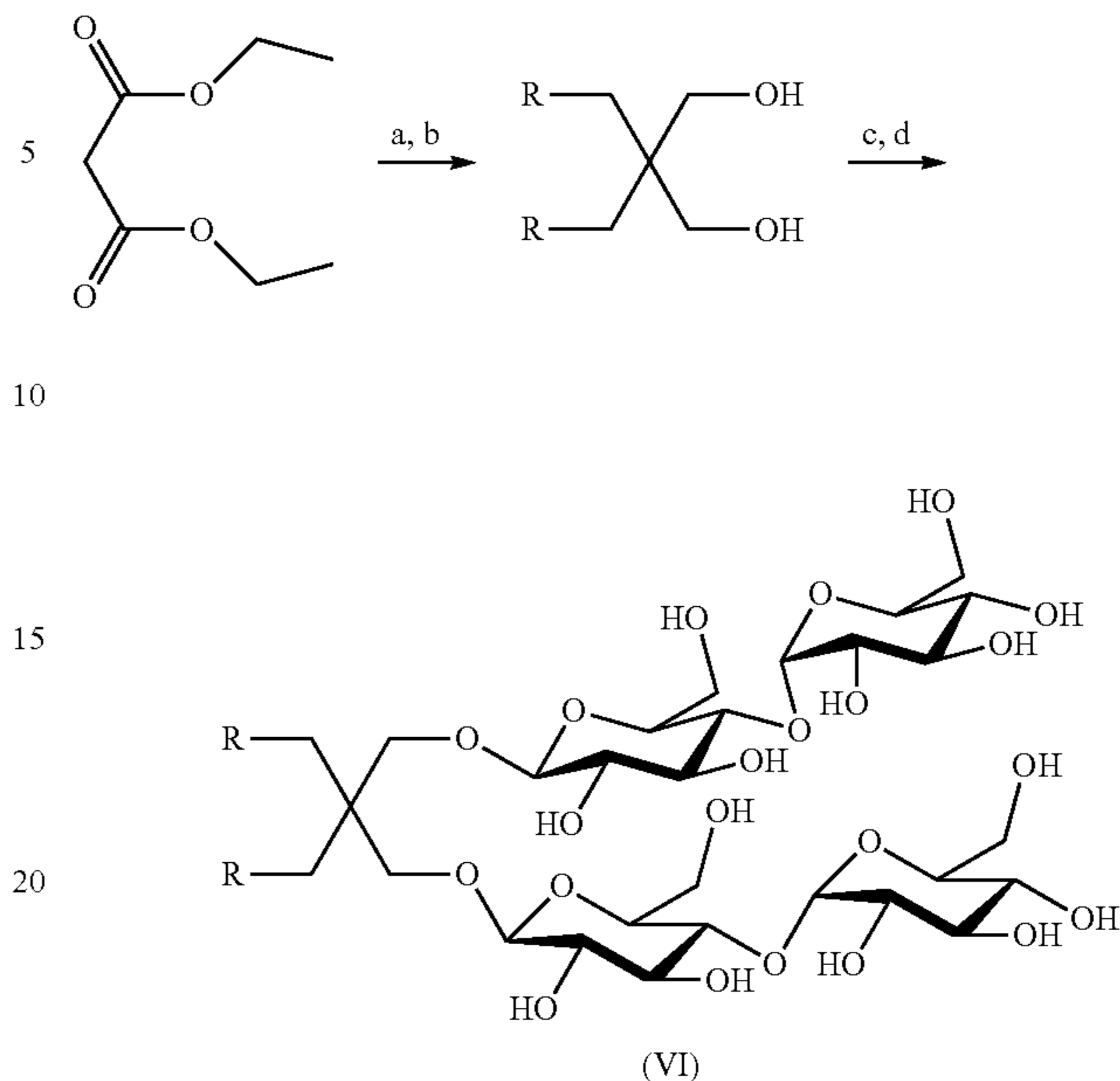
Scheme A. Preparation of Disaccharide Amphiphiles
