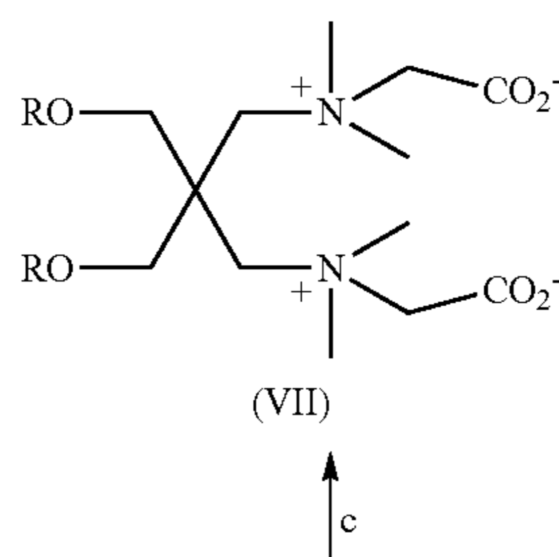
Scheme B. Preparation of Zwitterionic Amphiphiles
