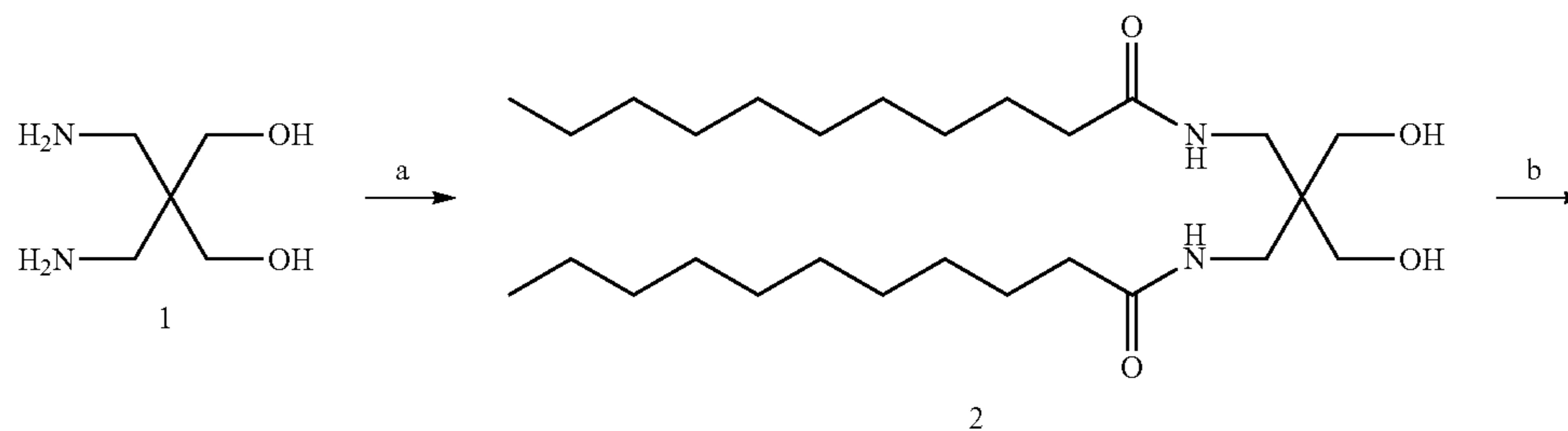
Scheme 1. Preparation of MNG Amphiphiles
