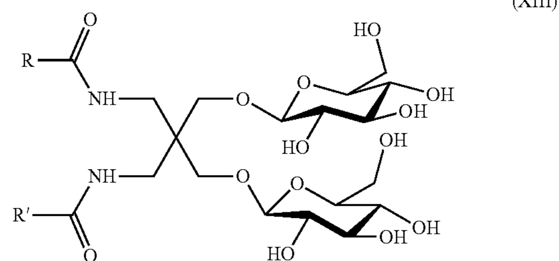
Scheme E. GNG Amphiphiles
