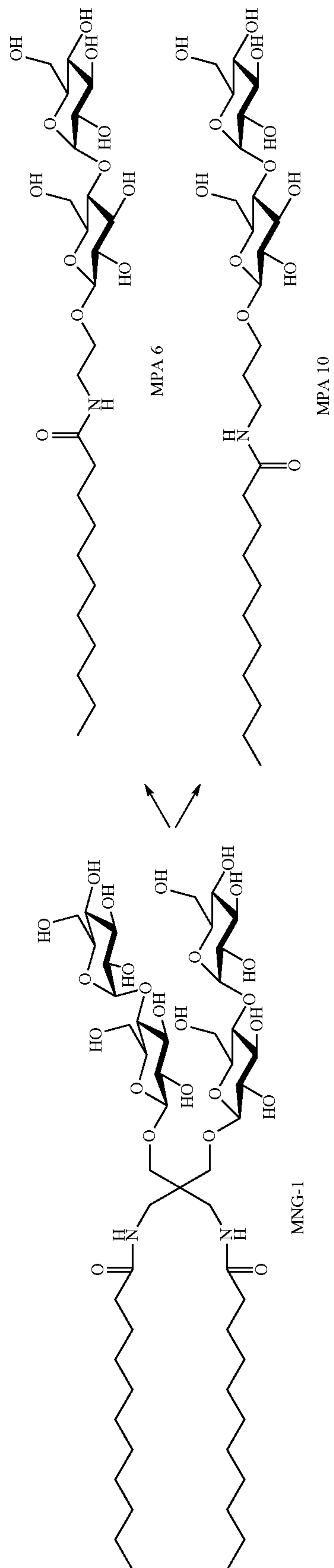
Scheme G. Specific MNG and MPA Amphiphiles
