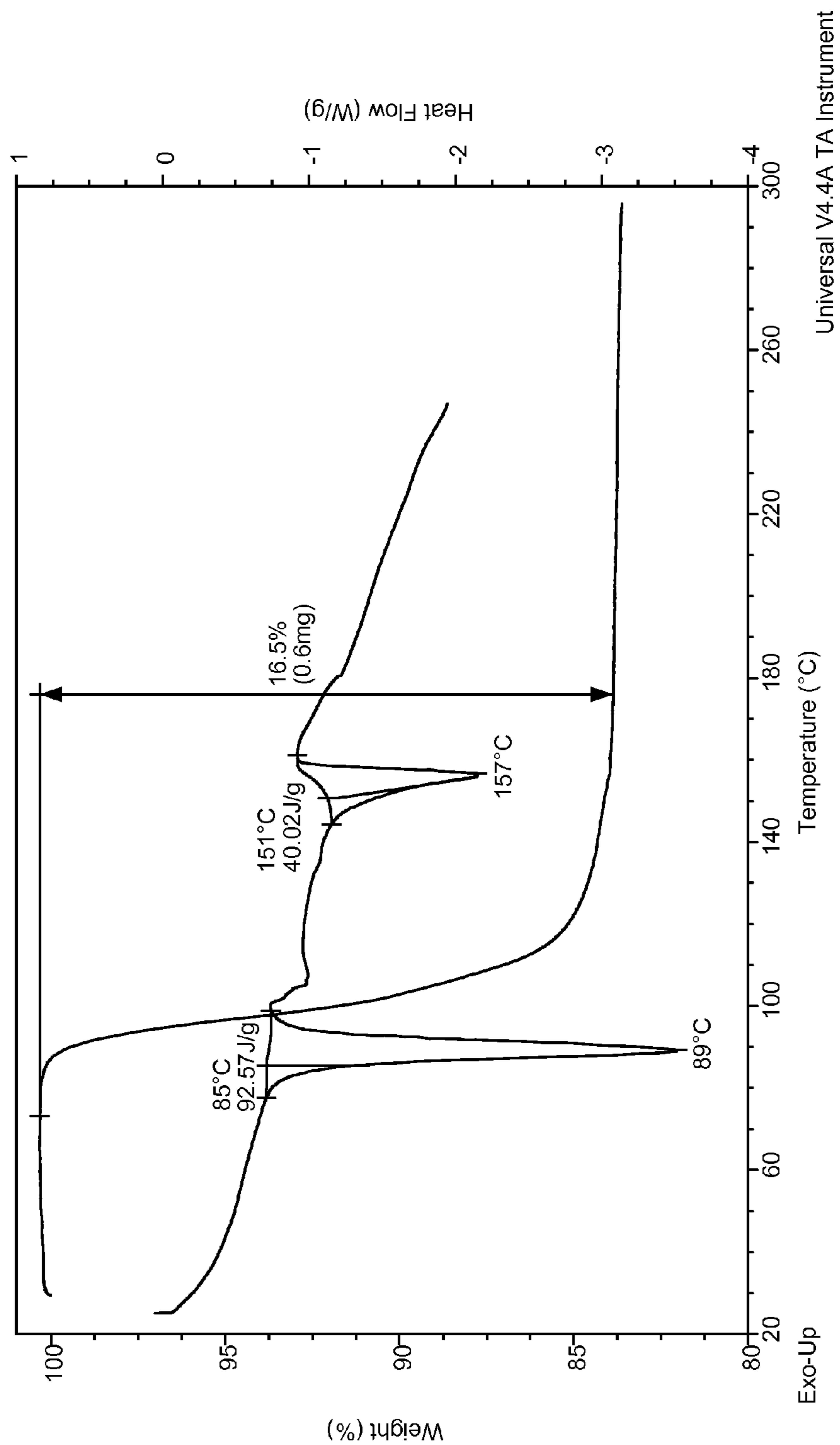
FIG. 15 TGA/DSC Thermograms of Form E
